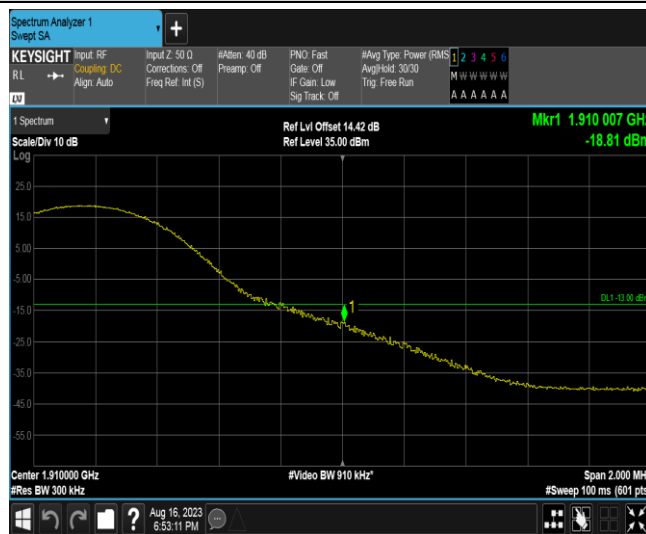
Band2-15MHz-QPSK-19125-1RB#74
