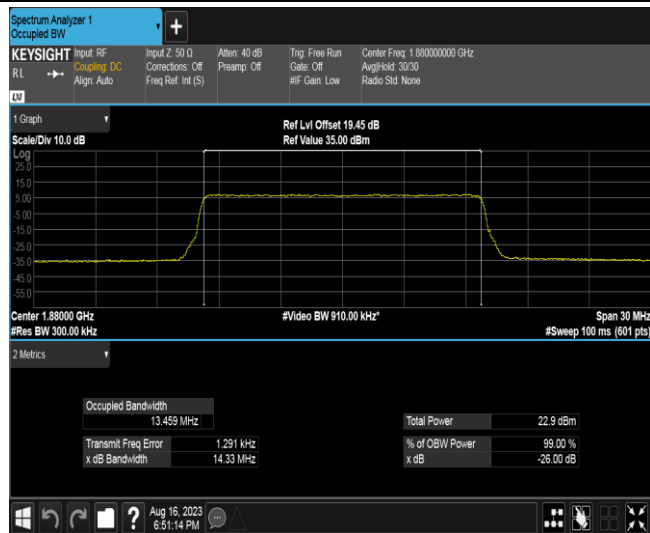
Band2-15MHz-16QAM-19125-75RB#0
