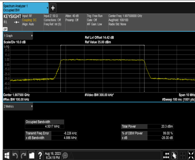
Band2-5MHz-QPSK-19175-25RB#0
