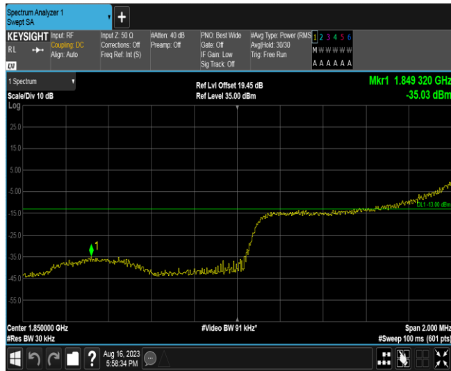
Band2-1.4MHz-QPSK-18607-6RB#0
