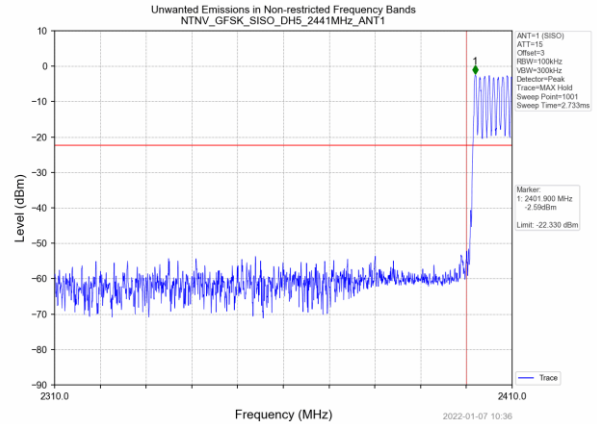
Hopping mode
