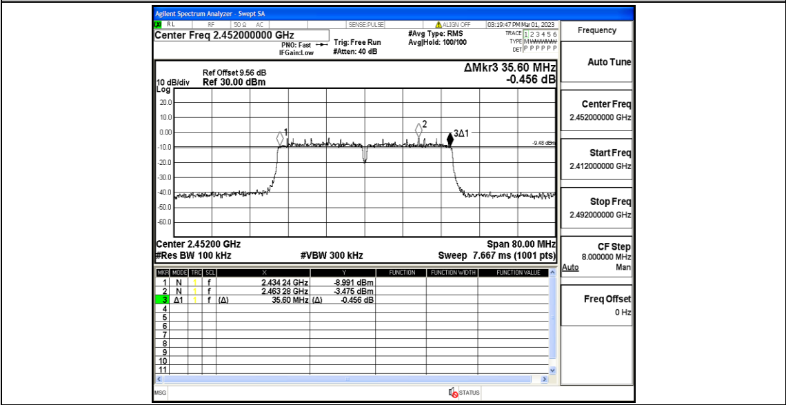
11N40SISO_Ant1_2452
