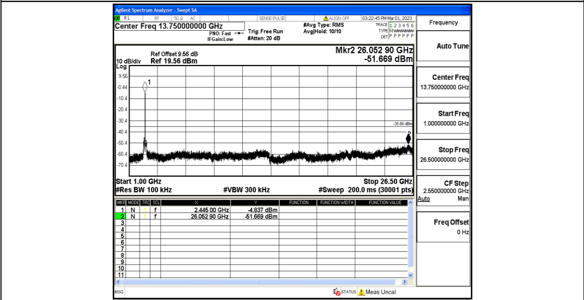
11N40SISO_Ant1_2452_1000~26500
