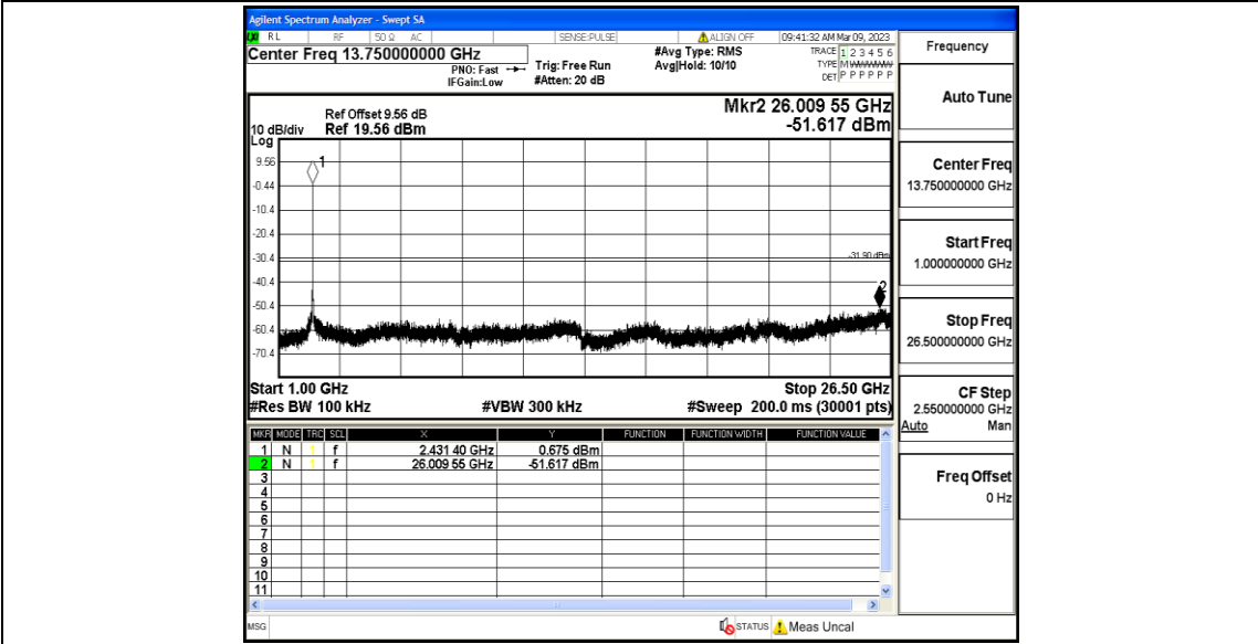
11G_Ant1_2437_1000~26500
