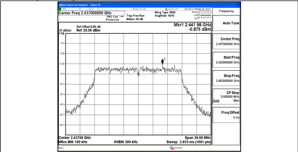
11N20SISO_Ant1_2437_0~Reference
