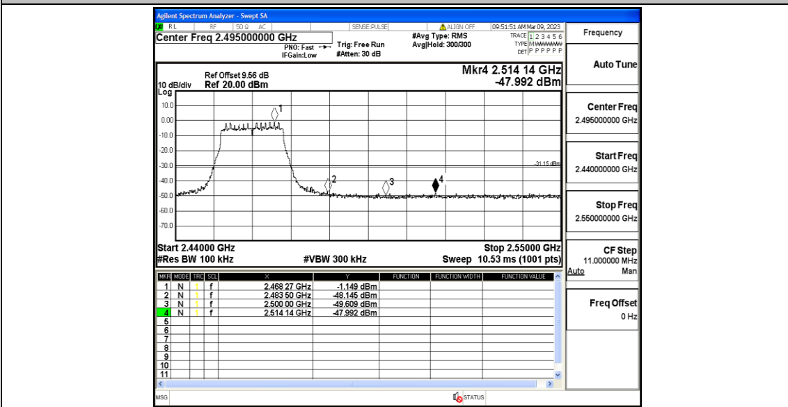
11N20SISO_Ant1_High_2462
