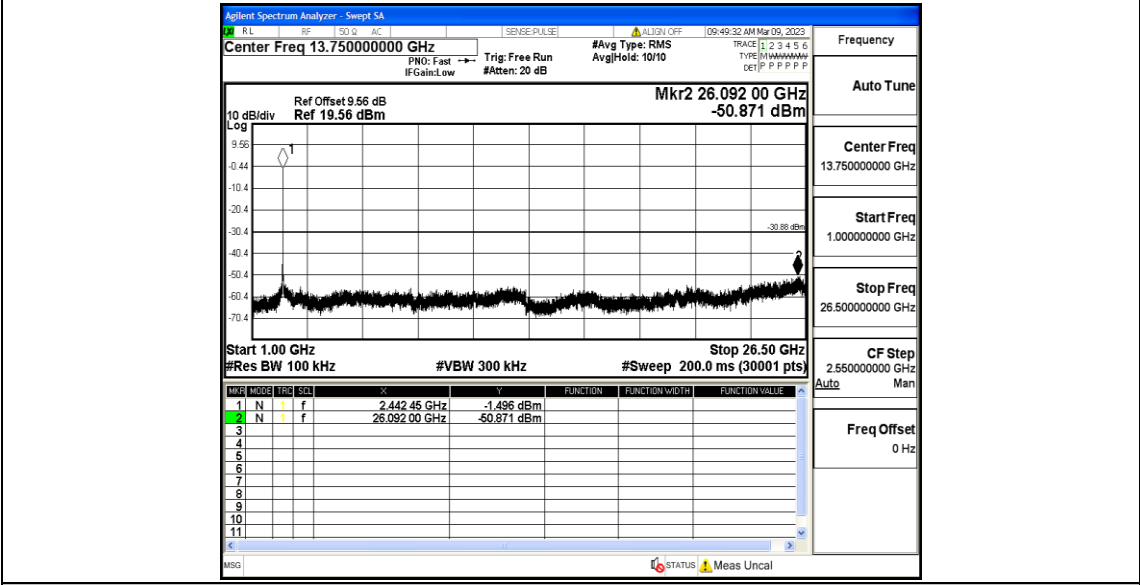
11N20SISO_Ant1_2437_1000~26500
