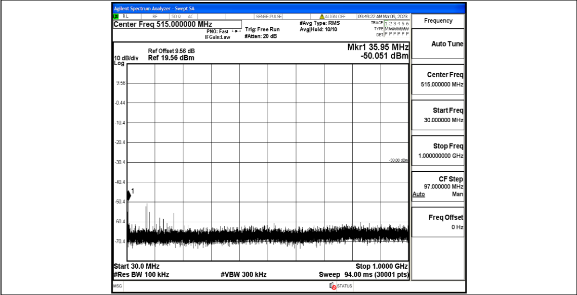
11N20SISO_Ant1_2437_30~1000
