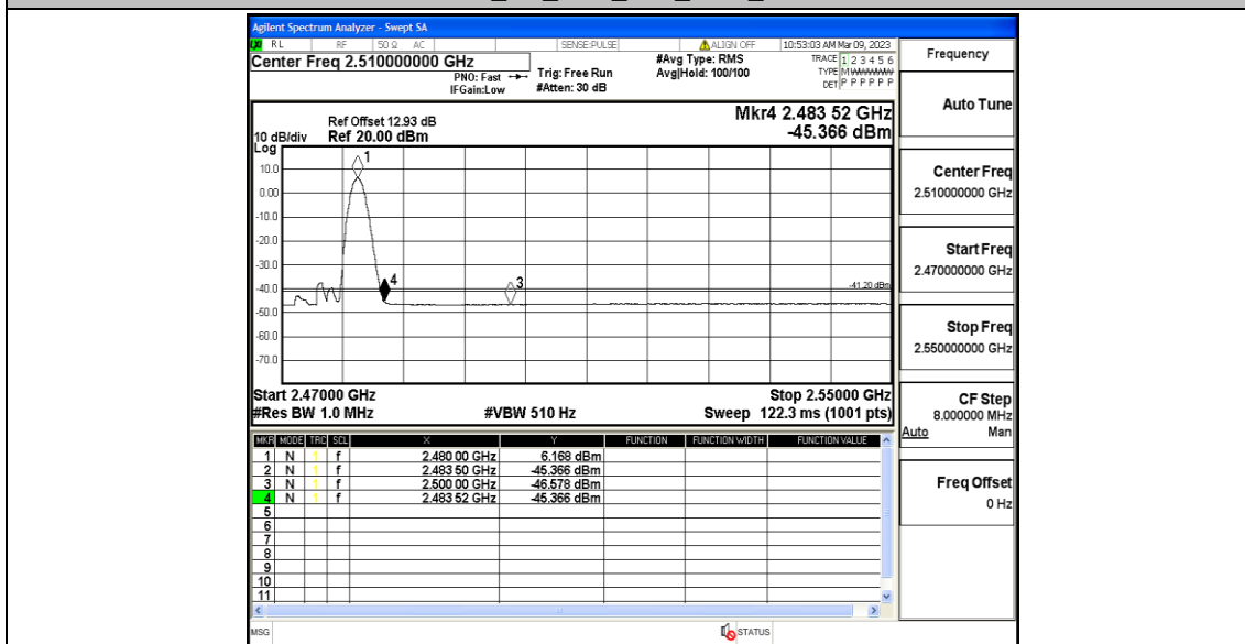
BLE_1M_Ant1_High_2480_AV
