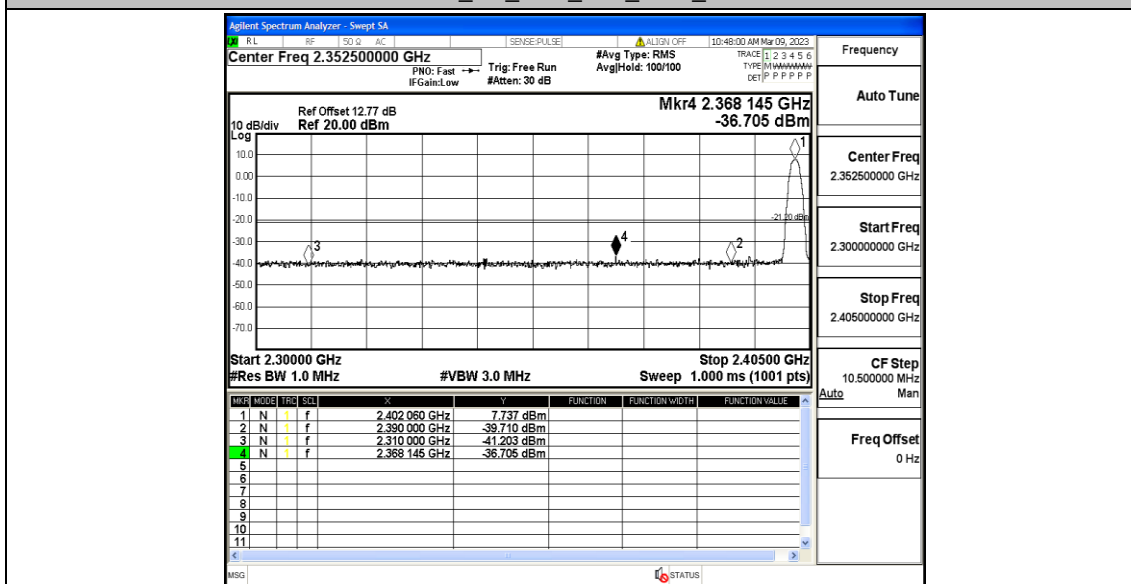
BLE_1M_Ant1_Low_2402_Peak
