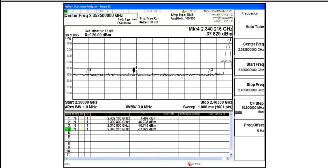
BLE_2M_Ant1_Low_2402_Peak
