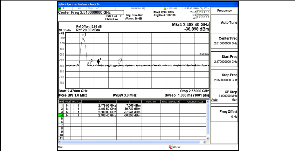
BLE_1M_Ant1_High_2480_Peak
