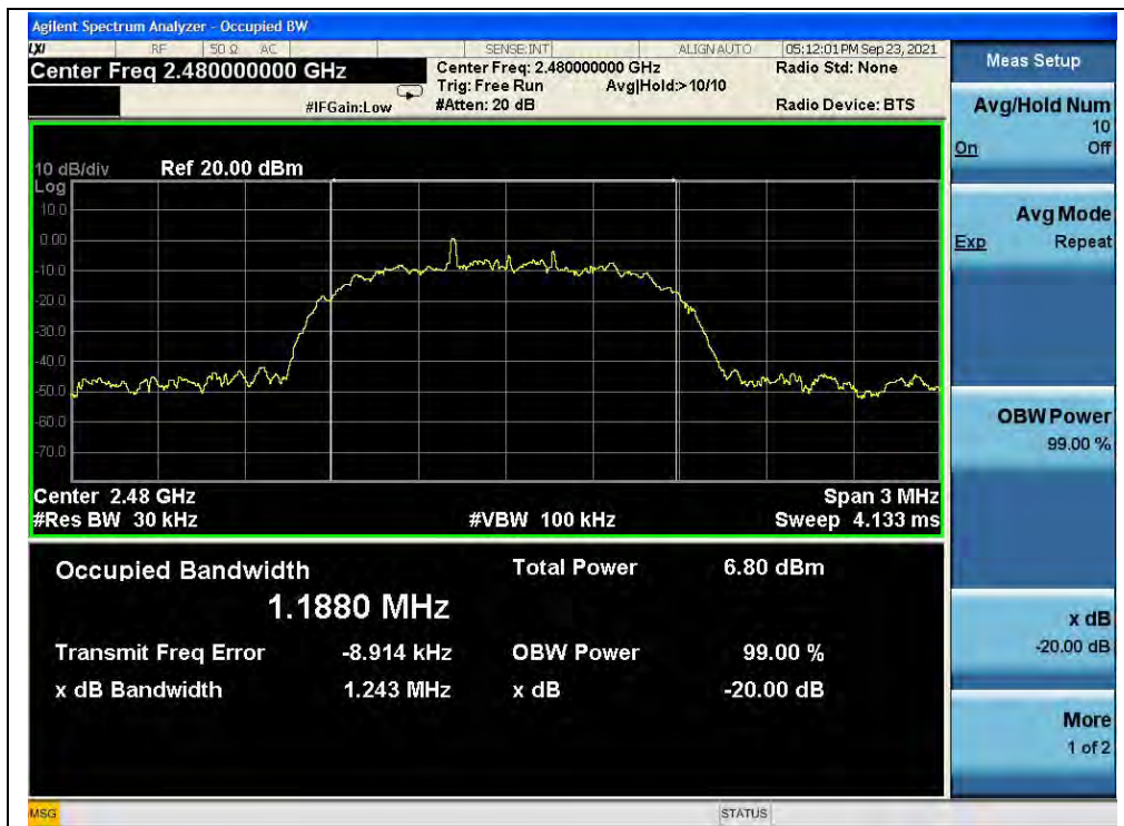
(Channel 78, 8-DPSK)
