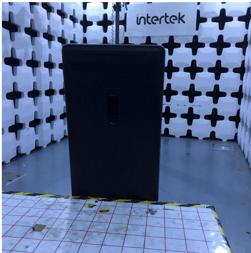
The EUT and transmitting antenna was centered on the turntable.
