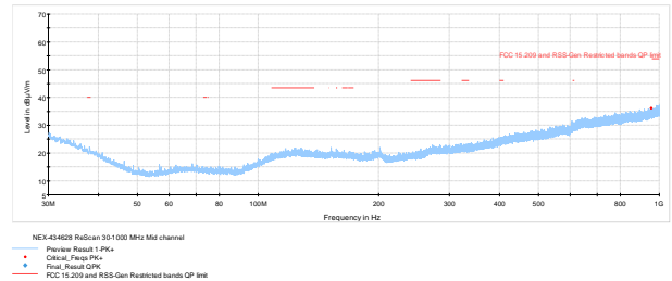
Figure 8.6-7: Radiated spurious emissions on Mid channel
