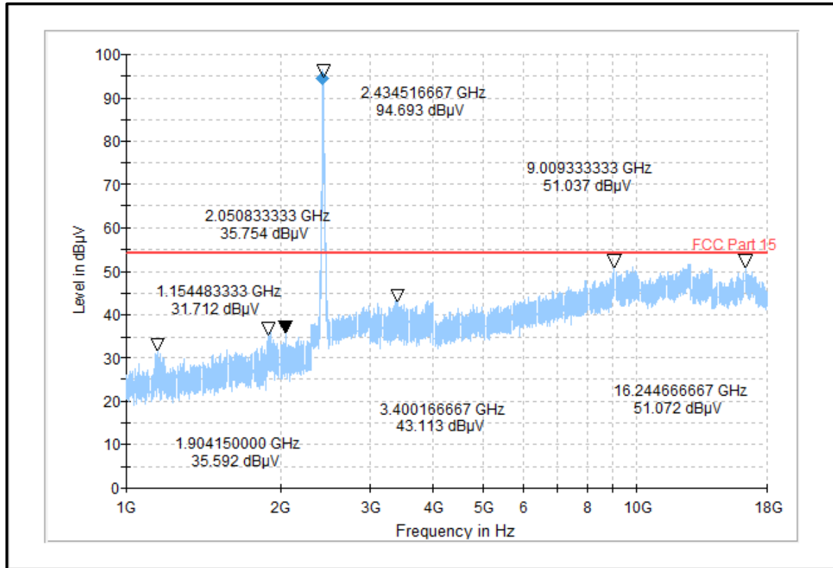
Plot: 1 GHz – 18GHz: 802.11g / 20 MHz / 6 Mbps / PWR 12 / Middle Channel
