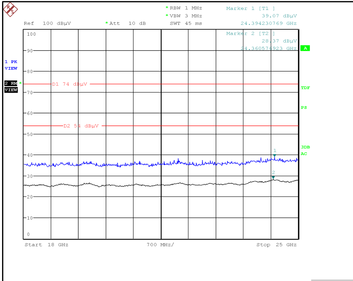
Plot: 18 GHz – 25 GHz: 802.11g / 20 MHz / 6 Mbps / PWR 12 / Middle Channel
