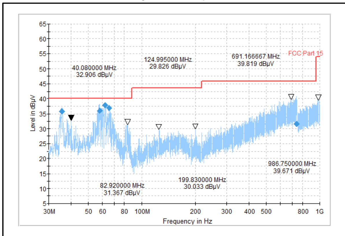
Plot: 30 MHz – 1GHz: 802.11g / 20 MHz / 6 Mbps / PWR 12 / Middle Channel
