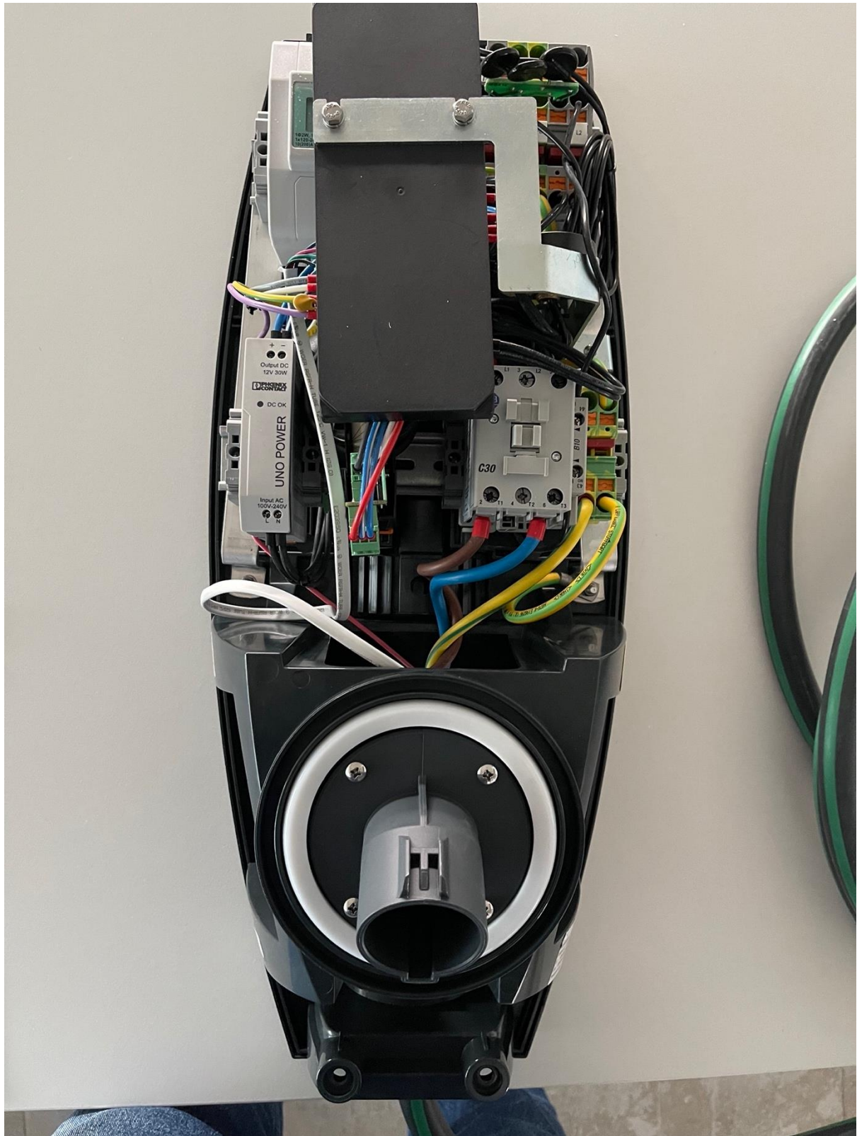
Internal view 1, top cover removed.
