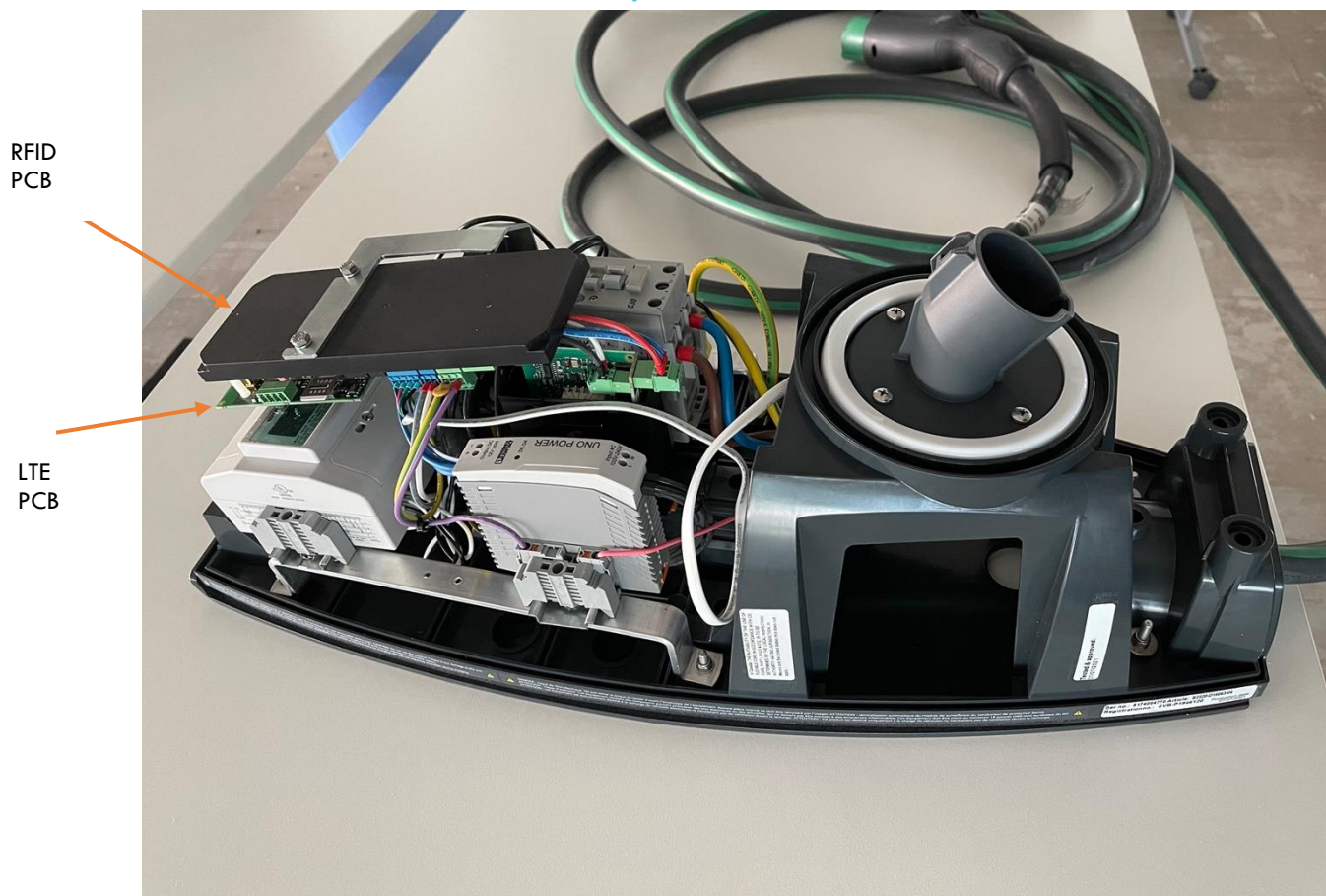
Internal view 2, Radio PCBs placement.
