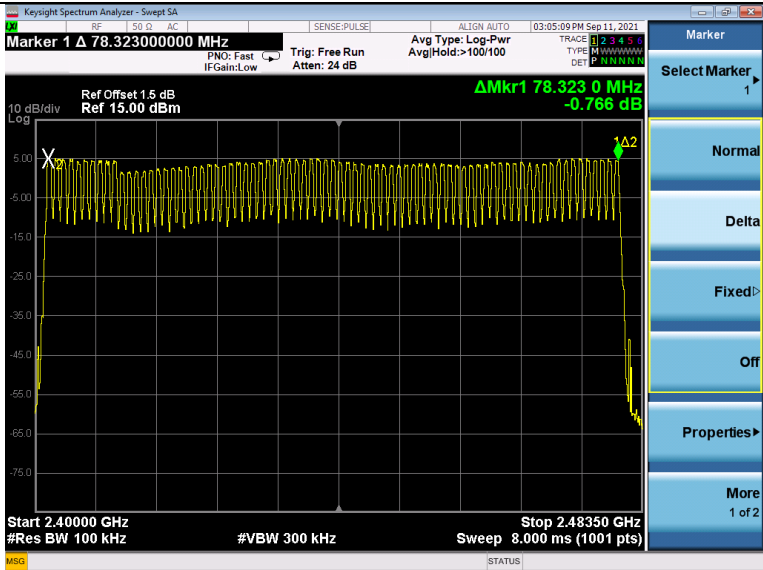
GFSK Modulation
