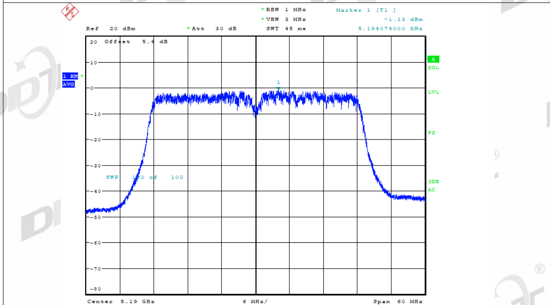
PSD NVNT n40 5190MHz Ant2
