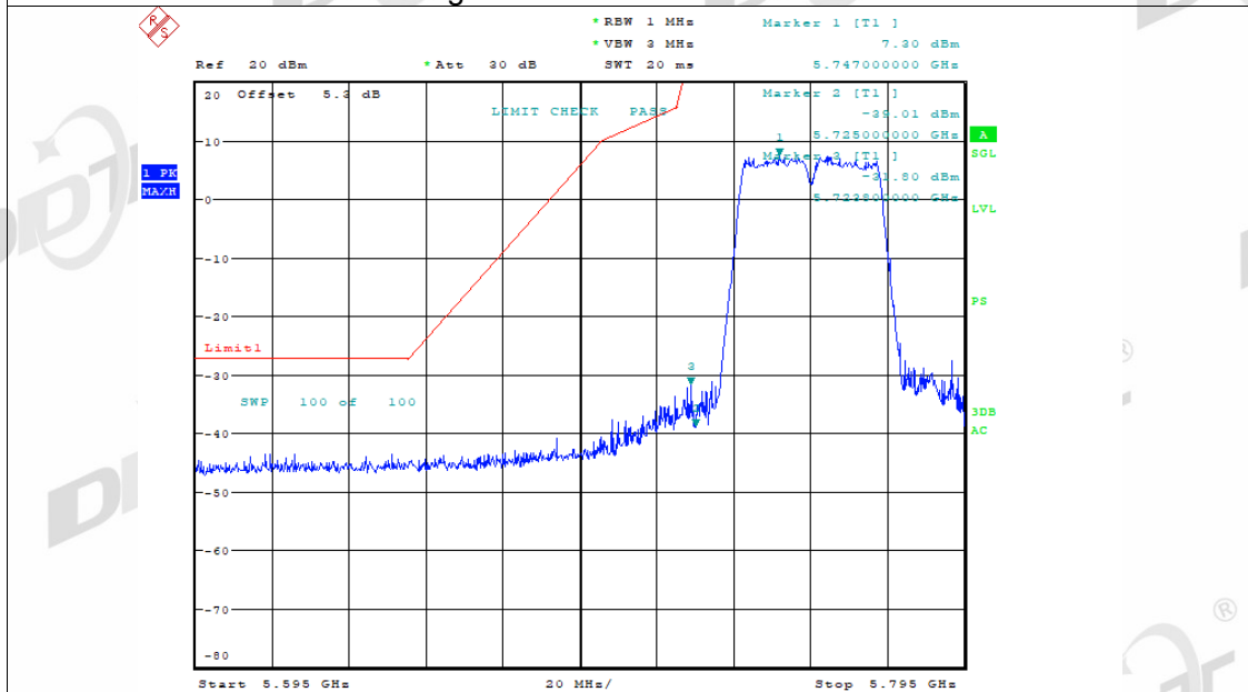
Band Edge NVNT ac40 5755MHz Low Ant2
