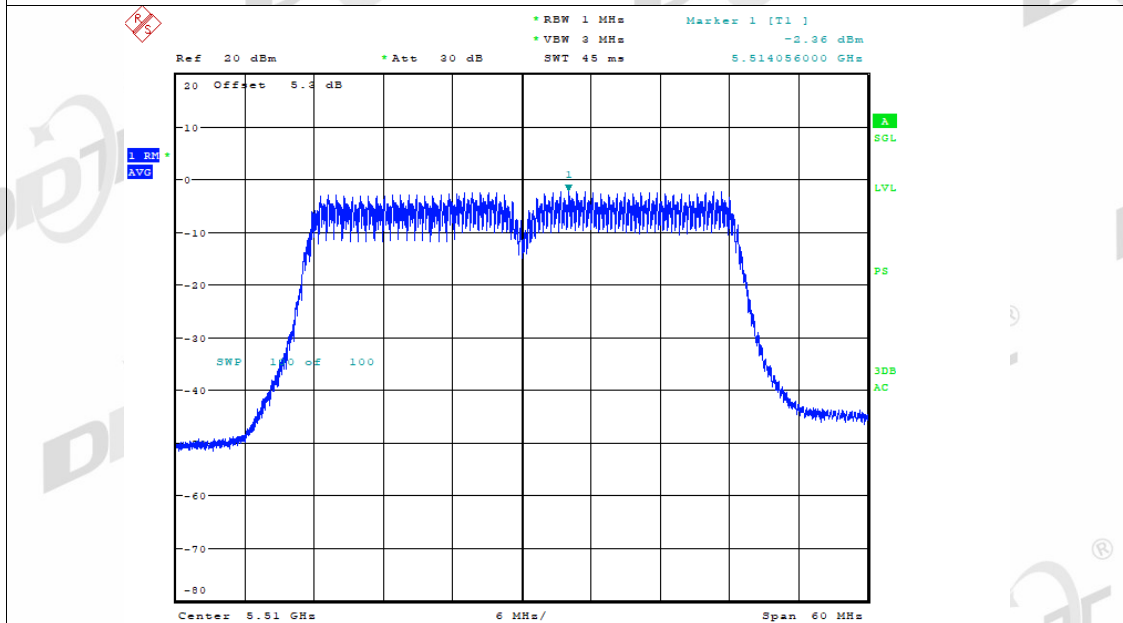
PSD NVNT n40 5510MHz Ant2
