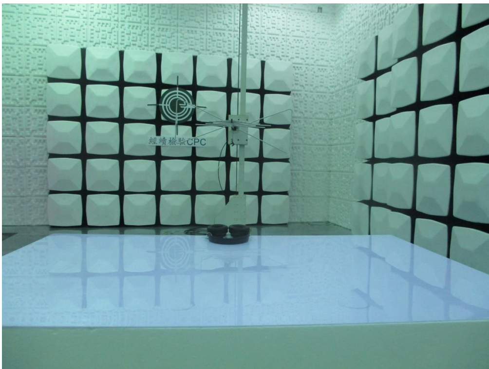
Setup Photo FCC ID: 2A3AP-ANC-HB111
