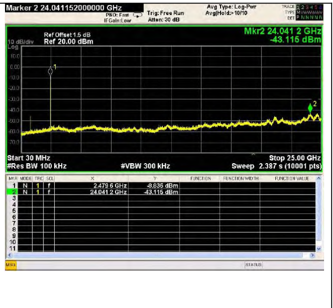
Test Mode: EDR--High
