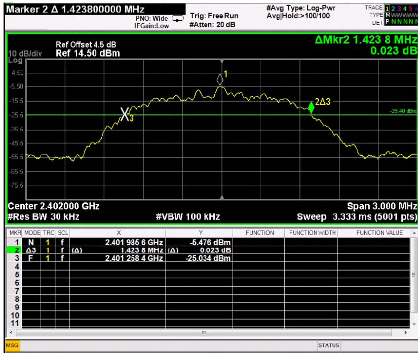
Test Mode: EDR---Low
