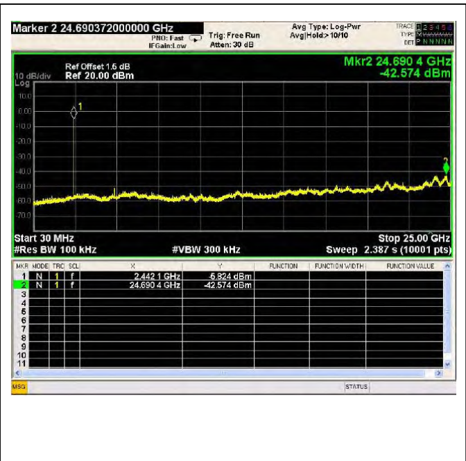
Test Mode: BDR---Mid
