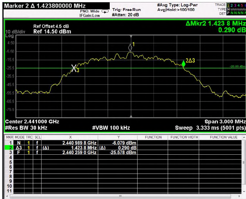
Test Mode: EDR---Middle
