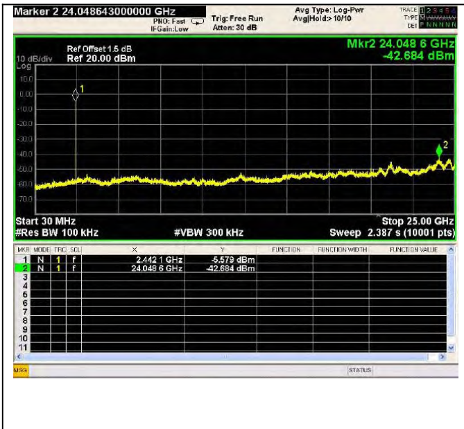
Test Mode: EDR---Mid
