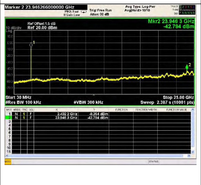
Test Mode: EDR---Low
