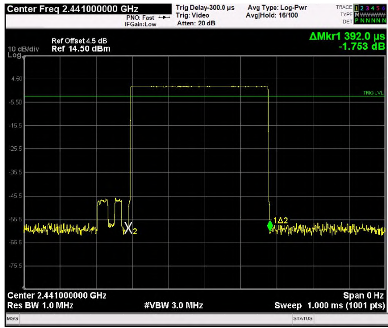
Test Mode: EDR---3DH1
