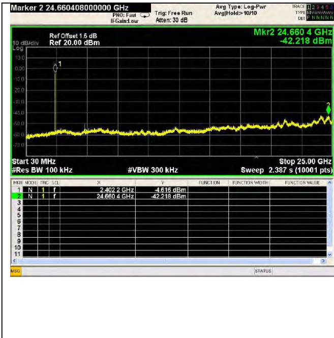
Test Mode: BDR---Low
