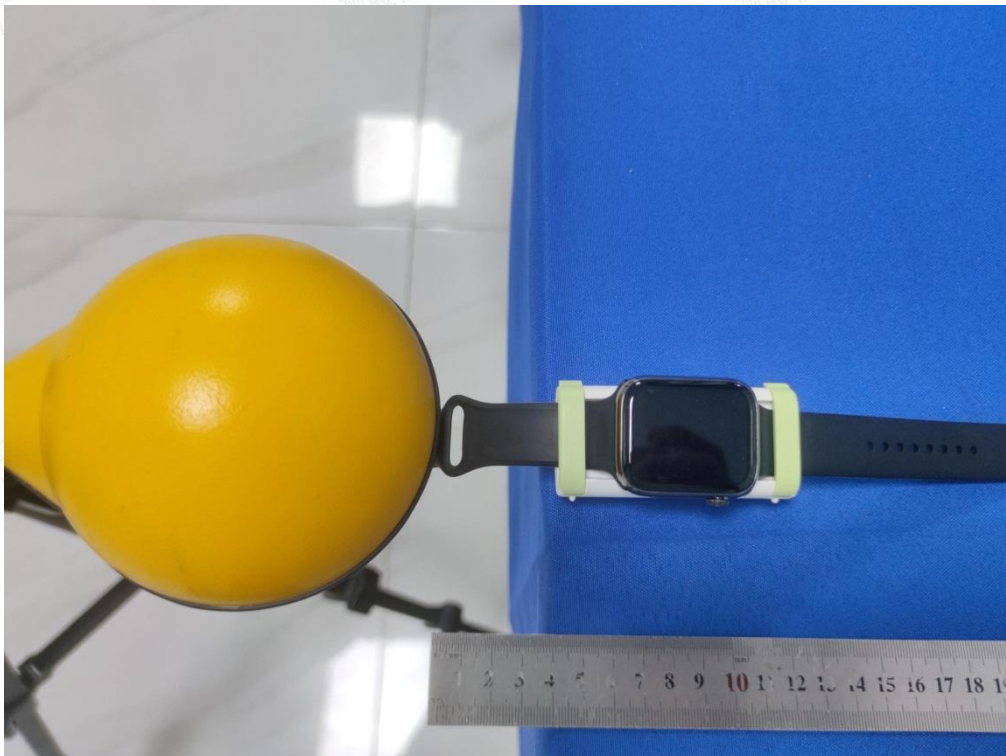
Test Position E(4cm) - Exposure photo from side edge surface-Right(TM1)
