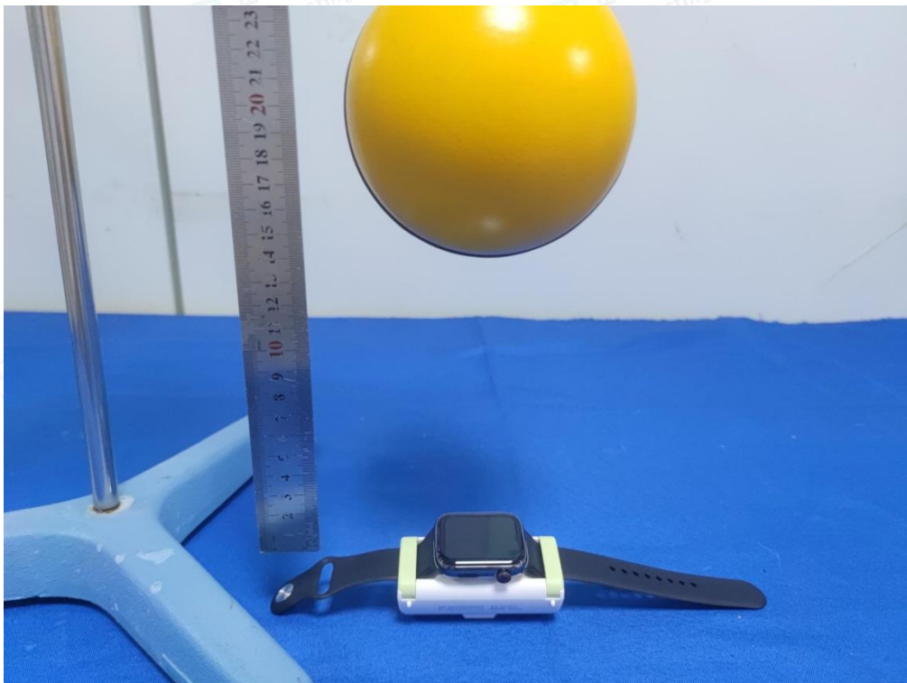
Test Position A (14cm) - Exposure photo from top surface (TM1)
