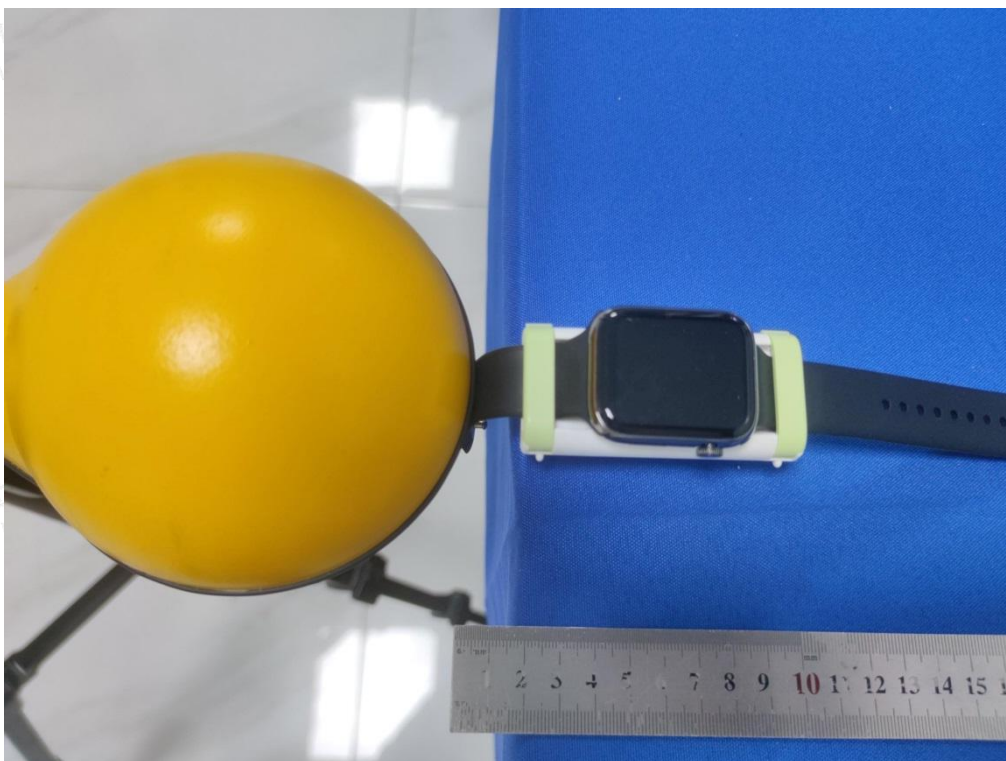
Test Position E(2cm) - Exposure photo from side edge surface-Right(TM1)
