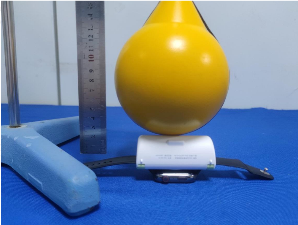
Test Position F(0cm) - Exposure photo from bottom surface(TM1)
