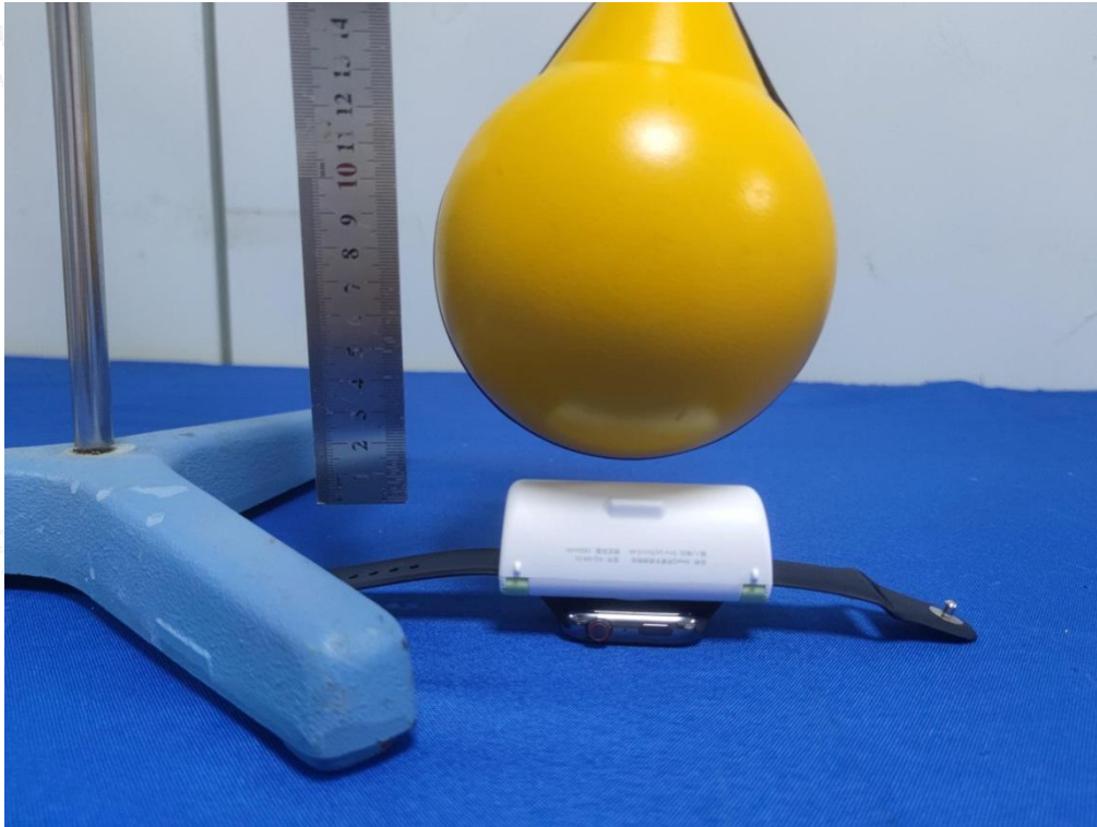
Test Position F(2cm) - Exposure photo from bottom surface(TM1)
