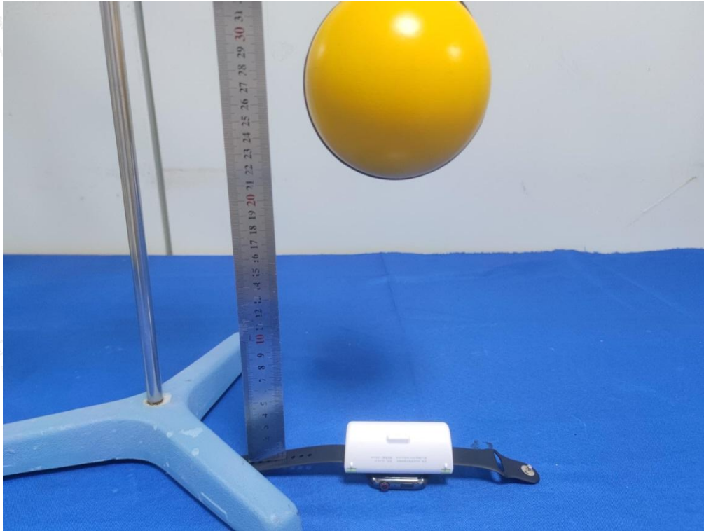
Test Position F(20cm) - Exposure photo from bottom surface(TM1)
