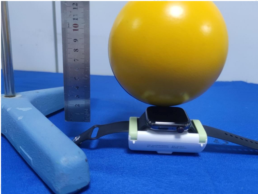
Test Position A (0cm) - Exposure photo from top surface (TM1)
