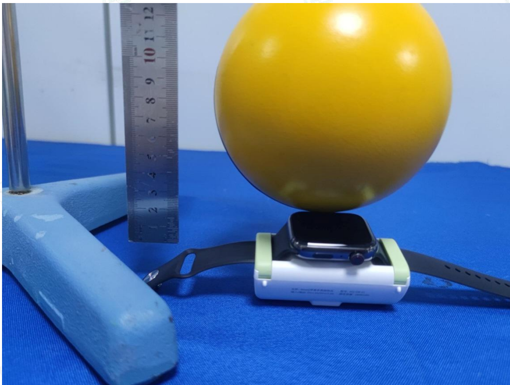
Test Position A (2cm) - Exposure photo from top surface (TM1)
