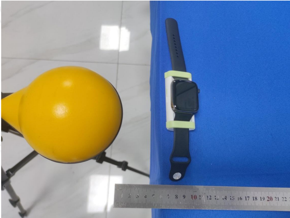
Test Position D(6cm) - Exposure photo from side edge surface-Front(TM1)
