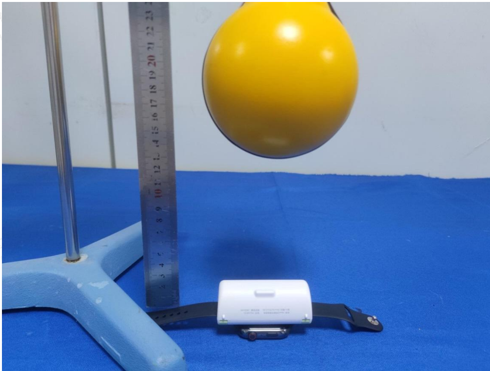
Test Position F(12cm) - Exposure photo from bottom surface(TM1)
