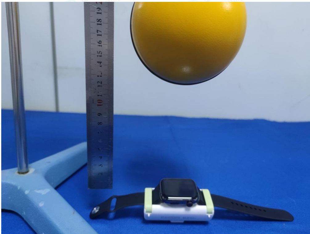
Test Position A (12cm) - Exposure photo from top surface (TM1)
