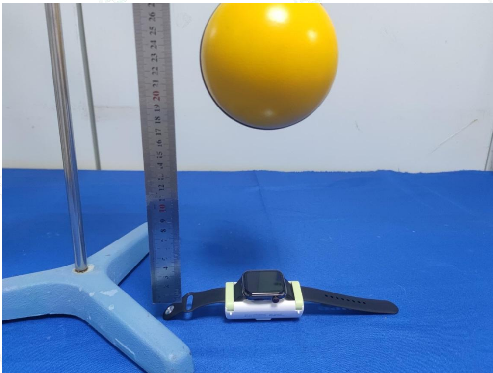
Test Position A (16cm) - Exposure photo from top surface (TM1)
