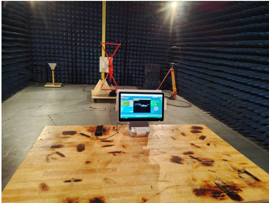
Radiated Test Setup Photograph(HK528 (second display:15.6 inch))
