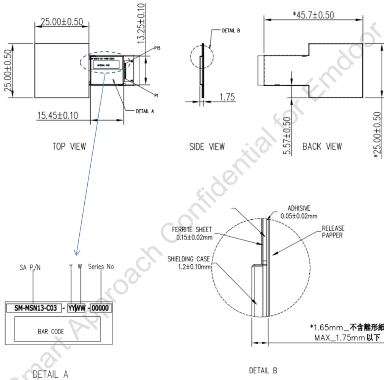
Figure 8 Antenna Module Drawing
