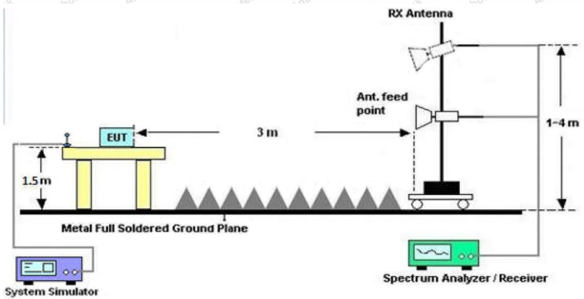
Figure 3. Above 1 GHz
