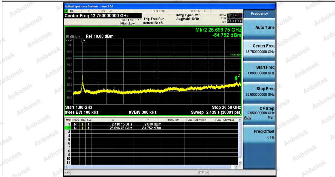
11B_Ant2_2412_0~Reference
