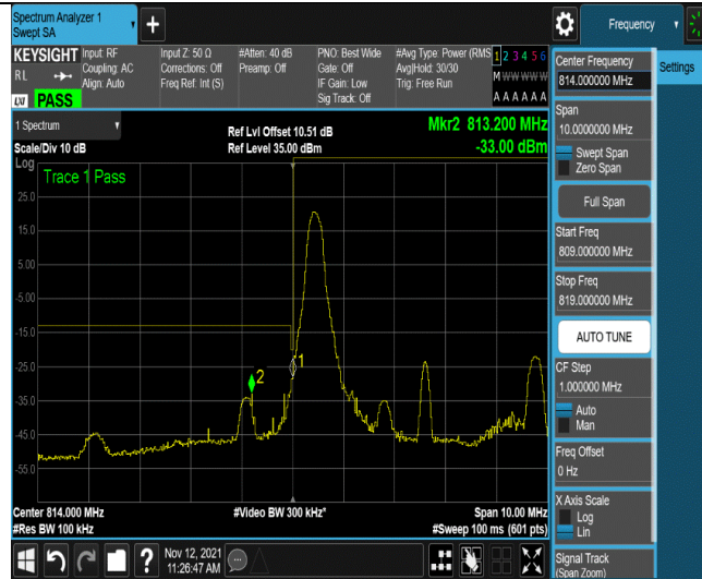
Band26-5MHz-16QAM-26715-1RB#24
