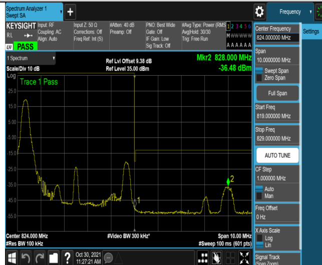
Band26-5MHz-16QAM-26765-1RB#24
