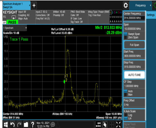
Band26-3MHz-16QAM-26705-1RB#14
