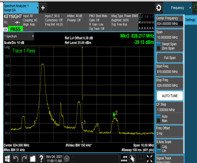
Band26-3MHz-16QAM-26775-1RB#14
