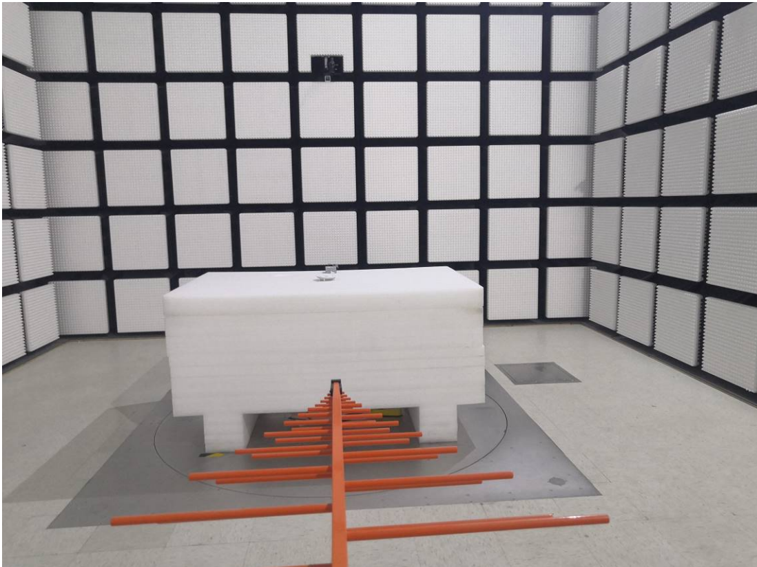
Radiated Emission Below 1GHz View EPCL-WIFI-RGBCW-4INCH- Power Drive 4#
