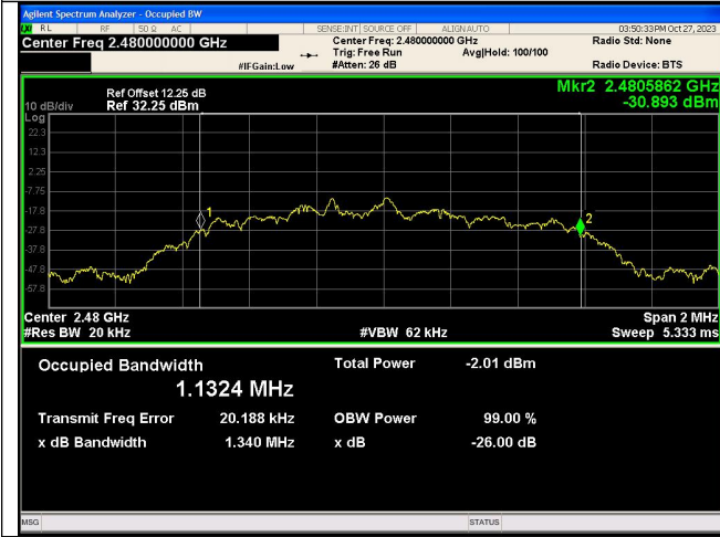
8DPSK_3-DH5_Channel 78
