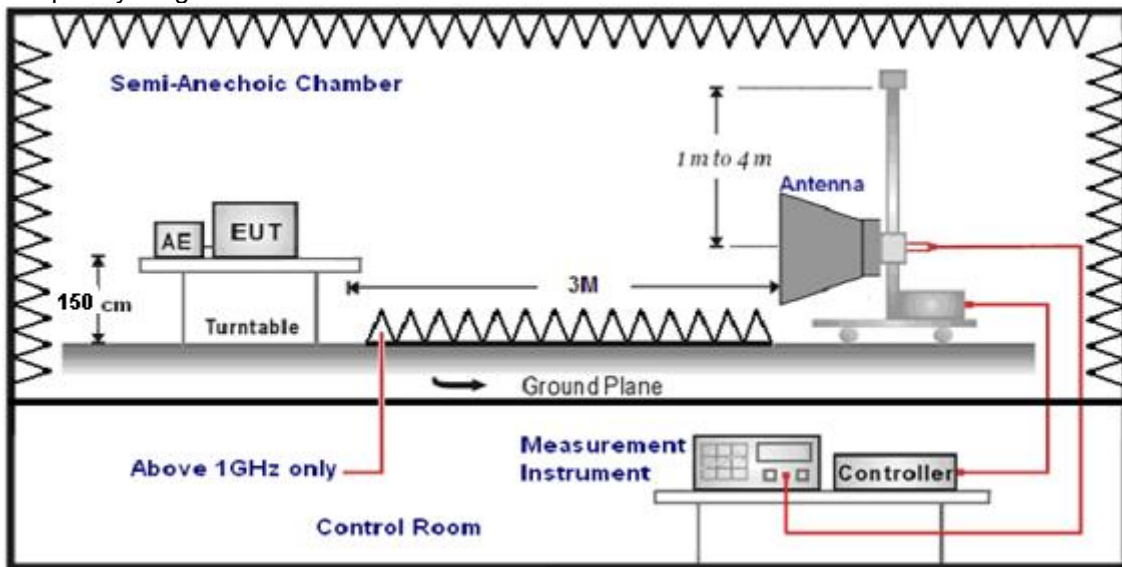
Frequency range above 1GHz-25GHz
