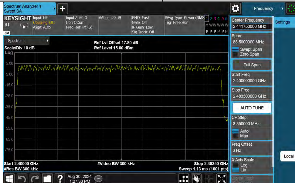
3DH5-Ant1-Hop-PASS
