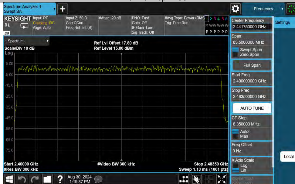
3DH5-Ant1-Hop-PASS
