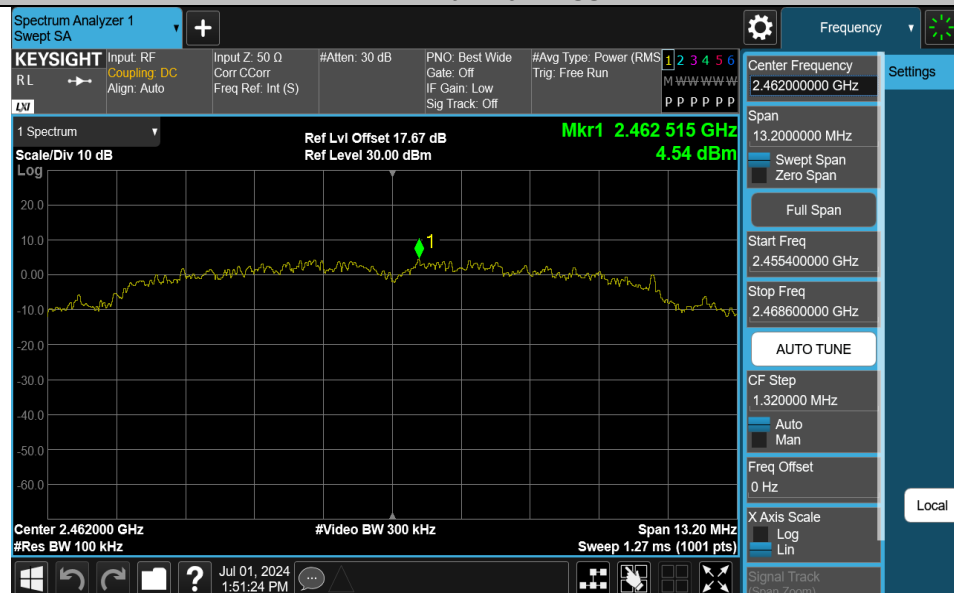
11B-Ant1-2462-PASS
