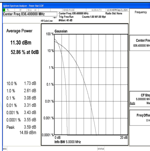
Channel 4182/ 836.4 MHz
