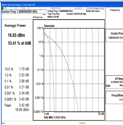
Channel 9400 / 1880.0 MHz
