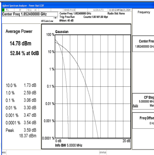
Channel 9262 / 1852.4 MHz
