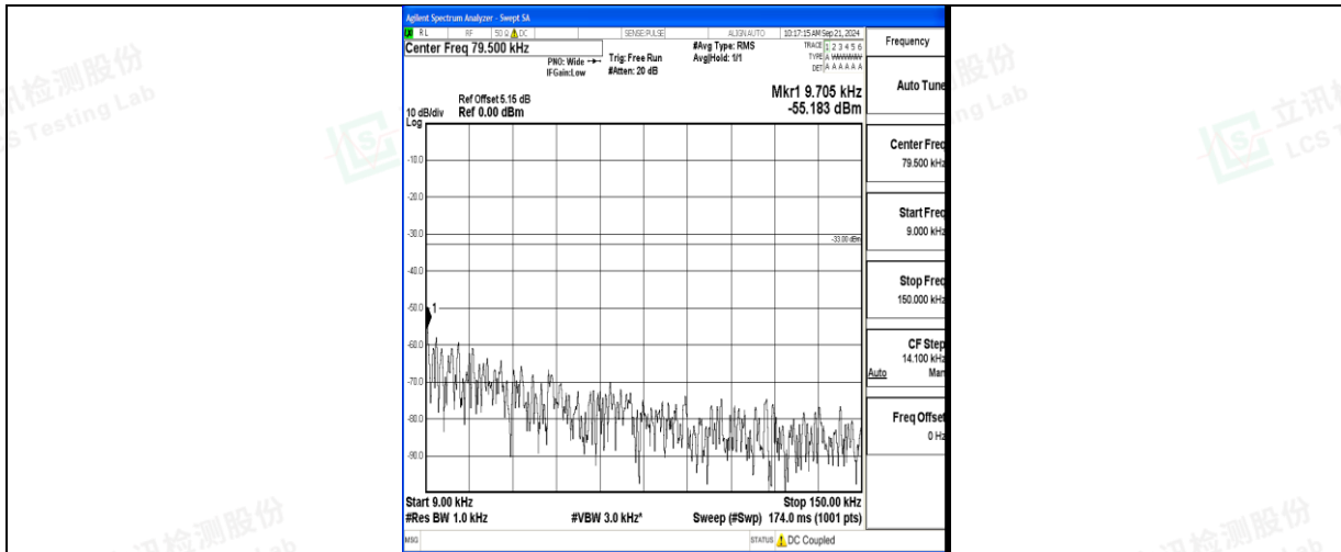
Band71_15MHz_QPSK_133197_1RB#0_0.009~0.15_0.009~0.15
