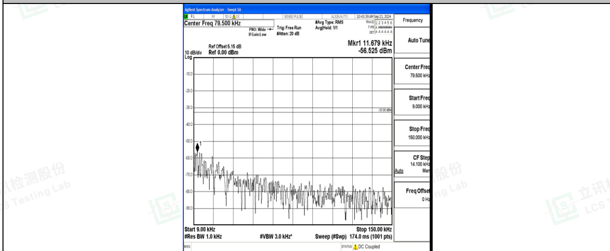
Band71_20MHz_16QAM_133222_1RB#0_0.009~0.15_0.009~0.15
