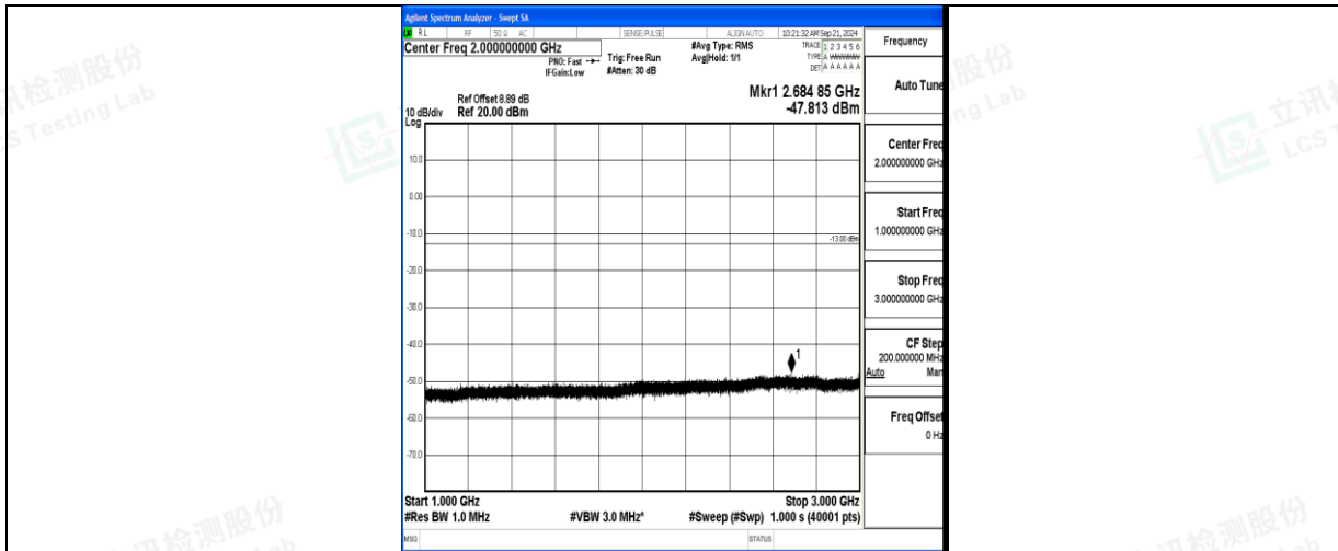
Band71_15MHz_16QAM_133297_1RB#0_1000~3000_1000~3000
