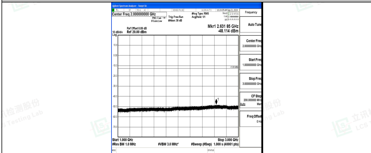
Band71_15MHz_16QAM_133397_1RB#0_1000~3000_1000~3000
