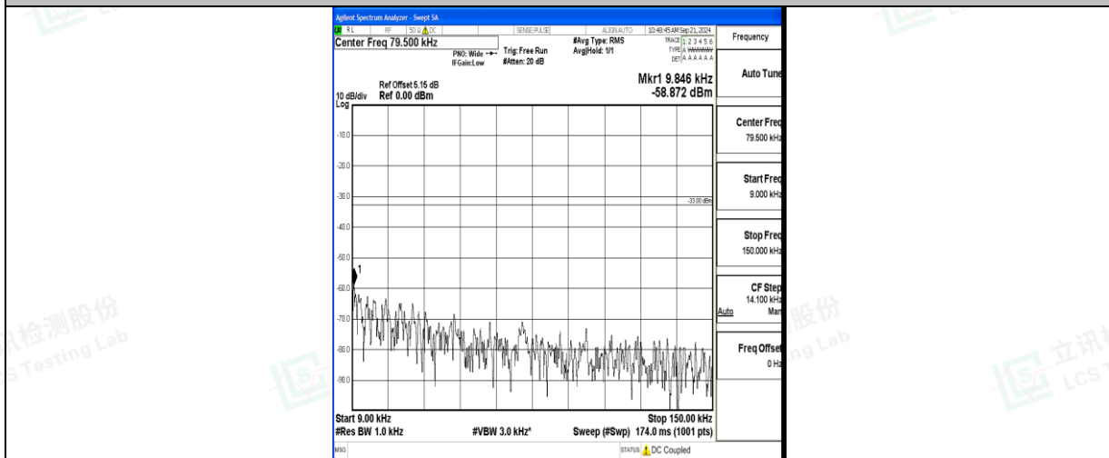
Band71_20MHz_16QAM_133372_1RB#0_0.009~0.15_0.009~0.15
