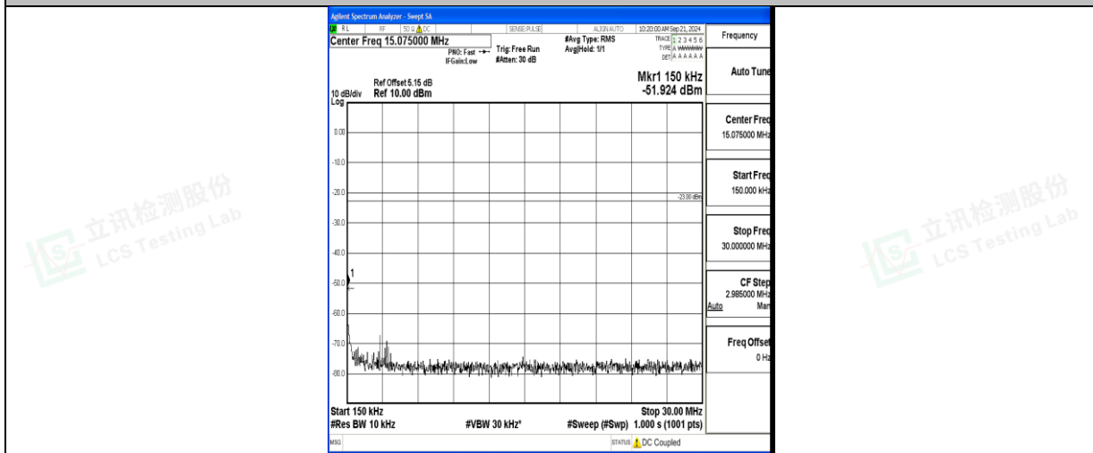
Band71_15MHz_QPSK_133297_1RB#0_0.15~30_0.15~30
