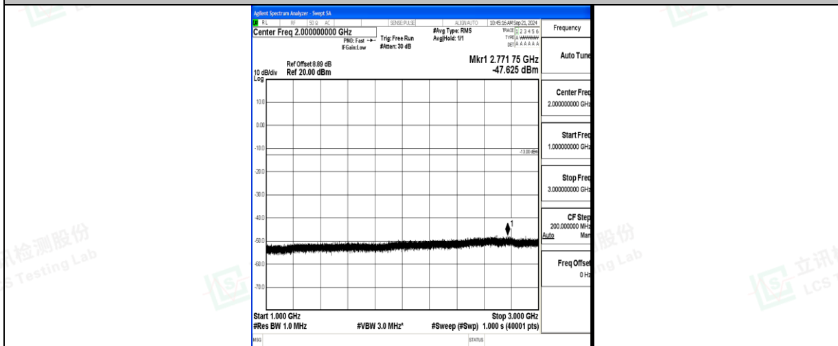
Band71_20MHz_QPSK_133322_1RB#0_1000~3000_1000~3000
