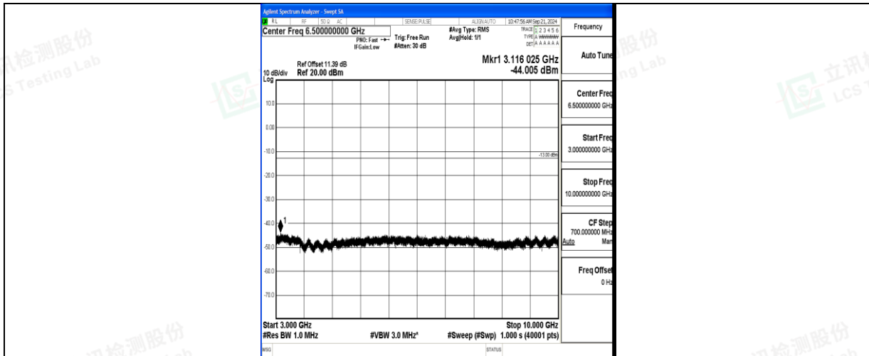
Band71_20MHz_QPSK_133372_1RB#0_3000~10000_3000~10000
