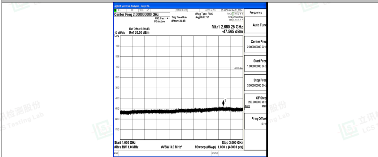
Band71_20MHz_16QAM_133222_1RB#0_1000~3000_1000~3000
