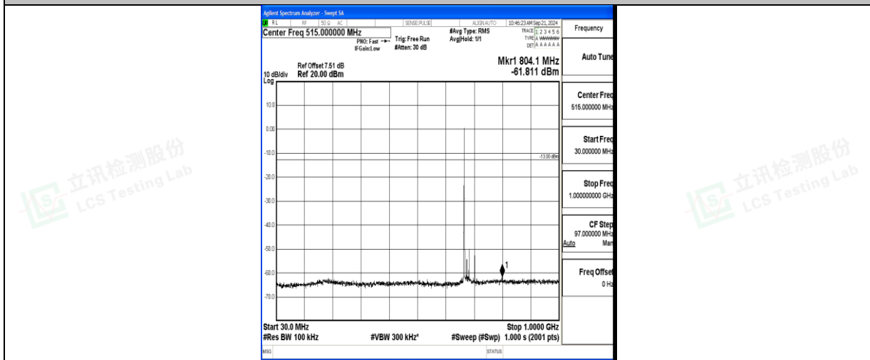
Band71_20MHz_16QAM_133322_1RB#0_30~1000_30~1000
