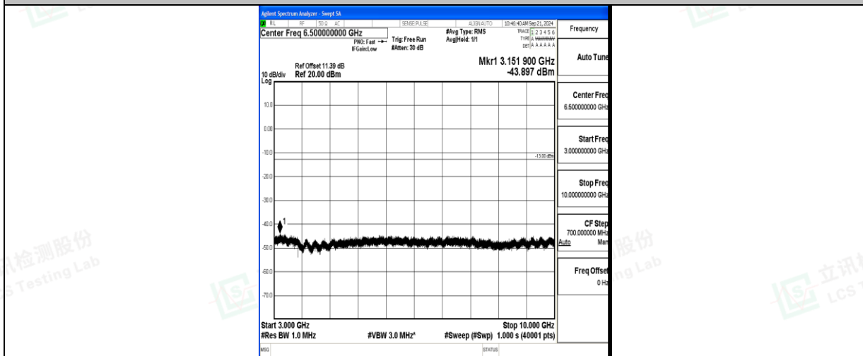
Band71_20MHz_16QAM_133322_1RB#0_3000~10000_3000~10000
