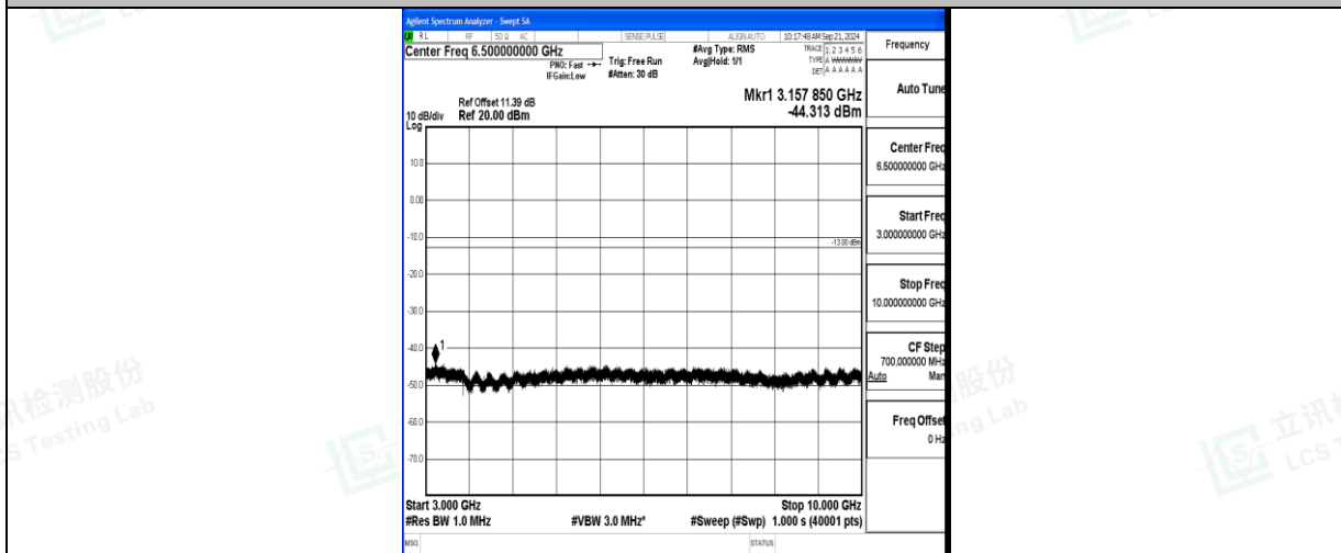
Band71_15MHz_QPSK_133197_1RB#0_3000~10000_3000~10000
