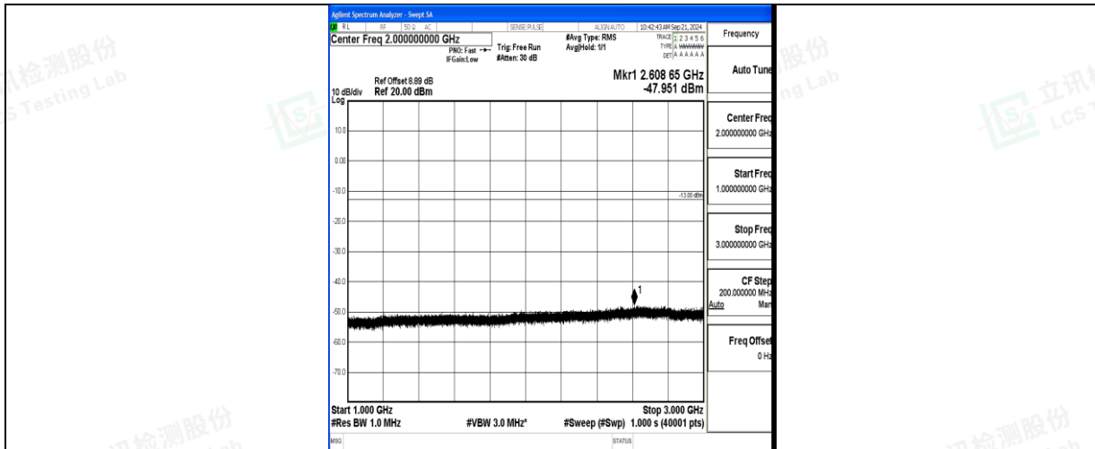
Band71_20MHz_QPSK_133222_1RB#0_1000~3000_1000~3000
