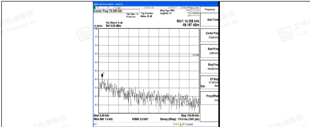
Band71_20MHz_16QAM_133322_1RB#0_0.009~0.15_0.009~0.15
