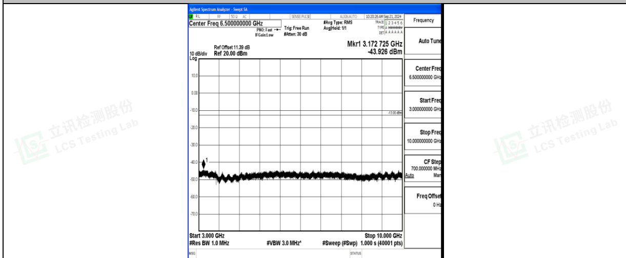
Band71_15MHz_QPSK_133297_1RB#0_3000~10000_3000~10000
