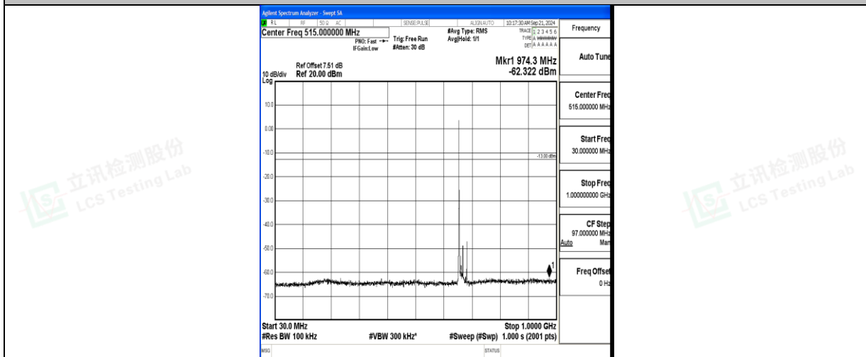
Band71_15MHz_QPSK_133197_1RB#0_30~1000_30~1000
