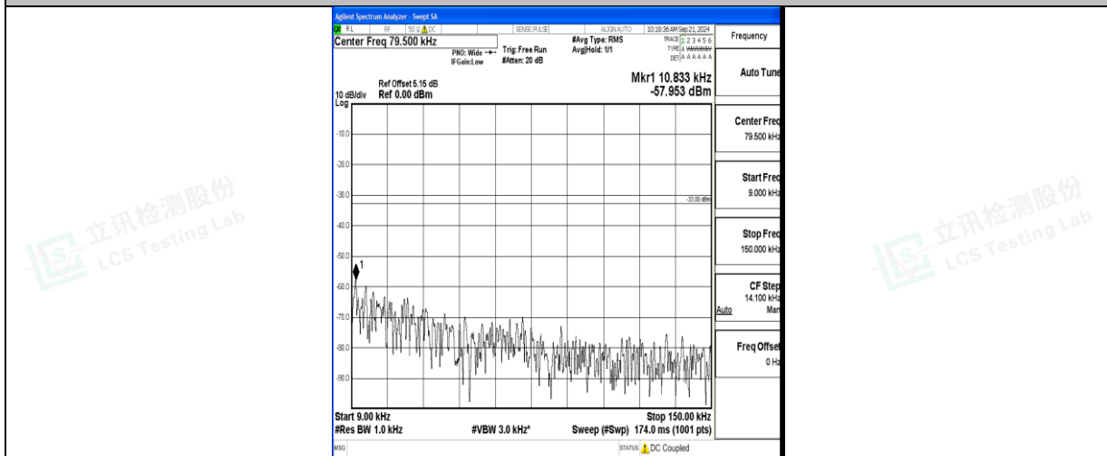
Band71_15MHz_16QAM_133197_1RB#0_0.009~0.15_0.009~0.15
