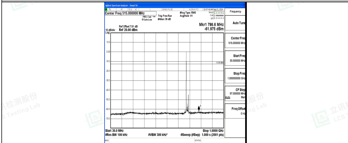
Band71_20MHz_QPSK_133372_1RB#0_30~1000_30~1000
