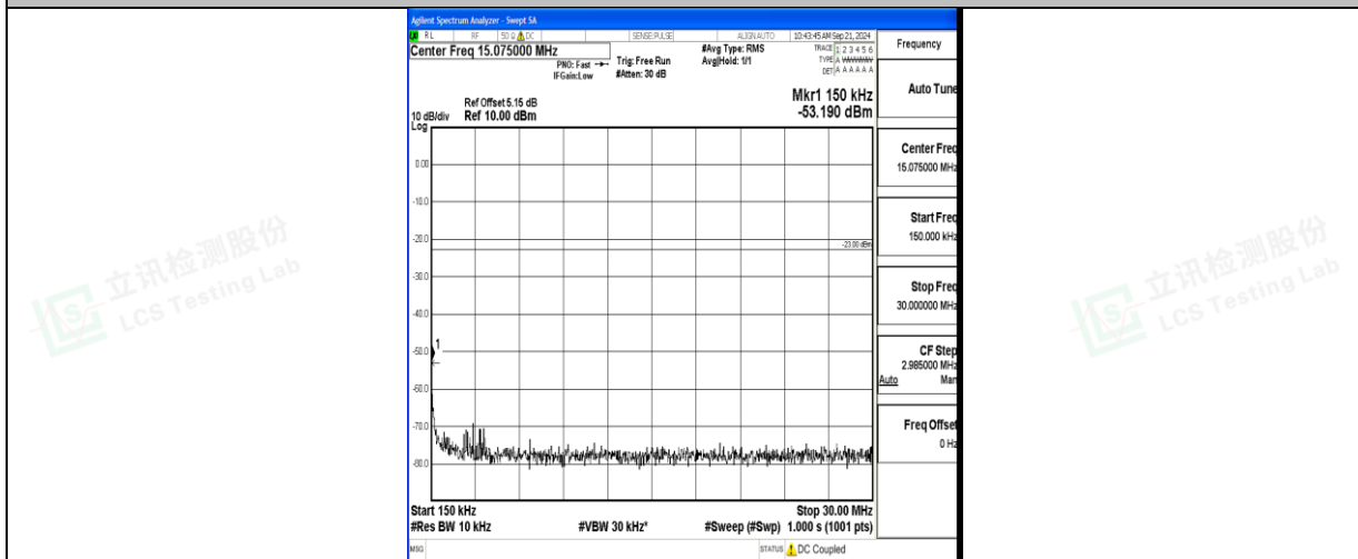
Band71_20MHz_16QAM_133222_1RB#0_0.15~30_0.15~30
