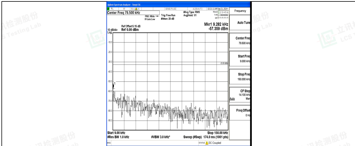
Band71_15MHz_16QAM_133297_1RB#0_0.009~0.15_0.009~0.15
