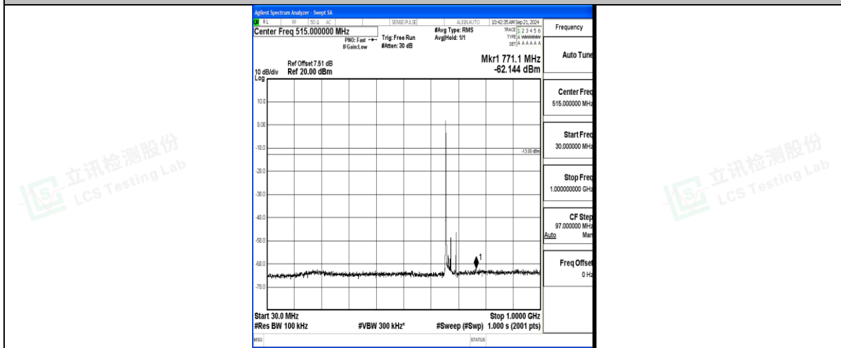
Band71_20MHz_QPSK_133222_1RB#0_30~1000_30~1000
