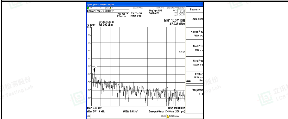
Band71_15MHz_QPSK_133297_1RB#0_0.009~0.15_0.009~0.15
