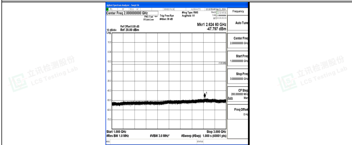
Band71_15MHz_16QAM_133197_1RB#0_1000~3000_1000~3000
