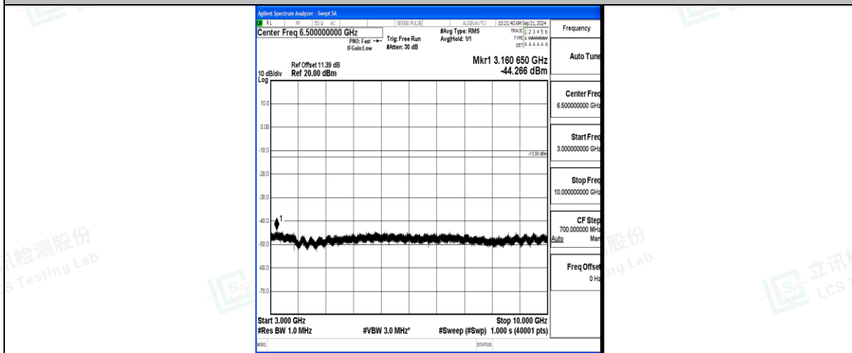
Band71_15MHz_16QAM_133297_1RB#0_3000~10000_3000~10000
