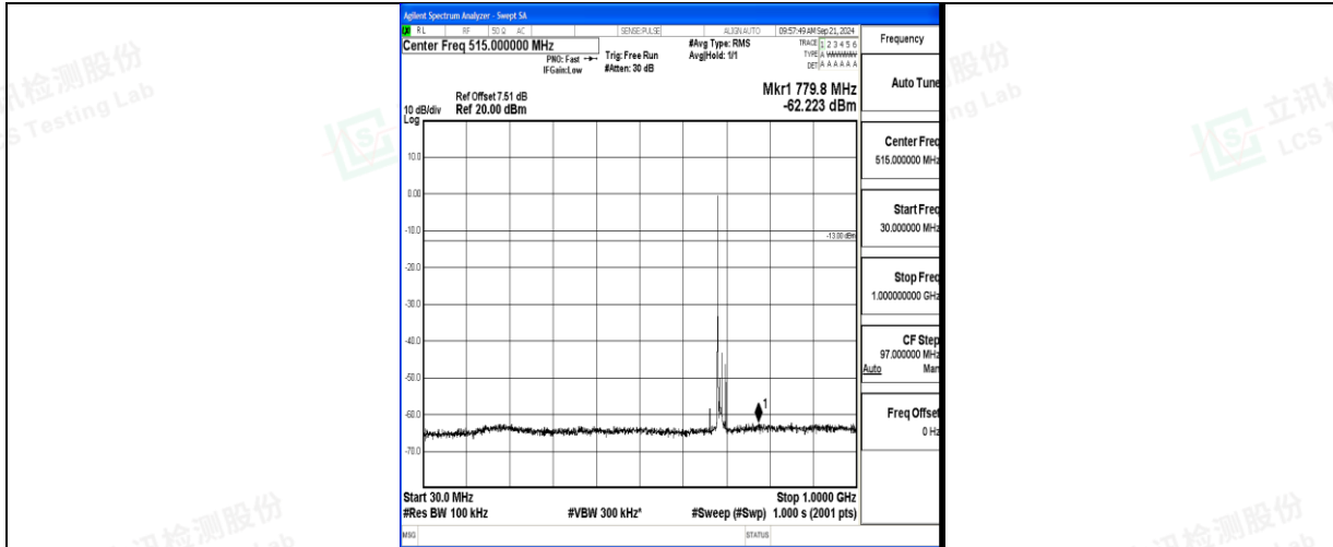
Band71_10MHz_16QAM_133422_1RB#0_30~1000_30~1000
