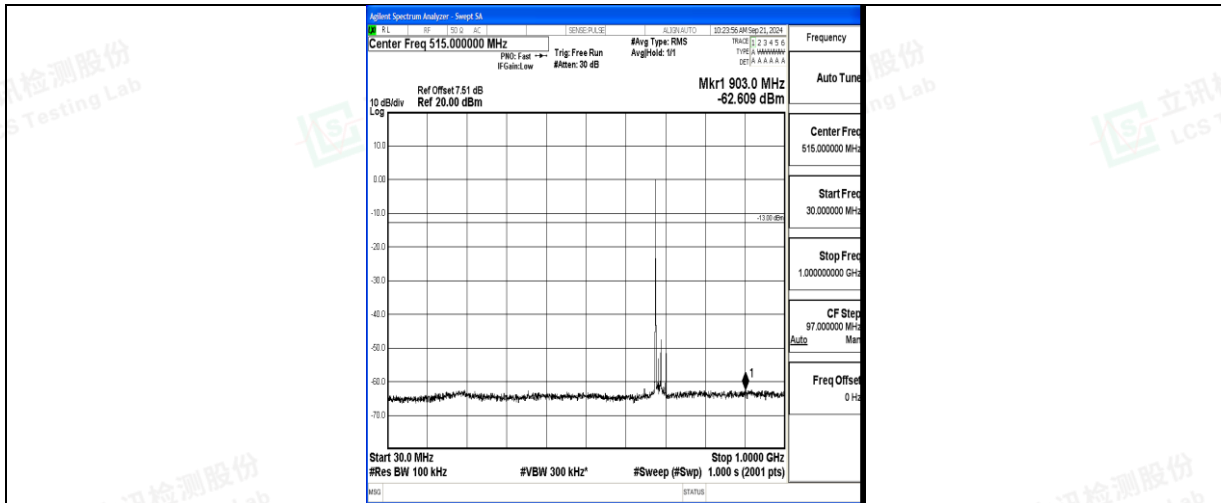
Band71_15MHz_16QAM_133397_1RB#0_30~1000_30~1000
