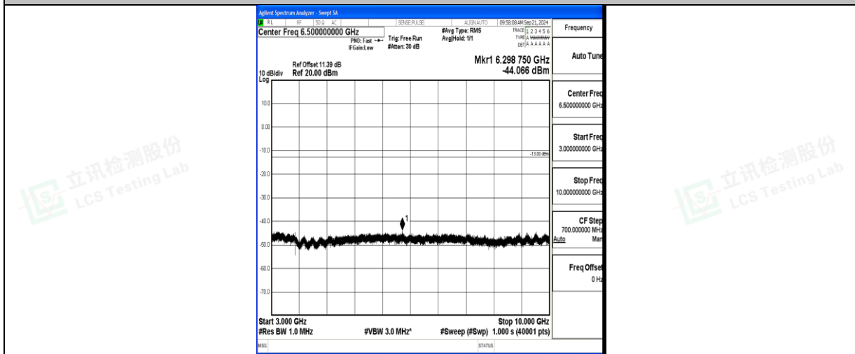
Band71_10MHz_16QAM_133422_1RB#0_3000~10000_3000~10000
