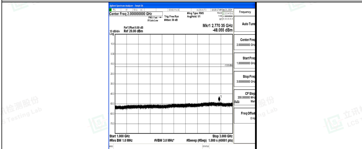
Band71_15MHz_QPSK_133297_1RB#0_1000~3000_1000~3000
