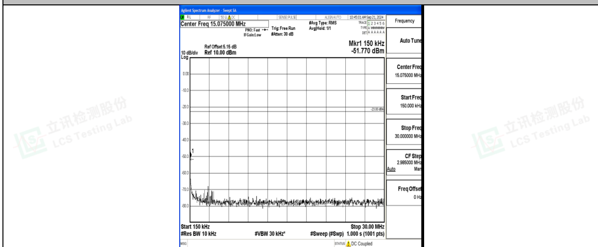
Band71_20MHz_QPSK_133322_1RB#0_0.15~30_0.15~30
