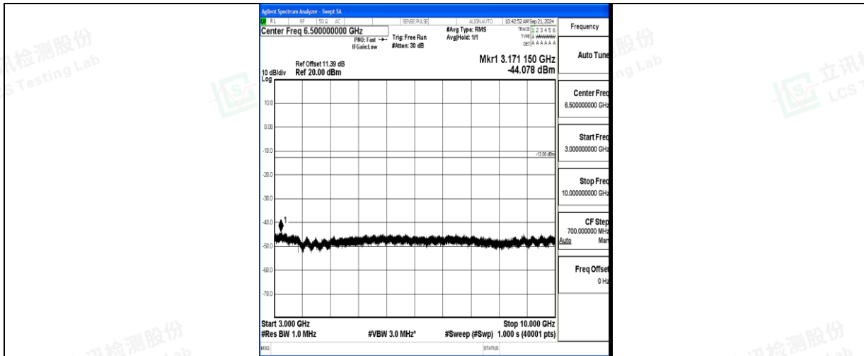
Band71_20MHz_QPSK_133222_1RB#0_3000~10000_3000~10000
