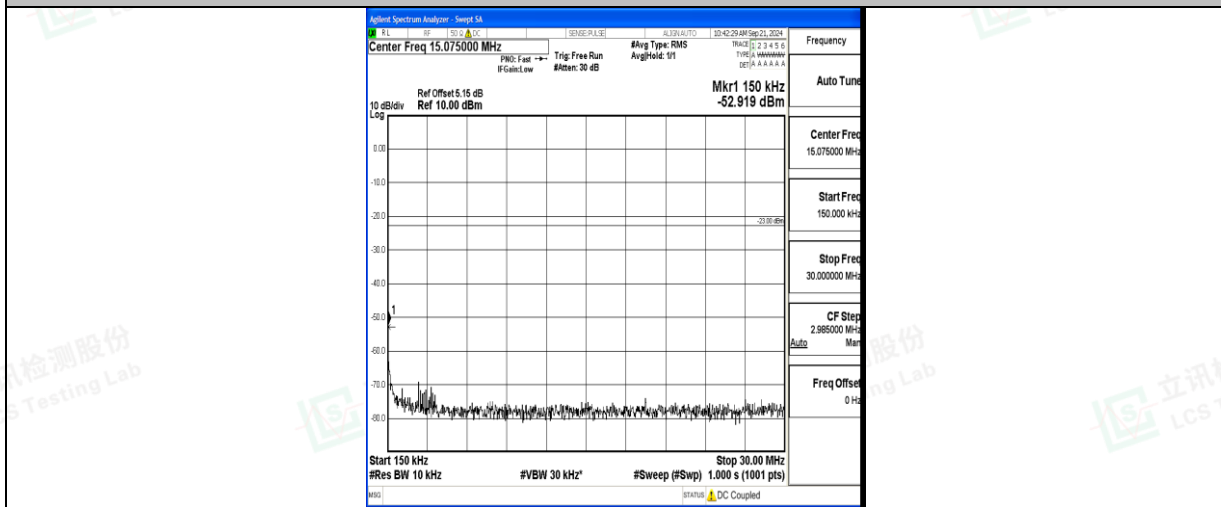
Band71_20MHz_QPSK_133222_1RB#0_0.15~30_0.15~30
