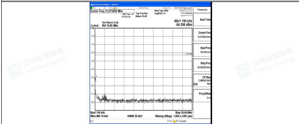
Band71_10MHz_16QAM_133422_1RB#0_0.15~30_0.15~30
