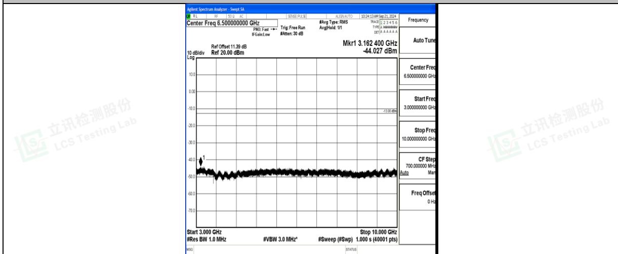
Band71_15MHz_16QAM_133397_1RB#0_3000~10000_3000~10000
