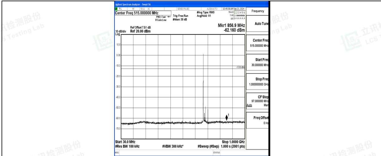
Band71_20MHz_QPSK_133322_1RB#0_30~1000_30~1000
