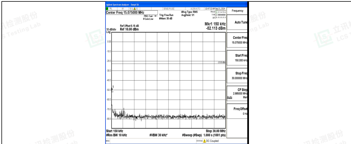
Band71_20MHz_QPSK_133372_1RB#0_0.15~30_0.15~30
