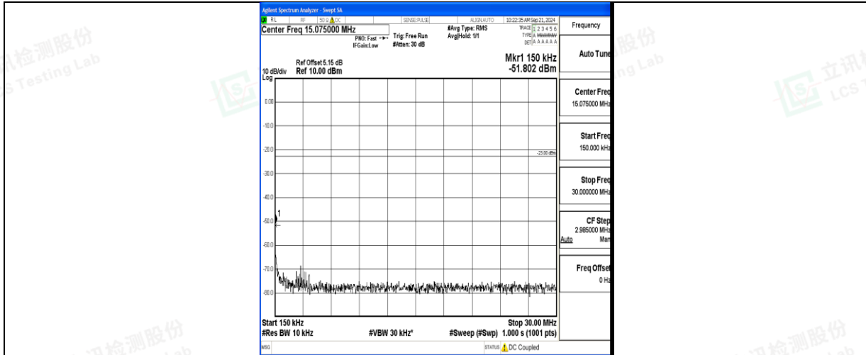
Band71_15MHz_QPSK_133397_1RB#0_0.15~30_0.15~30
