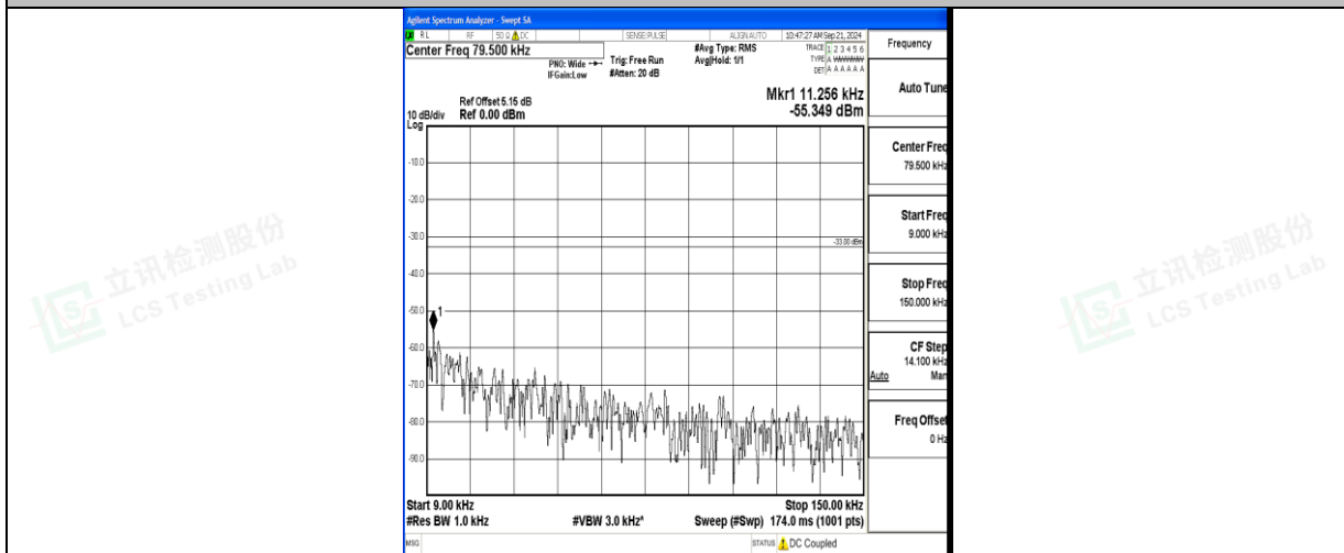
Band71_20MHz_QPSK_133372_1RB#0_0.009~0.15_0.009~0.15
