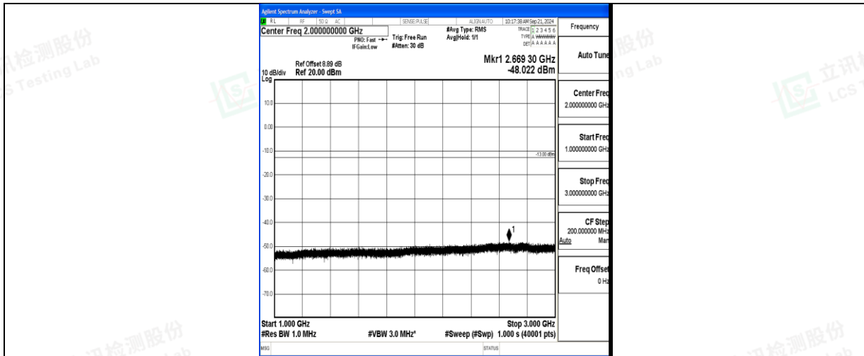
Band71_15MHz_QPSK_133197_1RB#0_1000~3000_1000~3000
