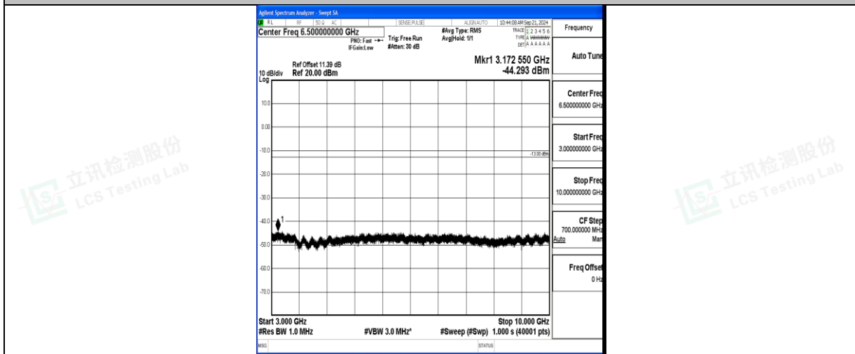
Band71_20MHz_16QAM_133222_1RB#0_3000~10000_3000~10000
