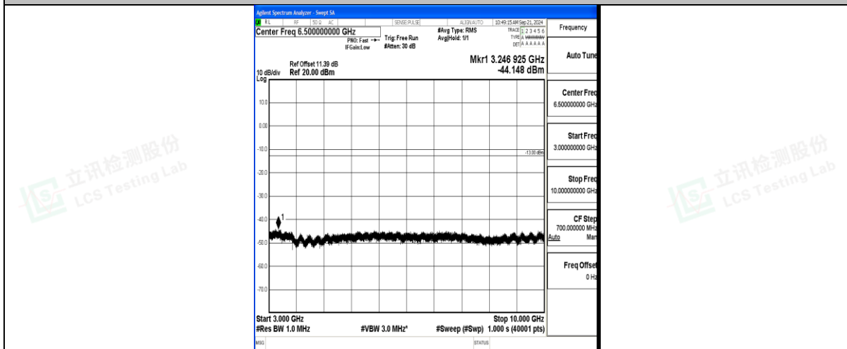
Band71_20MHz_16QAM_133372_1RB#0_3000~10000_3000~10000
