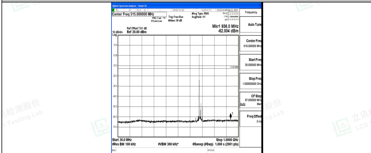
Band71_15MHz_QPSK_133397_1RB#0_30~1000_30~1000
