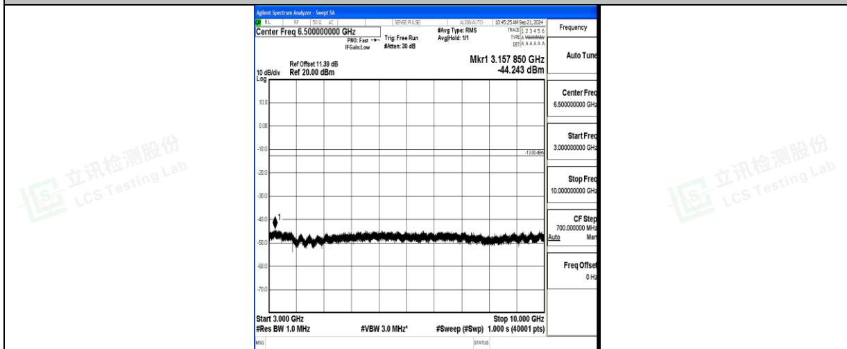
Band71_20MHz_QPSK_133322_1RB#0_3000~10000_3000~10000
