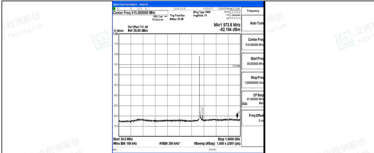
Band71_15MHz_QPSK_133297_1RB#0_30~1000_30~1000
