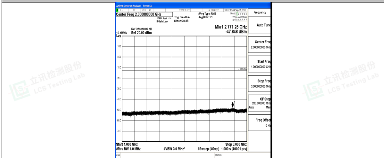
Band71_20MHz_QPSK_133372_1RB#0_1000~3000_1000~3000
