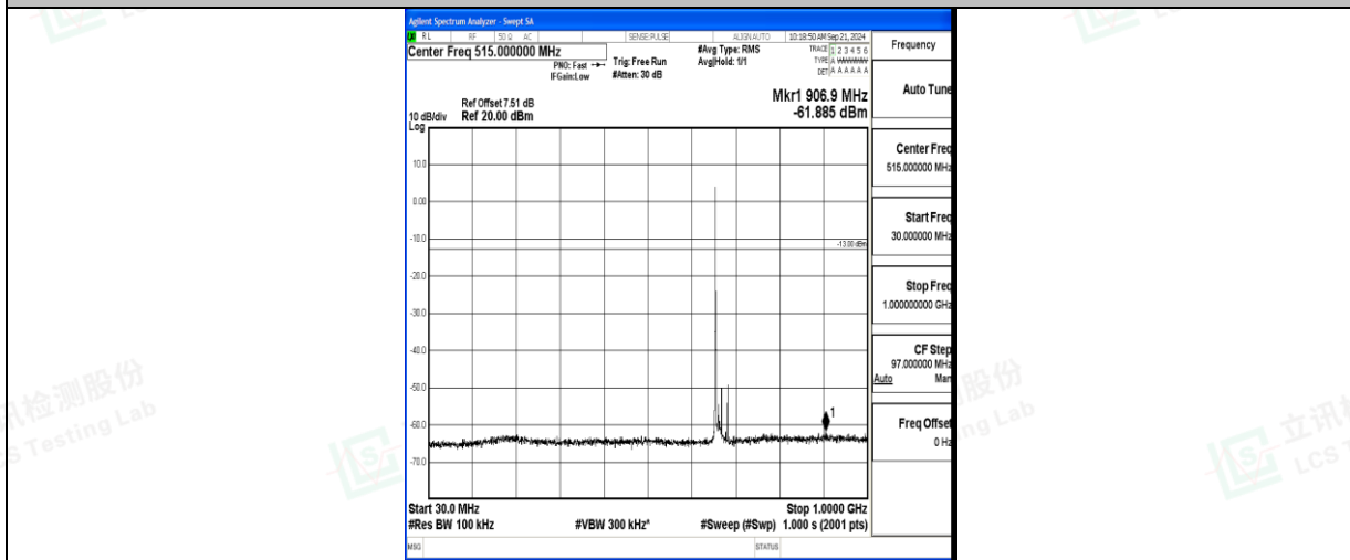
Band71_15MHz_16QAM_133197_1RB#0_30~1000_30~1000
