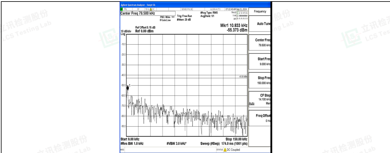
Band66_10MHz_16QAM_132622_1RB#0_0.009~0.15_0.009~0.15
