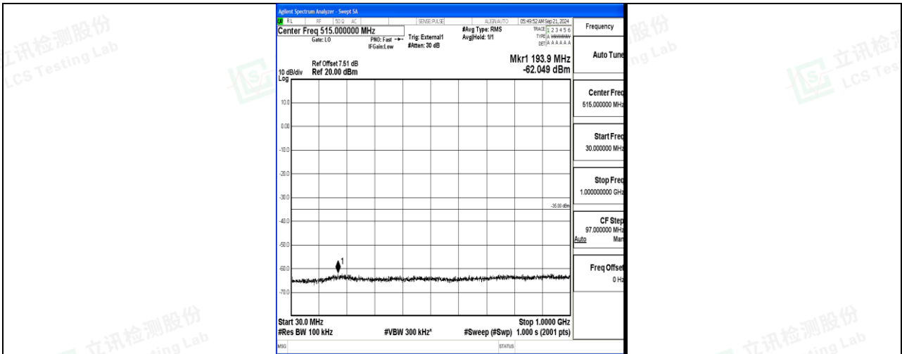
Band41_20MHz_QPSK_40620_1RB#0_30~1000_30~1000
