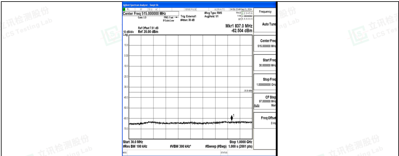
Band41_10MHz_16QAM_41540_1RB#0_30~1000_30~1000
