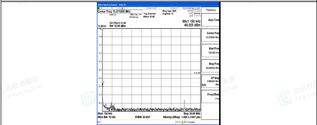
Band41_15MHz_16QAM_40620_1RB#0_0.15~30_0.15~30
