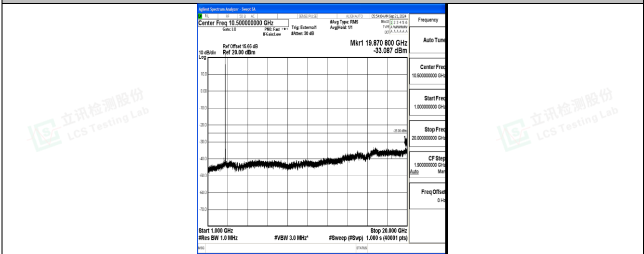
Band41_20MHz_QPSK_41490_1RB#0_1000~20000_1000~20000
