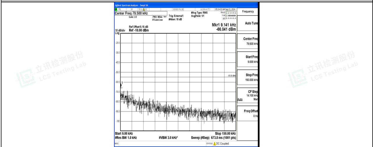
Band41_15MHz_QPSK_41515_1RB#0_0.009~0.15_0.009~0.15
