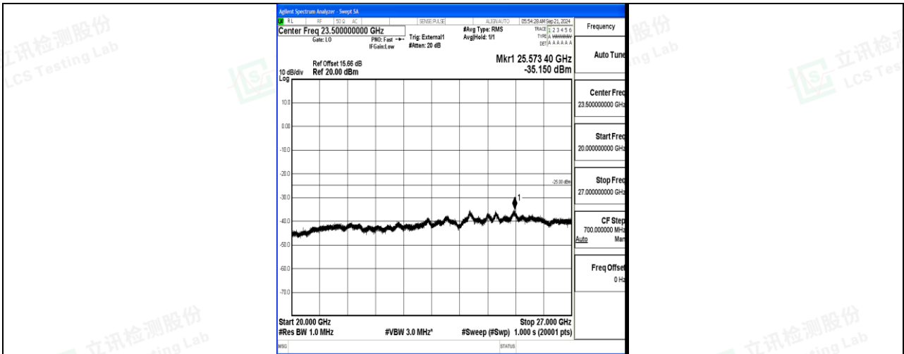
Band41_20MHz_QPSK_41490_1RB#0_20000~27000_20000~27000
