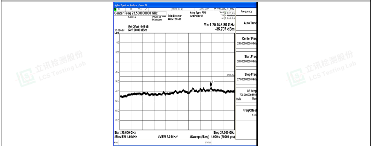
Band41_15MHz_16QAM_41515_1RB#0_20000~27000_20000~27000
