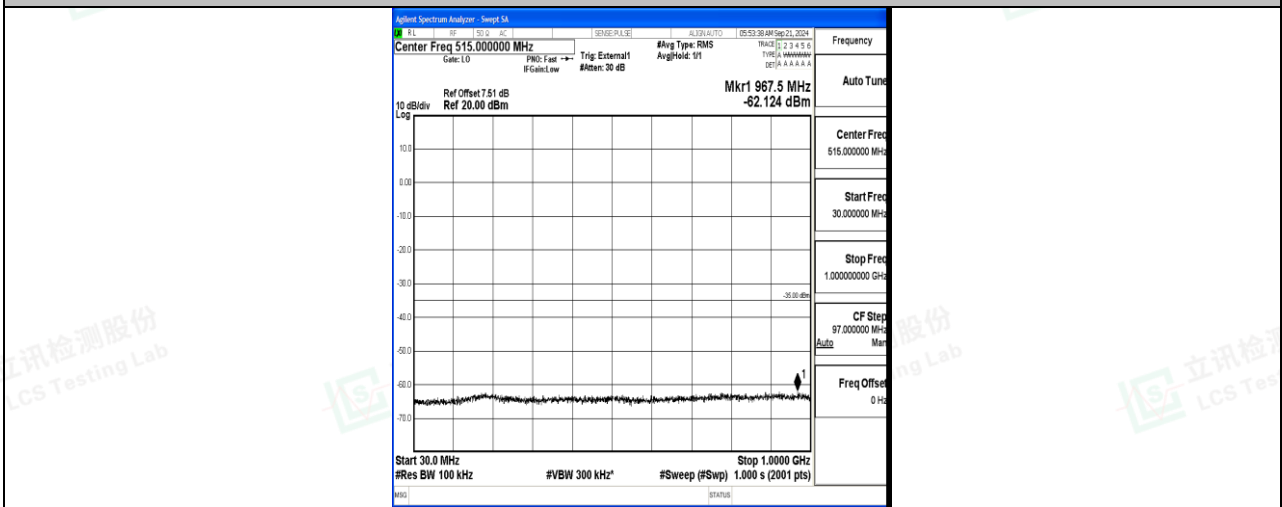
Band41_20MHz_QPSK_41490_1RB#0_30~1000_30~1000
