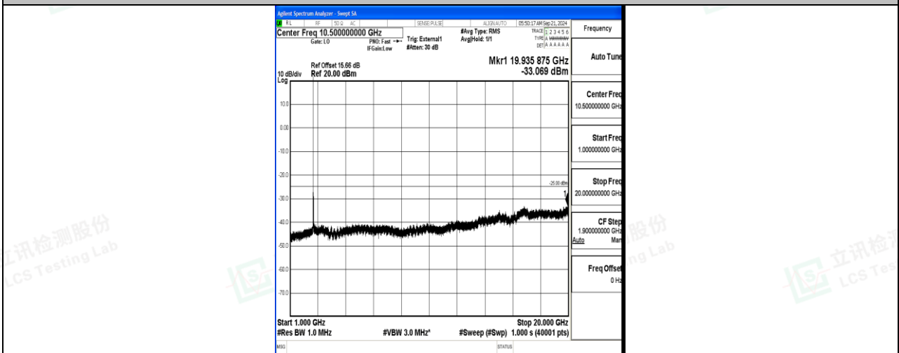
Band41_20MHz_QPSK_40620_1RB#0_1000~20000_1000~20000
