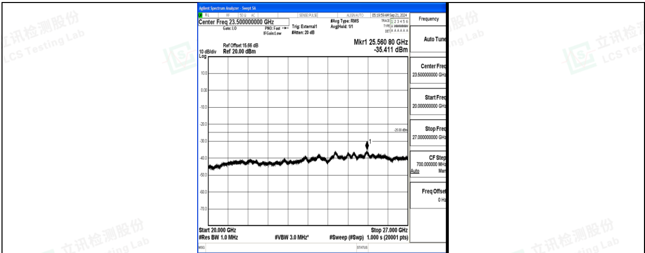
Band41_15MHz_16QAM_39725_1RB#0_20000~27000_20000~27000
