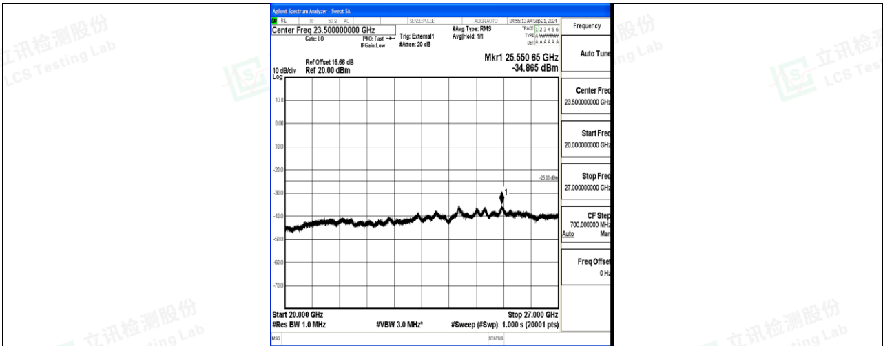
Band41_10MHz_QPSK_41540_1RB#0_20000~27000_20000~27000
