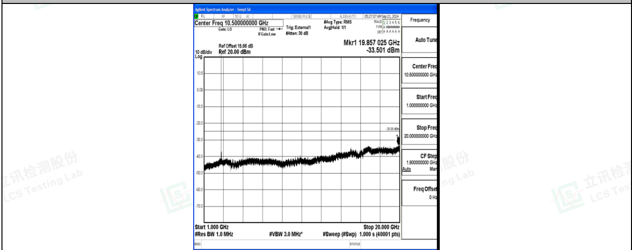
Band41_15MHz_16QAM_41515_1RB#0_1000~20000_1000~20000
