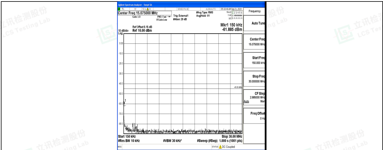
Band41_15MHz_16QAM_39725_1RB#0_0.15~30_0.15~30
