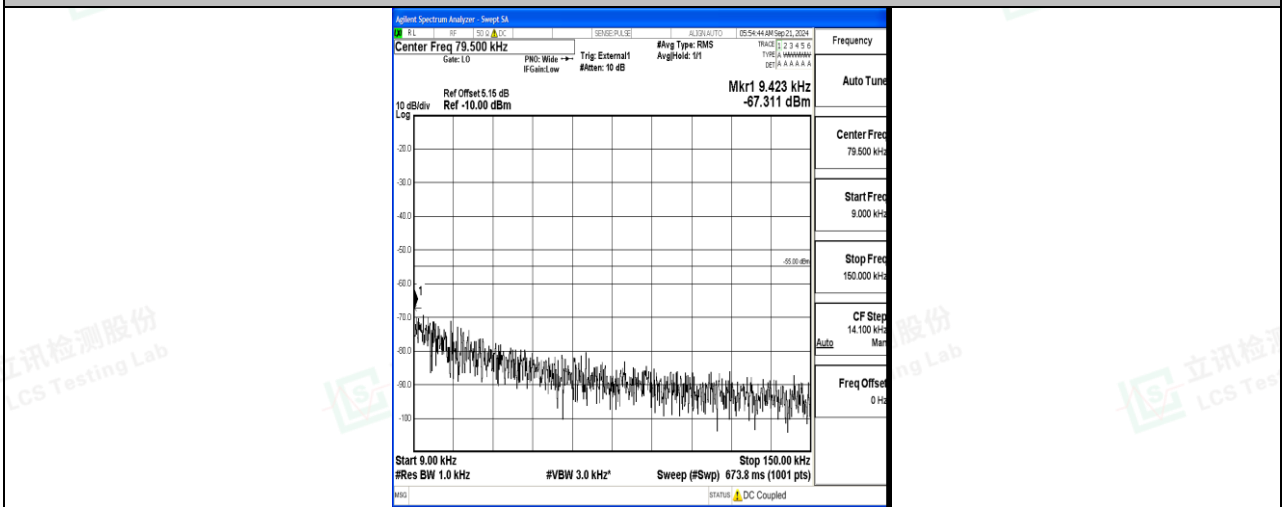
Band41_20MHz_16QAM_41490_1RB#0_0.009~0.15_0.009~0.15
