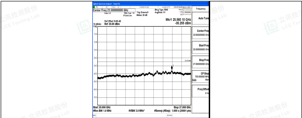
Band41_15MHz_QPSK_41515_1RB#0_20000~27000_20000~27000
