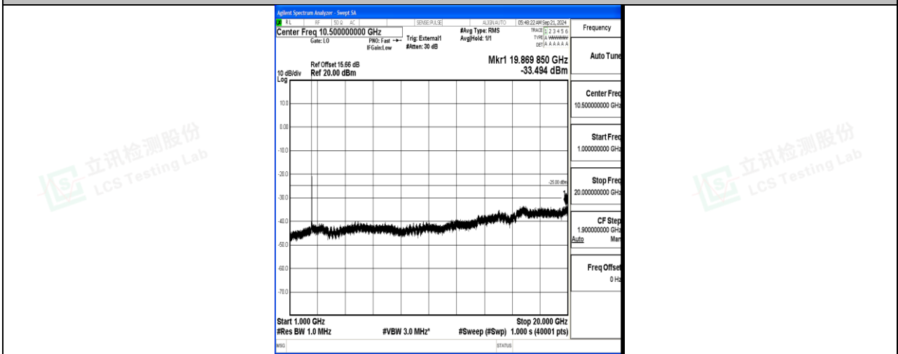
Band41_20MHz_16QAM_39750_1RB#0_1000~20000_1000~20000
