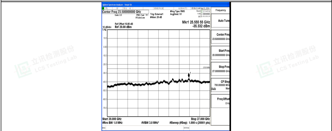
Band41_20MHz_16QAM_41490_1RB#0_20000~27000_20000~27000
