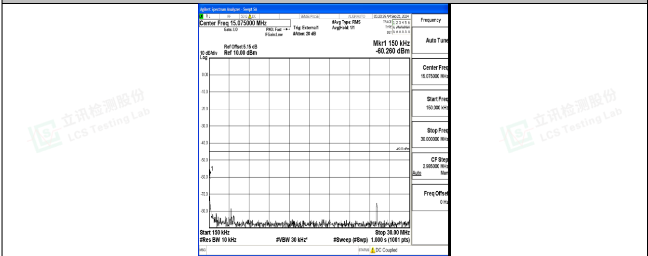
Band41_15MHz_QPSK_40620_1RB#0_0.15~30_0.15~30
