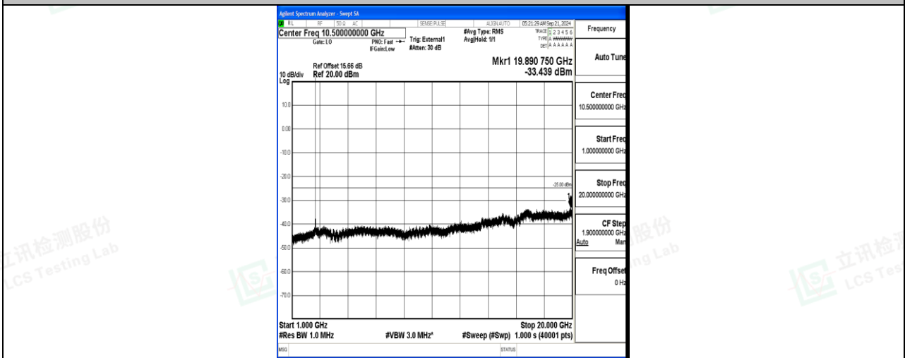
Band41_15MHz_QPSK_40620_1RB#0_1000~20000_1000~20000
