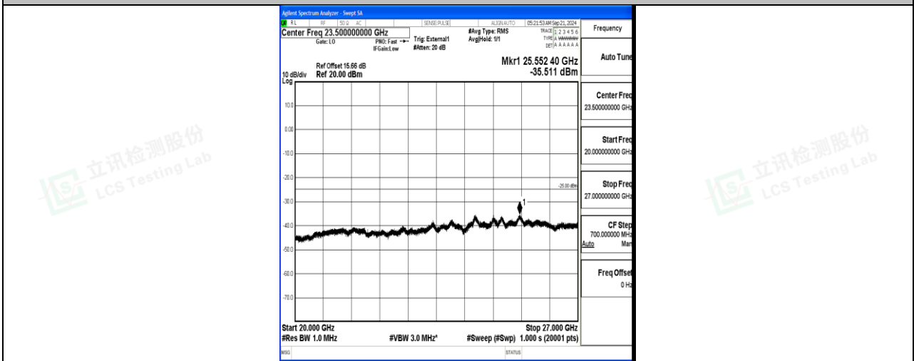
Band41_15MHz_QPSK_40620_1RB#0_20000~27000_20000~27000
