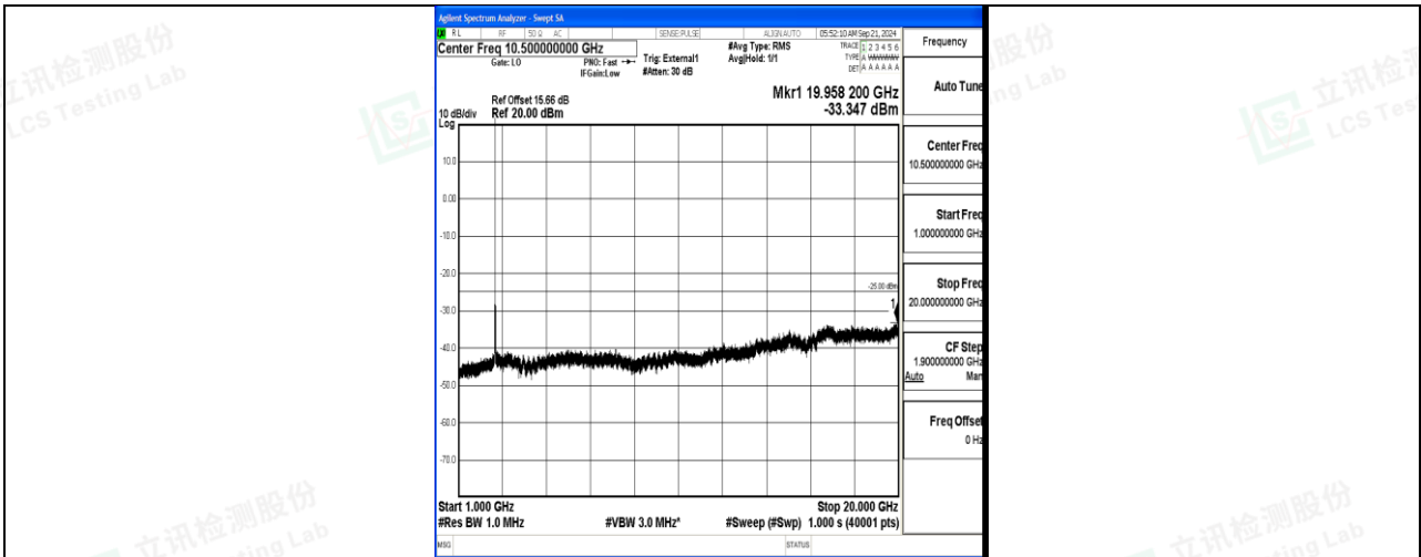
Band41_20MHz_16QAM_40620_1RB#0_1000~20000_1000~20000
