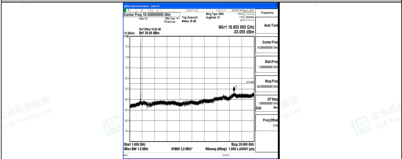
Band41_20MHz_16QAM_41490_1RB#0_1000~20000_1000~20000
