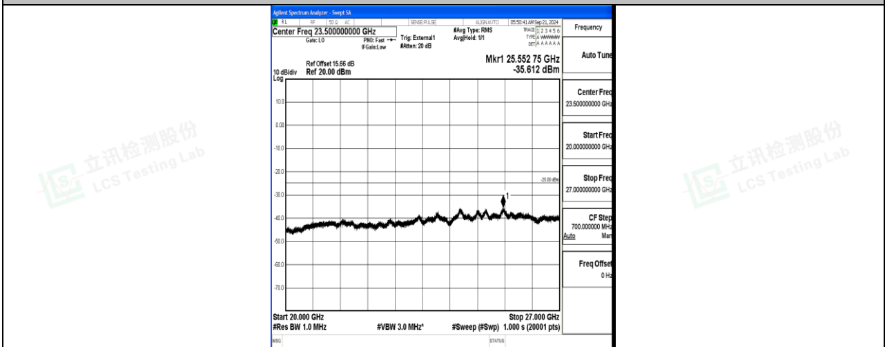
Band41_20MHz_QPSK_40620_1RB#0_20000~27000_20000~27000
