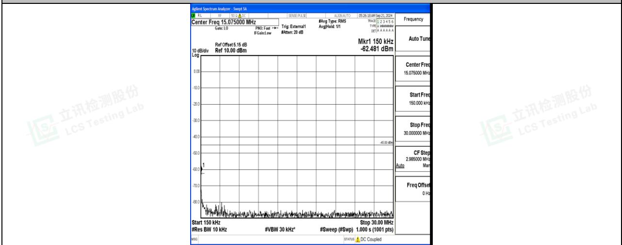
Band41_15MHz_16QAM_41515_1RB#0_0.15~30_0.15~30
