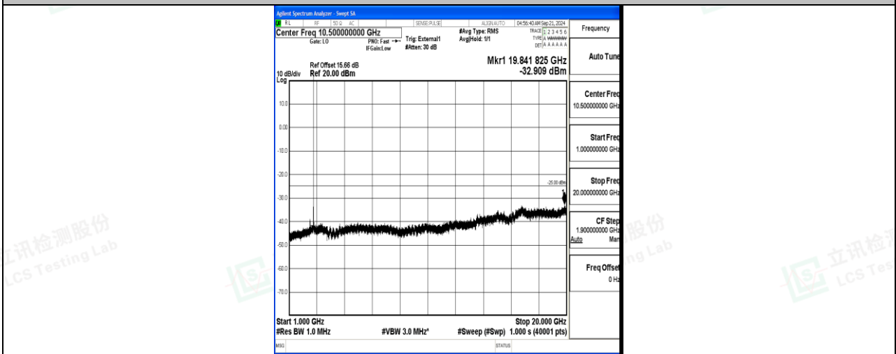
Band41_10MHz_16QAM_41540_1RB#0_1000~20000_1000~20000
