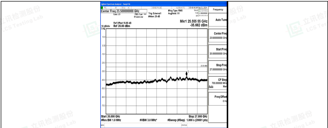
Band41_20MHz_16QAM_39750_1RB#0_20000~27000_20000~27000
