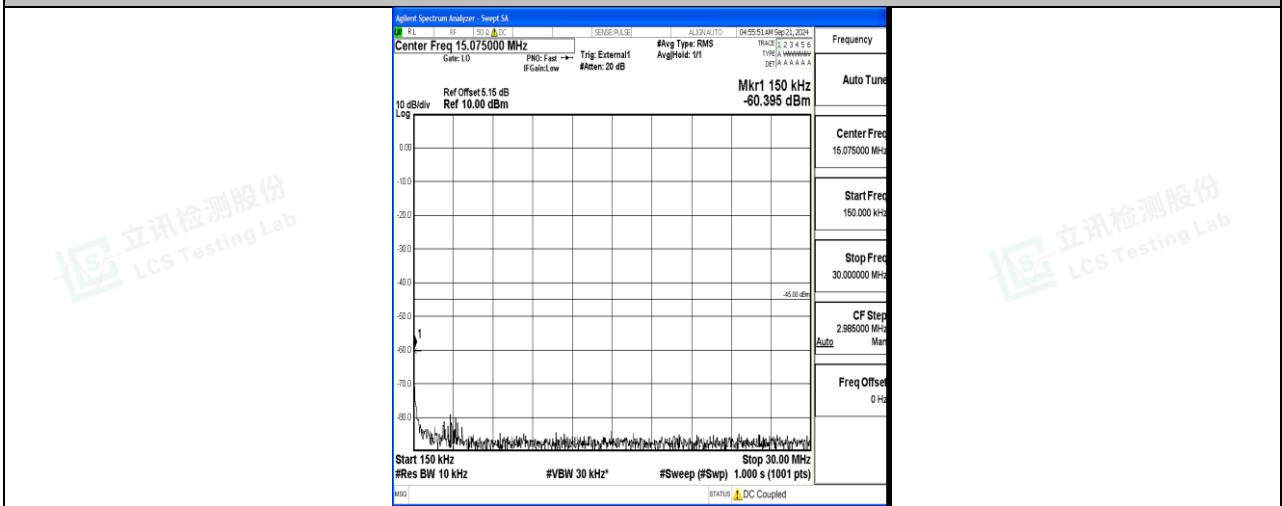
Band41_10MHz_16QAM_41540_1RB#0_0.15~30_0.15~30
