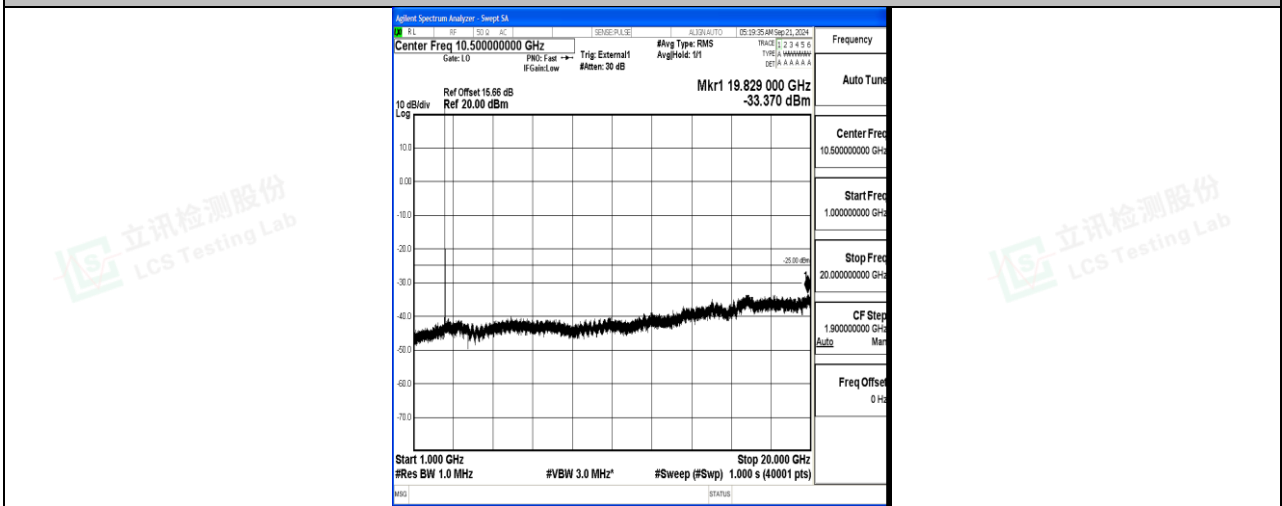
Band41_15MHz_16QAM_39725_1RB#0_1000~20000_1000~20000
