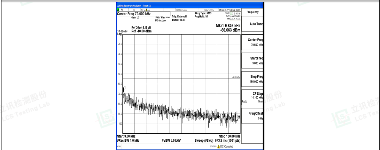
Band41_15MHz_QPSK_40620_1RB#0_0.009~0.15_0.009~0.15
