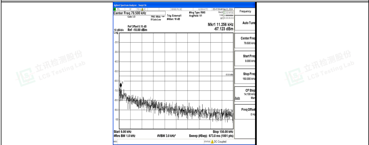
Band41_20MHz_16QAM_39750_1RB#0_0.009~0.15_0.009~0.15
