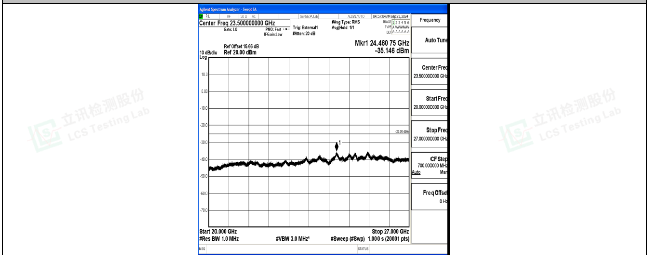
Band41_10MHz_16QAM_41540_1RB#0_20000~27000_20000~27000
