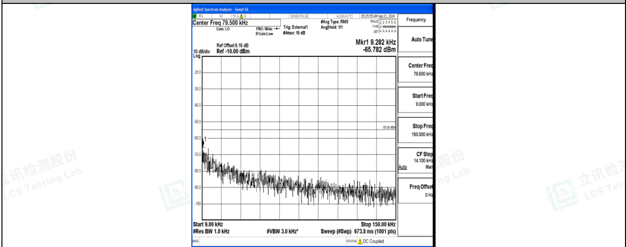
Band41_15MHz_16QAM_41515_1RB#0_0.009~0.15_0.009~0.15
