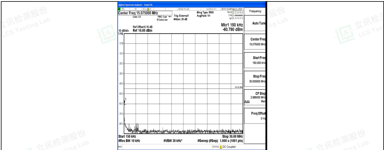
Band41_20MHz_16QAM_39750_1RB#0_0.15~30_0.15~30
