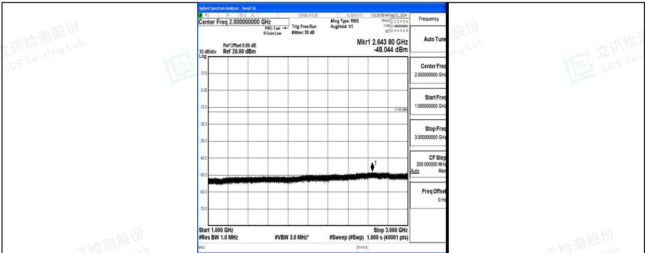
Band17_5MHz_QPSK_23790_1RB#0_1000~3000_1000~3000
