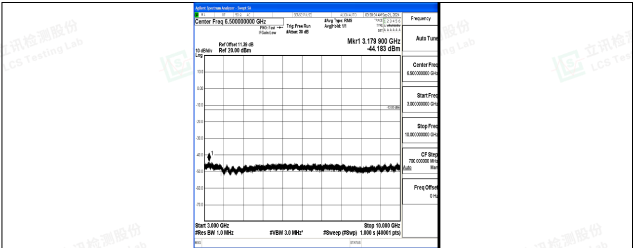
Band17_5MHz_16QAM_23790_1RB#0_3000~10000_3000~10000
