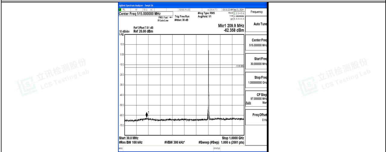
Band17_5MHz_16QAM_23825_1RB#0_30~1000_30~1000
