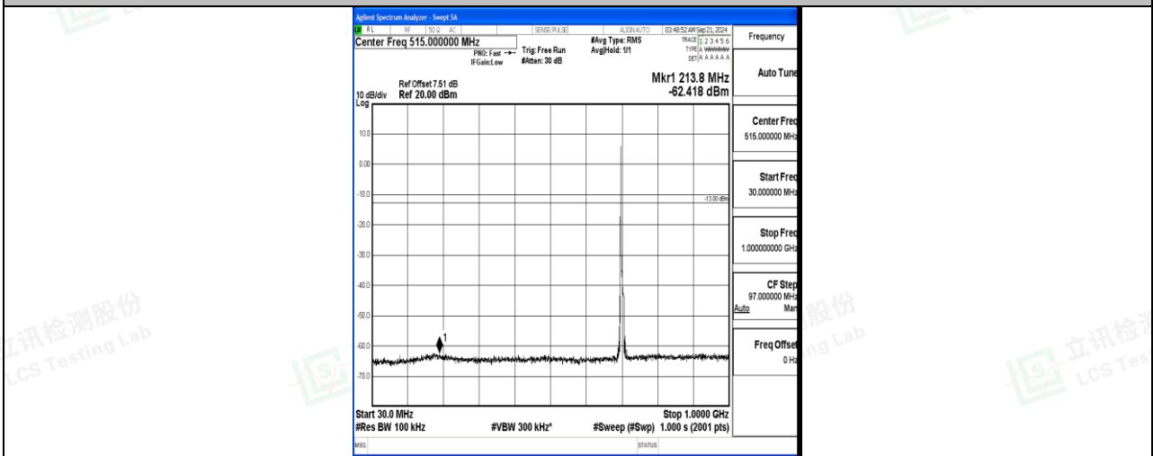
Band17_10MHz_QPSK_23780_1RB#0_30~1000_30~1000
