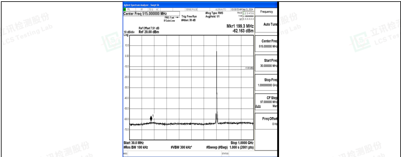
Band17_5MHz_QPSK_23825_1RB#0_30~1000_30~1000
