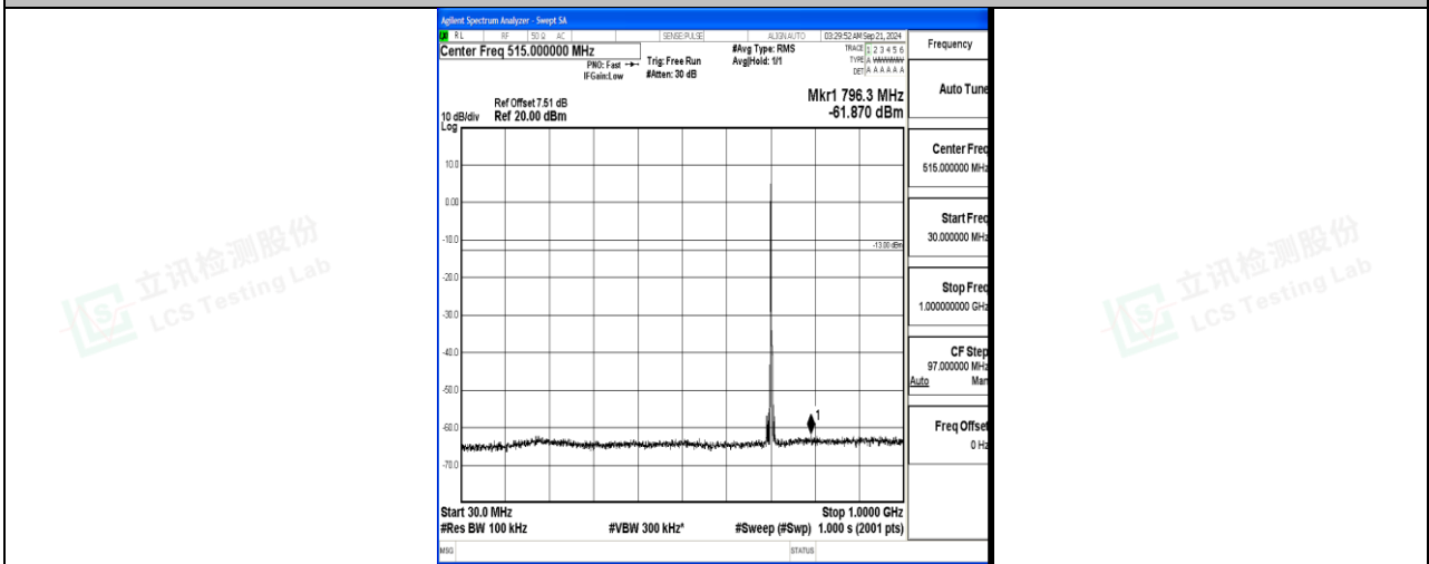
Band17_5MHz_QPSK_23790_1RB#0_30~1000_30~1000
