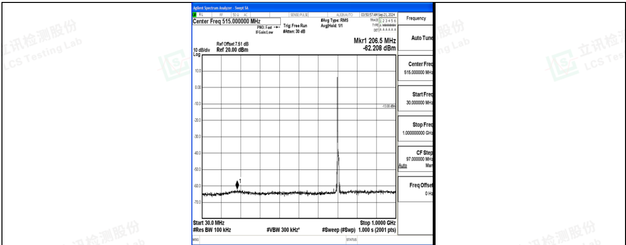
Band17_10MHz_QPSK_23800_1RB#0_30~1000_30~1000
