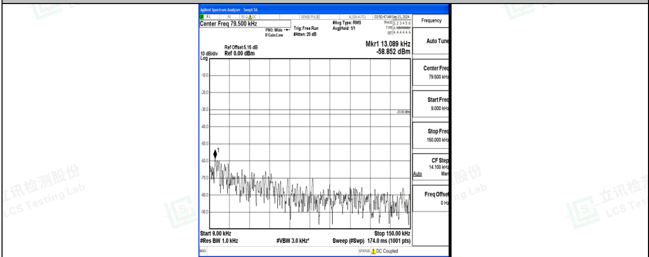
Band17_10MHz_QPSK_23800_1RB#0_0.009~0.15_0.009~0.15
