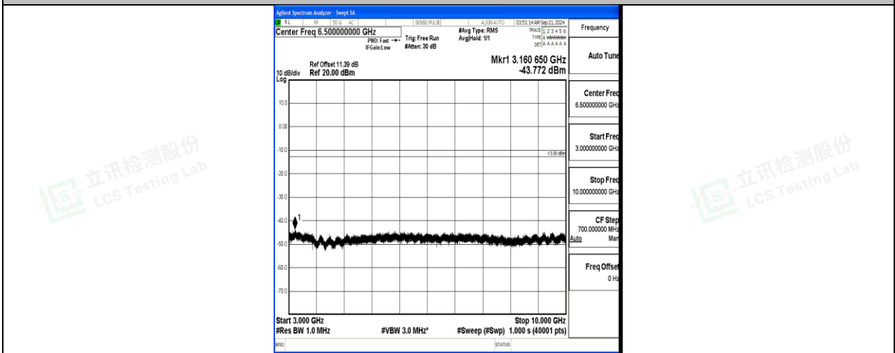
Band17_10MHz_QPSK_23800_1RB#0_3000~10000_3000~10000
