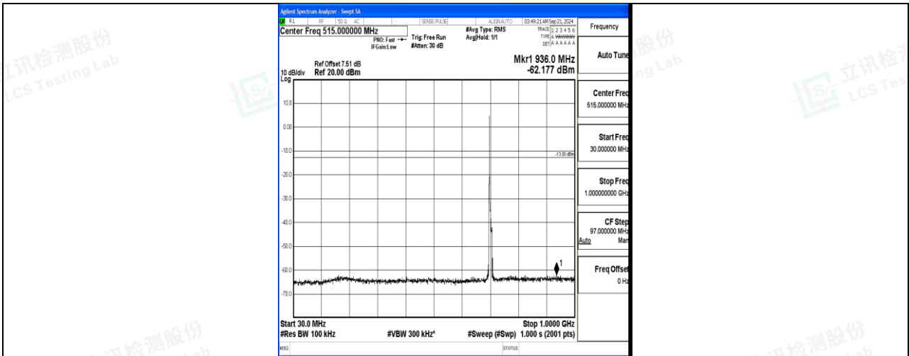
Band17_10MHz_16QAM_23780_1RB#0_30~1000_30~1000
