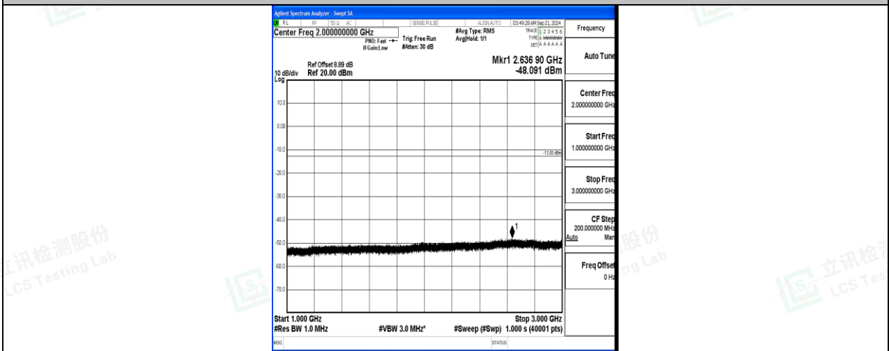
Band17_10MHz_16QAM_23780_1RB#0_1000~3000_1000~3000
