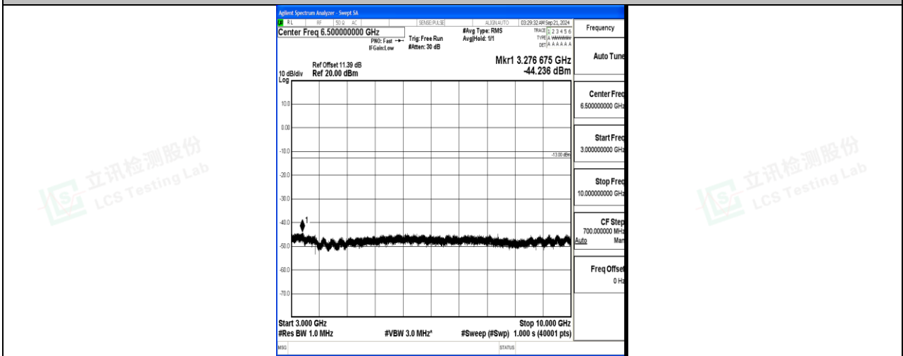
Band17_5MHz_16QAM_23755_1RB#0_3000~10000_3000~10000
