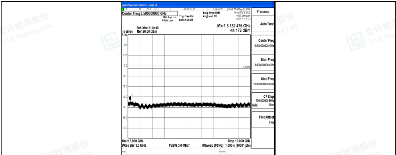
Band17_10MHz_QPSK_23780_1RB#0_3000~10000_3000~10000
