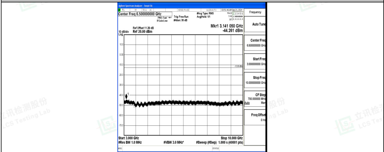
Band17_10MHz_16QAM_23800_1RB#0_3000~10000_3000~10000
