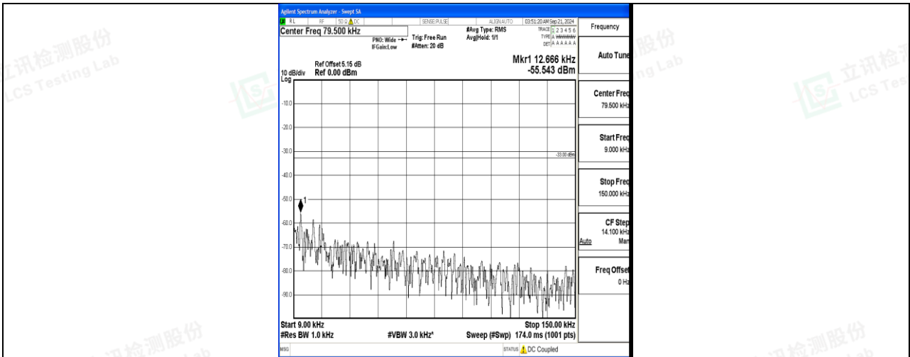
Band17_10MHz_16QAM_23800_1RB#0_0.009~0.15_0.009~0.15
