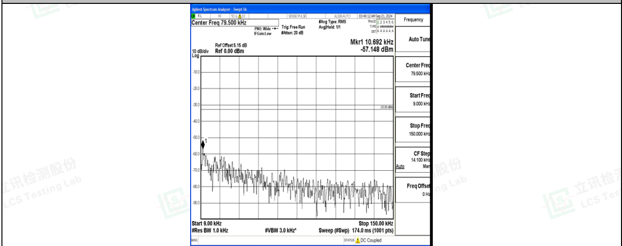
Band17_10MHz_16QAM_23780_1RB#0_0.009~0.15_0.009~0.15
