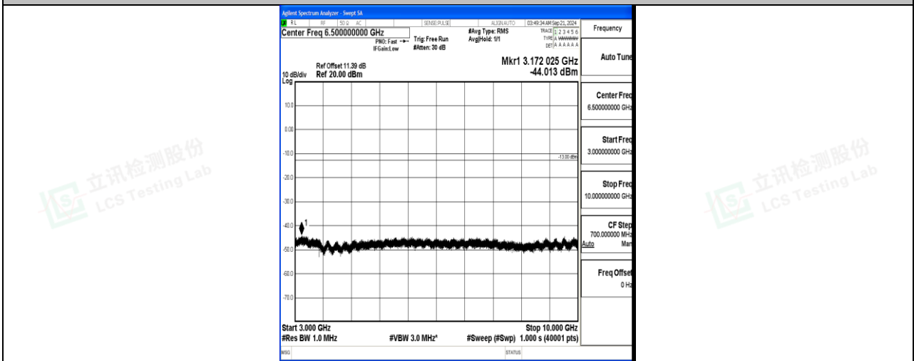
Band17_10MHz_16QAM_23780_1RB#0_3000~10000_3000~10000
