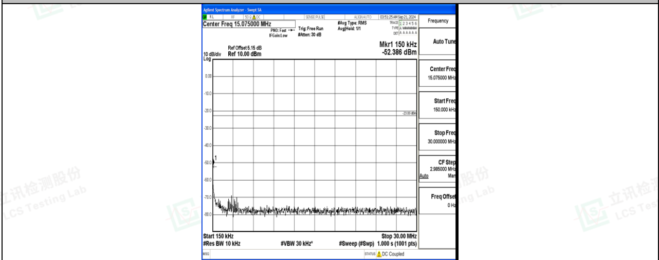
Band17_10MHz_16QAM_23800_1RB#0_0.15~30_0.15~30
