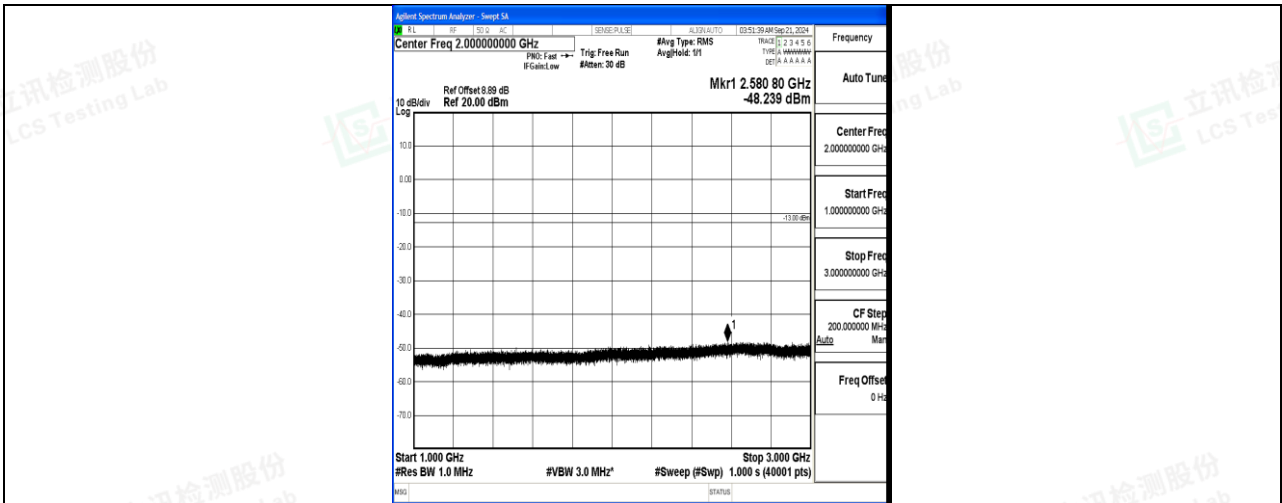
Band17_10MHz_16QAM_23800_1RB#0_1000~3000_1000~3000
