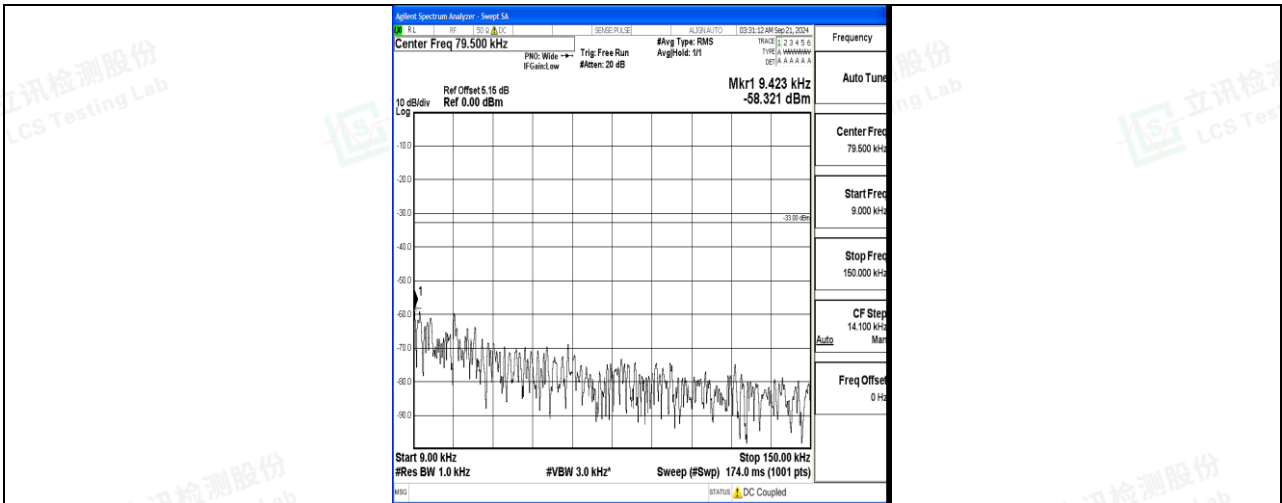
Band17_5MHz_16QAM_23825_1RB#0_0.009~0.15_0.009~0.15
