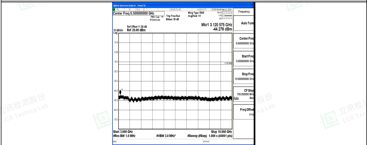
Band17_10MHz_QPSK_23790_1RB#0_3000~10000_3000~10000
