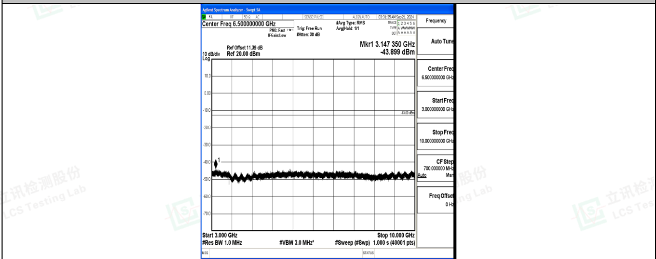
Band17_5MHz_16QAM_23825_1RB#0_3000~10000_3000~10000
