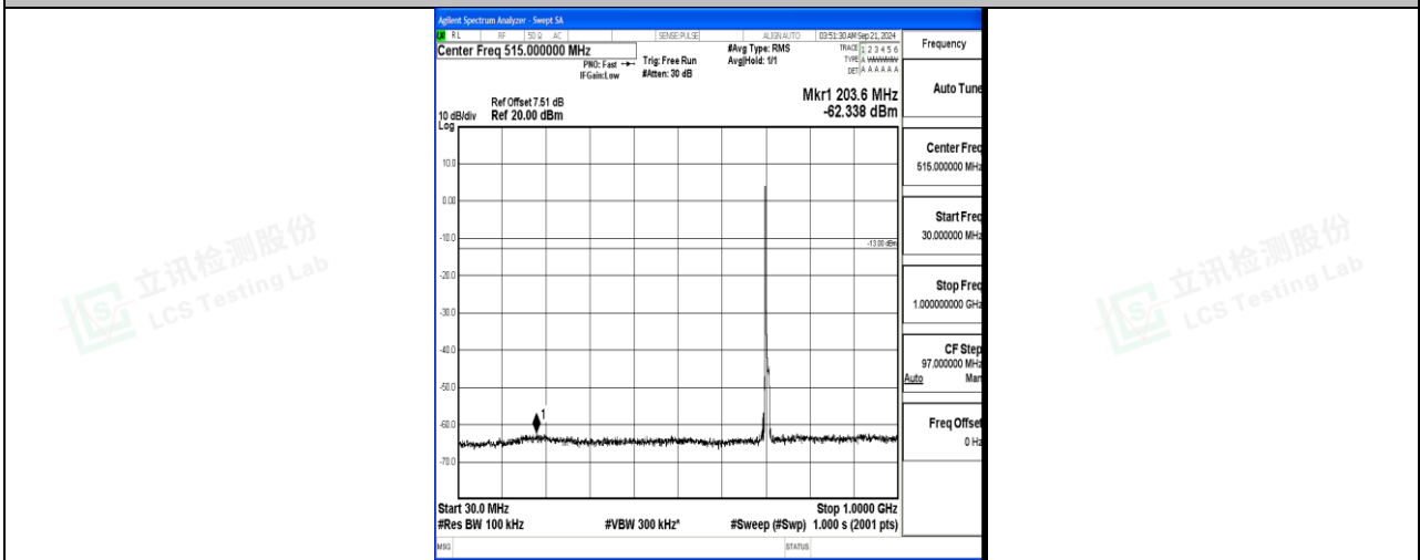
Band17_10MHz_16QAM_23800_1RB#0_30~1000_30~1000
