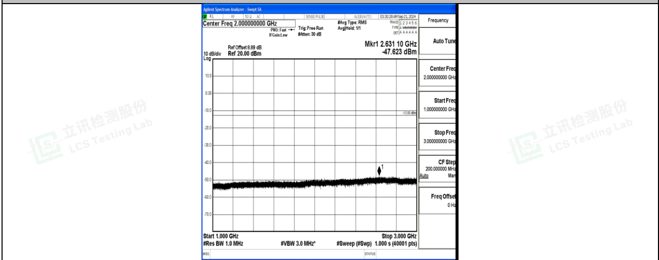
Band17_5MHz_16QAM_23790_1RB#0_1000~3000_1000~3000
