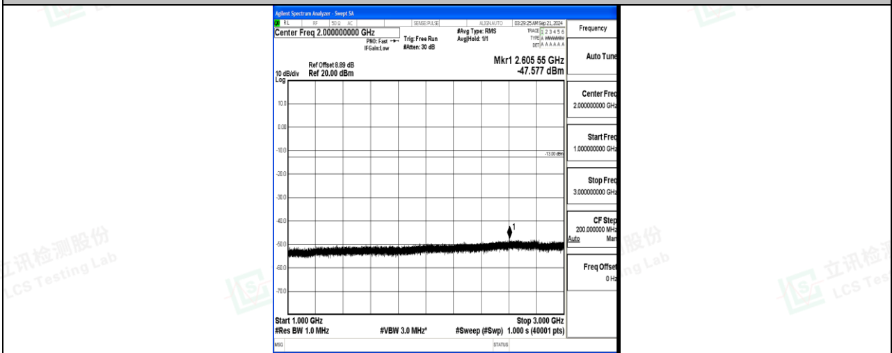
Band17_5MHz_16QAM_23755_1RB#0_1000~3000_1000~3000
