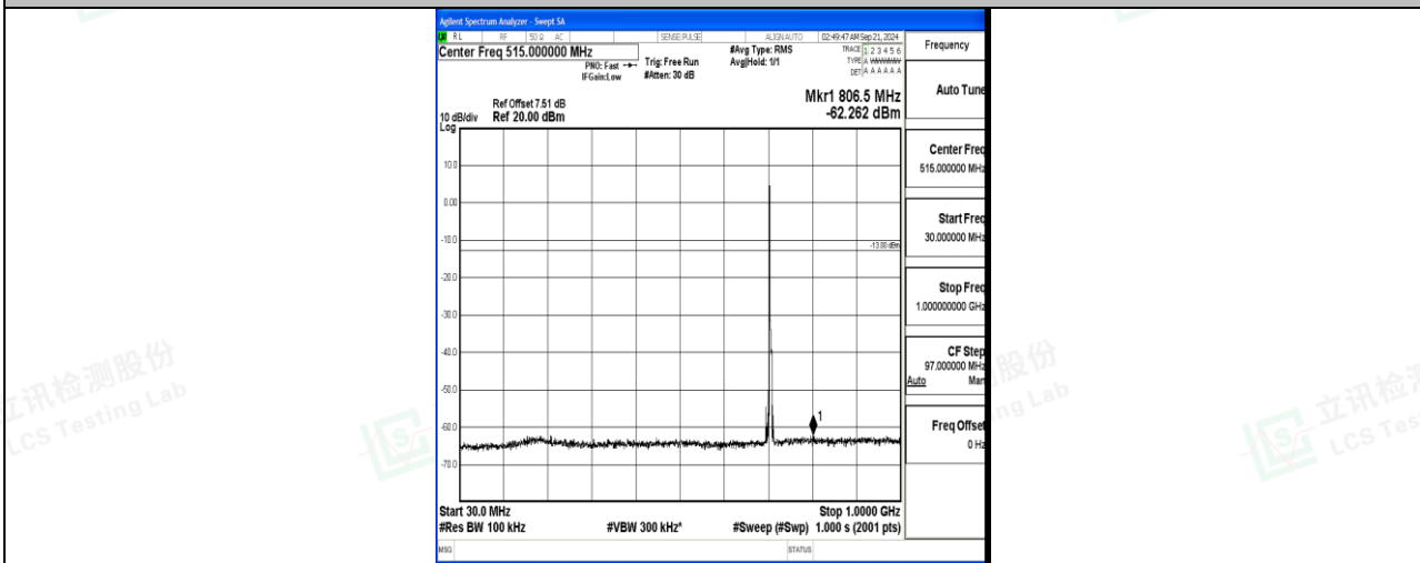
Band12_5MHz_QPSK_23155_1RB#0_30~1000_30~1000
