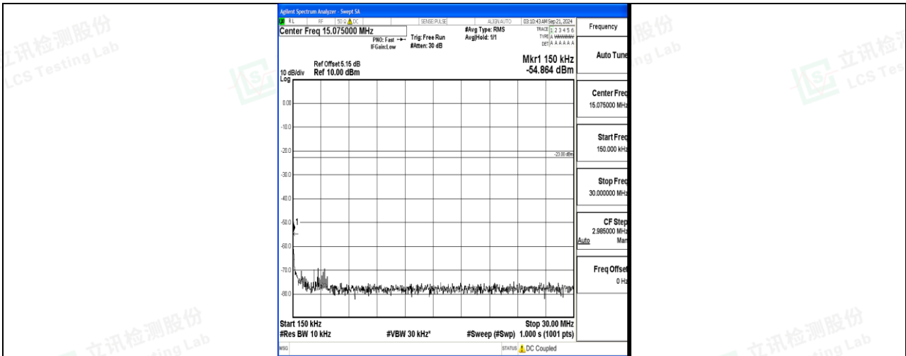
Band12_10MHz_QPSK_23130_1RB#0_0.15~30_0.15~30
