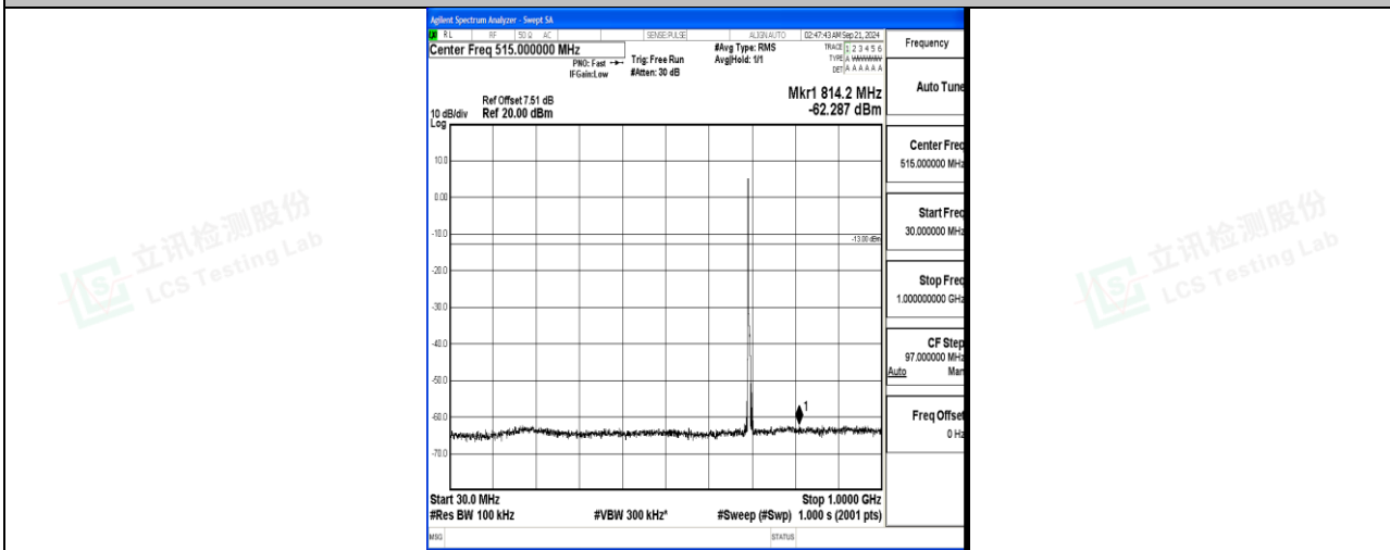
Band12_5MHz_QPSK_23035_1RB#0_30~1000_30~1000
