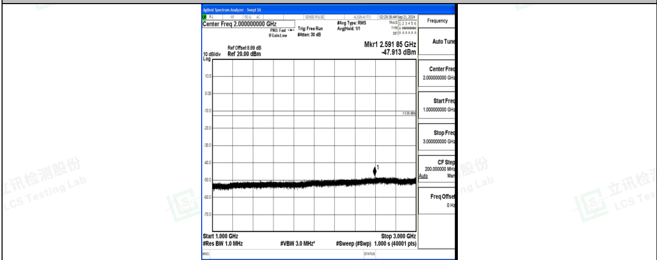
Band12_3MHz_16QAM_23165_1RB#0_1000~3000_1000~3000
