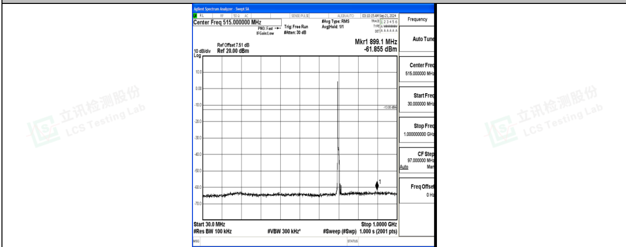
Band12_10MHz_16QAM_23095_1RB#0_30~1000_30~1000
