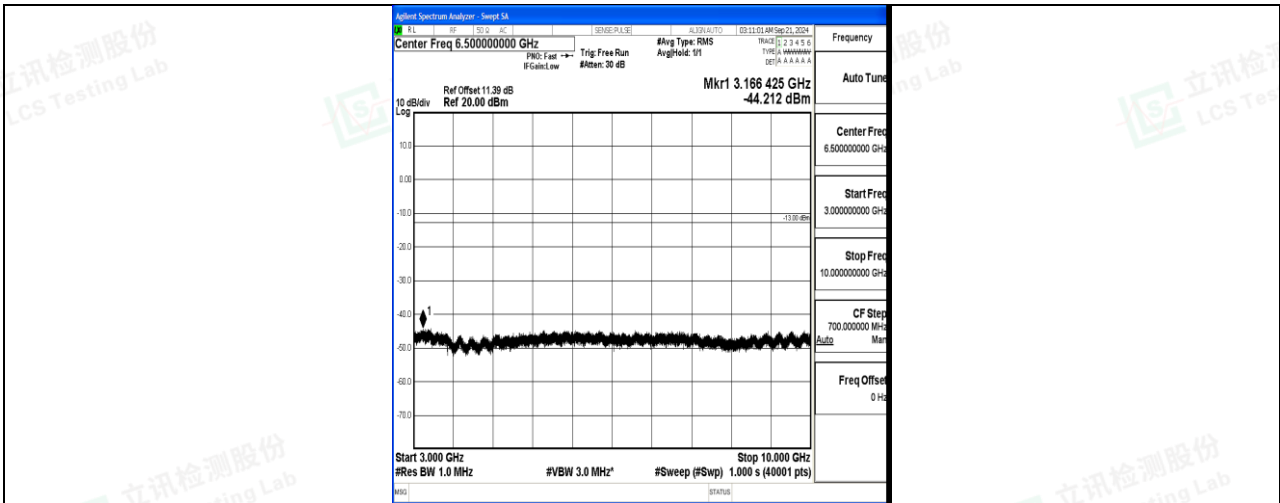
Band12_10MHz_QPSK_23130_1RB#0_3000~10000_3000~10000
