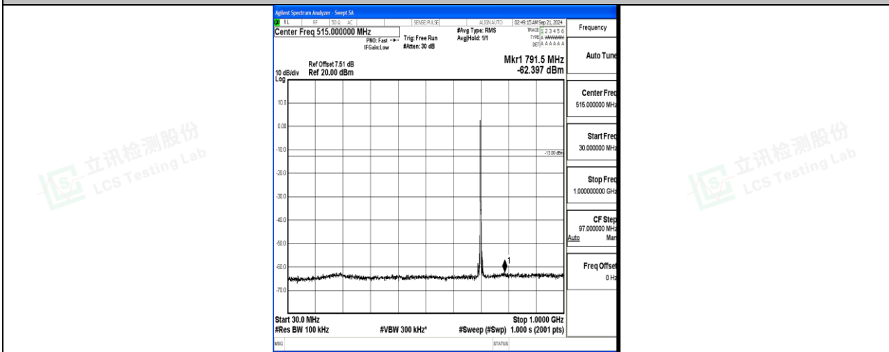
Band12_5MHz_16QAM_23095_1RB#0_30~1000_30~1000
