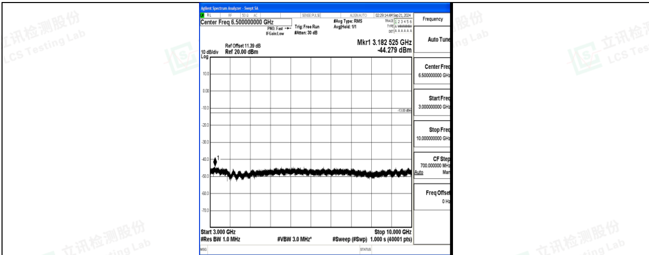
Band12_3MHz_QPSK_23165_1RB#0_3000~10000_3000~10000
