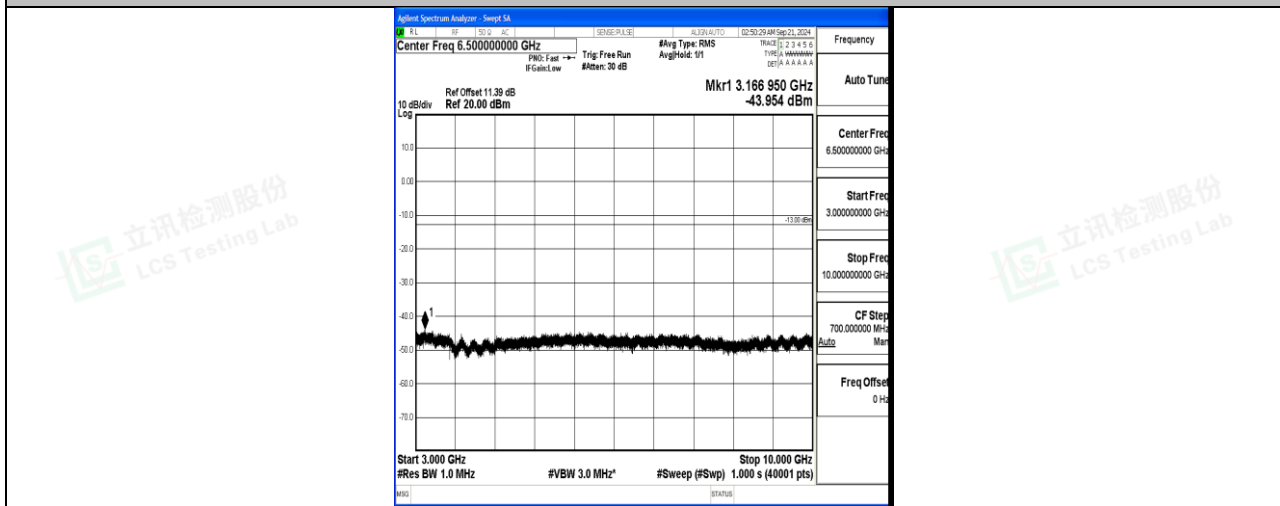
Band12_5MHz_16QAM_23155_1RB#0_3000~10000_3000~10000
