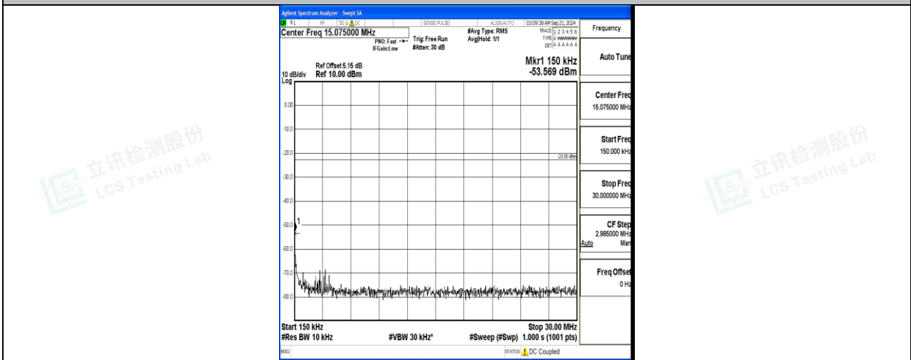
Band12_10MHz_QPSK_23095_1RB#0_0.15~30_0.15~30
