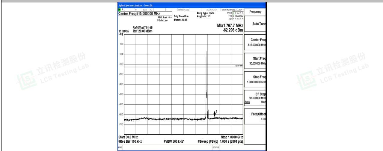
Band12_10MHz_QPSK_23060_1RB#0_30~1000_30~1000
