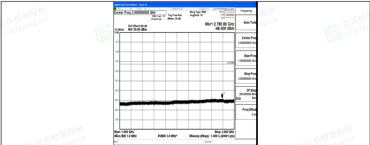
Band12_5MHz_QPSK_23035_1RB#0_1000~3000_1000~3000
