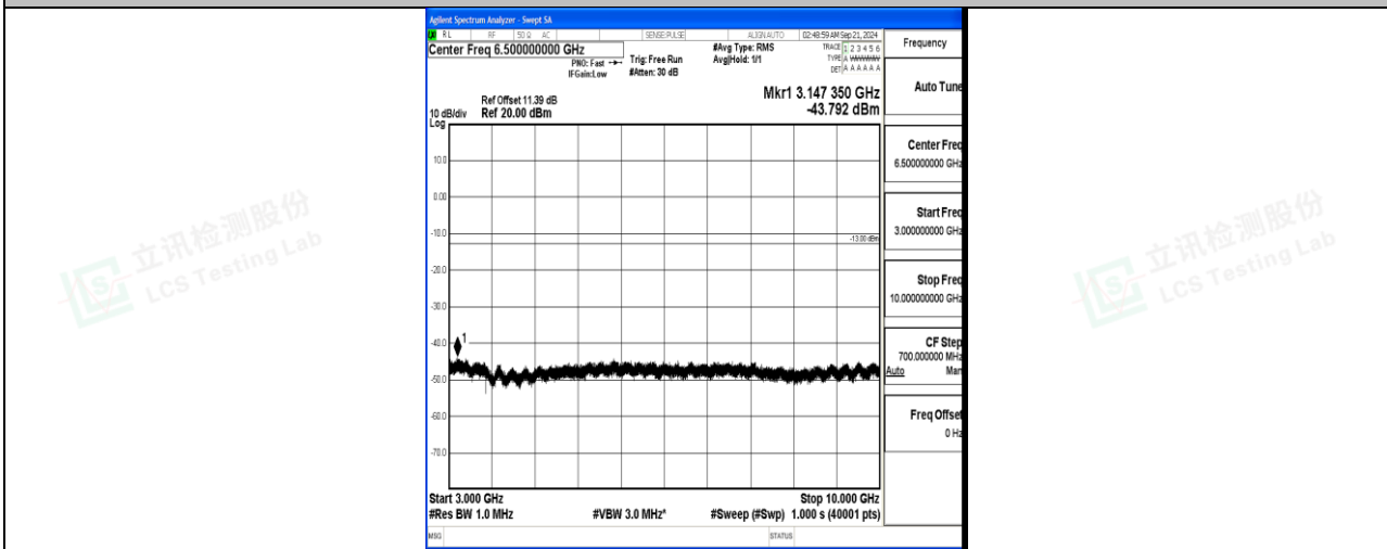
Band12_5MHz_QPSK_23095_1RB#0_3000~10000_3000~10000
