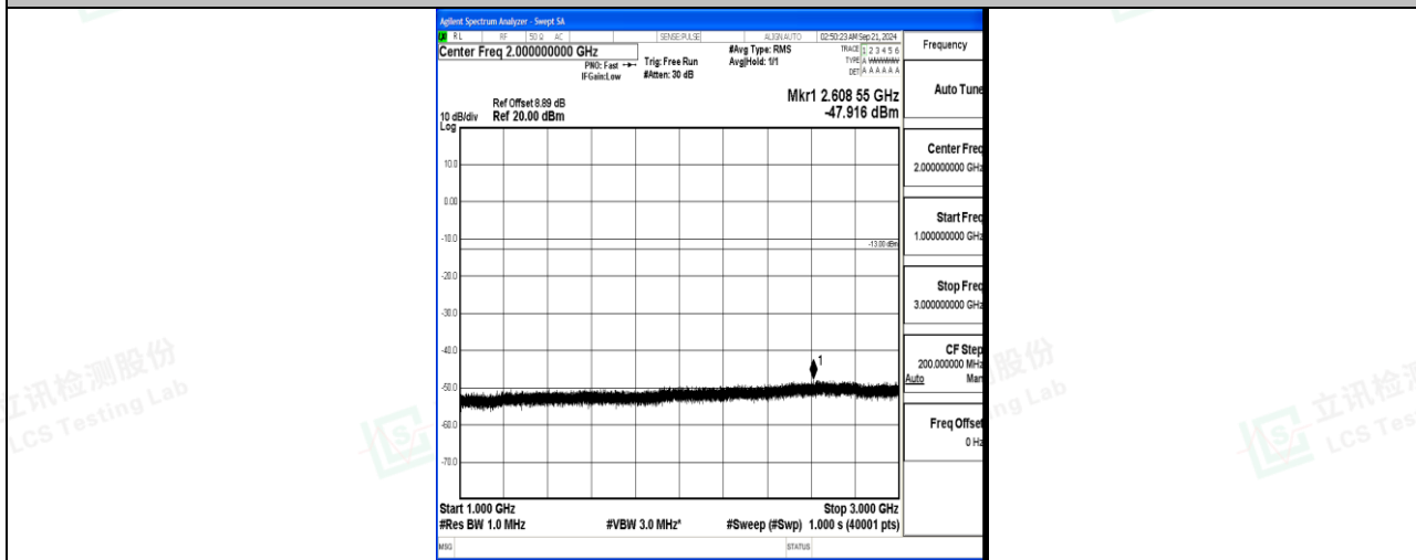
Band12_5MHz_16QAM_23155_1RB#0_1000~3000_1000~3000
