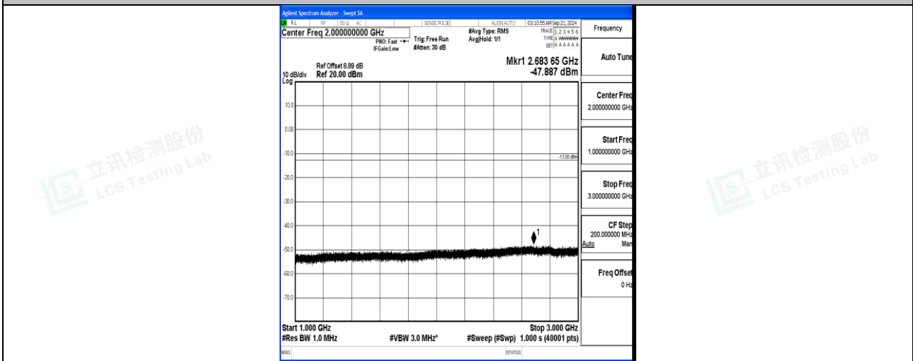
Band12_10MHz_QPSK_23130_1RB#0_1000~3000_1000~3000
