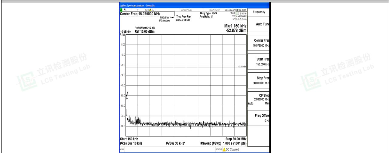
Band12_10MHz_16QAM_23130_1RB#0_0.15~30_0.15~30
