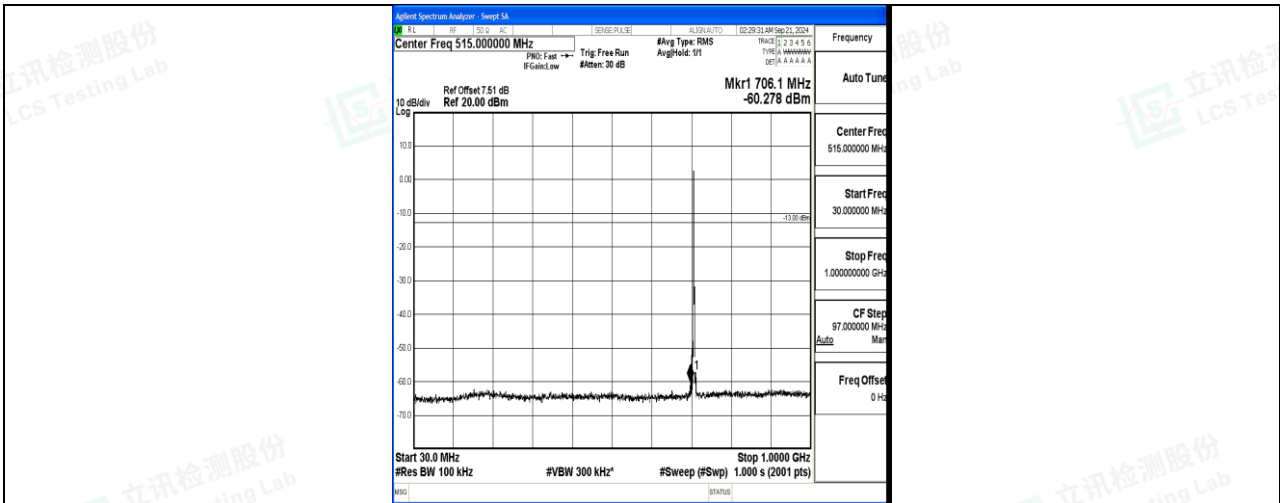
Band12_3MHz_16QAM_23165_1RB#0_30~1000_30~1000
