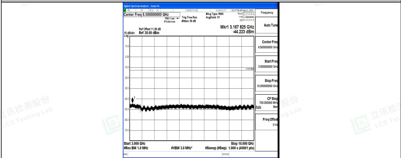
Band12_5MHz_QPSK_23035_1RB#0_3000~10000_3000~10000
