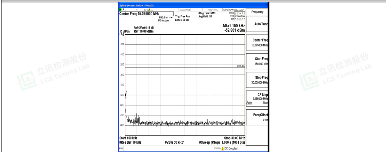
Band12_5MHz_QPSK_23095_1RB#0_0.15~30_0.15~30
