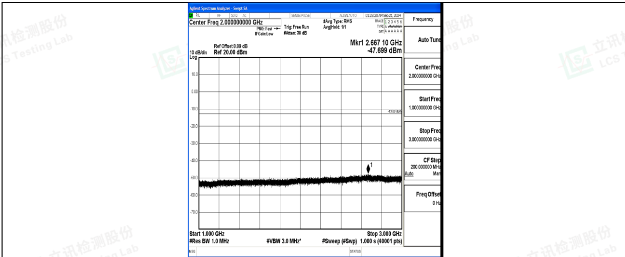
Band5_5MHz_16QAM_20525_1RB#0_1000~3000_1000~3000
