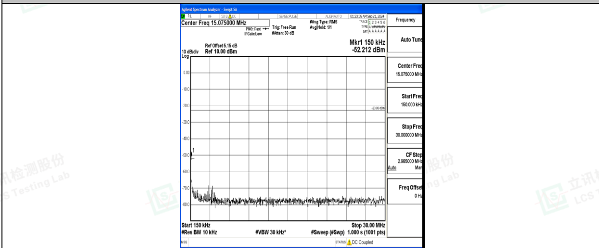
Band5_5MHz_16QAM_20525_1RB#0_0.15~30_0.15~30
