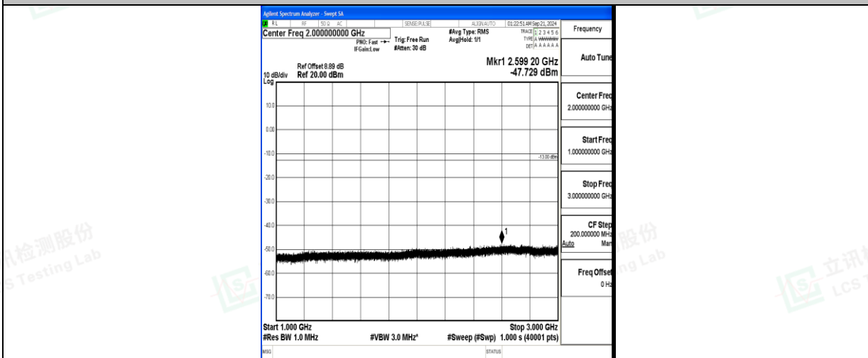
Band5_5MHz_QPSK_20525_1RB#0_1000~3000_1000~3000
