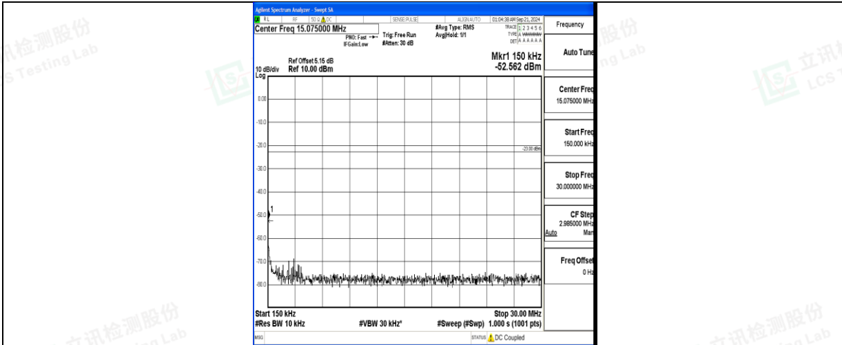
Band5_3MHz_QPSK_20635_1RB#0_0.15~30_0.15~30
