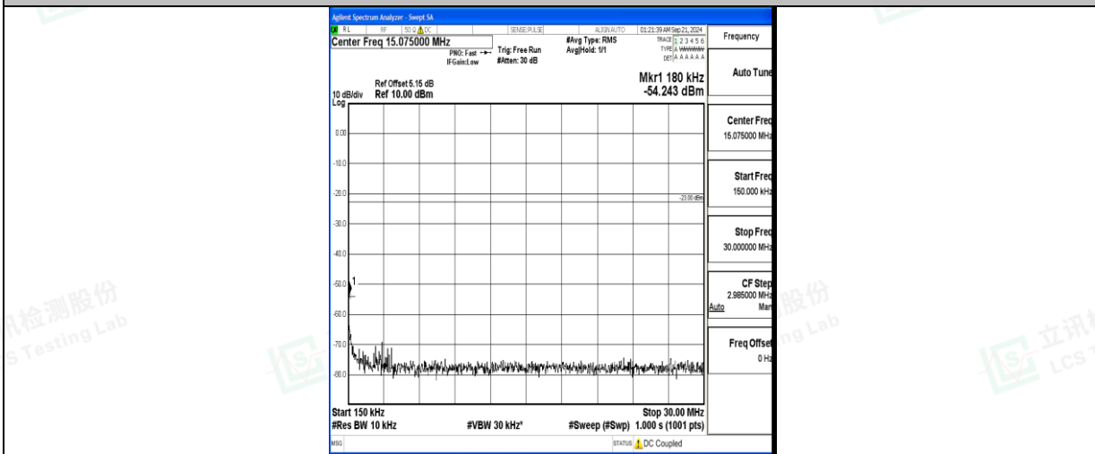
Band5_5MHz_QPSK_20425_1RB#0_0.15~30_0.15~30
