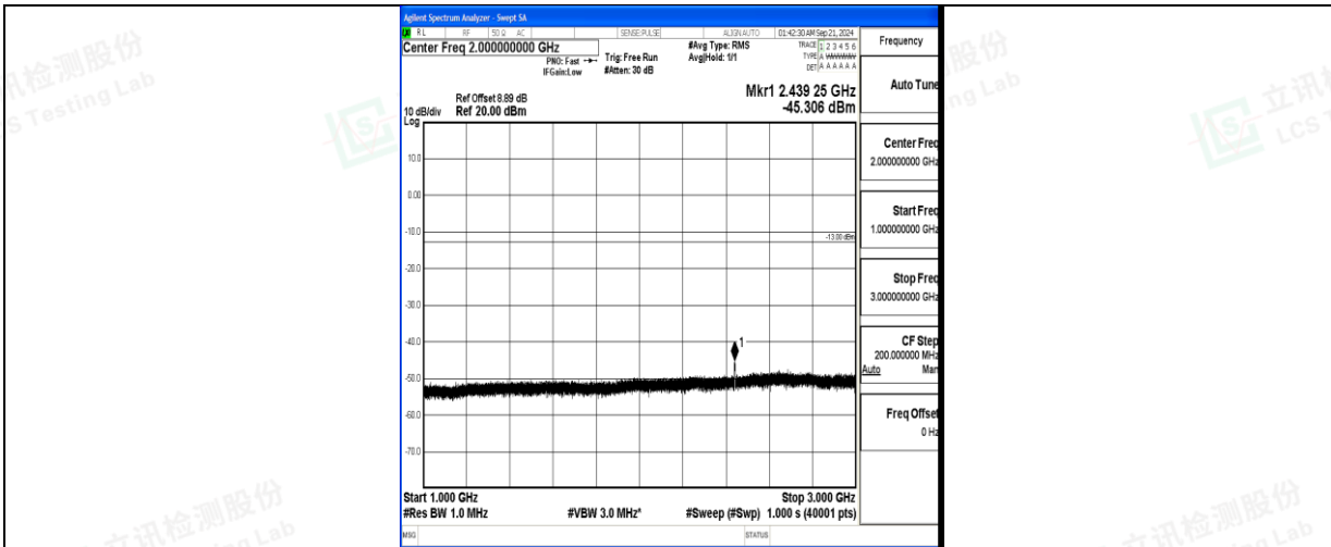
Band5_10MHz_16QAM_20525_1RB#0_1000~3000_1000~3000
