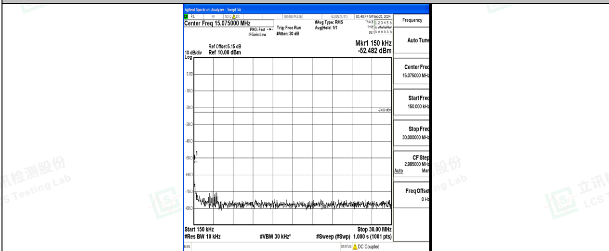
Band5_10MHz_QPSK_20450_1RB#0_0.15~30_0.15~30
