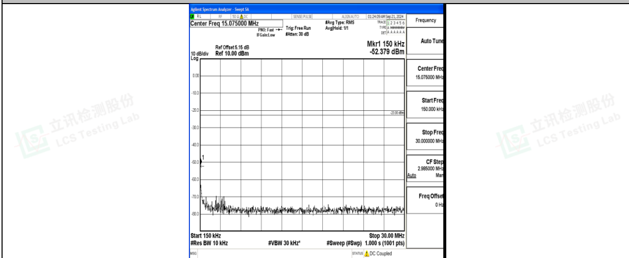
Band5_5MHz_16QAM_20625_1RB#0_0.15~30_0.15~30
