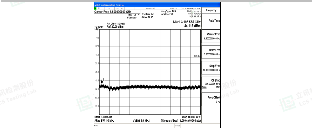
Band5_10MHz_16QAM_20525_1RB#0_3000~10000_3000~10000
