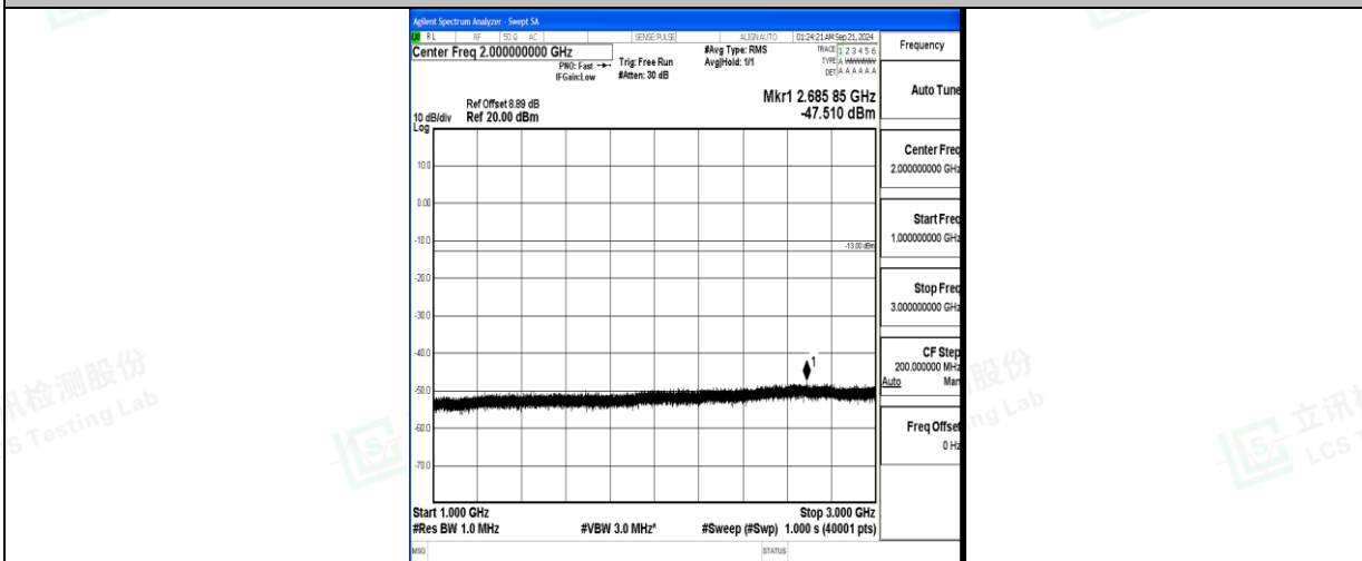
Band5_5MHz_16QAM_20625_1RB#0_1000~3000_1000~3000
