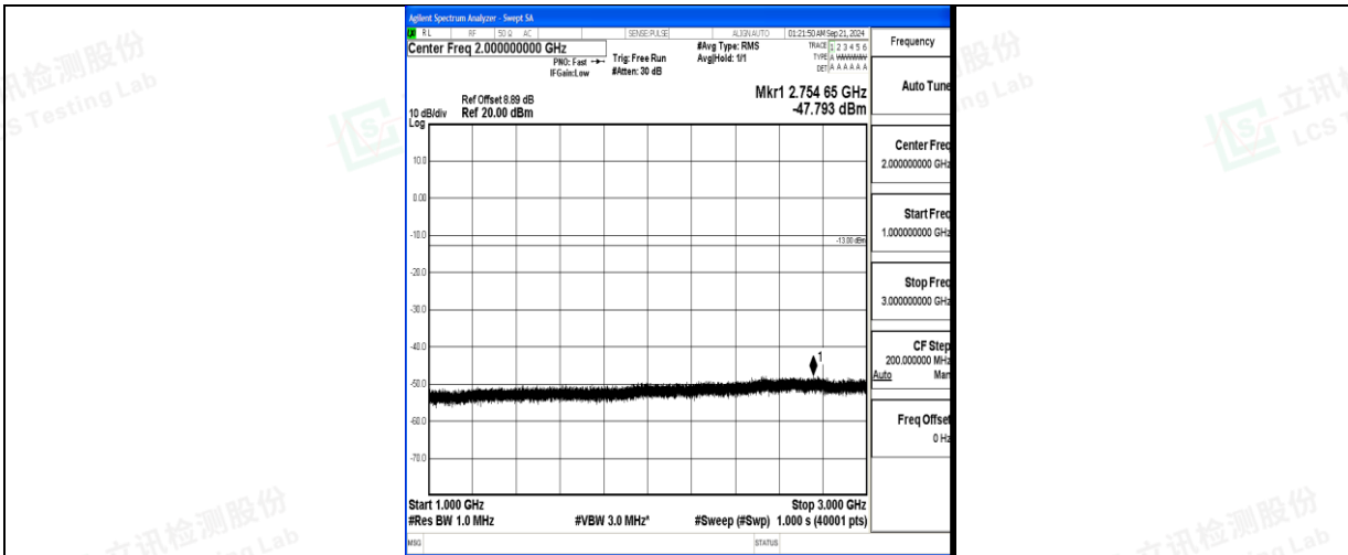
Band5_5MHz_QPSK_20425_1RB#0_1000~3000_1000~3000
