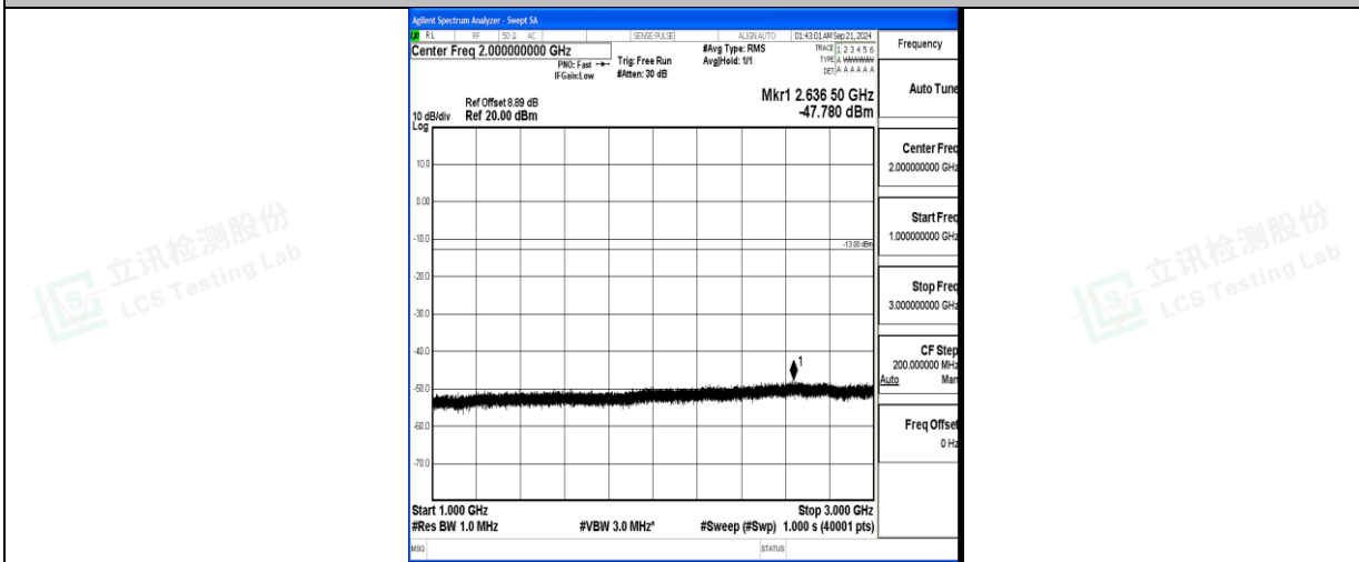
Band5_10MHz_QPSK_20600_1RB#0_1000~3000_1000~3000
