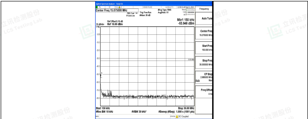
Band4_15MHz_16QAM_20325_1RB#0_0.15~30_0.15~30
