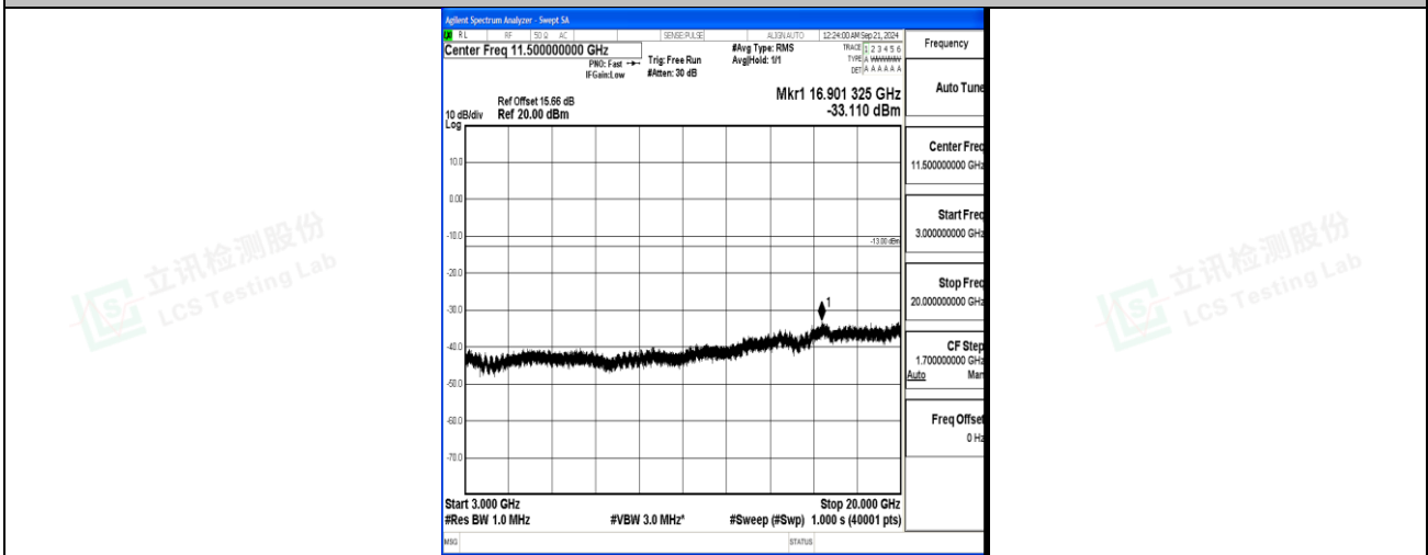
Band4_20MHz_16QAM_20175_1RB#0_3000~20000_3000~20000
