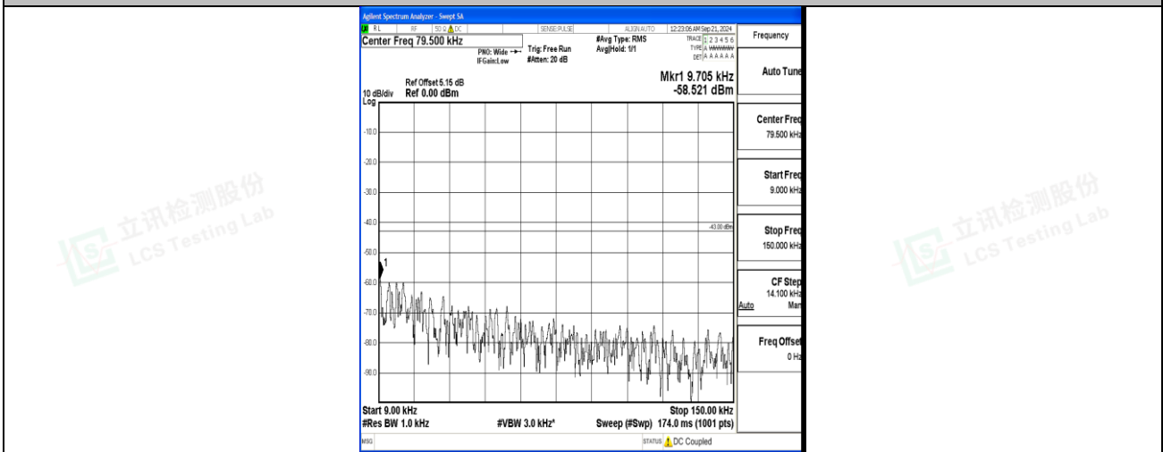
Band4_20MHz_QPSK_20175_1RB#0_0.009~0.15_0.009~0.15
