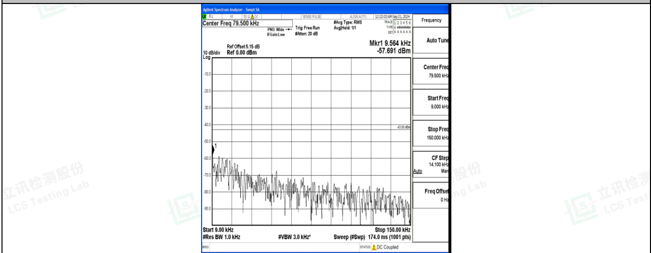
Band4_20MHz_QPSK_20050_1RB#0_0.009~0.15_0.009~0.15
