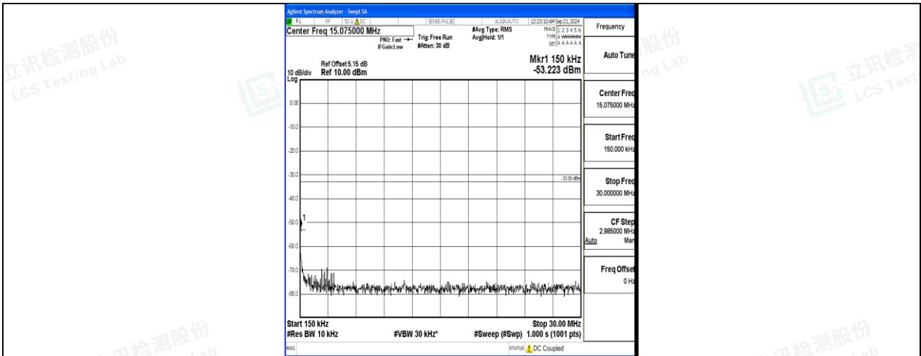
Band4_20MHz_QPSK_20175_1RB#0_0.15~30_0.15~30
