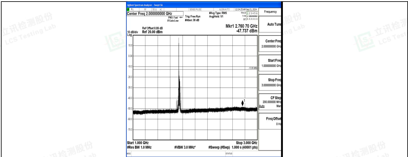
Band4_20MHz_QPSK_20300_1RB#0_1000~3000_1000~3000
