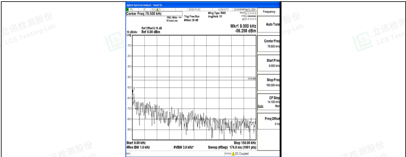
Band4_20MHz_QPSK_20300_1RB#0_0.009~0.15_0.009~0.15
