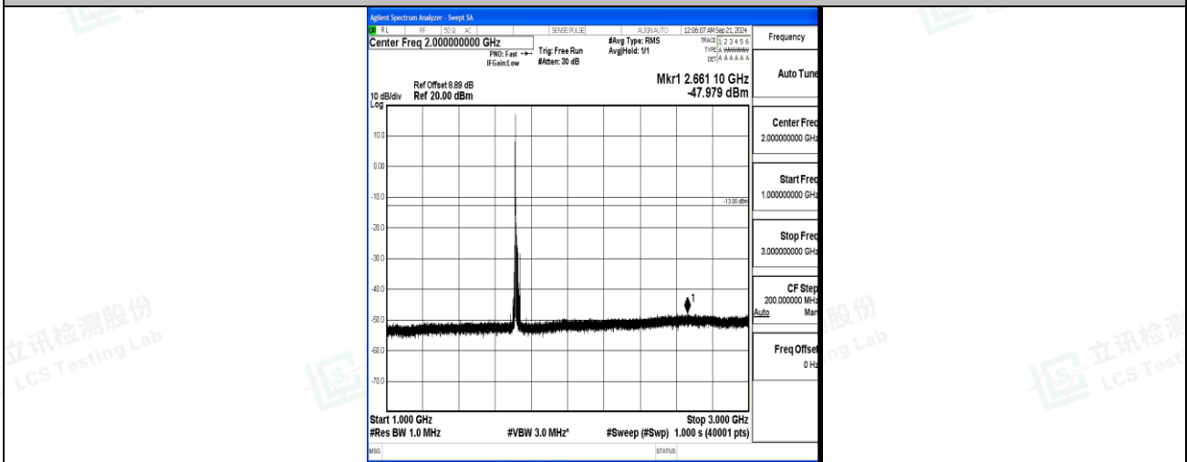
Band4_15MHz_QPSK_2025_1RB#0_1000~3000_1000~3000
