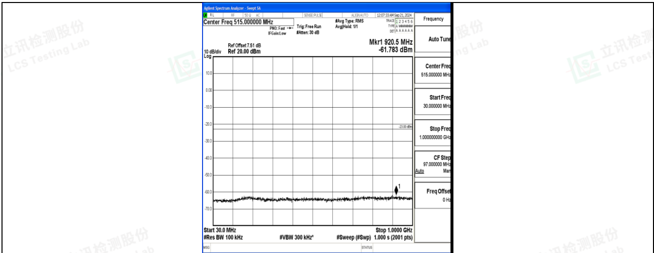
Band4_15MHz_16QAM_20175_1RB#0_30~1000_30~1000
