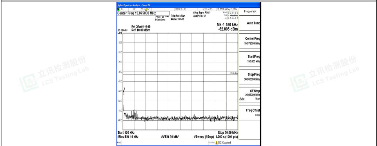
Band4_15MHz_16QAM_20175_1RB#0_0.15~30_0.15~30
