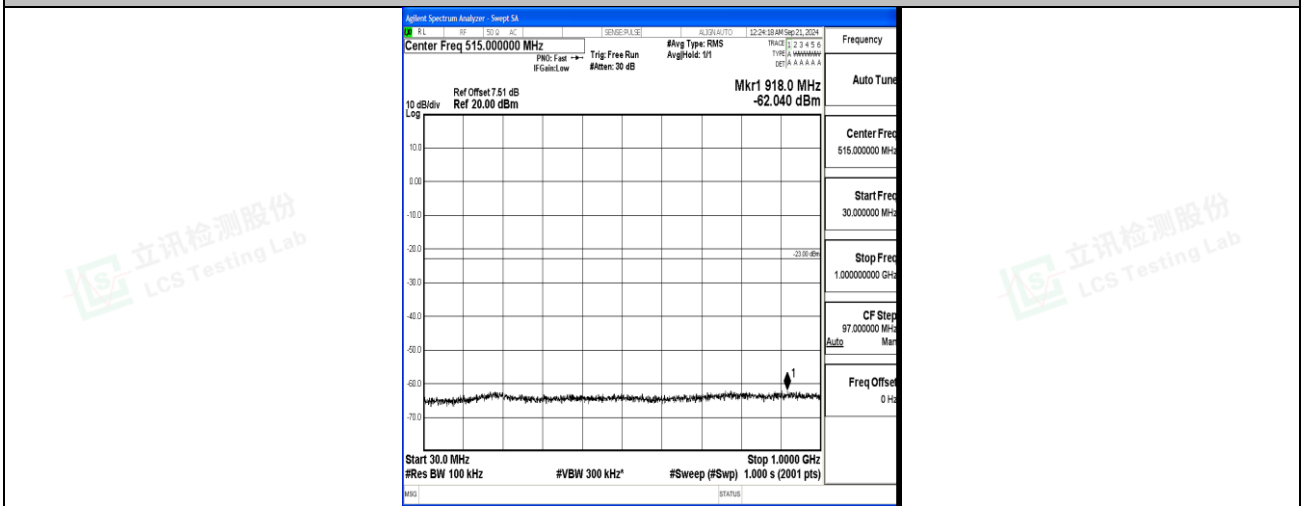
Band4_20MHz_QPSK_20300_1RB#0_30~1000_30~1000
