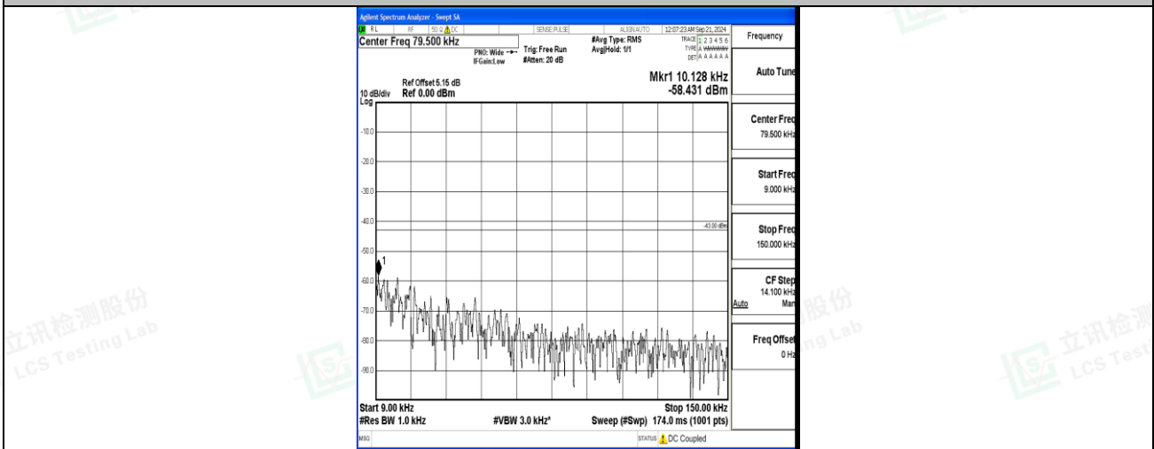
Band4_15MHz_16QAM_20175_1RB#0_0.009~0.15_0.009~0.15
