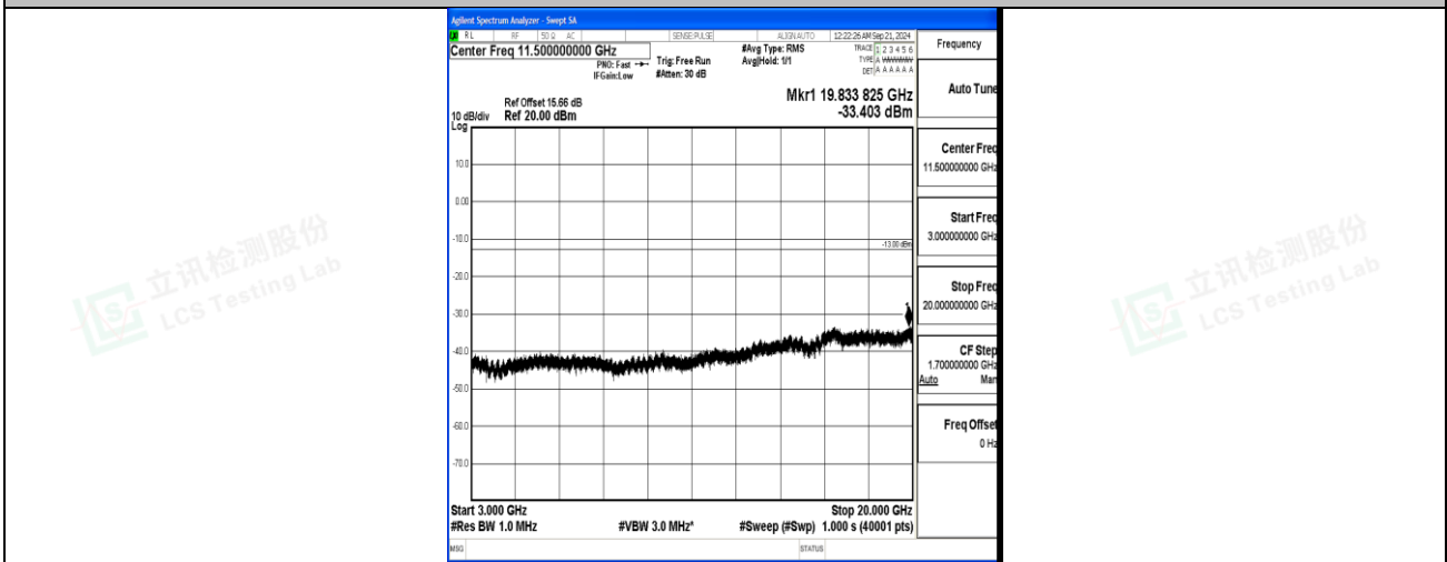
Band4_20MHz_QPSK_20050_1RB#0_3000~20000_3000~20000
