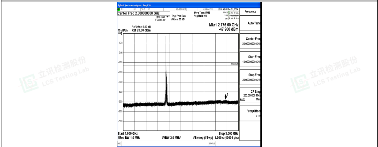
Band4_15MHz_16QAM_20325_1RB#0_1000~3000_1000~3000
