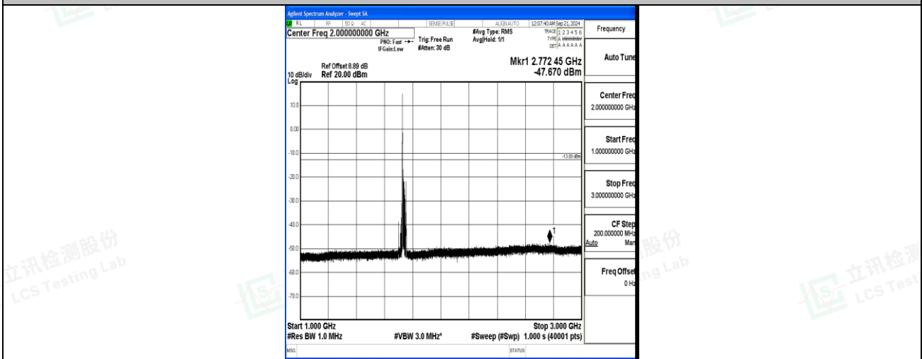
Band4_15MHz_16QAM_20175_1RB#0_1000~3000_1000~3000
