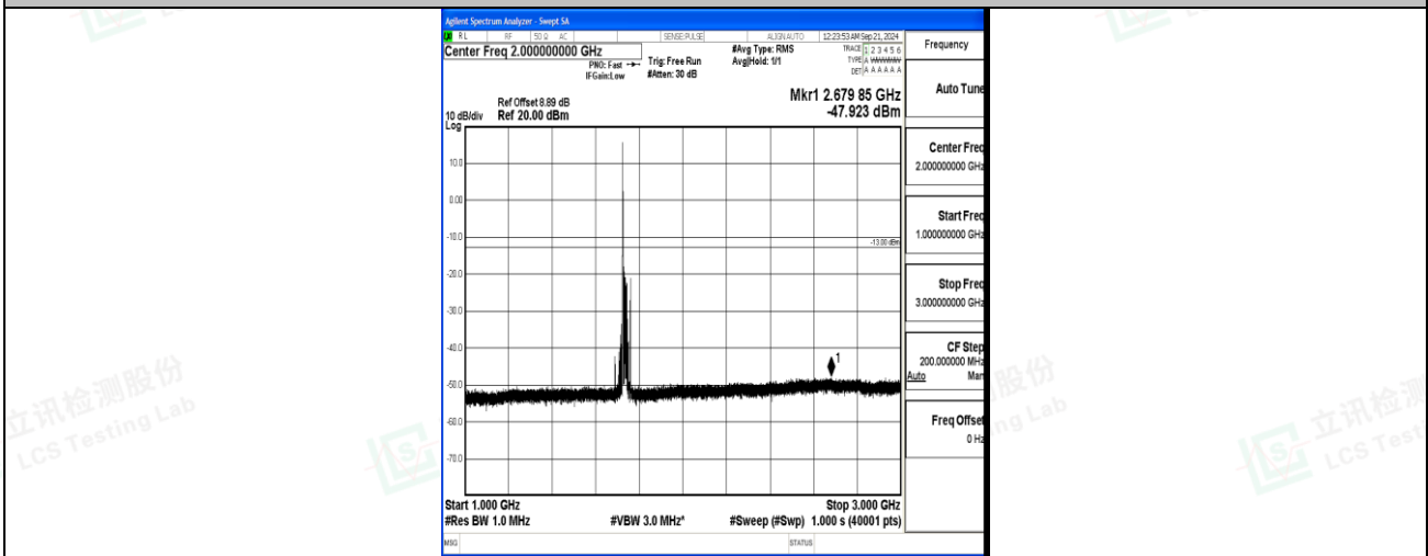
Band4_20MHz_16QAM_20175_1RB#0_1000~3000_1000~3000
