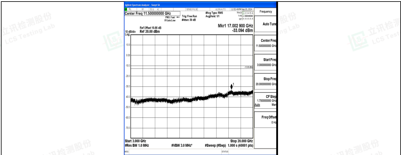
Band4_10MHz_16QAM_20350_1RB#0_3000~20000_3000~20000
