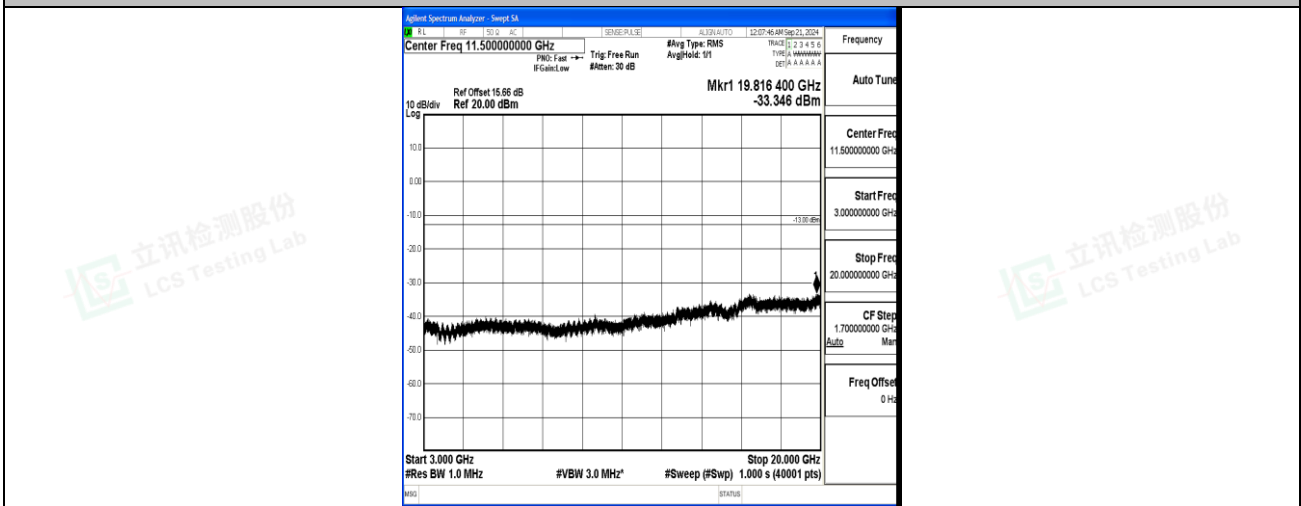
Band4_15MHz_16QAM_20175_1RB#0_3000~20000_3000~20000
