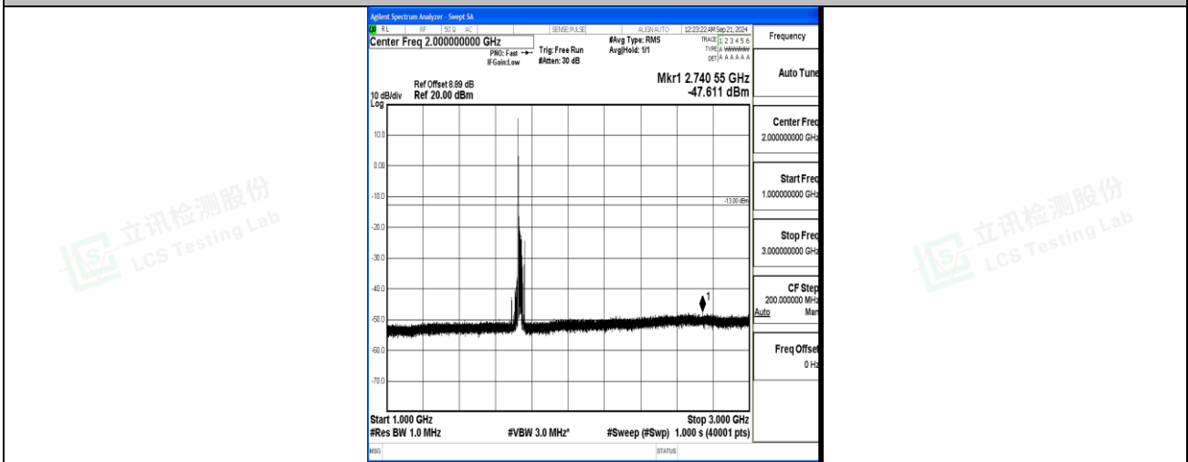
Band4_20MHz_QPSK_20175_1RB#0_1000~3000_1000~3000
