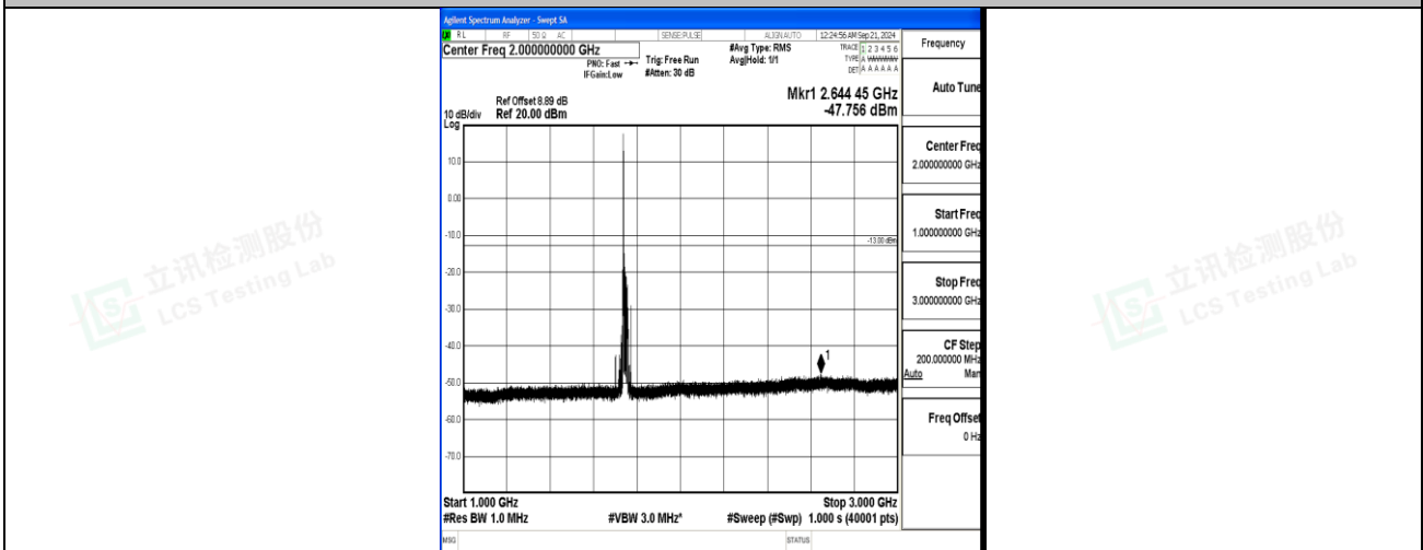
Band4_20MHz_16QAM_20300_1RB#0_1000~3000_1000~3000
