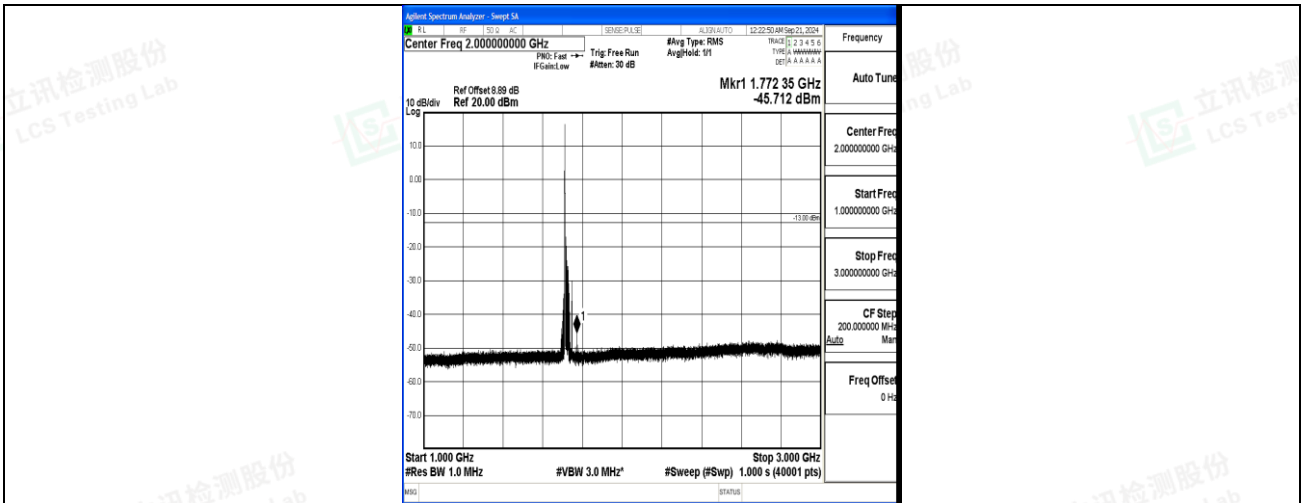
Band4_20MHz_16QAM_20050_1RB#0_1000~3000_1000~3000
