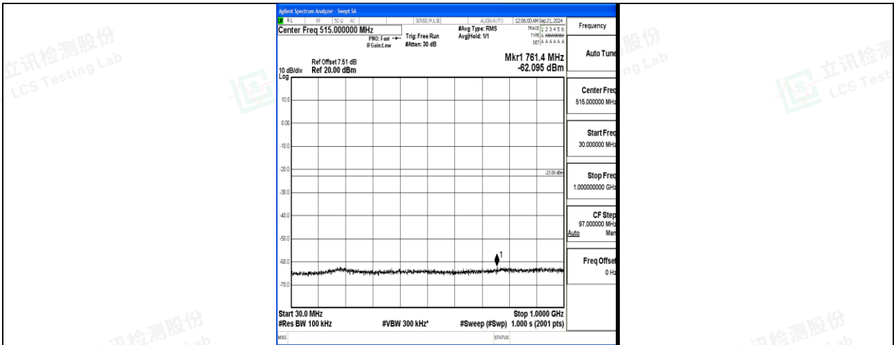
Band4_15MHz_QPSK_2025_1RB#0_30~1000_30~1000
