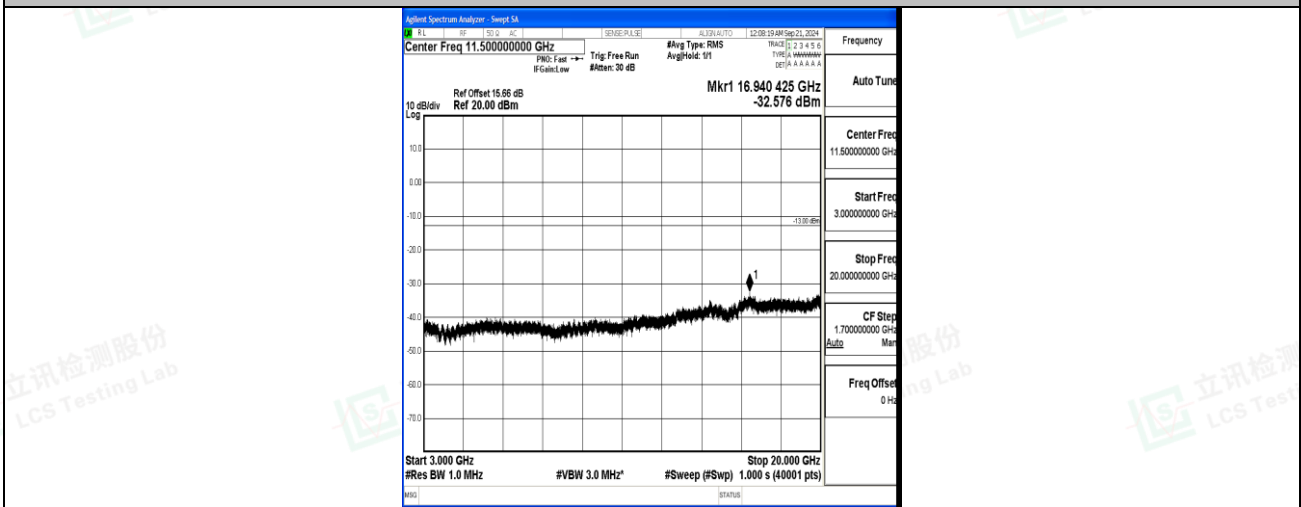
Band4_15MHz_QPSK_20325_1RB#0_3000~20000_3000~20000
