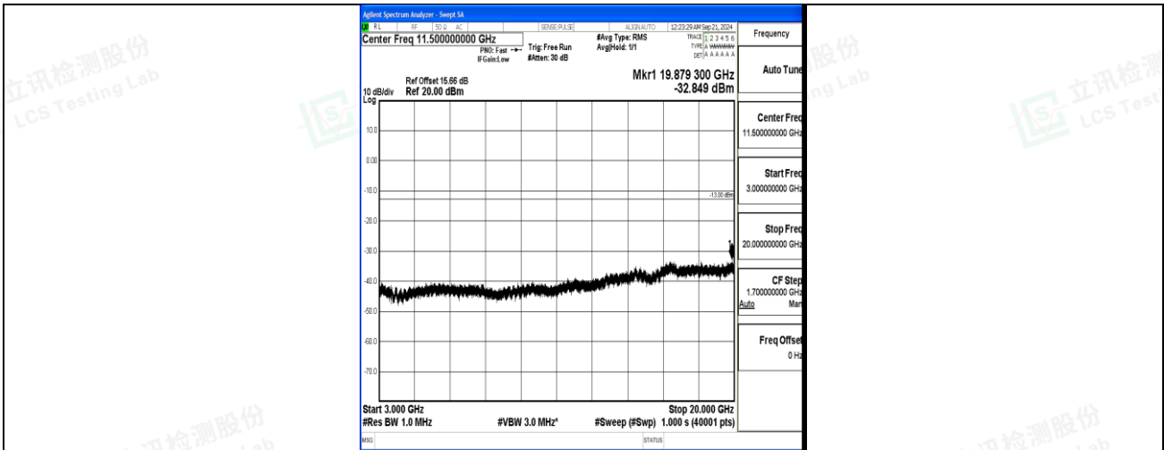
Band4_20MHz_QPSK_20175_1RB#0_3000~20000_3000~20000
