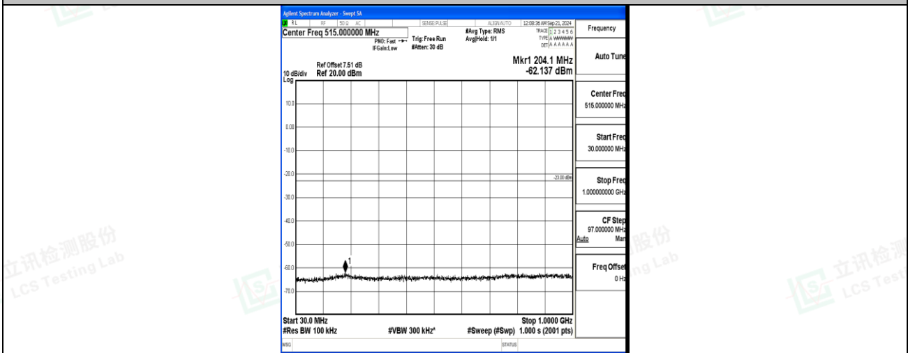
Band4_15MHz_16QAM_20325_1RB#0_30~1000_30~1000
