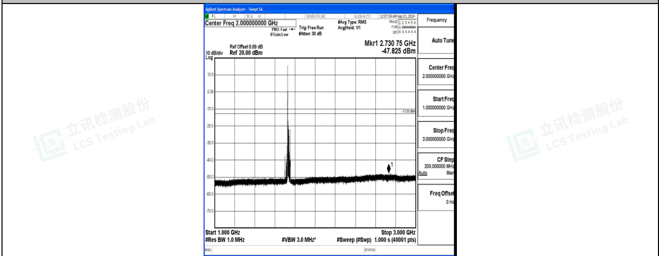
Band4_15MHz_QPSK_20175_1RB#0_1000~3000_1000~3000
