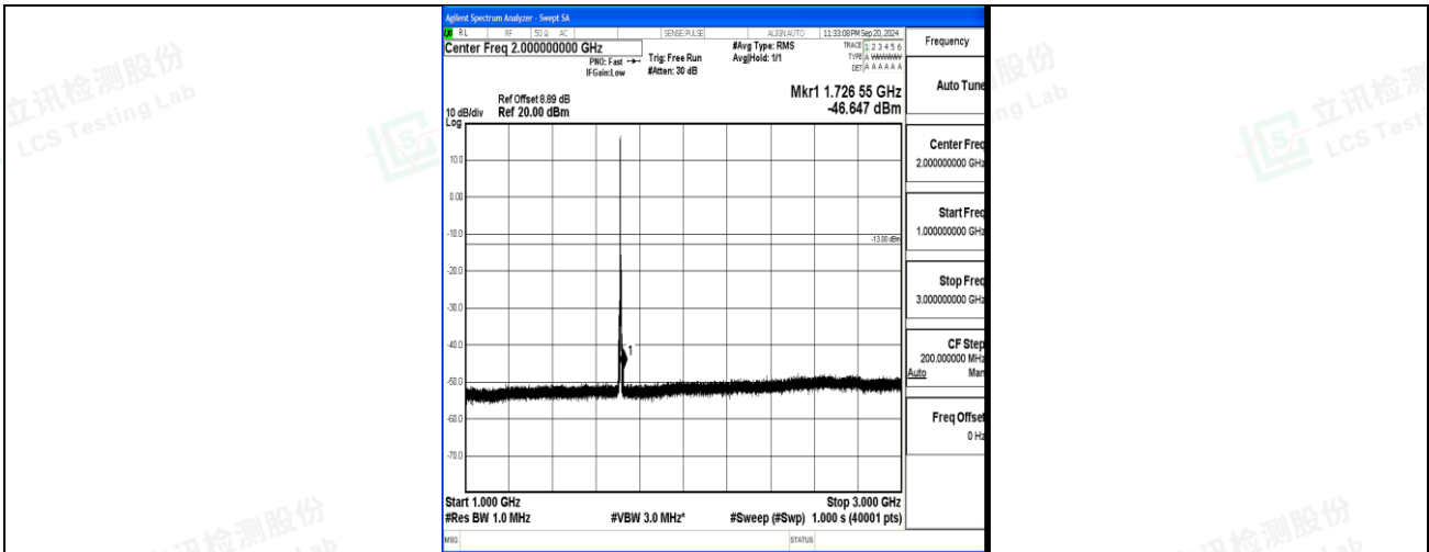
Band4_5MHz_16QAM_19975_1RB#0_1000~3000_1000~3000
