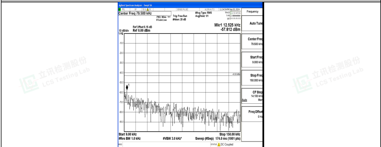
Band4_5MHz_16QAM_20375_1RB#0_0.009~0.15_0.009~0.15
