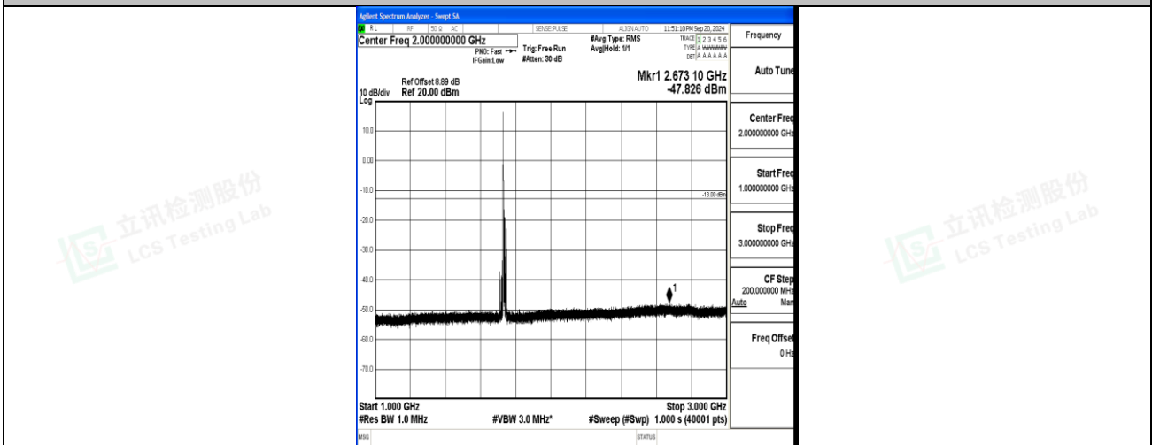
Band4_10MHz_QPSK_20175_1RB#0_1000~3000_1000~3000
