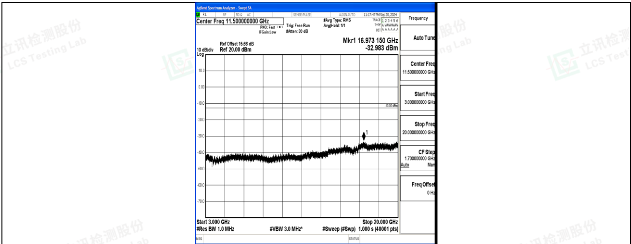
Band4_3MHz_16QAM_20385_1RB#0_3000~20000_3000~20000
