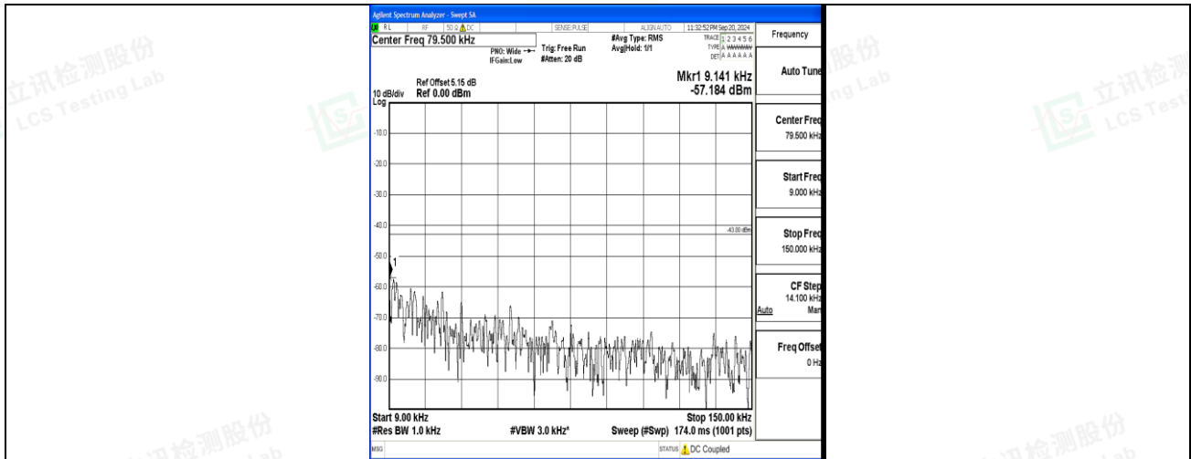
Band4_5MHz_16QAM_19975_1RB#0_0.009~0.15_0.009~0.15
