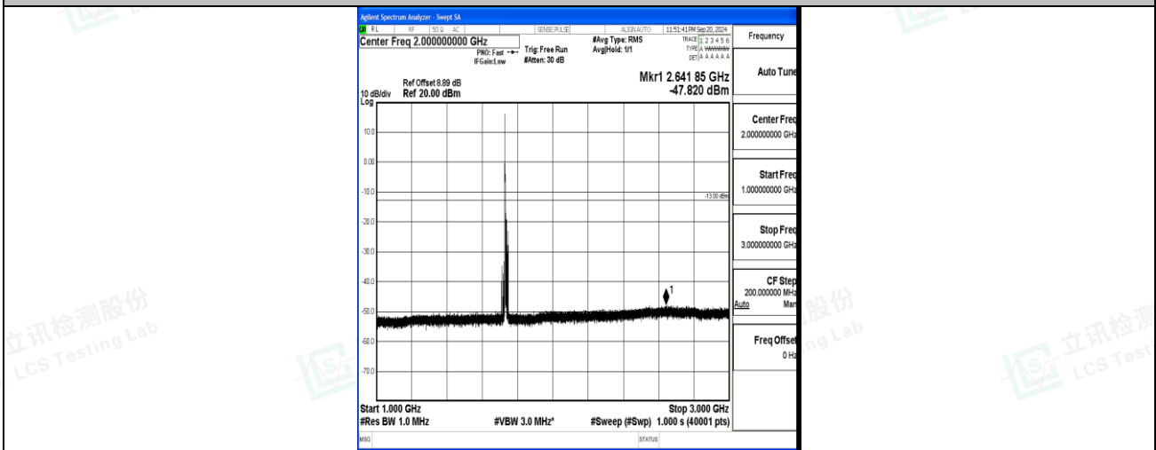
Band4_10MHz_16QAM_20175_1RB#0_1000~3000_1000~3000
