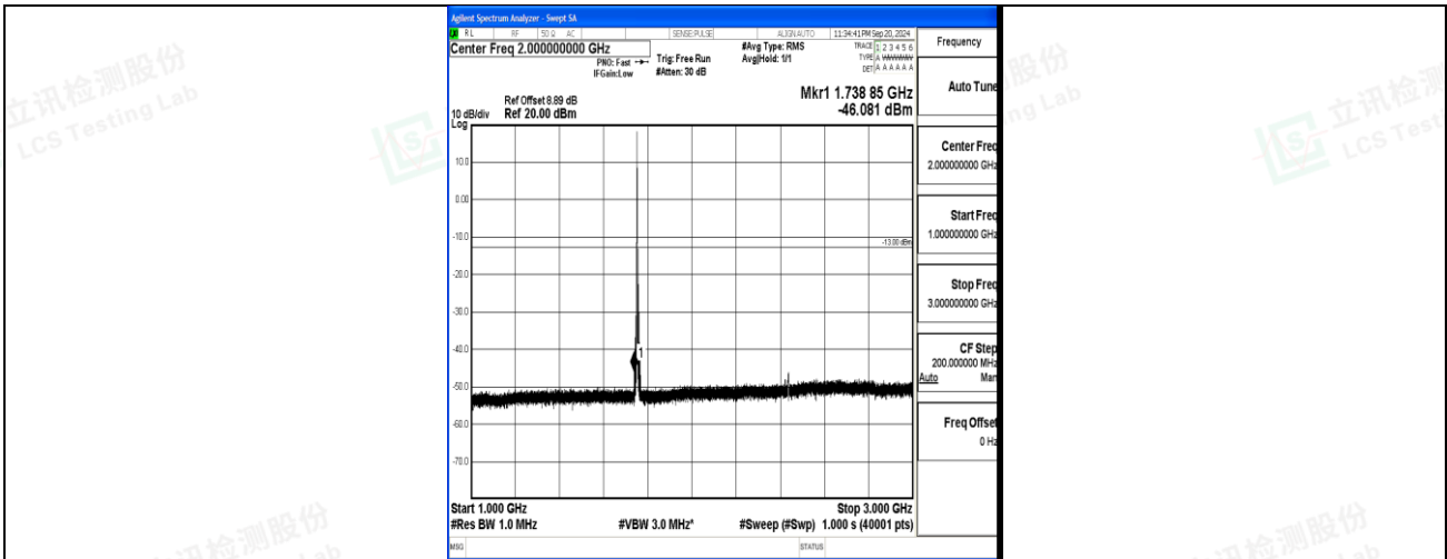
Band4_5MHz_QPSK_20375_1RB#0_1000~3000_1000~3000
