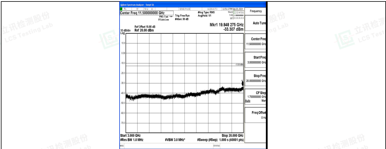
Band4_10MHz_QPSK_20175_1RB#0_3000~20000_3000~20000
