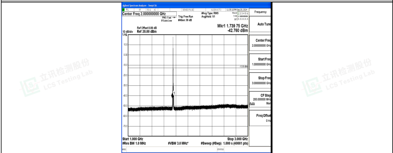
Band4_5MHz_16QAM_20375_1RB#0_1000~3000_1000~3000
