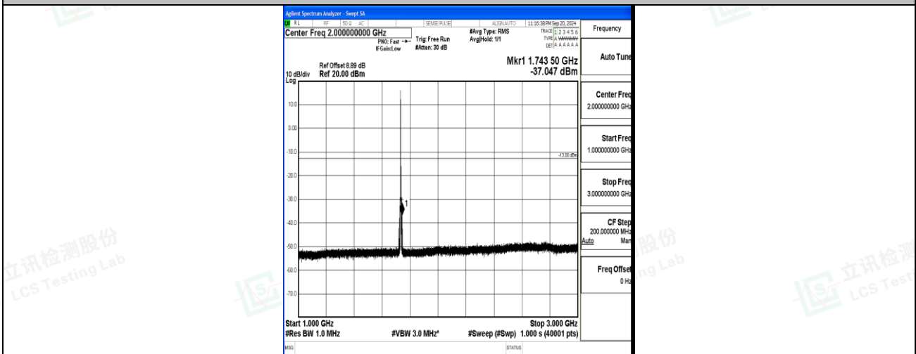
Band4_3MHz_16QAM_20175_1RB#0_1000~3000_1000~3000
