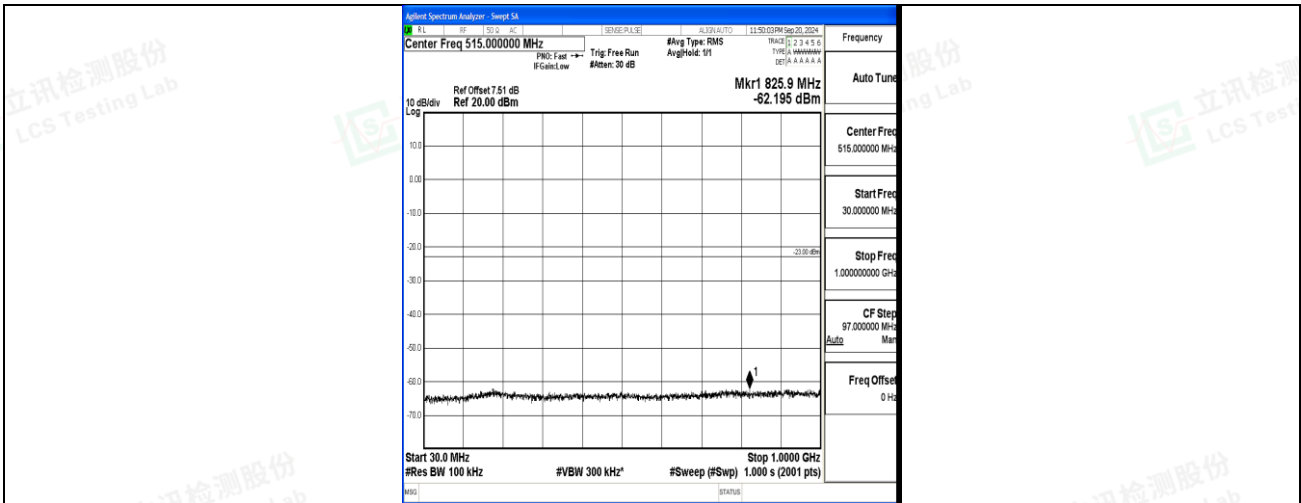
Band4_10MHz_QPSK_20000_1RB#0_30~1000_30~1000
