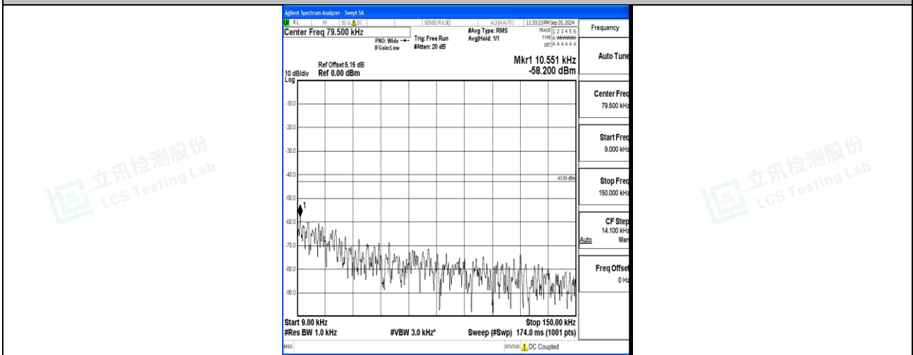
Band4_5MHz_QPSK_20175_1RB#0_0.009~0.15_0.009~0.15
