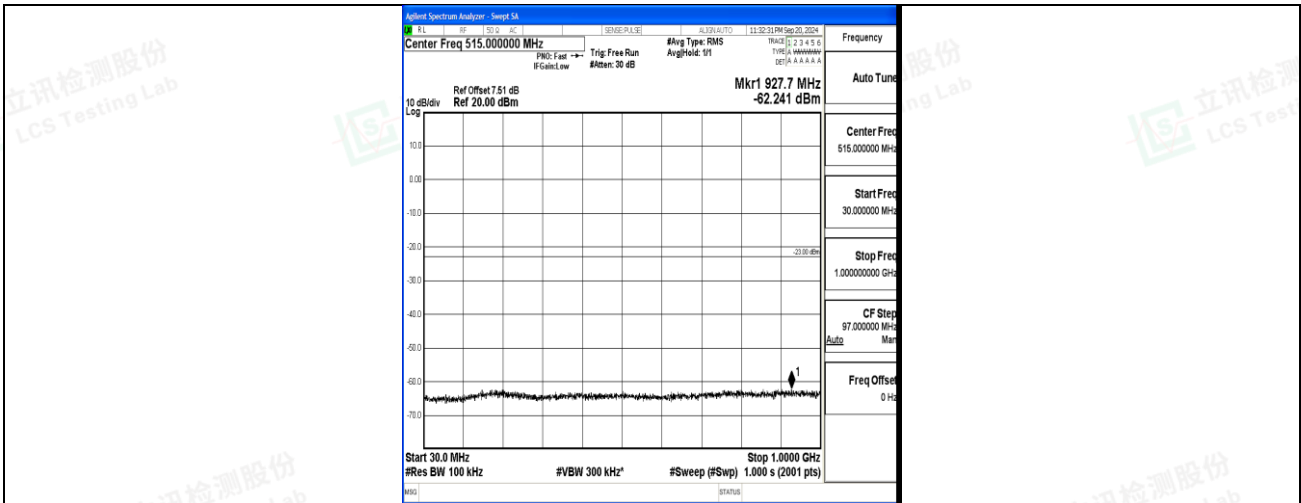
Band4_5MHz_QPSK_19975_1RB#0_30~1000_30~1000
