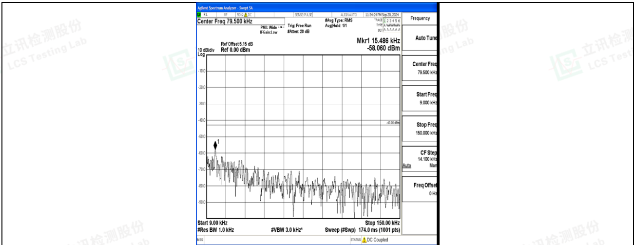
Band4_5MHz_QPSK_20375_1RB#0_0.009~0.15_0.009~0.15
