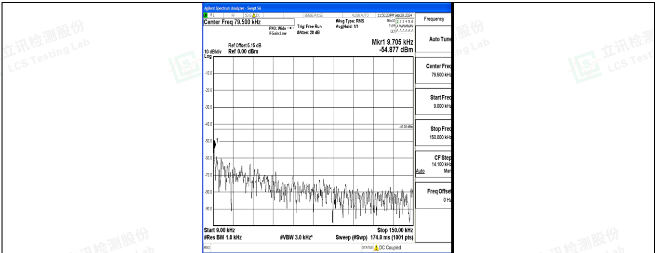
Band4_10MHz_16QAM_20000_1RB#0_0.009~0.15_0.009~0.15
