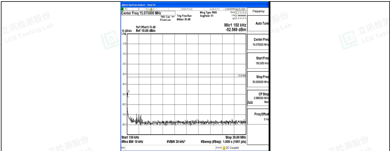
Band4_10MHz_QPSK_20175_1RB#0_0.15~30_0.15~30
