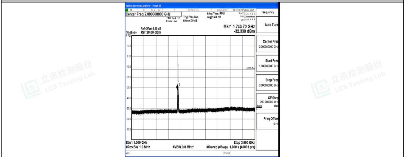
Band4_3MHz_16QAM_20385_1RB#0_1000~3000_1000~3000
