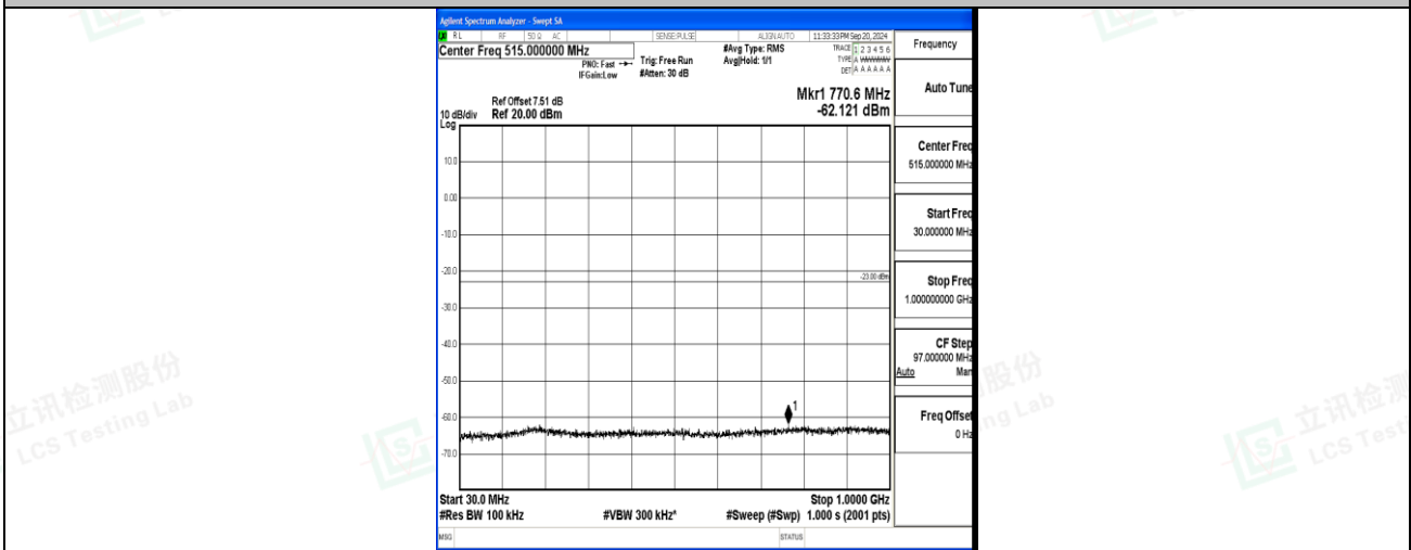
Band4_5MHz_QPSK_20175_1RB#0_30~1000_30~1000
