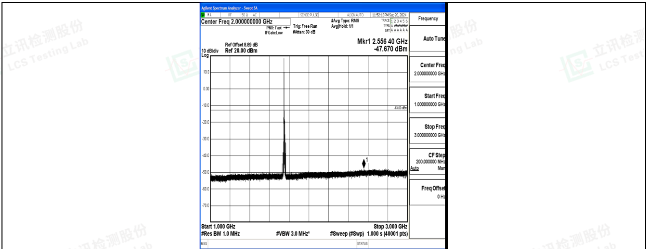
Band4_10MHz_QPSK_20350_1RB#0_1000~3000_1000~3000
