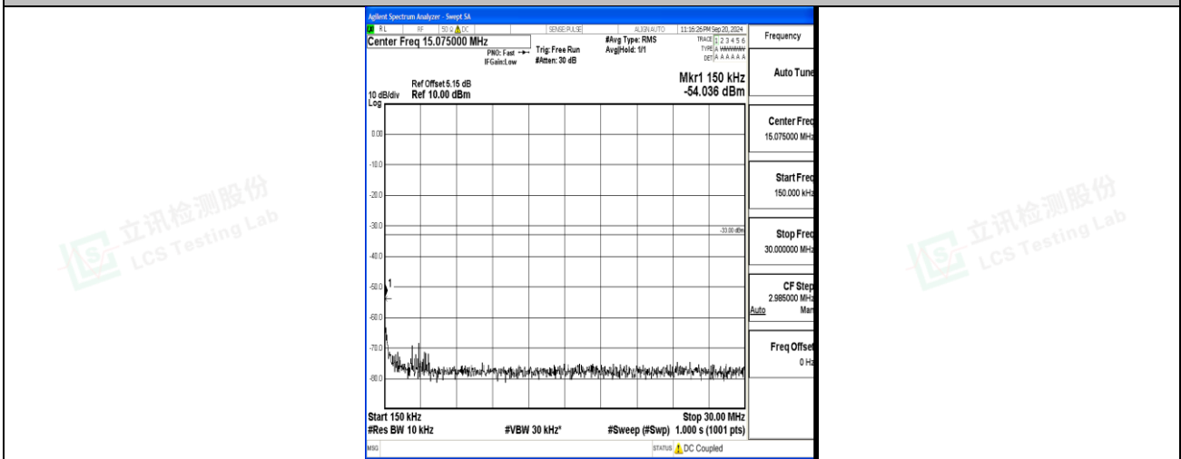
Band4_3MHz_16QAM_20175_1RB#0_0.15~30_0.15~30
