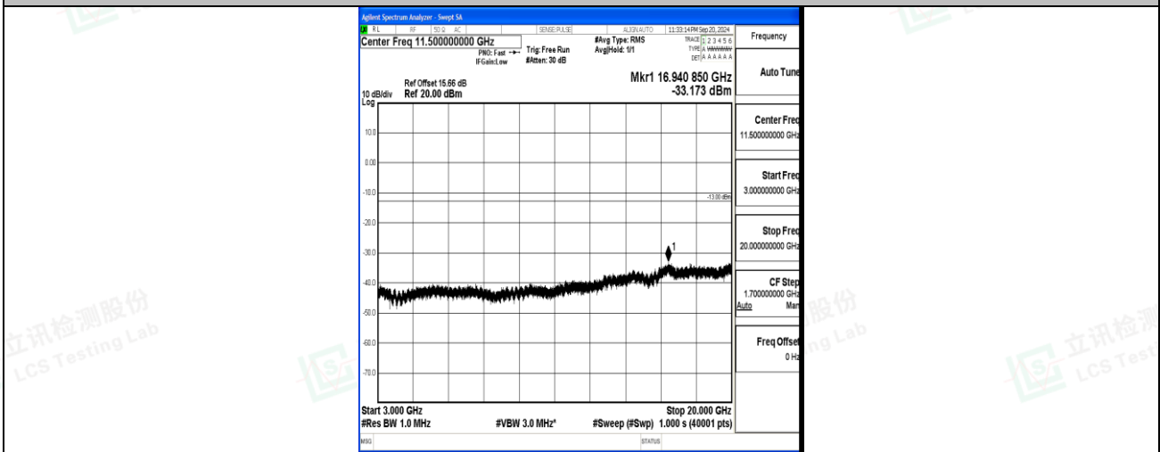
Band4_5MHz_16QAM_19975_1RB#0_3000~20000_3000~20000
