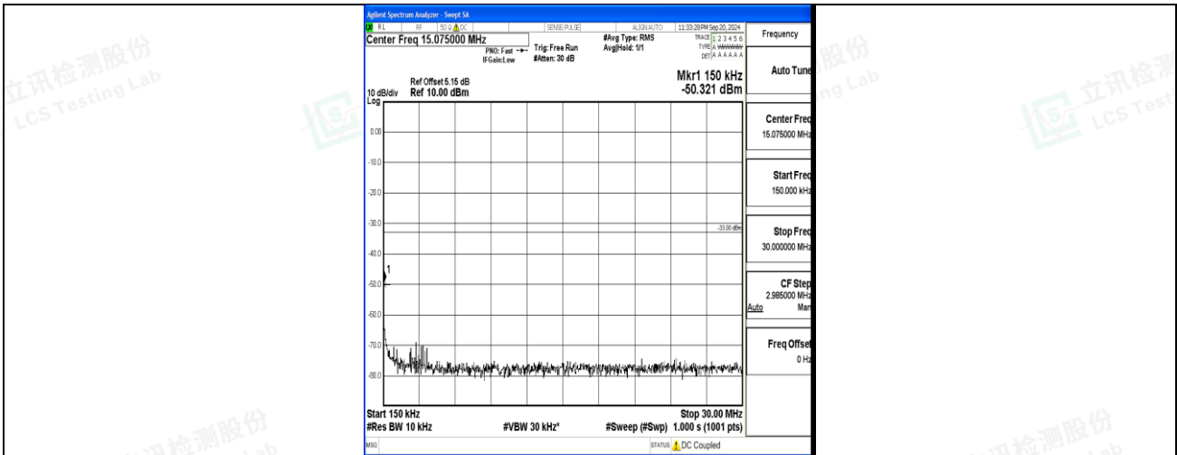
Band4_5MHz_QPSK_20175_1RB#0_0.15~30_0.15~30
