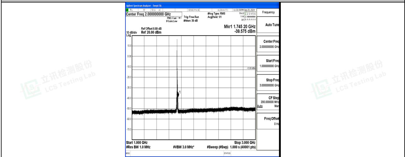
Band4_5MHz_QPSK_20175_1RB#0_1000~3000_1000~3000
