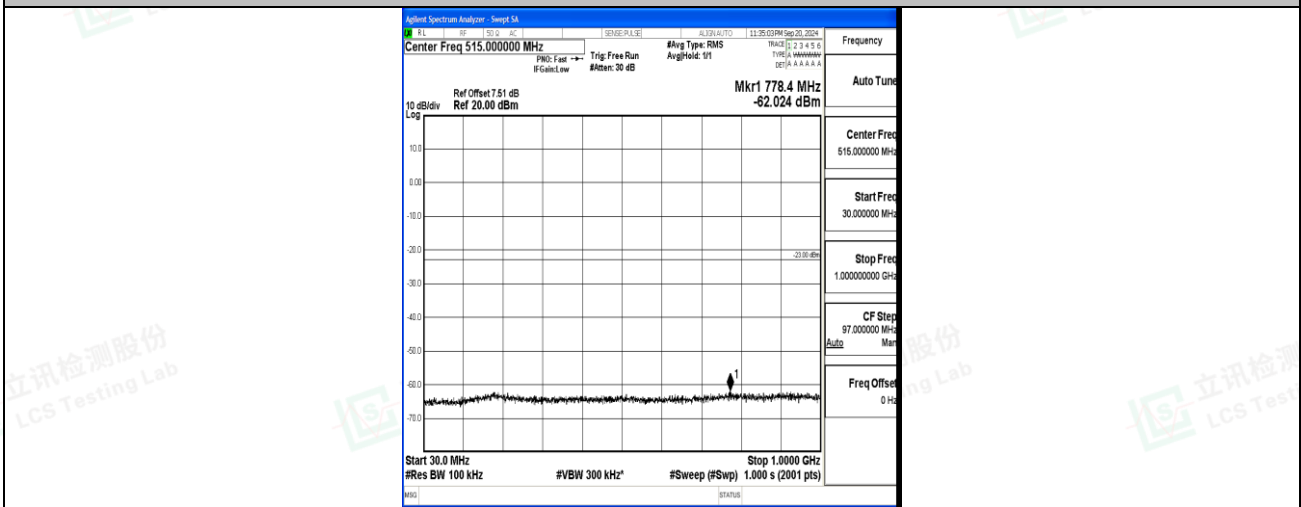
Band4_5MHz_16QAM_20375_1RB#0_30~1000_30~1000
