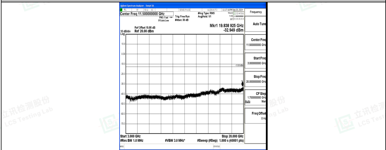
Band4_3MHz_QPSK_20385_1RB#0_3000~20000_3000~20000
