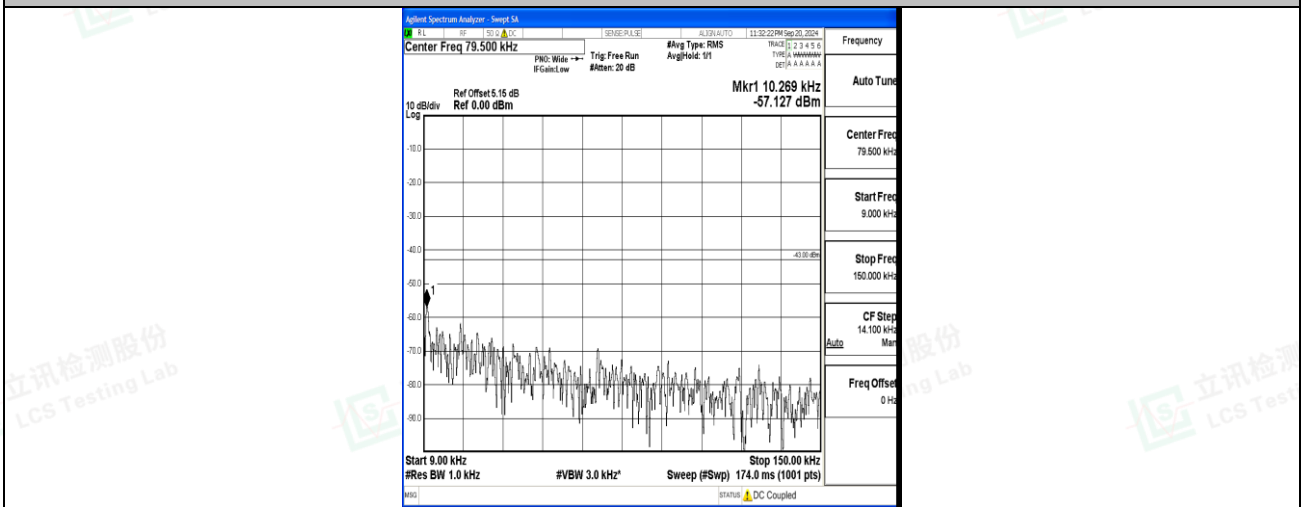
Band4_5MHz_QPSK_19975_1RB#0_0.009~0.15_0.009~0.15
