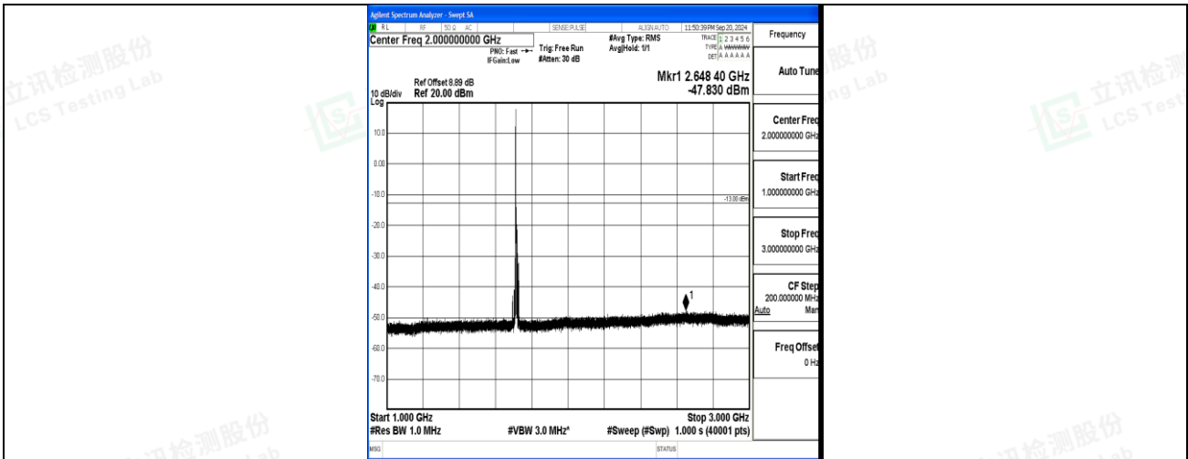
Band4_10MHz_16QAM_20000_1RB#0_1000~3000_1000~3000
