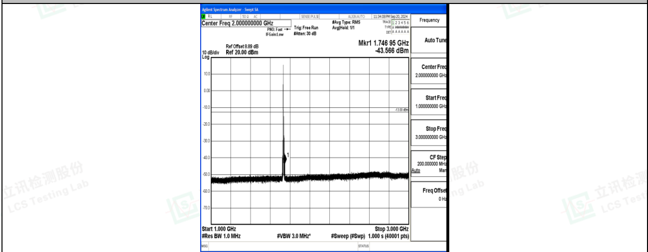
Band4_5MHz_16QAM_20175_1RB#0_1000~3000_1000~3000
