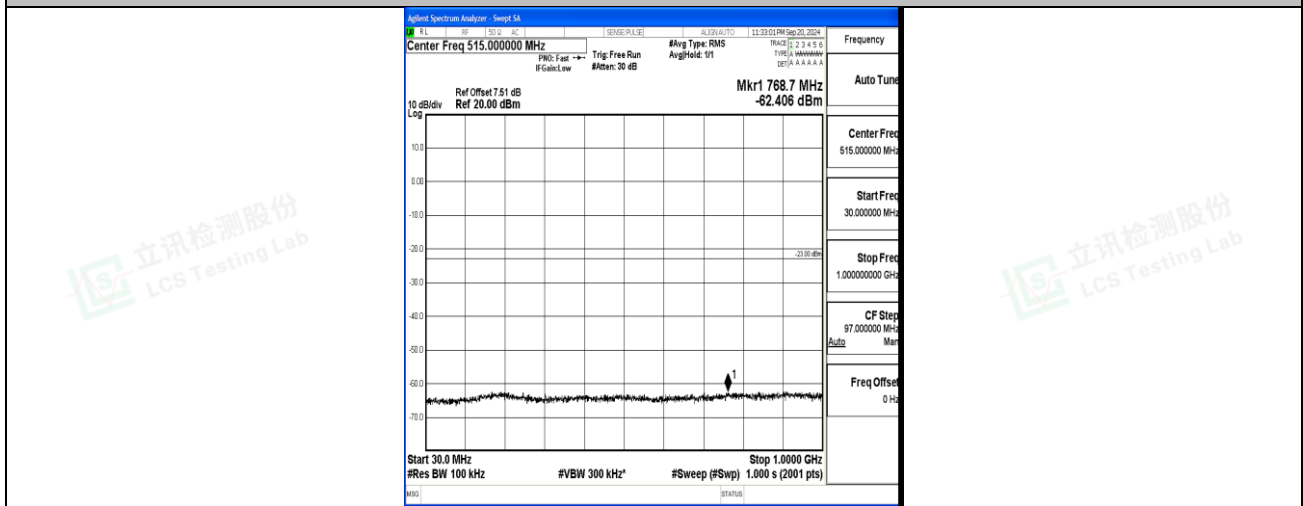
Band4_5MHz_16QAM_19975_1RB#0_30~1000_30~1000
