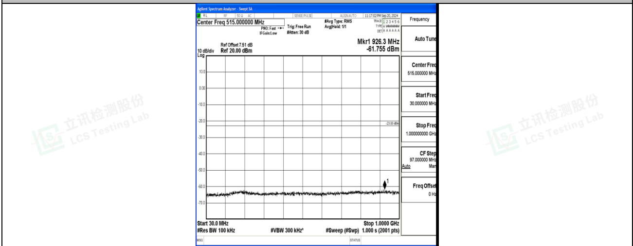
Band4_3MHz_QPSK_20385_1RB#0_30~1000_30~1000
