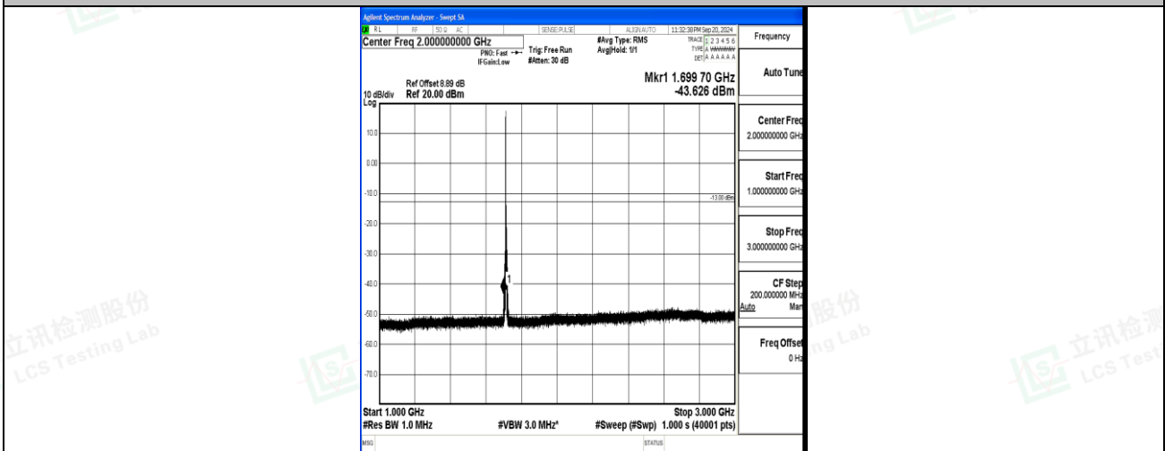
Band4_5MHz_QPSK_19975_1RB#0_1000~3000_1000~3000
