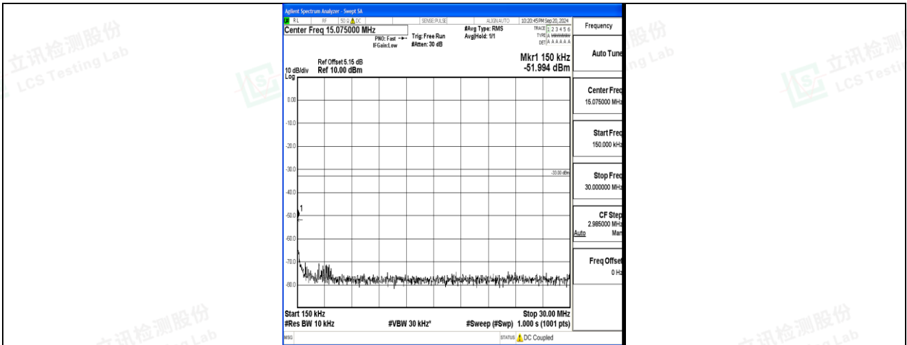
Band2_15MHz_16QAM_18900_1RB#0_0.15~30_0.15~30
