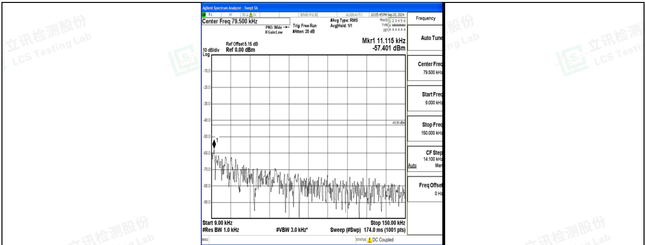
Band2_10MHz_16QAM_19150_1RB#0_0.009~0.15_0.009~0.15
