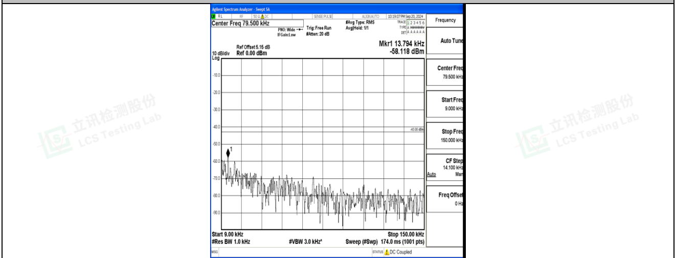
Band2_15MHz_QPSK_18675_1RB#0_0.009~0.15_0.009~0.15
