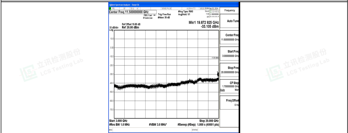
Band2_15MHz_QPSK_19125_1RB#0_3000~20000_3000~20000
