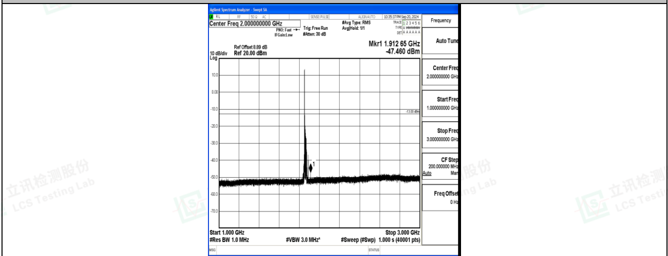
Band2_20MHz_16QAM_18700_1RB#0_1000~3000_1000~3000
