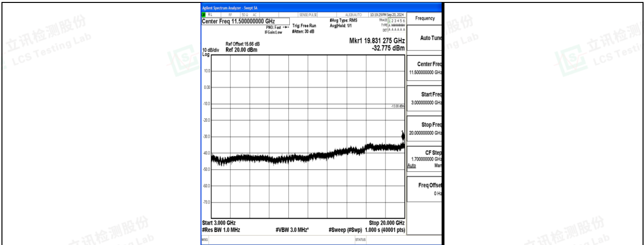
Band2_15MHz_QPSK_18675_1RB#0_3000~20000_3000~20000
