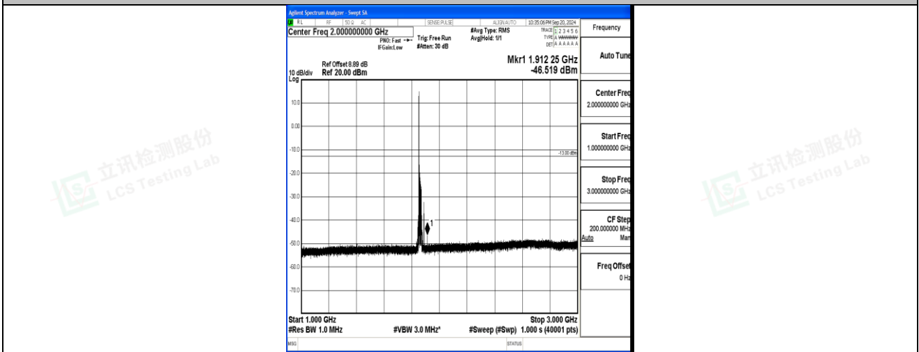
Band2_20MHz_QPSK_18700_1RB#0_1000~3000_1000~3000
