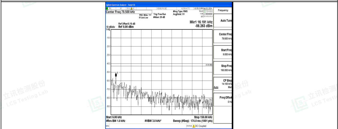
Band2_20MHz_16QAM_18700_1RB#0_0.009~0.15_0.009~0.15
