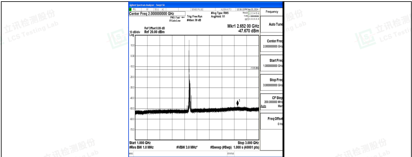
Band2_20MHz_QPSK_18900_1RB#0_1000~3000_1000~3000
