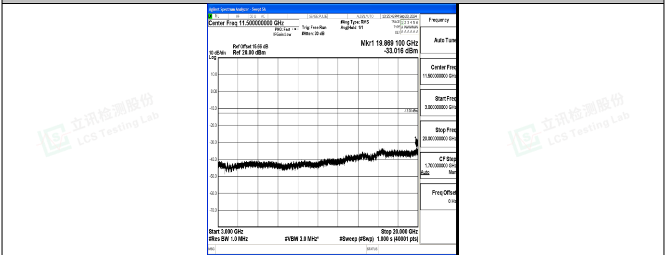
Band2_20MHz_16QAM_18700_1RB#0_3000~20000_3000~20000
