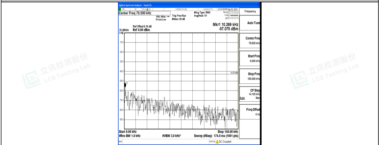
Band2_20MHz_QPSK_18700_1RB#0_0.009~0.15_0.009~0.15
