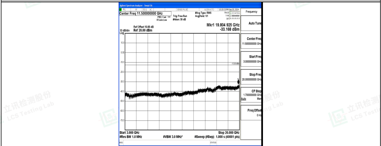
Band2_15MHz_QPSK_18900_1RB#0_3000~20000_3000~20000
