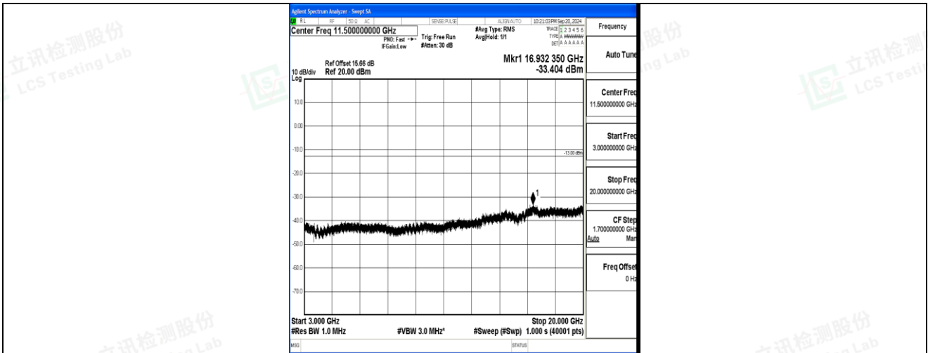
Band2_15MHz_16QAM_18900_1RB#0_3000~20000_3000~20000
