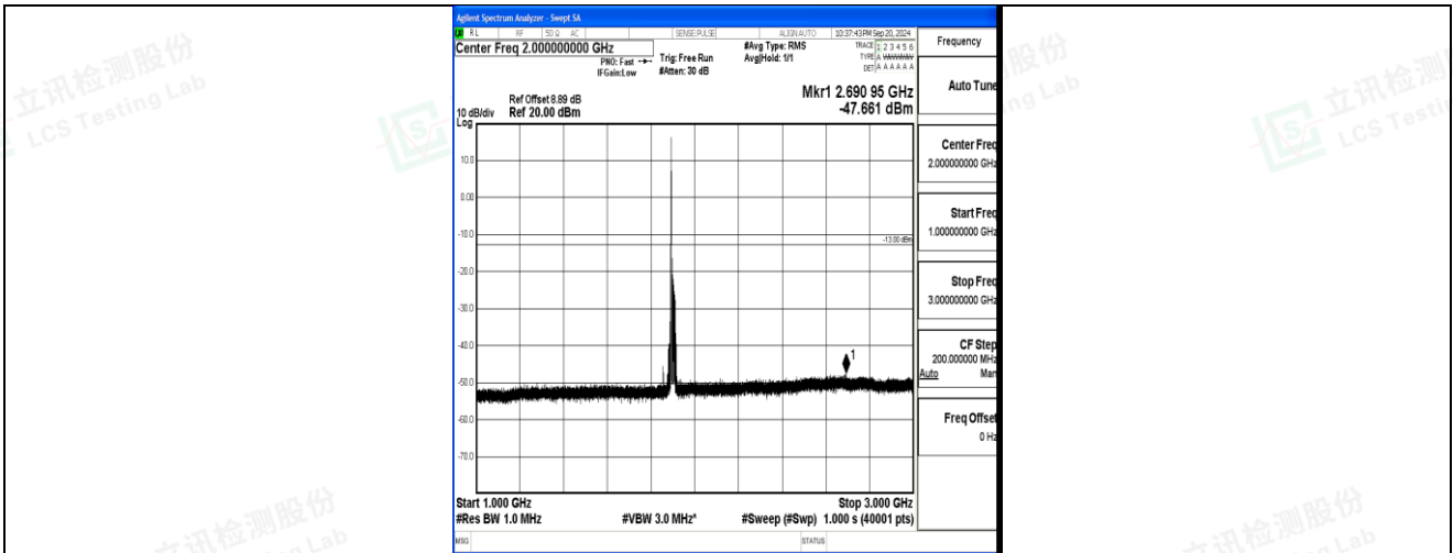
Band2_20MHz_16QAM_19100_1RB#0_1000~3000_1000~3000
