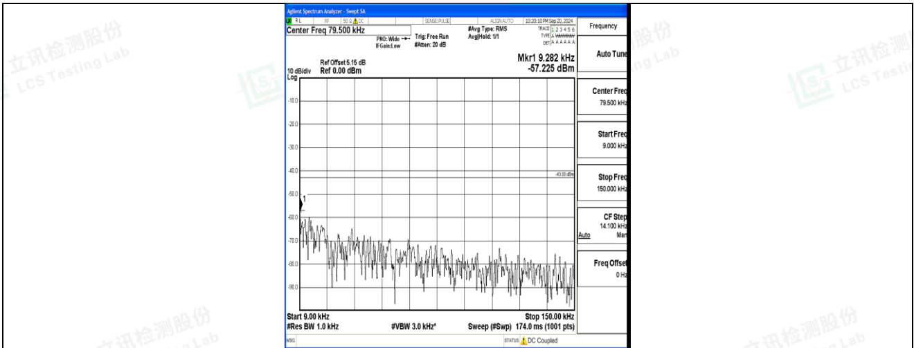
Band2_15MHz_QPSK_18900_1RB#0_0.009~0.15_0.009~0.15
