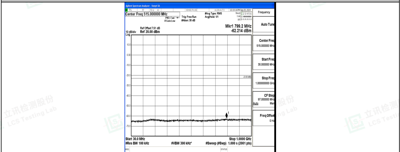
Band2_15MHz_QPSK_18675_1RB#0_30~1000_30~1000
