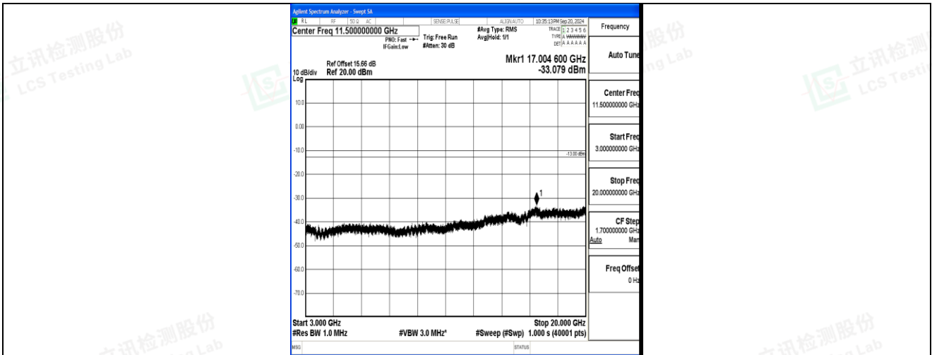
Band2_20MHz_QPSK_18700_1RB#0_3000~20000_3000~20000
