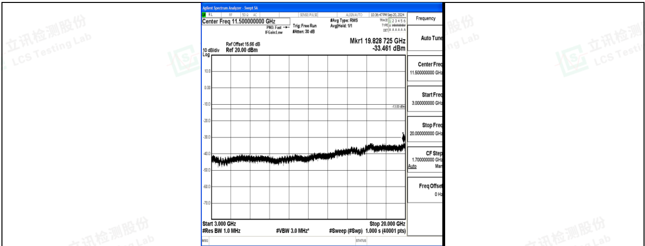
Band2_20MHz_16QAM_18900_1RB#0_3000~20000_3000~20000
