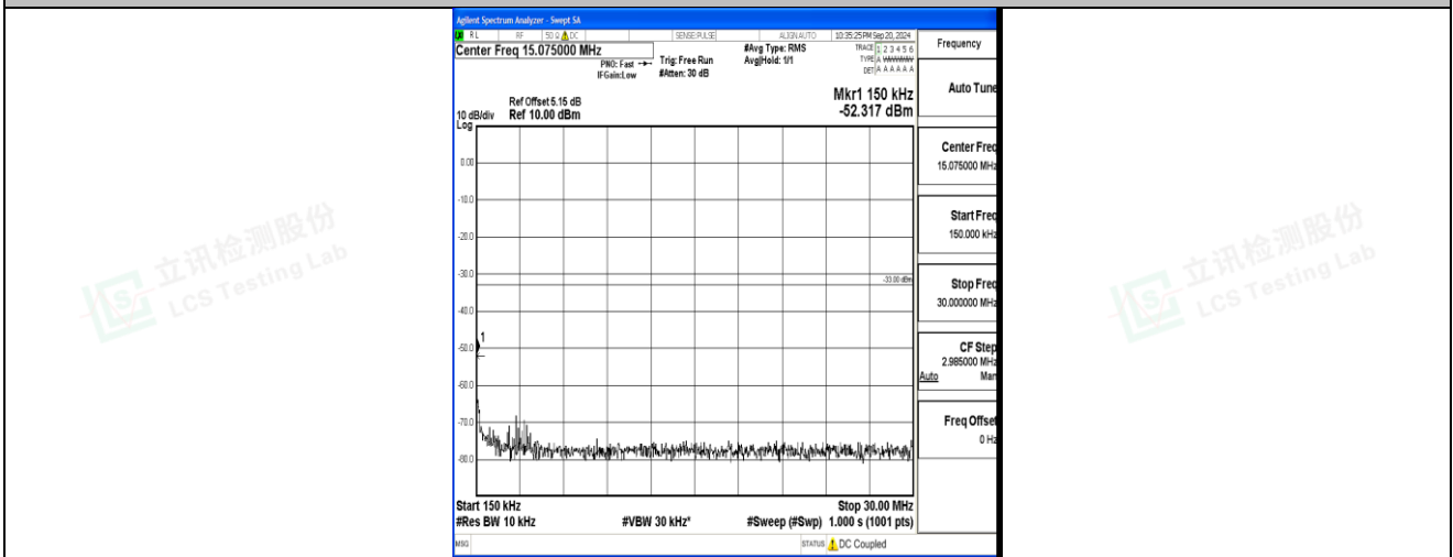
Band2_20MHz_16QAM_18700_1RB#0_0.15~30_0.15~30
