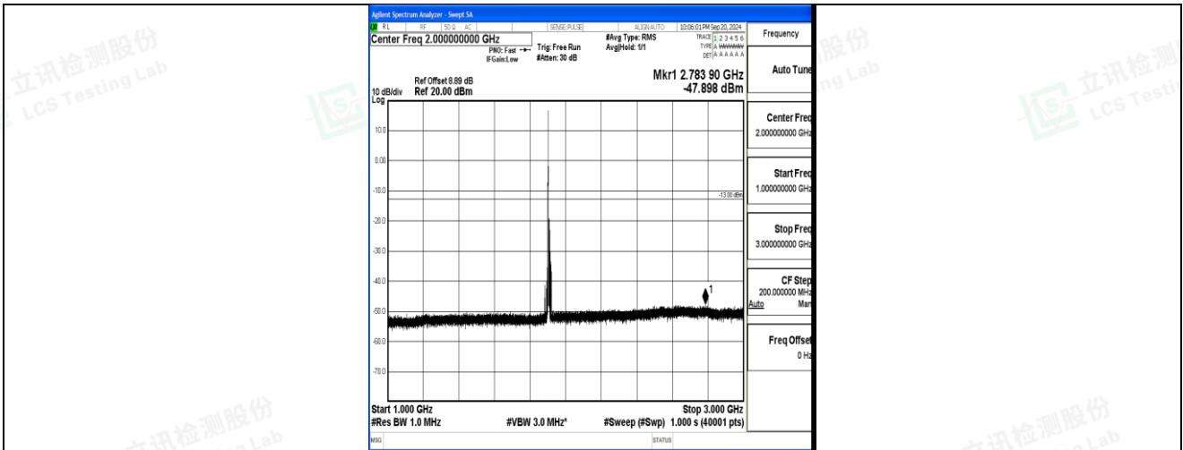
Band2_10MHz_16QAM_19150_1RB#0_1000~3000_1000~3000
