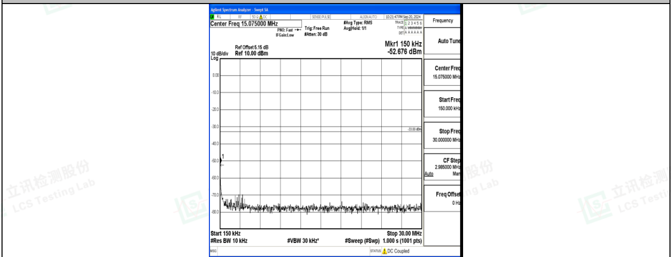
Band2_15MHz_16QAM_19125_1RB#0_0.15~30_0.15~30
