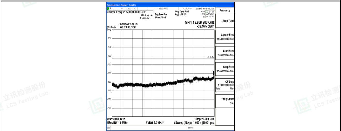
Band2_10MHz_16QAM_19150_1RB#0_3000~20000_3000~20000
