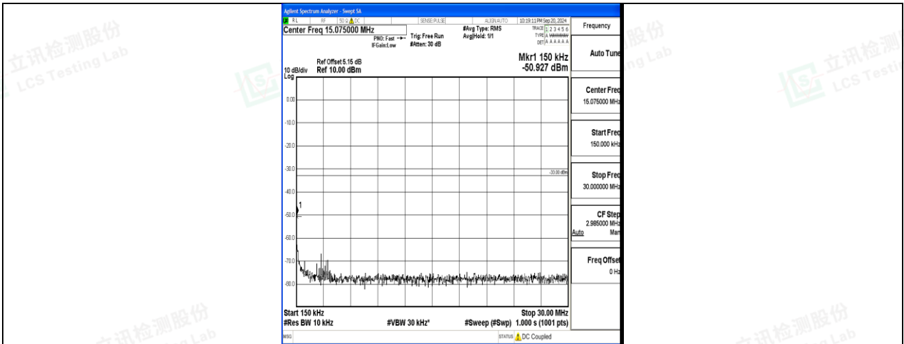
Band2_15MHz_QPSK_18675_1RB#0_0.15~30_0.15~30
