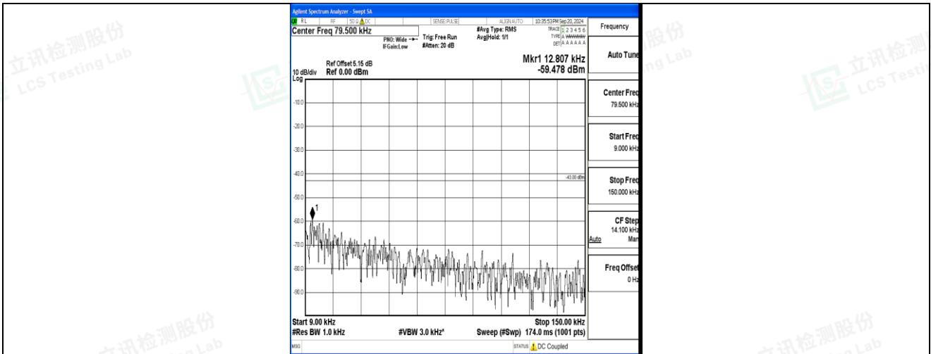
Band2_20MHz_QPSK_18900_1RB#0_0.009~0.15_0.009~0.15
