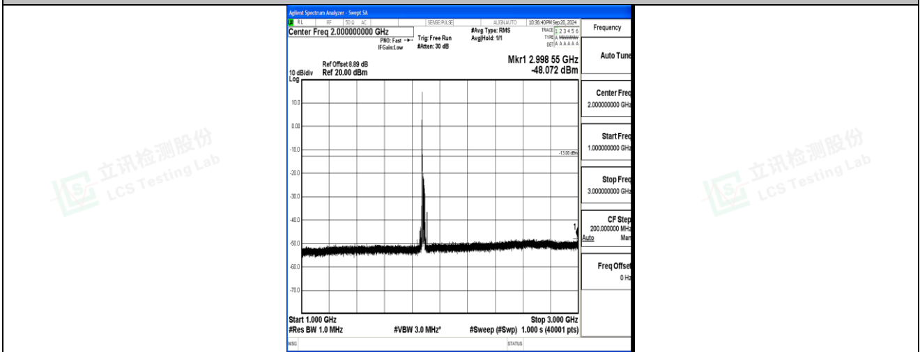
Band2_20MHz_16QAM_18900_1RB#0_1000~3000_1000~3000
