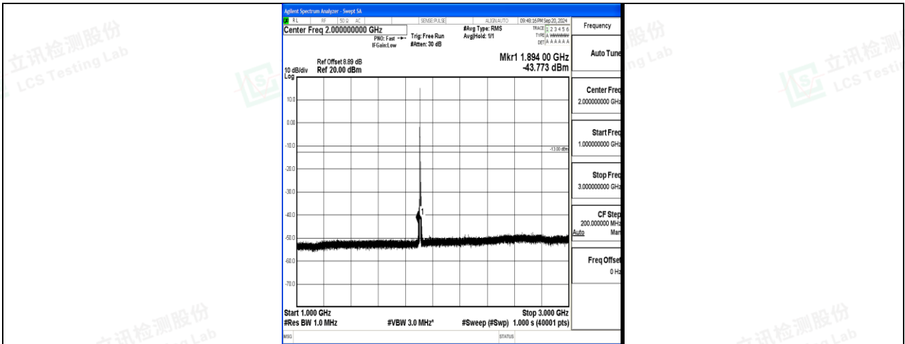
Band2_5MHz_16QAM_19175_1RB#0_1000~3000_1000~3000
