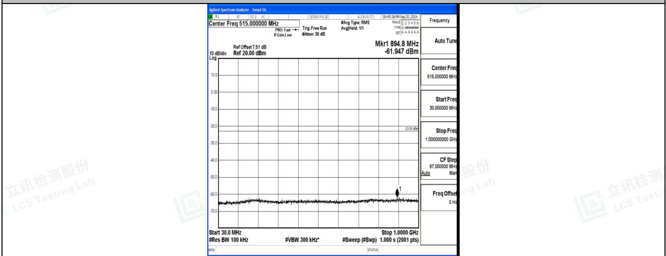
Band2_5MHz_QPSK_18625_1RB#0_30~1000_30~1000
