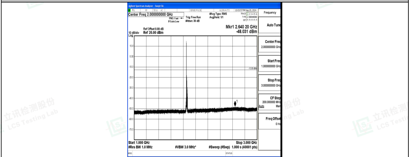
Band2_10MHz_16QAM_18650_1RB#0_1000~3000_1000~3000
