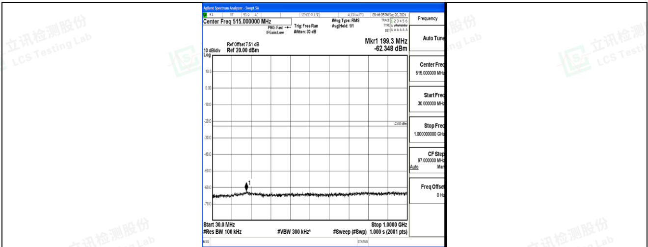
Band2_5MHz_16QAM_18625_1RB#0_30~1000_30~1000
