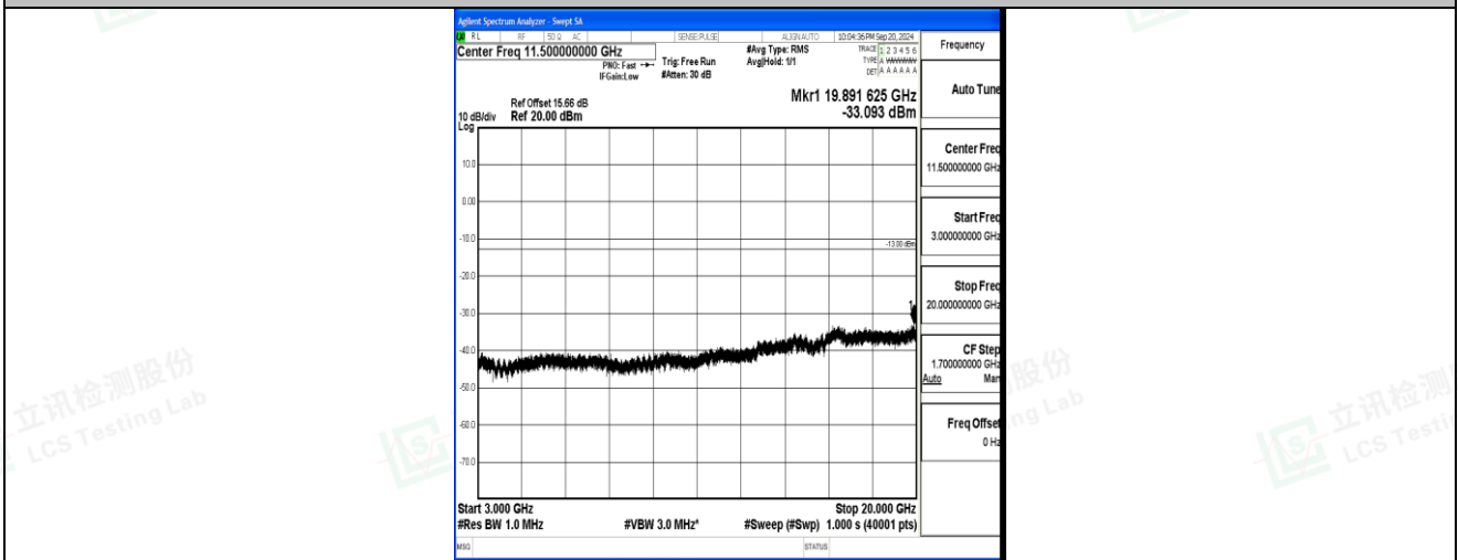
Band2_10MHz_QPSK_18900_1RB#0_3000~20000_3000~20000
