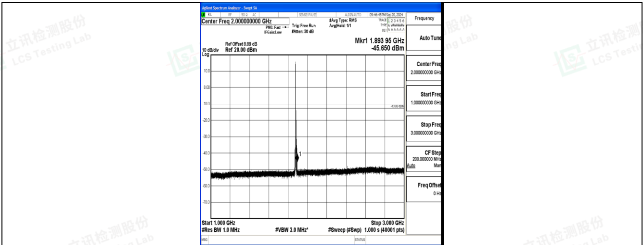
Band2_5MHz_QPSK_18900_1RB#0_1000~3000_1000~3000
