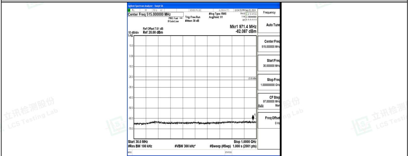
Band2_10MHz_16QAM_18900_1RB#0_30~1000_30~1000
