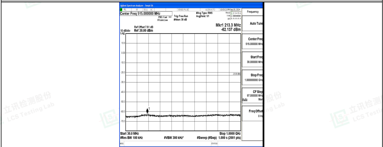
Band2_10MHz_QPSK_18650_1RB#0_30~1000_30~1000
