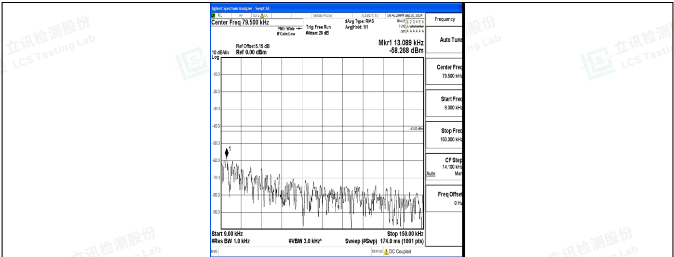
Band2_5MHz_QPSK_18900_1RB#0_0.009~0.15_0.009~0.15
