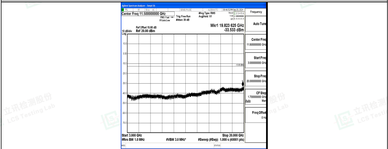
Band2_5MHz_QPSK_18900_1RB#0_3000~20000_3000~20000
