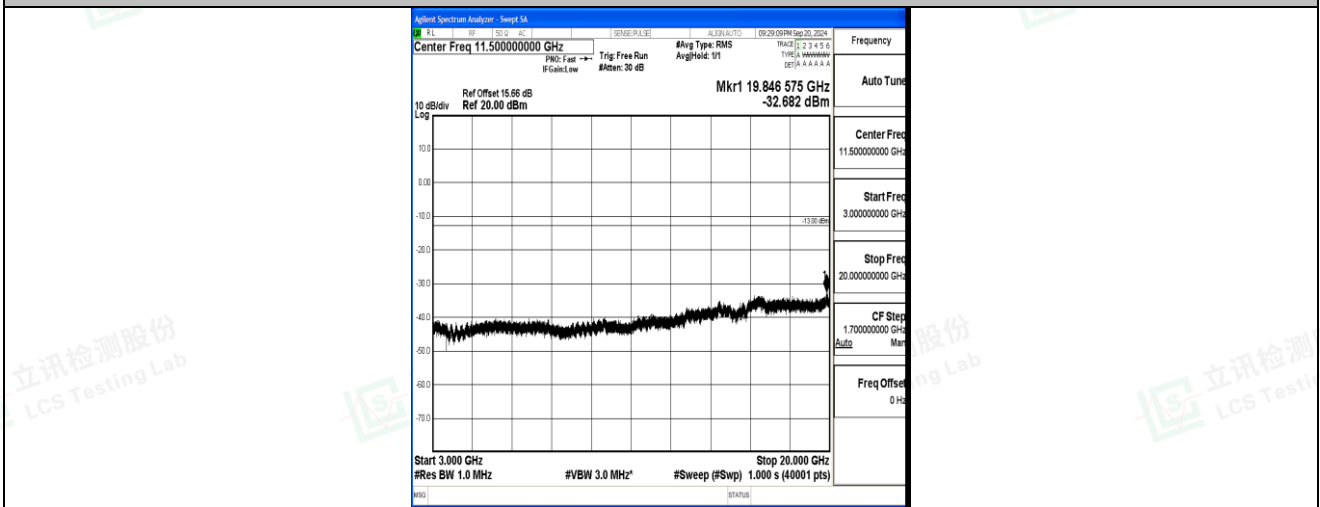
Band2_3MHz_QPSK_18900_1RB#0_3000~20000_3000~20000
