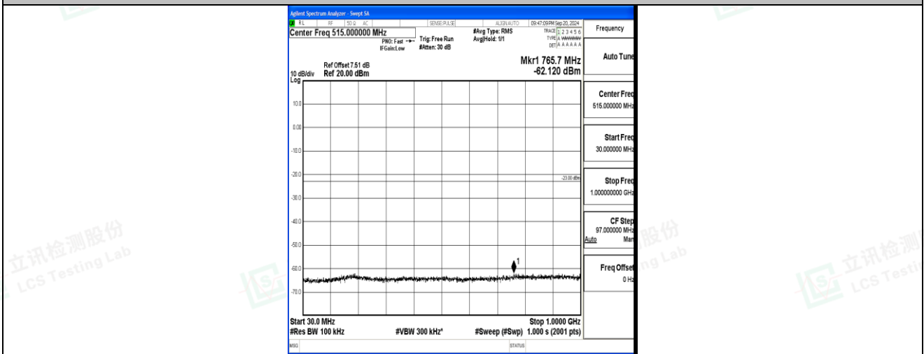
Band2_5MHz_16QAM_18900_1RB#0_30~1000_30~1000
