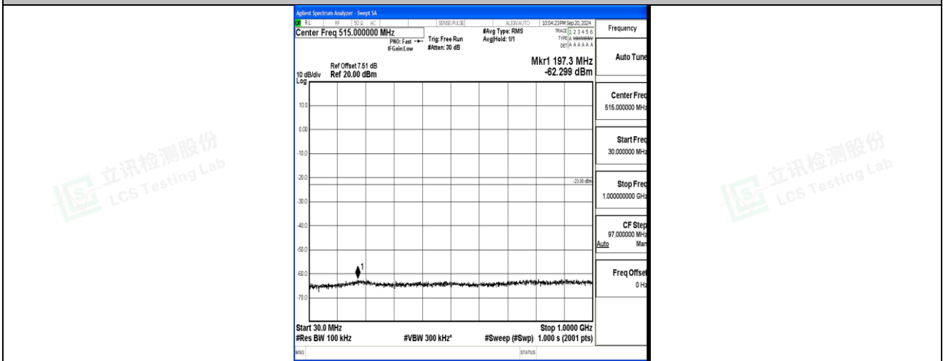
Band2_10MHz_QPSK_18900_1RB#0_30~1000_30~1000
