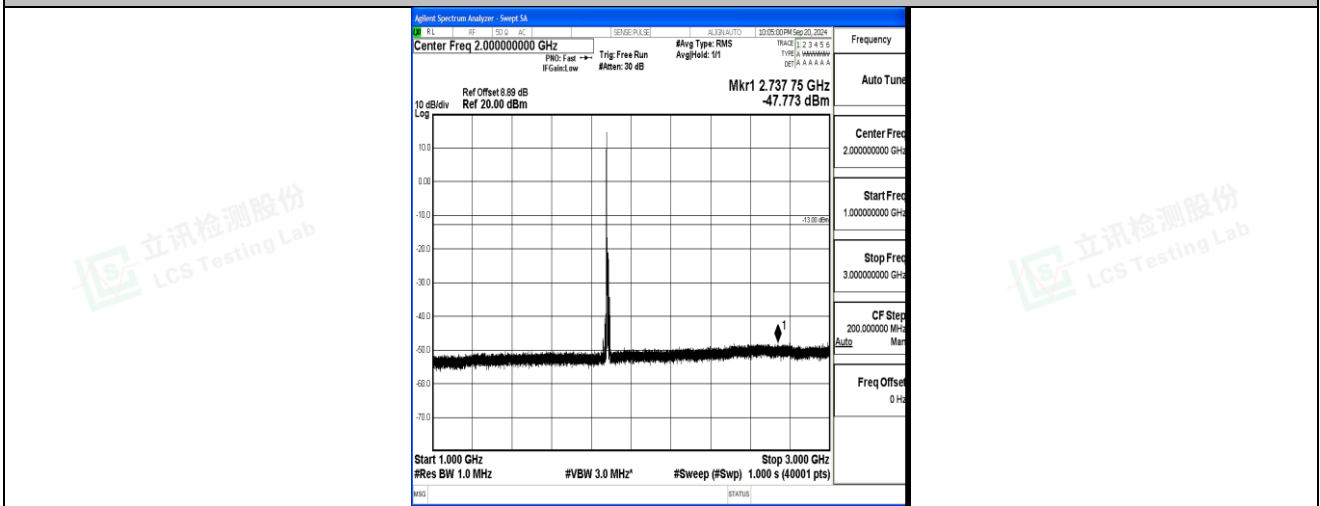
Band2_10MHz_16QAM_18900_1RB#0_1000~3000_1000~3000
