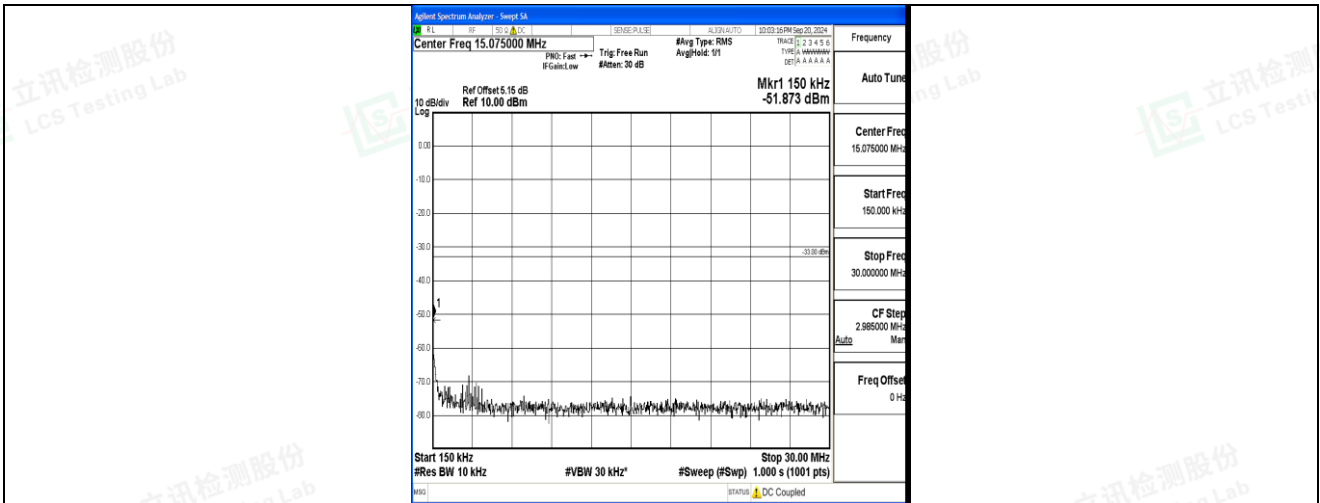
Band2_10MHz_QPSK_18650_1RB#0_0.15~30_0.15~30
