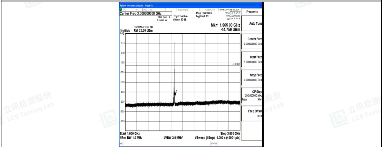
Band2_5MHz_16QAM_18625_1RB#0_1000~3000_1000~3000
