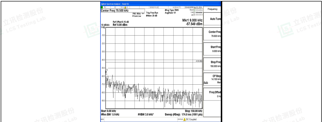
Band2_5MHz_16QAM_19175_1RB#0_0.009~0.15_0.009~0.15
