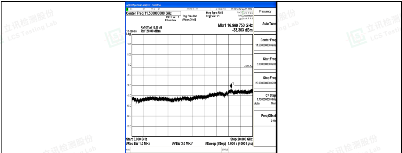
Band2_10MHz_QPSK_18650_1RB#0_3000~20000_3000~20000
