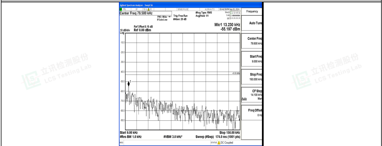
Band2_5MHz_16QAM_18900_1RB#0_0.009~0.15_0.009~0.15
