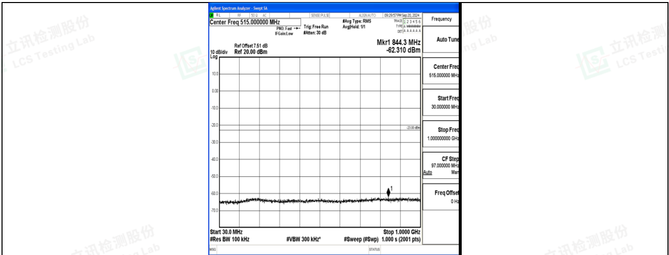
Band2_3MHz_QPSK_19185_1RB#0_30~100_30~1000
