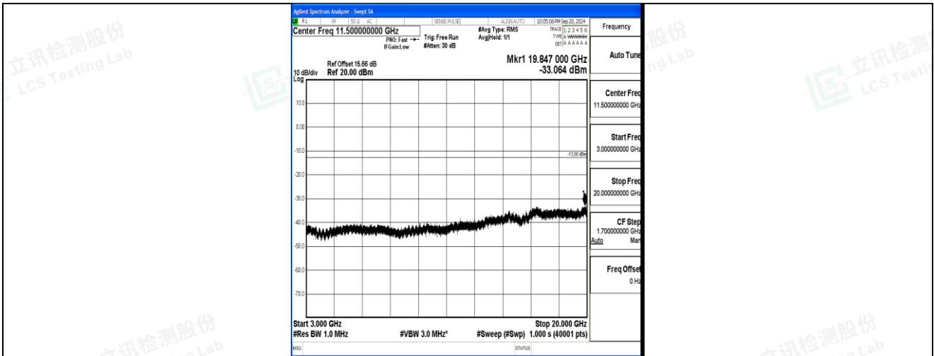
Band2_10MHz_16QAM_18900_1RB#0_3000~20000_3000~20000
