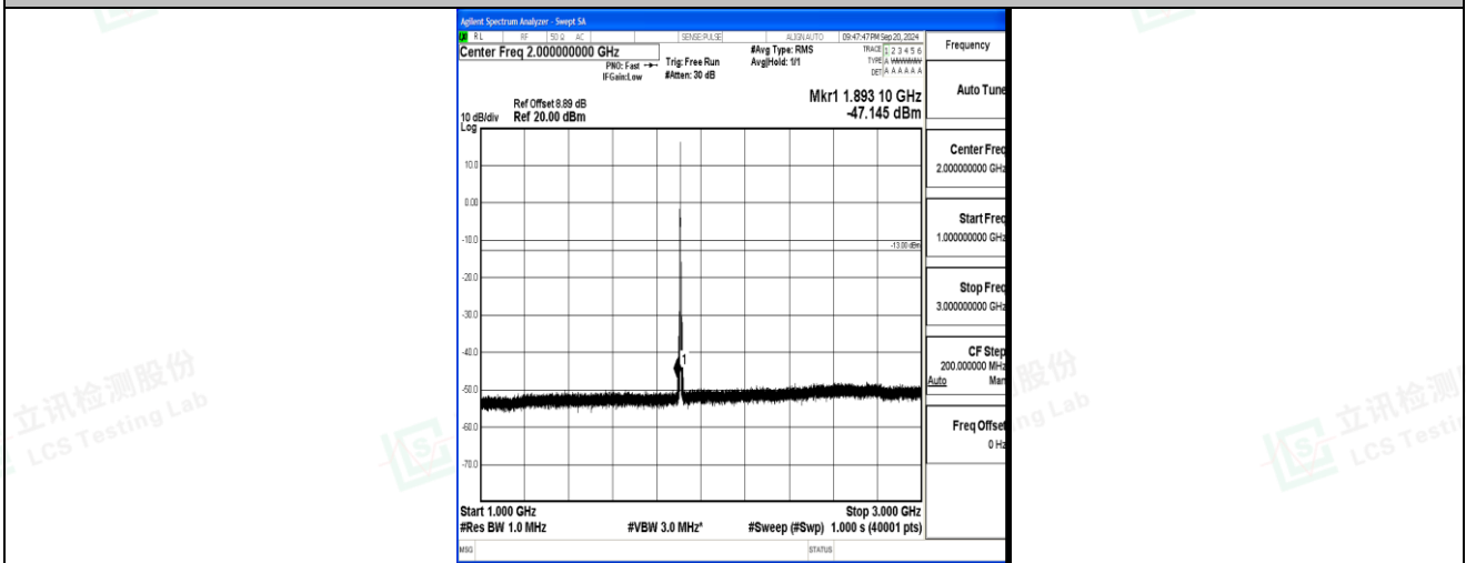
Band2_5MHz_QPSK_19175_1RB#0_1000~3000_1000~3000
