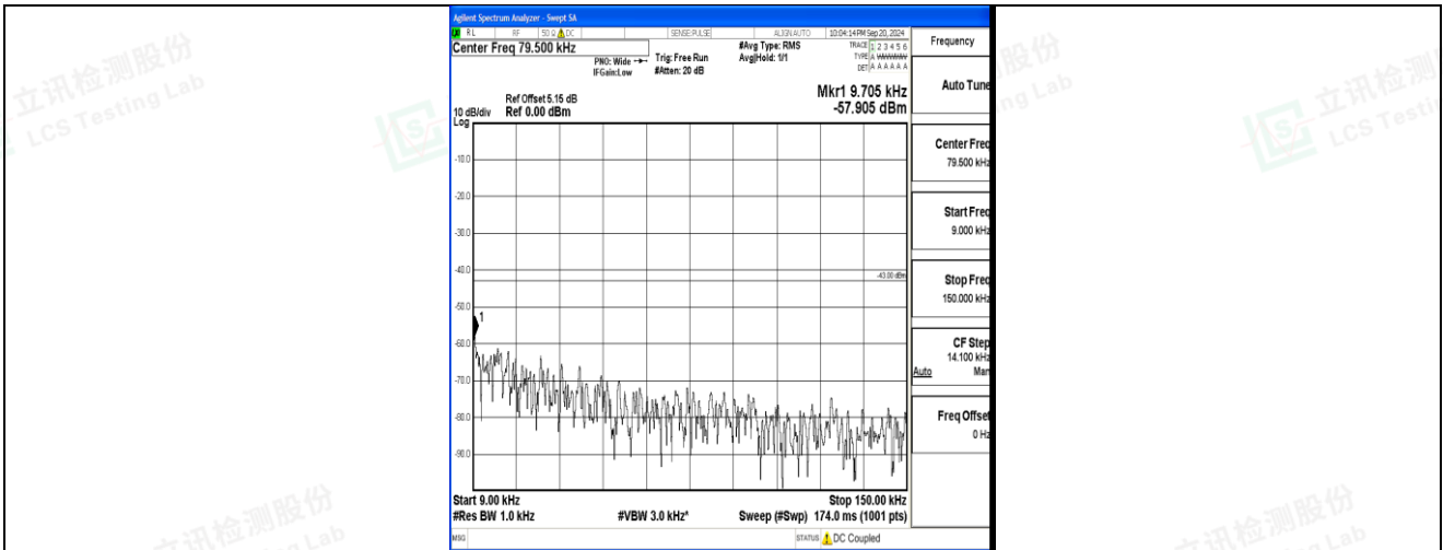
Band2_10MHz_QPSK_18900_1RB#0_0.009~0.15_0.009~0.15
