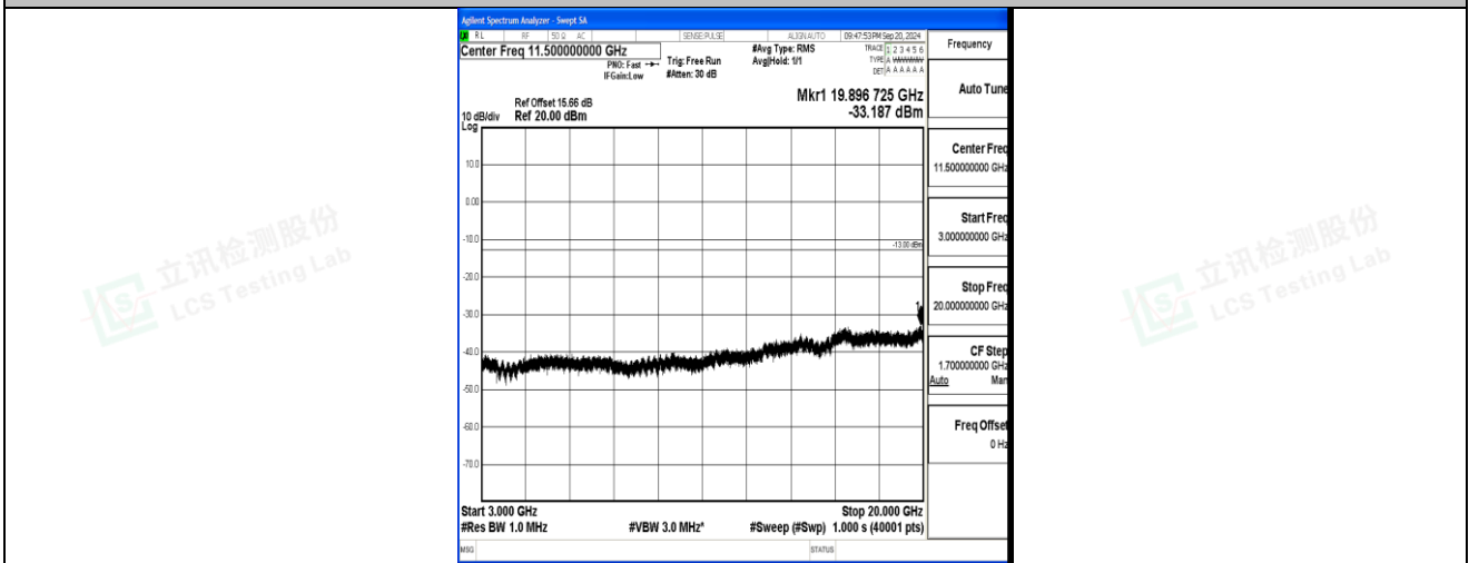
Band2_5MHz_QPSK_19175_1RB#0_3000~20000_3000~20000
