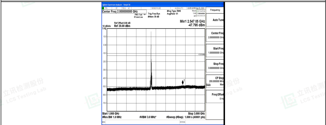
Band2_10MHz_QPSK_19150_1RB#0_1000~3000_1000~3000
