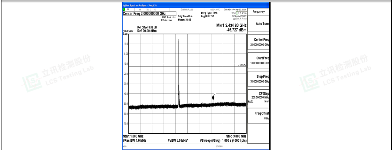
Band2_5MHz_QPSK_18625_1RB#0_1000~3000_1000~3000
