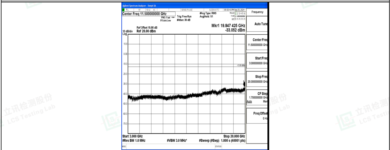
Band2_3MHz_16QAM_19185_1RB#0_3000~20000_3000~20000
