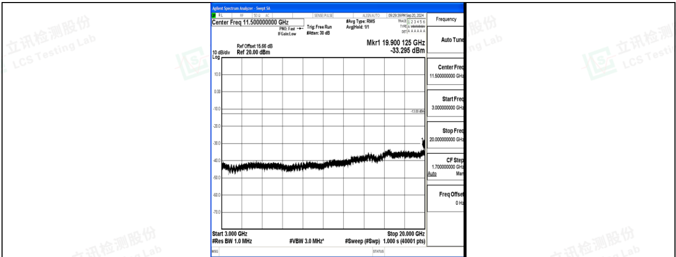
Band2_3MHz_16QAM_18900_1RB#0_3000~20000_3000~20000
