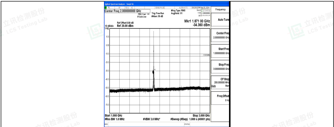
Band2_3MHz_QPSK_18900_1RB#0_1000~3000_1000~3000
