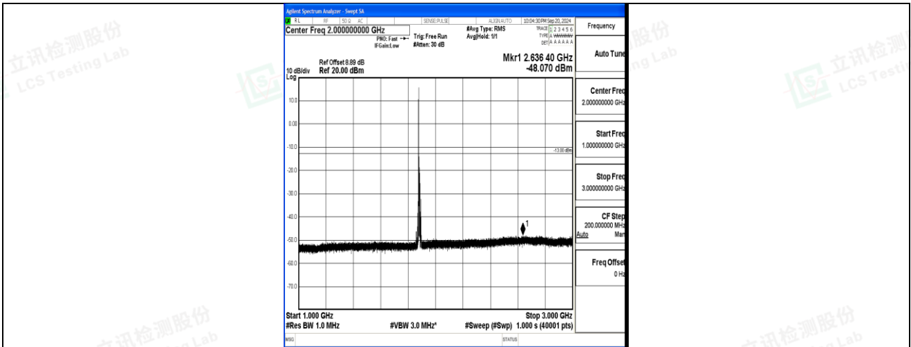
Band2_10MHz_QPSK_18900_1RB#0_1000~3000_1000~3000
