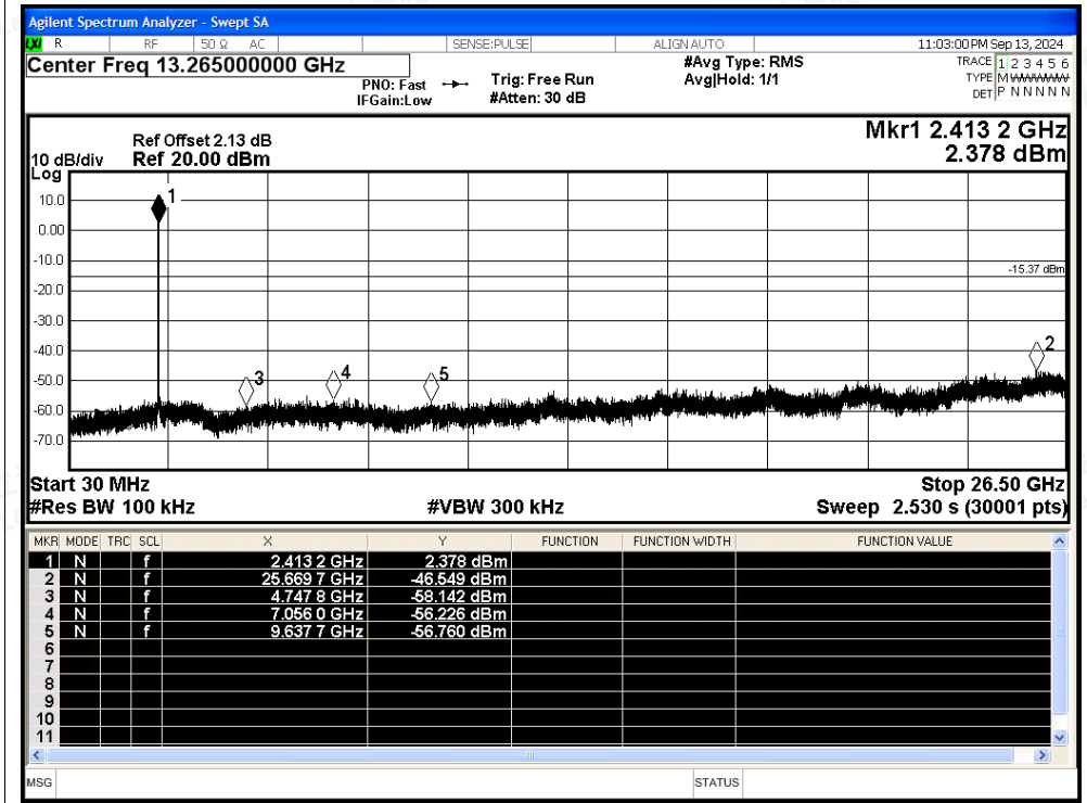
Tx. Spurious NVNT b 2412MHz Ant Emission
