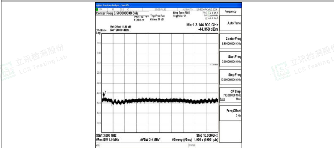
Band26_5MHz_16QAM_27015_1RB#0_3000~10000_3000~10000
