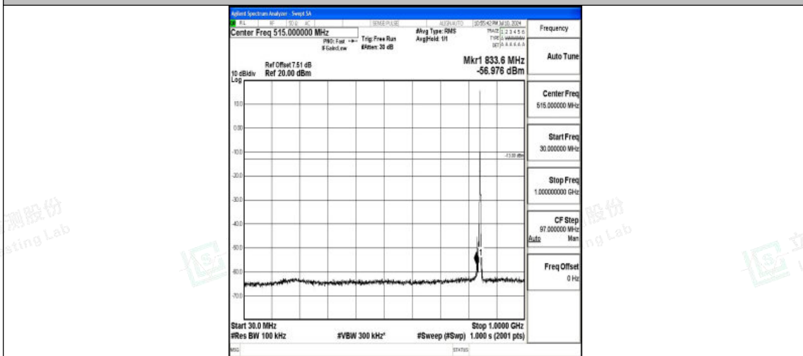
Band26_5MHz_QPSK_27015_1RB#0_30~1000_30~1000
