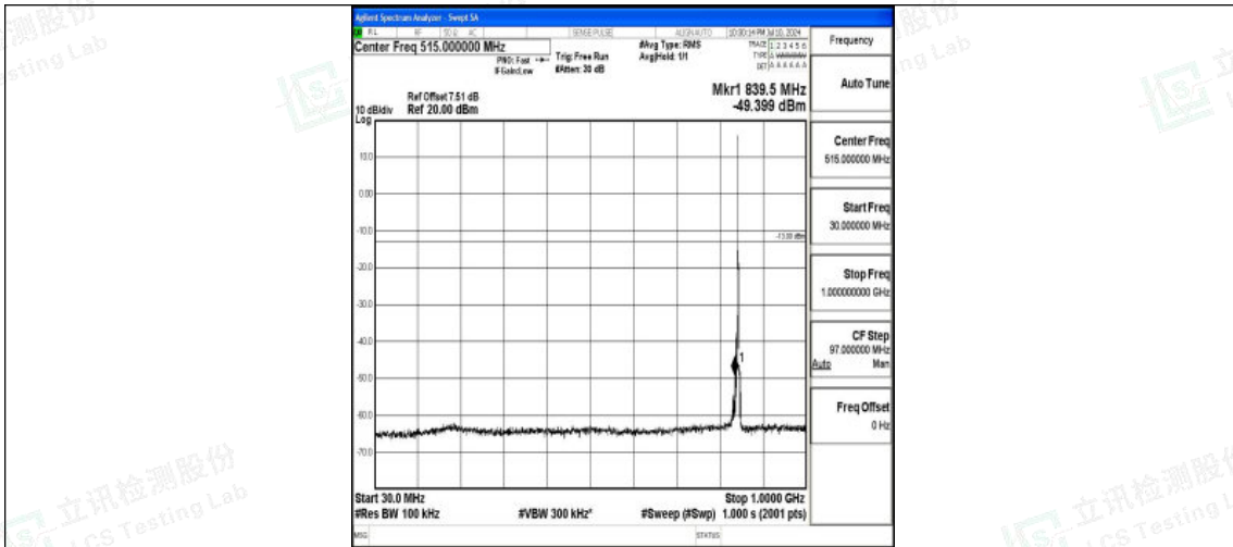
Band26_3MHz_16QAM_27025_1RB#0_30~1000_30~1000
