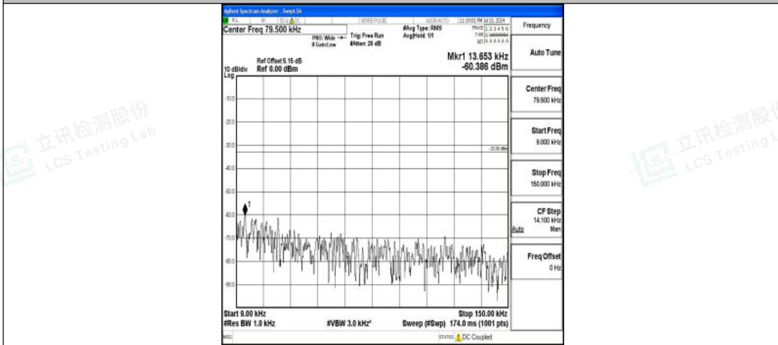
Band26_10MHz_16QAM_26840_1RB#0_0.009~0.15_0.009~0.15
