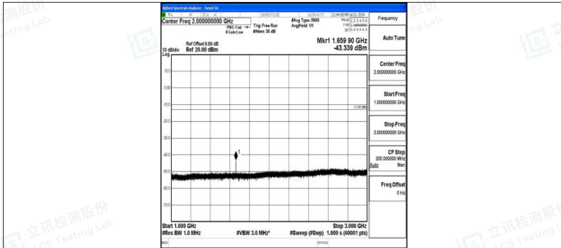
Band26_15MHz_16QAM_26915_1RB#0_1000~3000_1000~3000
