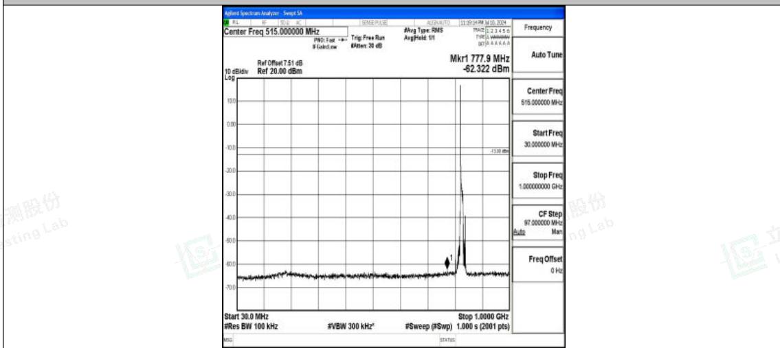
Band26_10MHz_16QAM_26840_1RB#0_30~1000_30~1000
