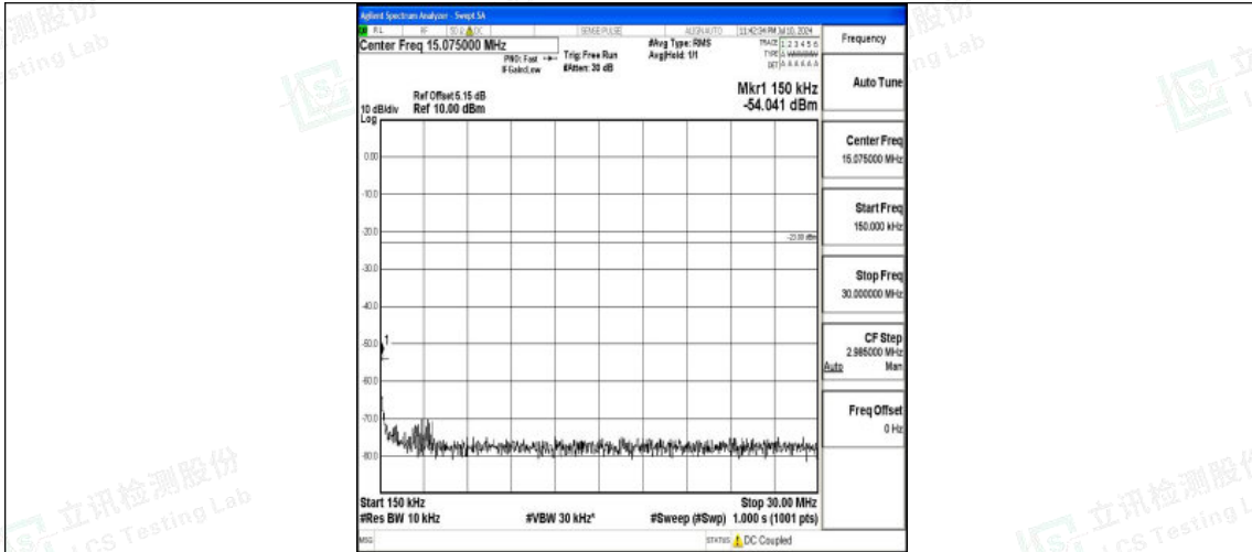
Band26_15MHz_16QAM_26865_1RB#0_0.15~30_0.15~30
