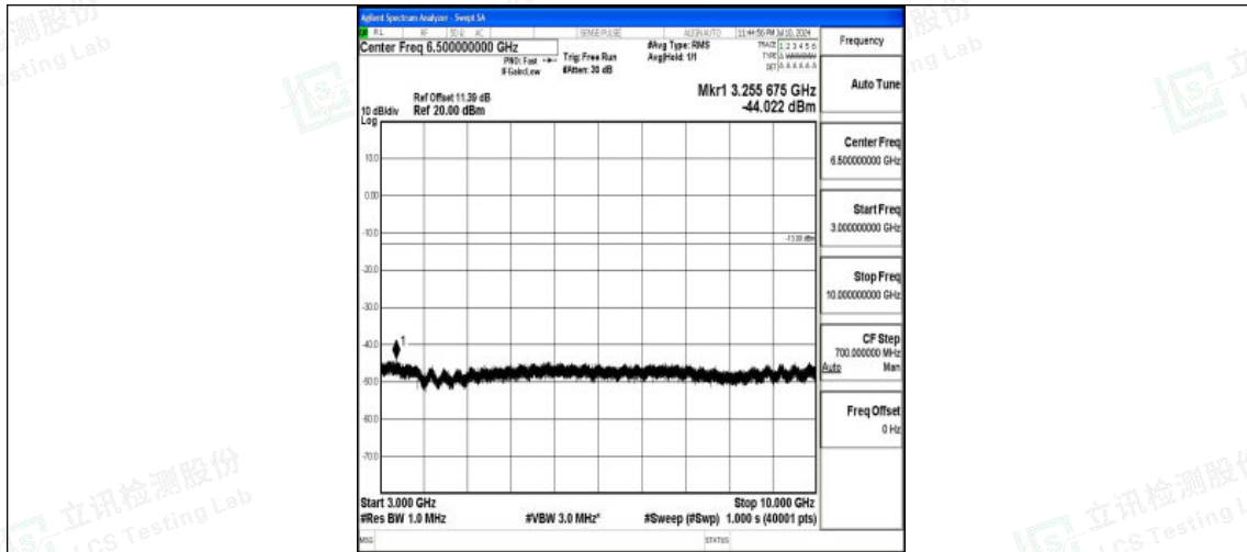
Band26_15MHz_QPSK_26965_1RB#0_3000~10000_3000~10000
