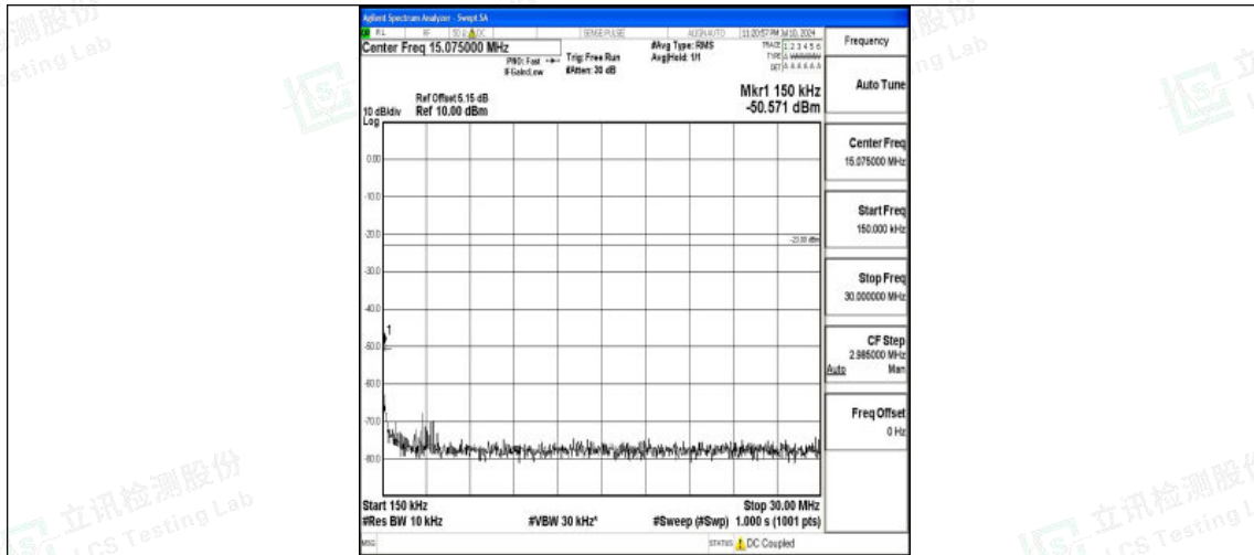
Band26_10MHz_QPSK_26990_1RB#0_0.15~30_0.15~30
