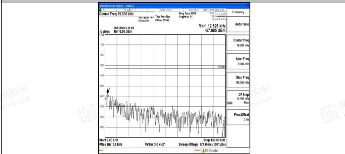
Band26_10MHz_16QAM_26990_1RB#0_0.009~0.15_0.009~0.15
