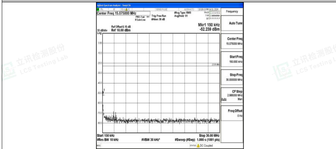
Band26_3MHz_QPSK_26915_1RB#0_0.15~30_0.15~30
