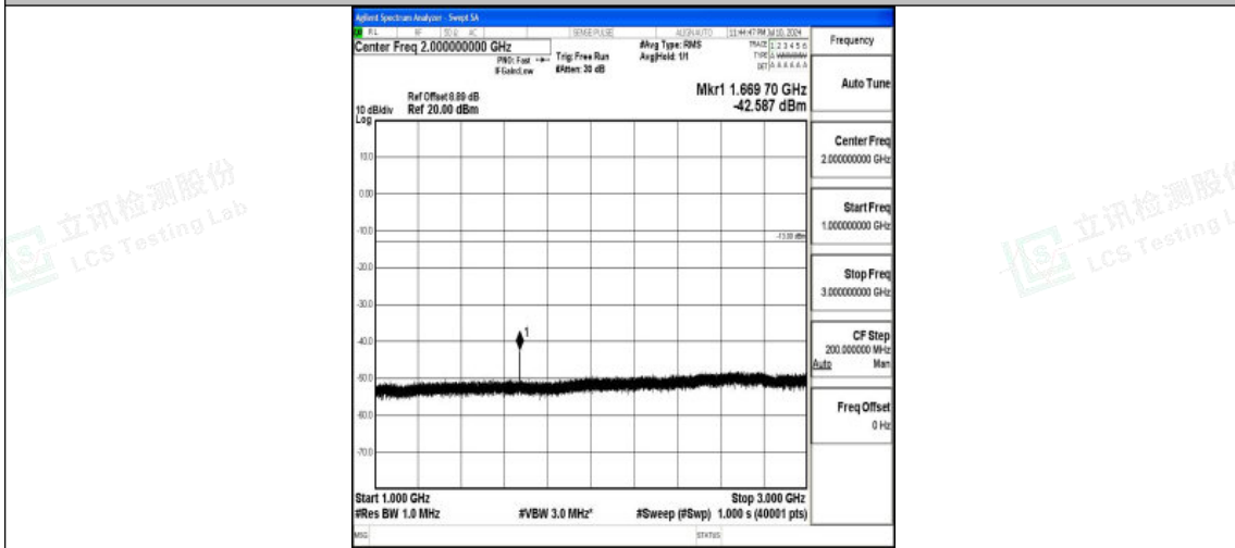
Band26_15MHz_QPSK_26965_1RB#0_1000~3000_1000~3000
