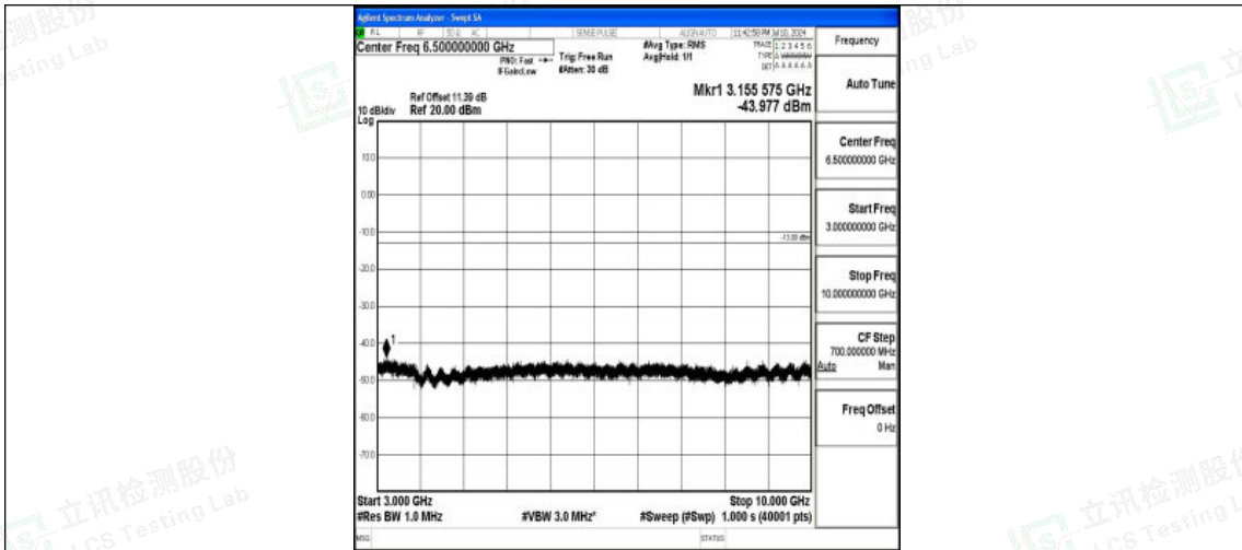
Band26_15MHz_16QAM_26865_1RB#0_3000~10000_3000~10000
