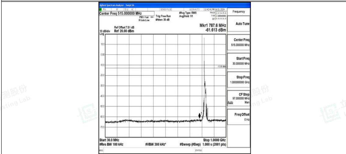
Band26_15MHz_16QAM_26865_1RB#0_30~1000_30~1000
