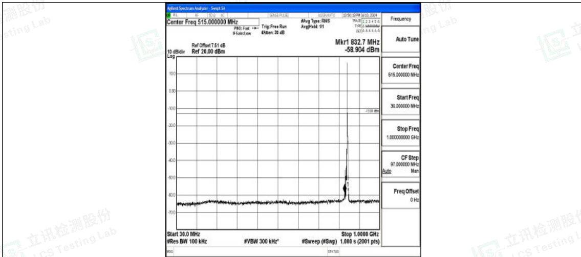
Band26_5MHz_16QAM_27015_1RB#0_30~1000_30~1000
