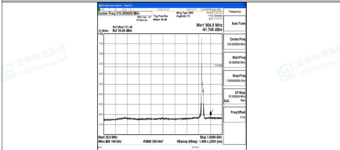
Band26_15MHz_16QAM_26915_1RB#0_30~1000_30~1000
