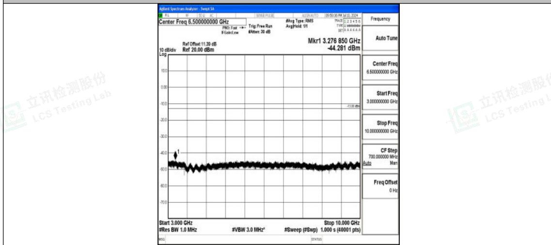
Band26_1.4MHz_16QAM_27033_1RB#0_3000~10000_3000~10000
