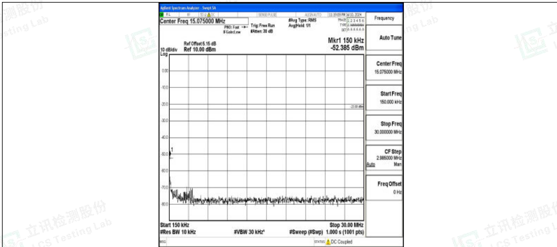
Band26_10MHz_16QAM_26840_1RB#0_0.15~30_0.15~30
