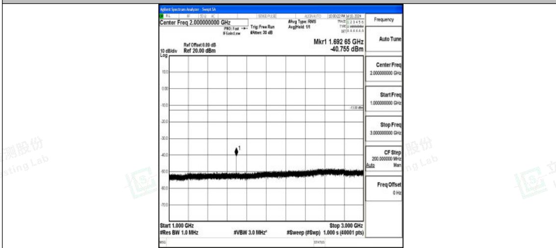
Band26_3MHz_16QAM_27025_1RB#0_1000~3000_1000~3000
