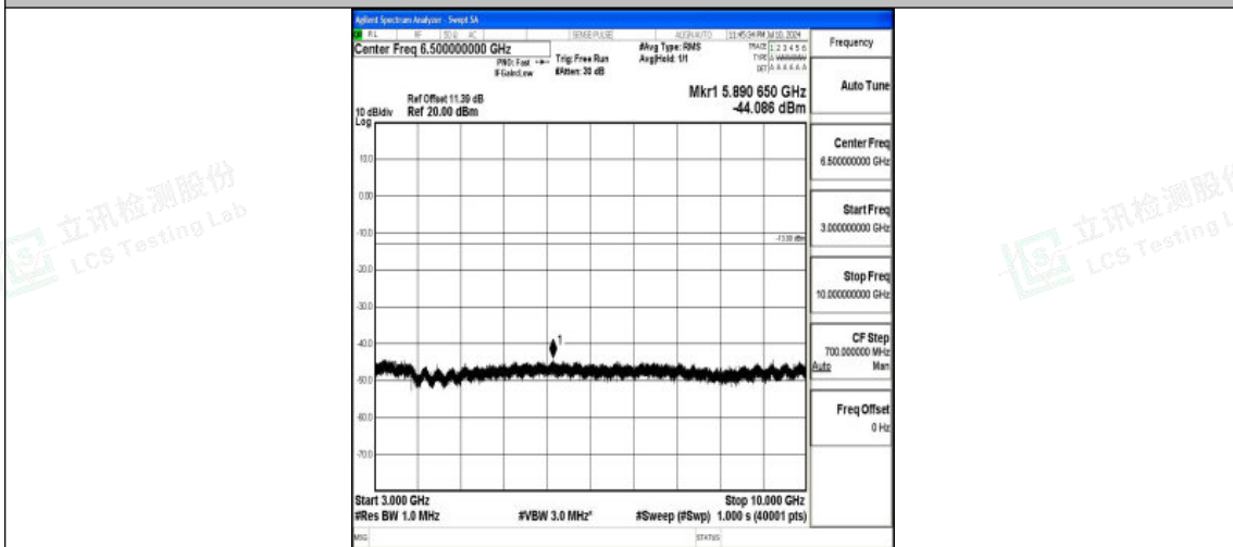
Band26_15MHz_16QAM_26965_1RB#0_3000~10000_3000~10000
