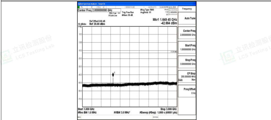
Band26_15MHz_16QAM_26865_1RB#0_1000~3000_1000~3000
