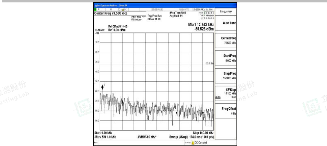
Band26_3MHz_QPSK_26915_1RB#0_0.009~0.15_0.009~0.15
