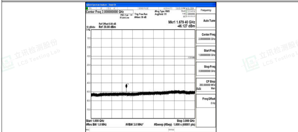
Band26_10MHz_QPSK_26990_1RB#0_1000~3000_1000~3000
