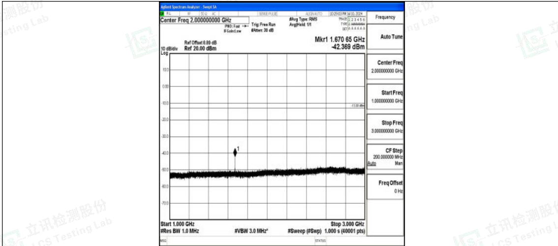
Band26_3MHz_16QAM_26915_1RB#0_1000~3000_1000~3000
