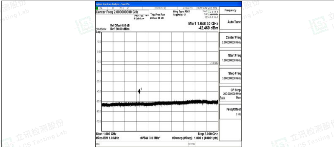
Band26_3MHz_QPSK_26805_1RB#0_1000~3000_1000~3000
