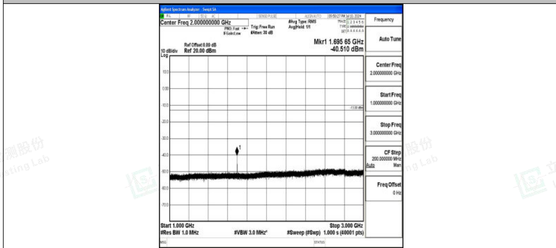
Band26_1.4MHz_16QAM_27033_1RB#0_1000~3000_1000~3000
