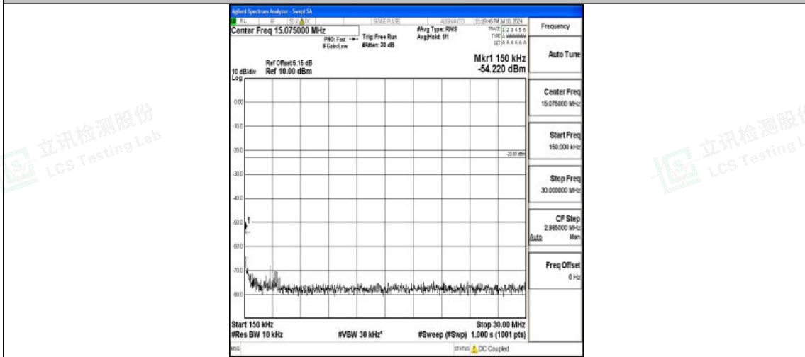
Band26_10MHz_QPSK_26915_1RB#0_0.15~30_0.15~30
