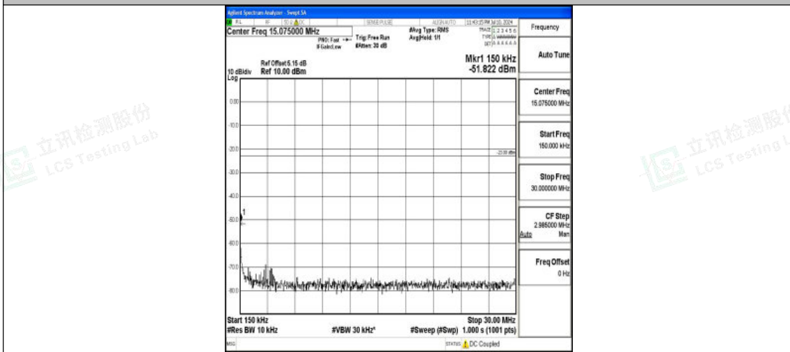
Band26_15MHz_QPSK_26915_1RB#0_0.15~30_0.15~30
