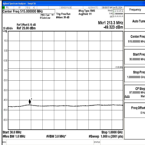
30 MHz - 1000 MHz
