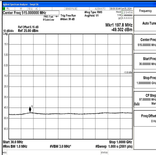
30 MHz - 1000 MHz
