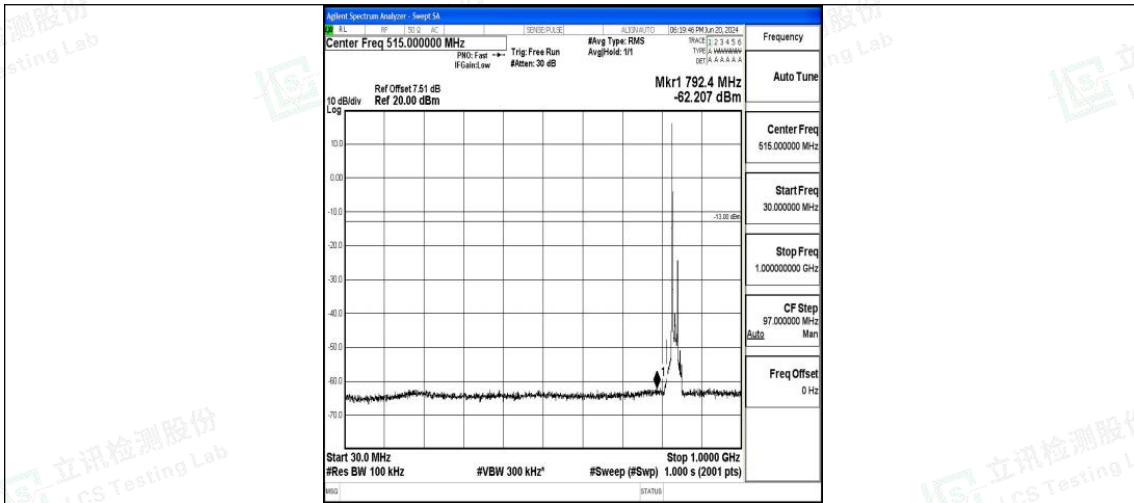
Band26_15MHz_QPSK_26915_1RB#0_30~1000_30~1000
