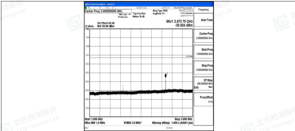
Band26_10MHz_QPSK_26840_1RB#0_1000~3000_1000~3000
