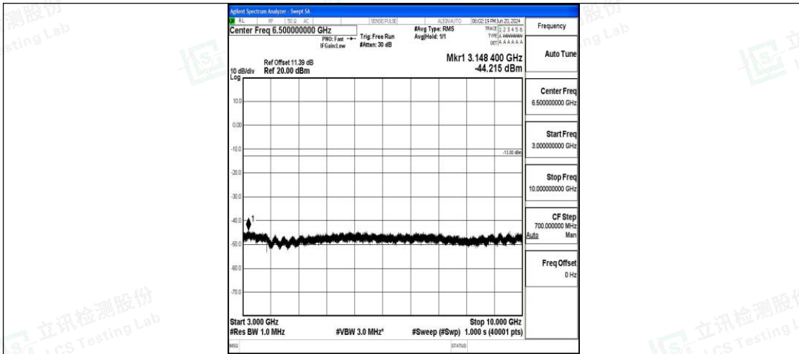
Band26_10MHz_QPSK_26990_1RB#0_3000~10000_3000~10000
