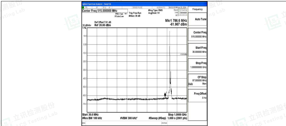
Band26_10MHz_QPSK_26915_1RB#0_30~1000_30~1000
