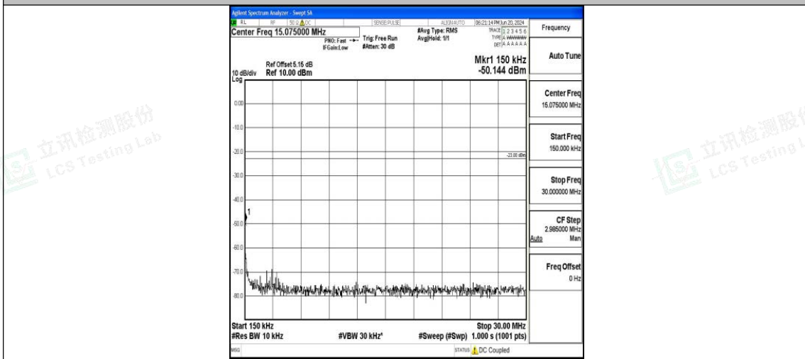
Band26_15MHz_16QAM_26965_1RB#0_0.15~30_0.15~30
