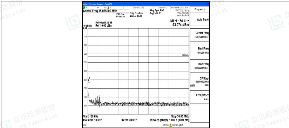
Band26_15MHz_QPSK_26965_1RB#0_0.15~30_0.15~30
