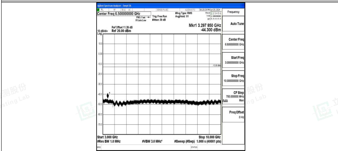
Band26_15MHz_16QAM_26915_1RB#0_3000~10000_3000~10000
