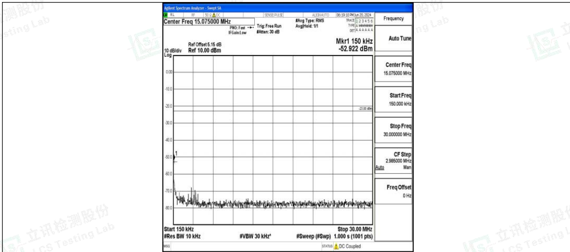
Band26_15MHz_16QAM_26865_1RB#0_0.15~30_0.15~30
