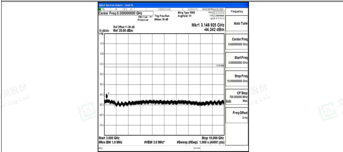
Band26_3MHz_QPSK_26740_1RB#0_3000~10000_3000~10000
