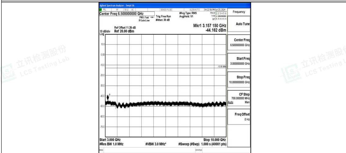
Band26_5MHz_16QAM_26715_1RB#0_3000~10000_3000~10000
