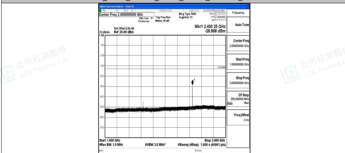
Band26_5MHz_16QAM_26740_1RB#0_1000~3000_1000~3000
