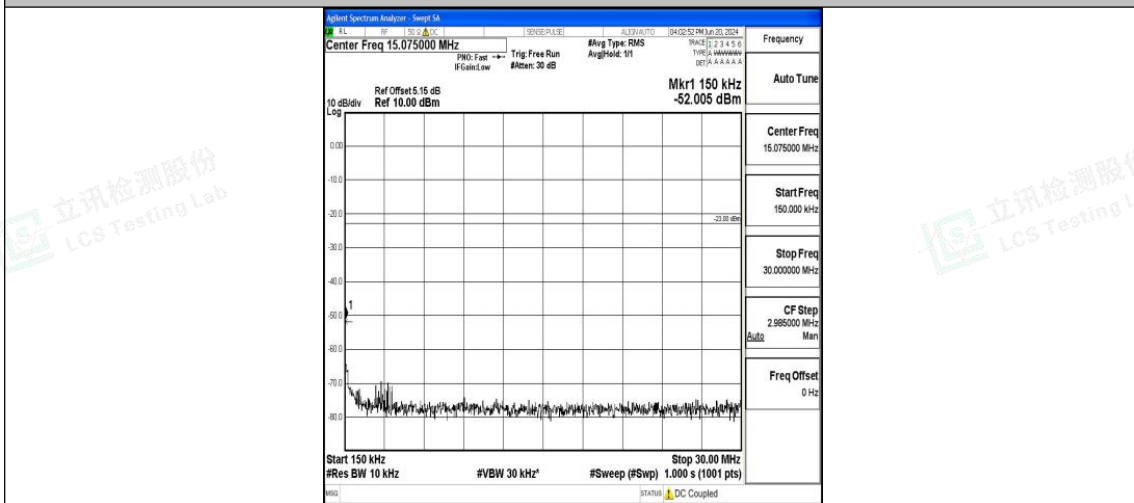
Band26_3MHz_QPSK_26775_1RB#0_0.15~30_0.15~30
