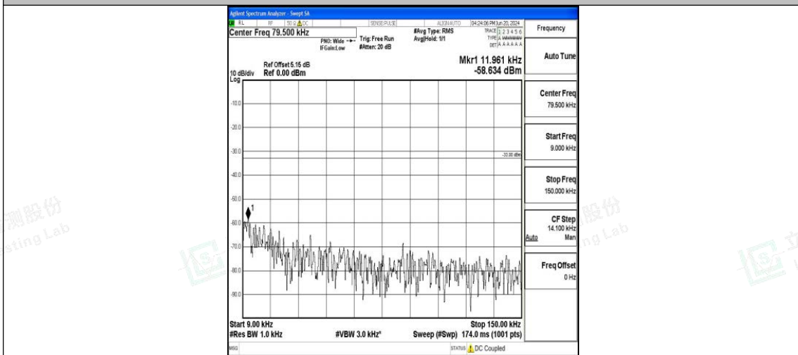
Band26_5MHz_QPSK_26765_1RB#0_0.009~0.15_0.009~0.15
