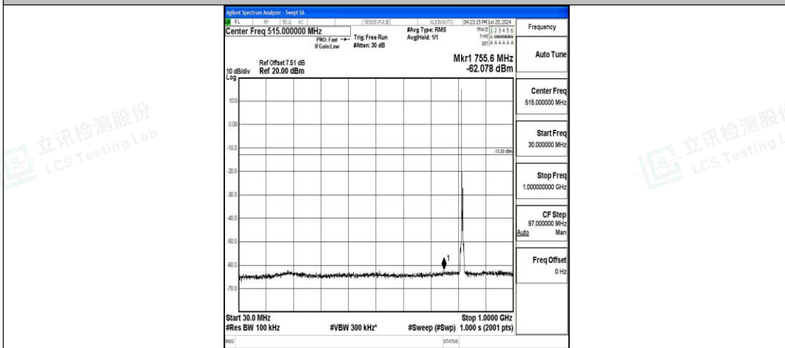
Band26_5MHz_QPSK_26740_1RB#0_30~1000_30~1000
