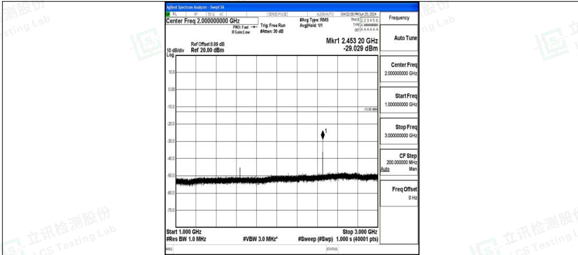
Band26_3MHz_QPSK_26740_1RB#0_1000~3000_1000~3000
