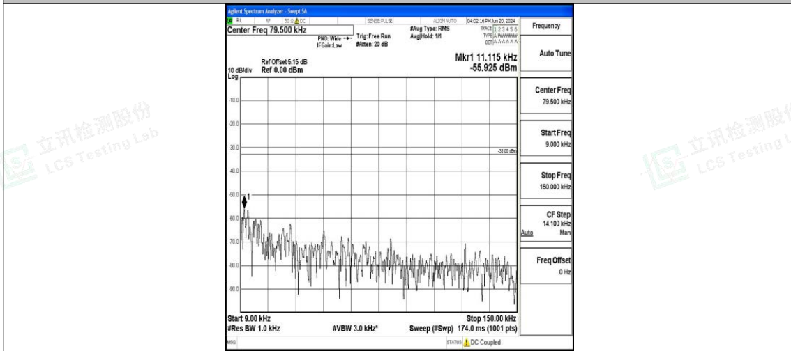
Band26_3MHz_16QAM_26740_1RB#0_0.009~0.15_0.009~0.15
