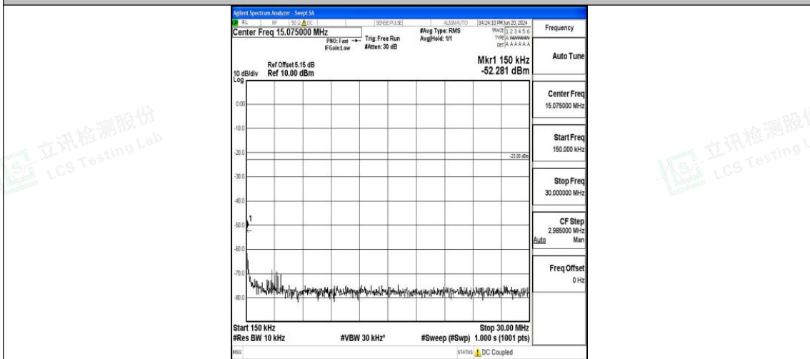
Band26_5MHz_QPSK_26765_1RB#0_0.15~30_0.15~30
