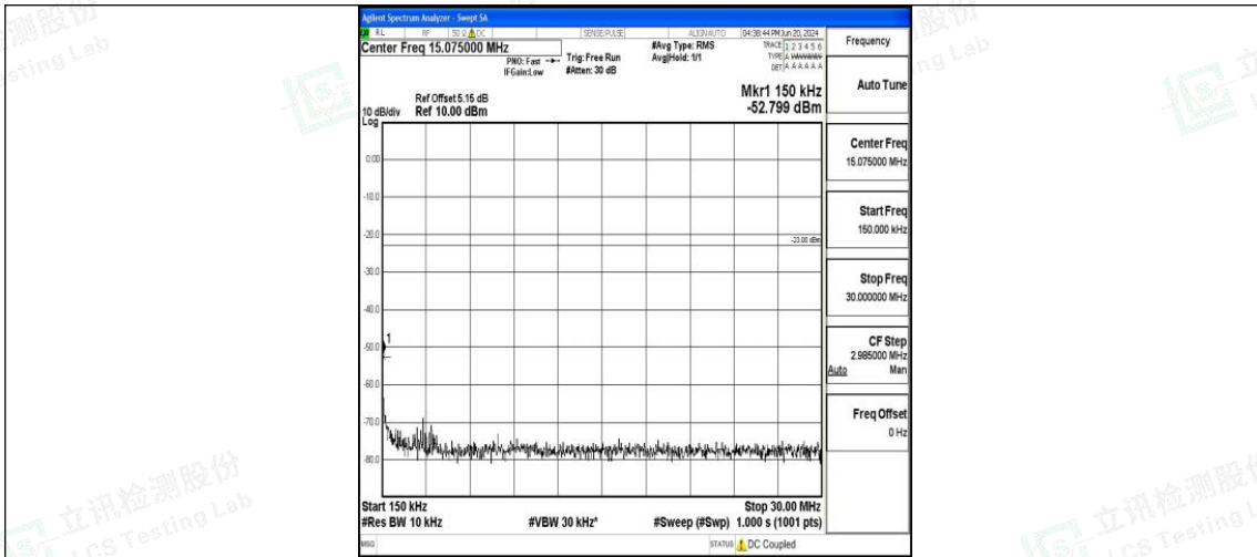
Band26_10MHz_QPSK_26740_1RB#0_0.15~30_0.15~30
