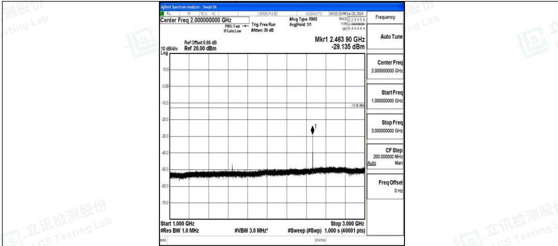
Band26_3MHz_16QAM_26775_1RB#0_1000~3000_1000~3000
