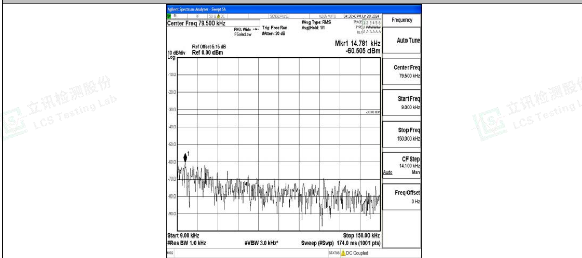
Band26_10MHz_QPSK_26740_1RB#0_0.009~0.15_0.009~0.15
