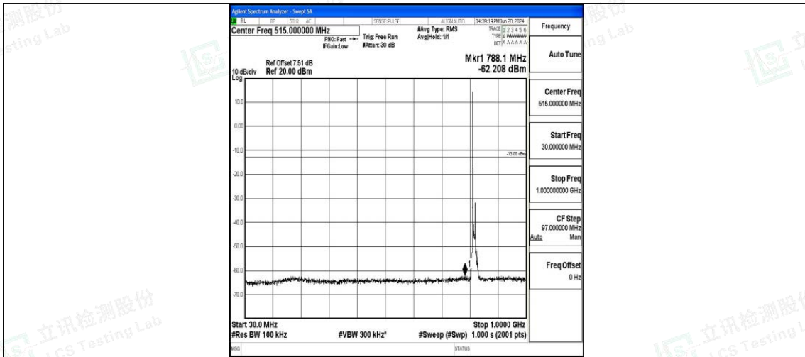
Band26_10MHz_16QAM_26740_1RB#0_30~1000_30~1000
