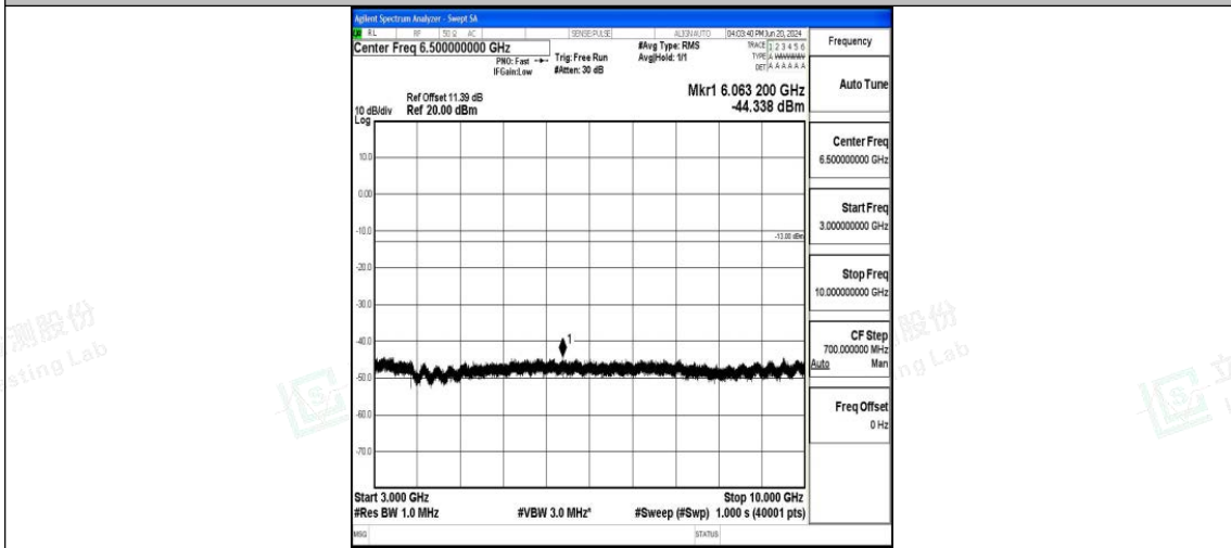
Band26_3MHz_16QAM_26775_1RB#0_3000~10000_3000~10000
