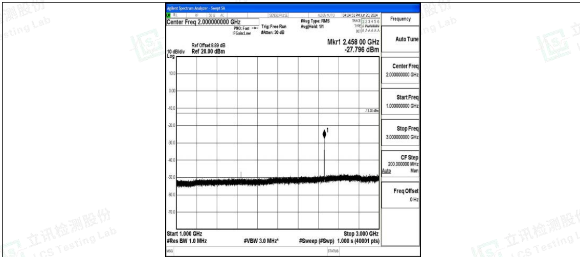
Band26_5MHz_16QAM_26765_1RB#0_1000~3000_1000~3000
