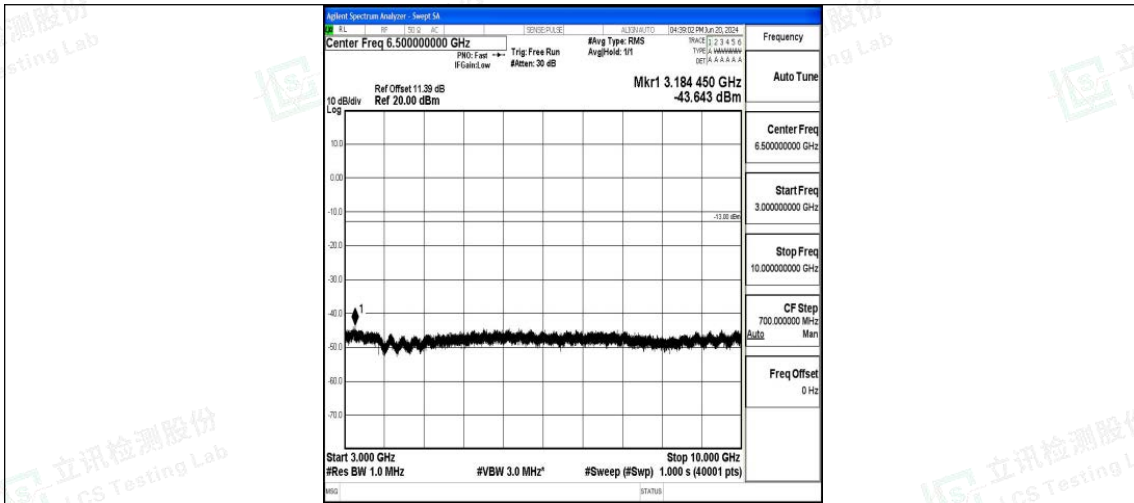
Band26_10MHz_QPSK_26740_1RB#0_3000~10000_3000~10000
