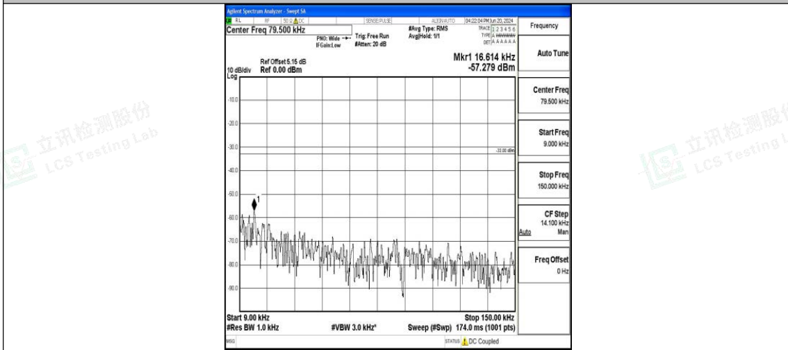
Band26_5MHz_QPSK_26715_1RB#0_0.009~0.15_0.009~0.15
