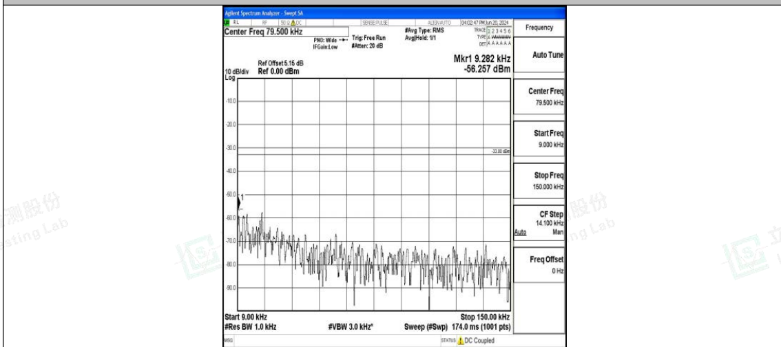
Band26_3MHz_QPSK_26775_1RB#0_0.009~0.15_0.009~0.15
