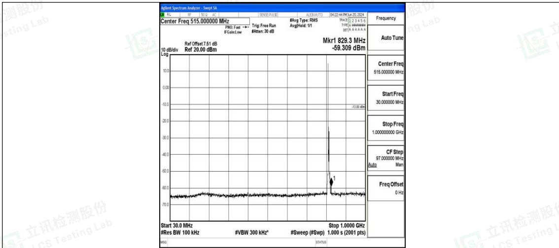
Band26_5MHz_16QAM_26715_1RB#0_30~1000_30~1000
