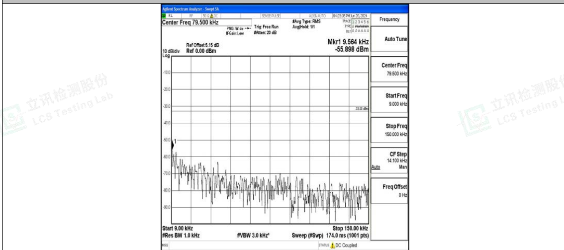
Band26_5MHz_16QAM_26740_1RB#0_0.009~0.15_0.009~0.15
