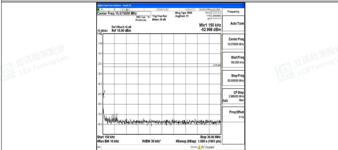
Band26_10MHz_16QAM_26740_1RB#0_0.15~30_0.15~30
