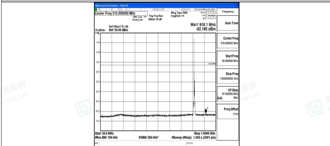
Band26_5MHz_16QAM_26740_1RB#0_30~1000_30~1000
