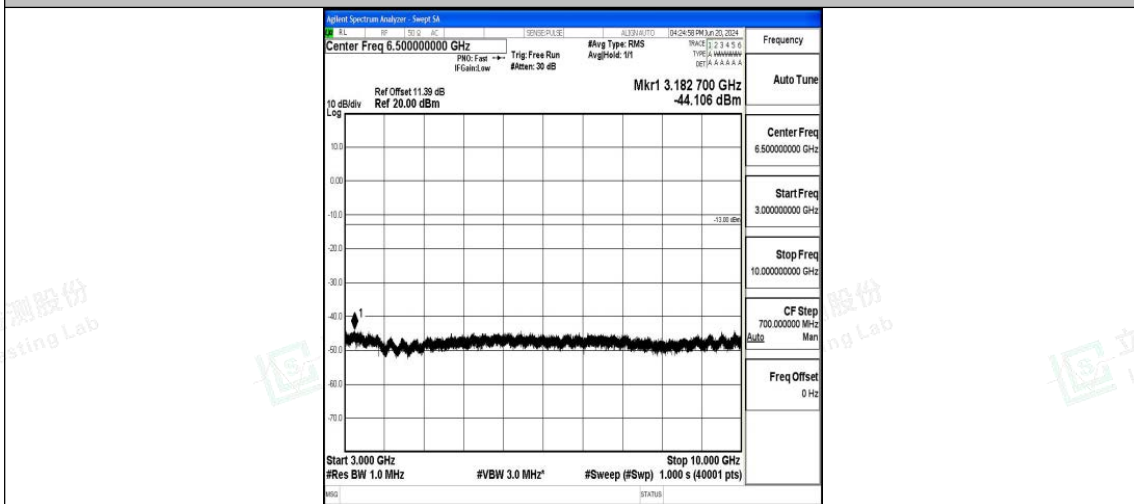
Band26_5MHz_16QAM_26765_1RB#0_3000~10000_3000~10000
