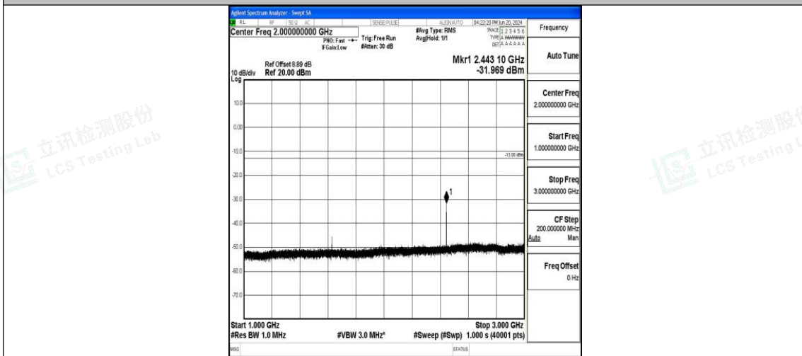
Band26_5MHz_QPSK_26715_1RB#0_1000~3000_1000~3000
