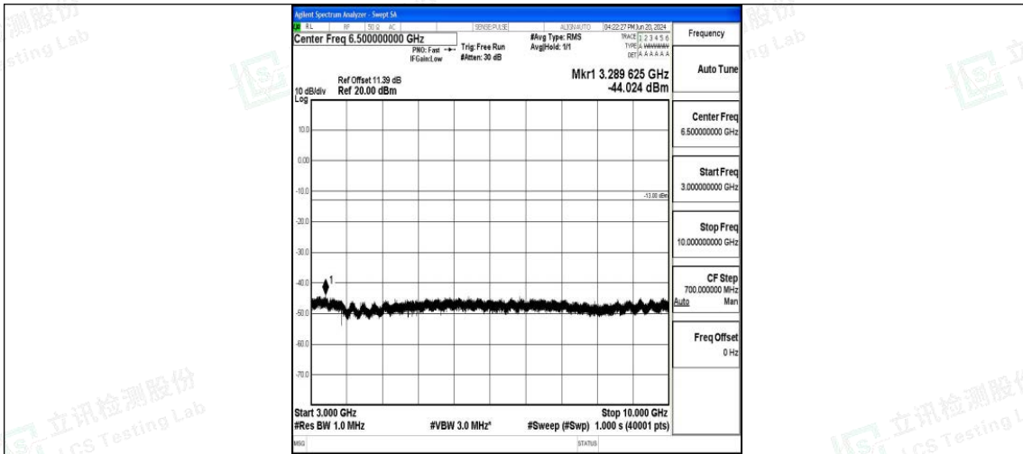
Band26_5MHz_QPSK_26715_1RB#0_3000~10000_3000~10000
