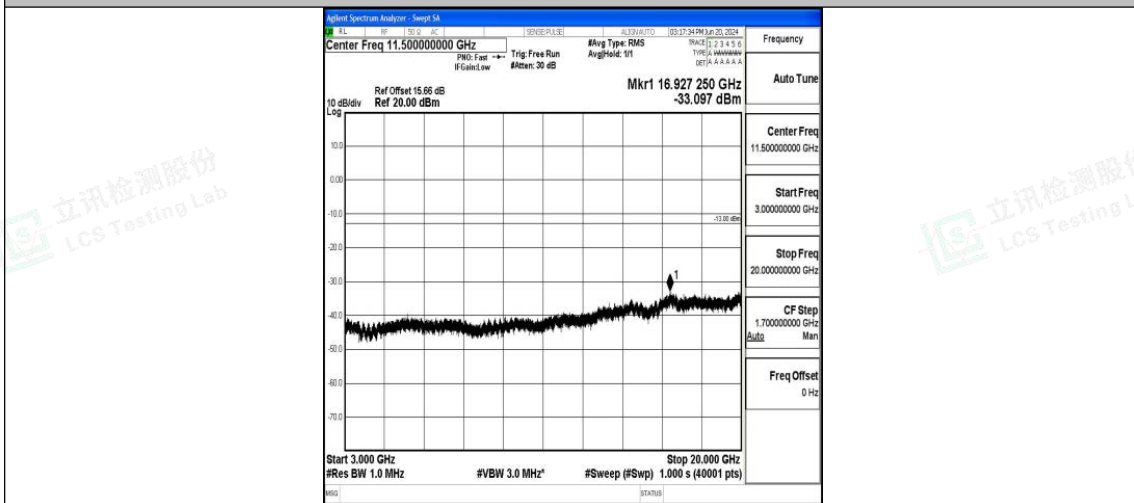
Band25_20MHz_QPSK_26590_1RB#0_3000~20000_3000~20000
