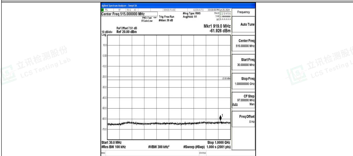
Band25_15MHz_16QAM_26615_1RB#0_30~1000_30~1000
