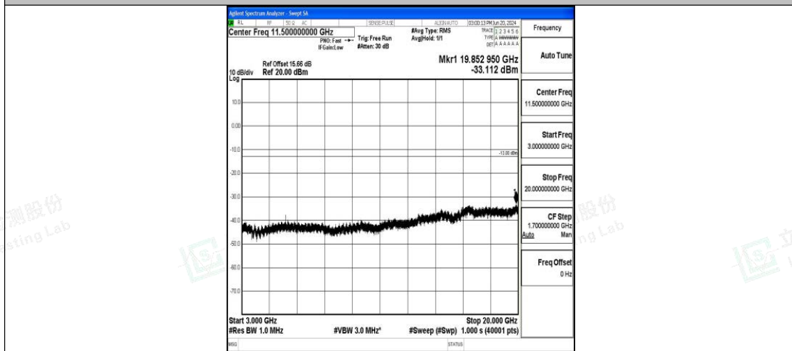
Band25_15MHz_16QAM_26615_1RB#0_3000~20000_3000~20000
