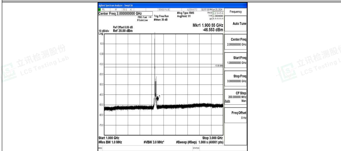
Band25_15MHz_QPSK_26115_1RB#0_1000~3000_1000~3000
