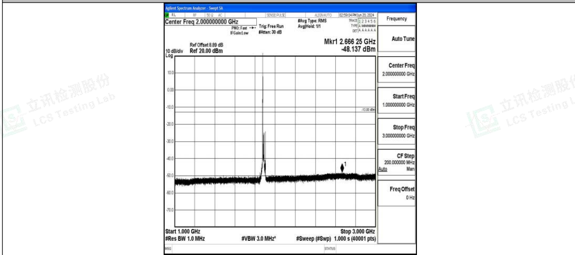
Band25_15MHz_16QAM_26365_1RB#0_1000~3000_1000~3000
