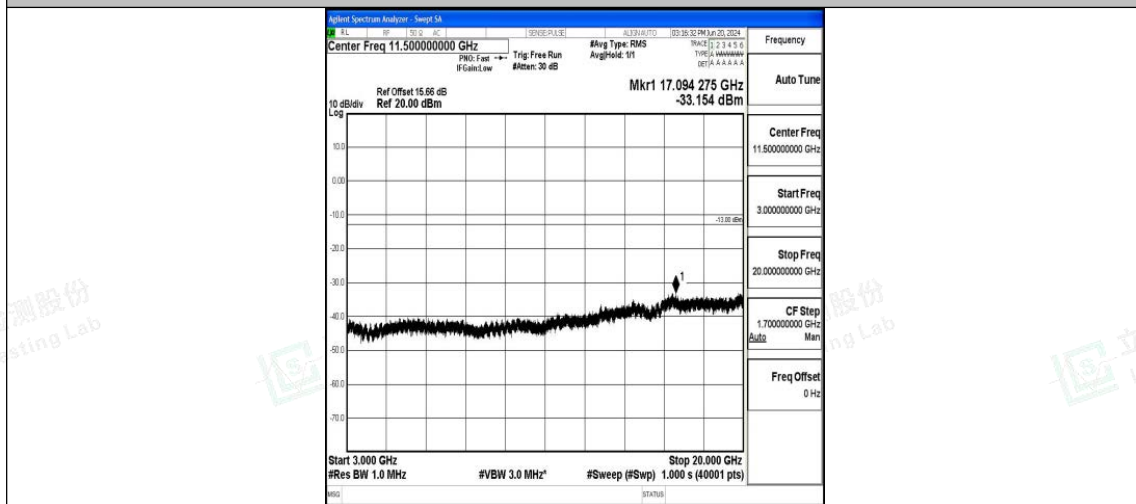
Band25_20MHz_QPSK_26365_1RB#0_3000~20000_3000~20000
