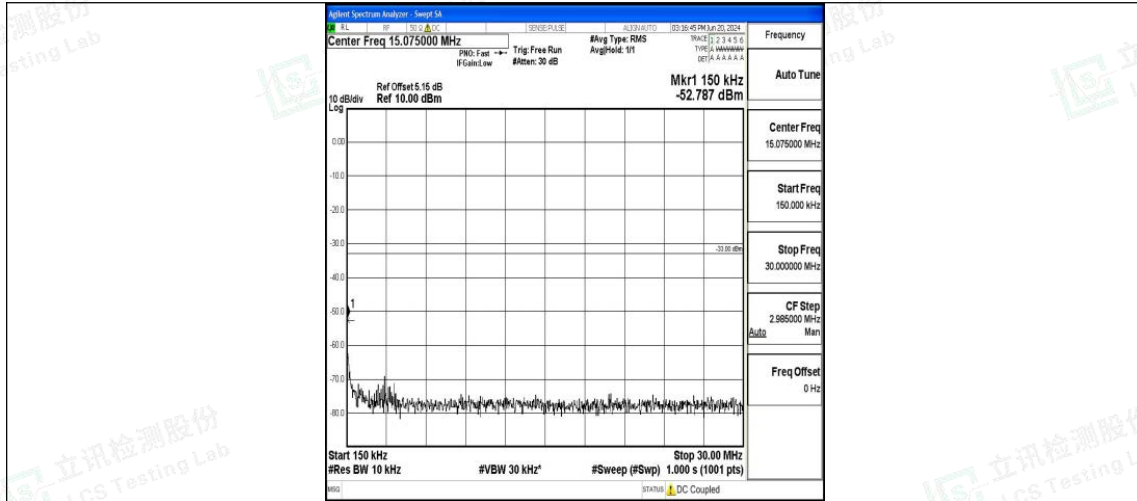
Band25_20MHz_16QAM_26365_1RB#0_0.15~30_0.15~30
