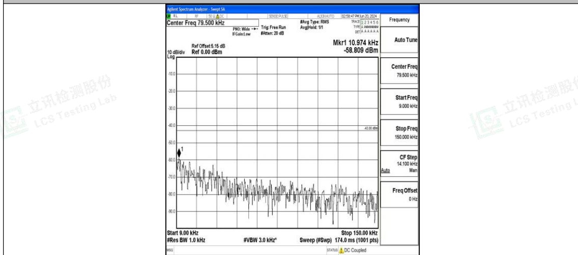
Band25_15MHz_16QAM_26365_1RB#0_0.009~0.15_0.009~0.15
