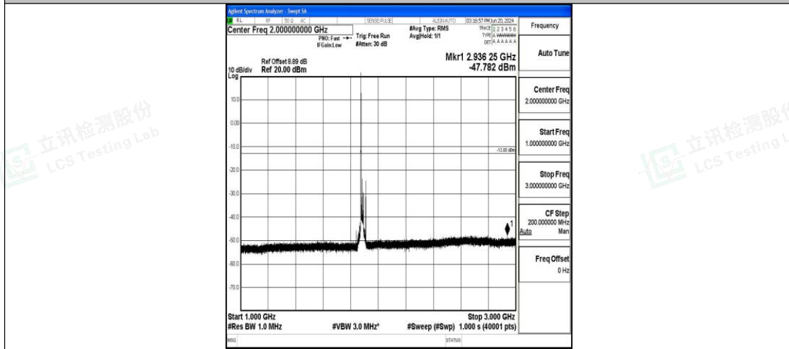
Band25_20MHz_16QAM_26365_1RB#0_1000~3000_1000~3000
