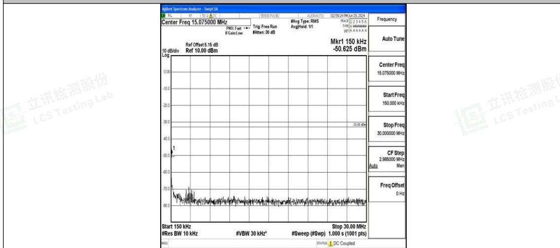
Band25_15MHz_QPSK_26615_1RB#0_0.15~30_0.15~30
