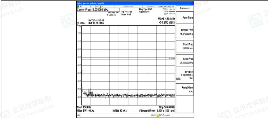
Band25_15MHz_16QAM_26365_1RB#0_0.15~30_0.15~30
