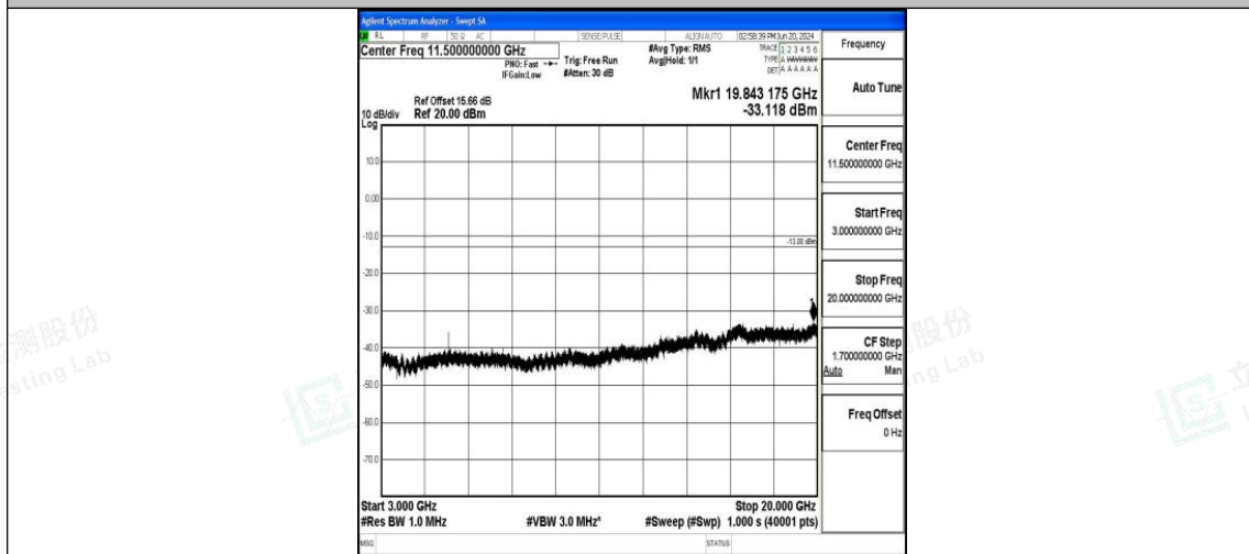
Band25_15MHz_QPSK_26365_1RB#0_3000~20000_3000~20000
