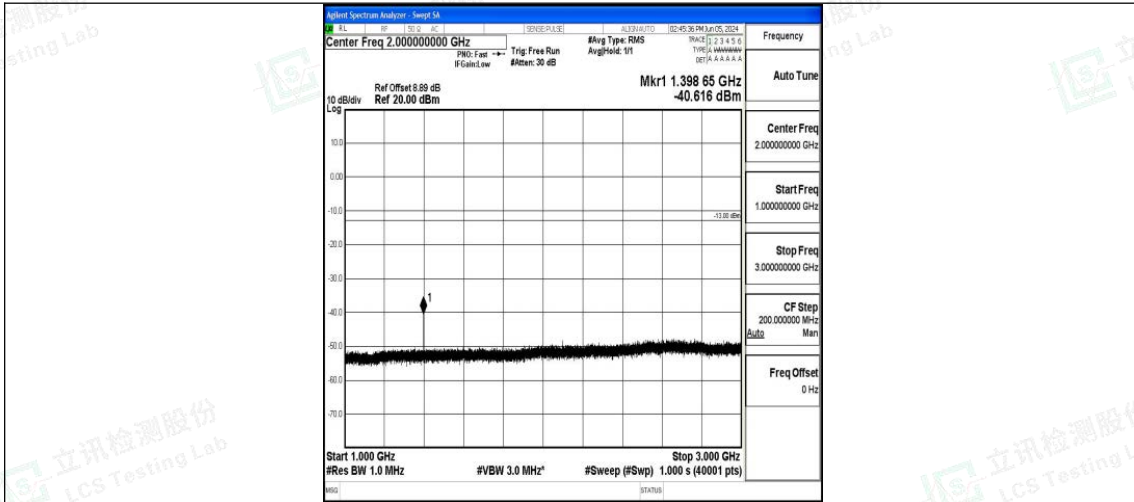
Band12_3MHz_16QAM_23025_1RB#0_1000~3000_1000~3000
