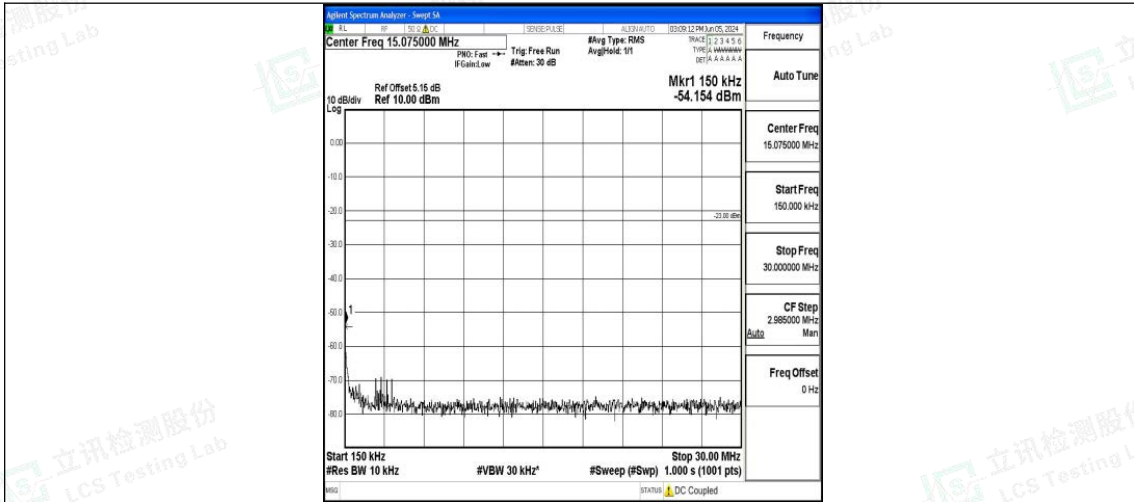
Band12_5MHz_16QAM_23155_1RB#0_0.15~30_0.15~30
