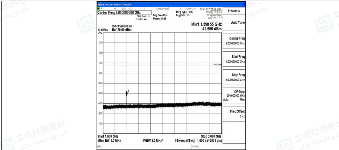
Band12_5MHz_16QAM_23035_1RB#0_1000~3000_1000~3000
