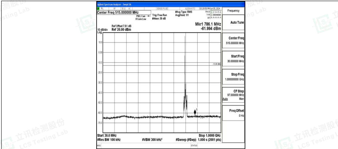
Band12_10MHz_16QAM_23095_1RB#0_30~1000_30~1000
