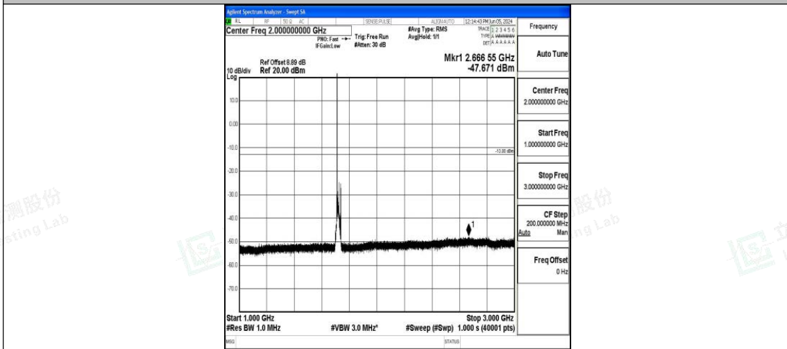
Band4_15MHz_16QAM_2025_1RB#0_1000~3000_1000~3000
