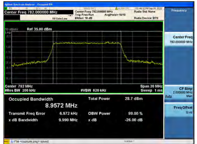
Band13 / 10MHz / 16QAM/ High CH
