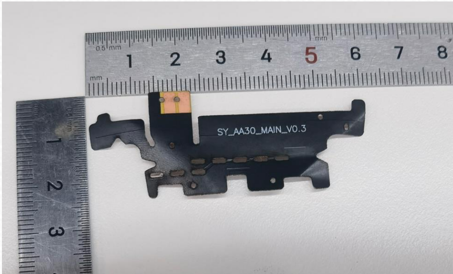
MAIN Antenna
