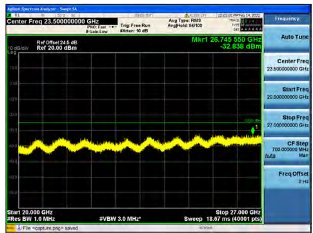
Band41-20G-27G / 10MHz / High CH / 16QAM
