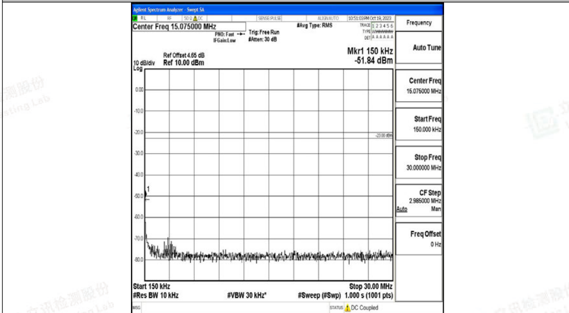
Band26_3MHz_QPSK_26805_1RB#0_0.15~30_0.15~30
