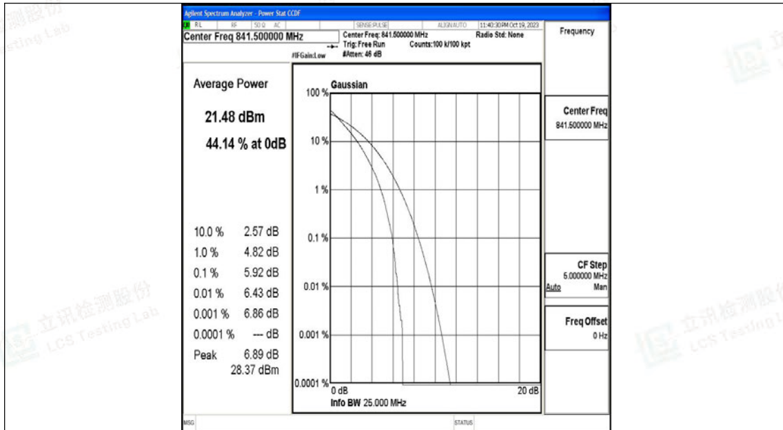
26(824-849)-15MHz-QPSK-26965-75RB#0-PASS
