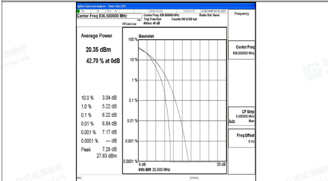
26(824-849)-15MHz-16QAM-26915-75RB#0-PASS
