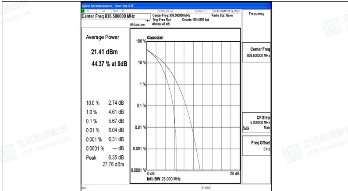
26(824-849)-1.4MHz-QPSK-26915-6RB#0-PASS
