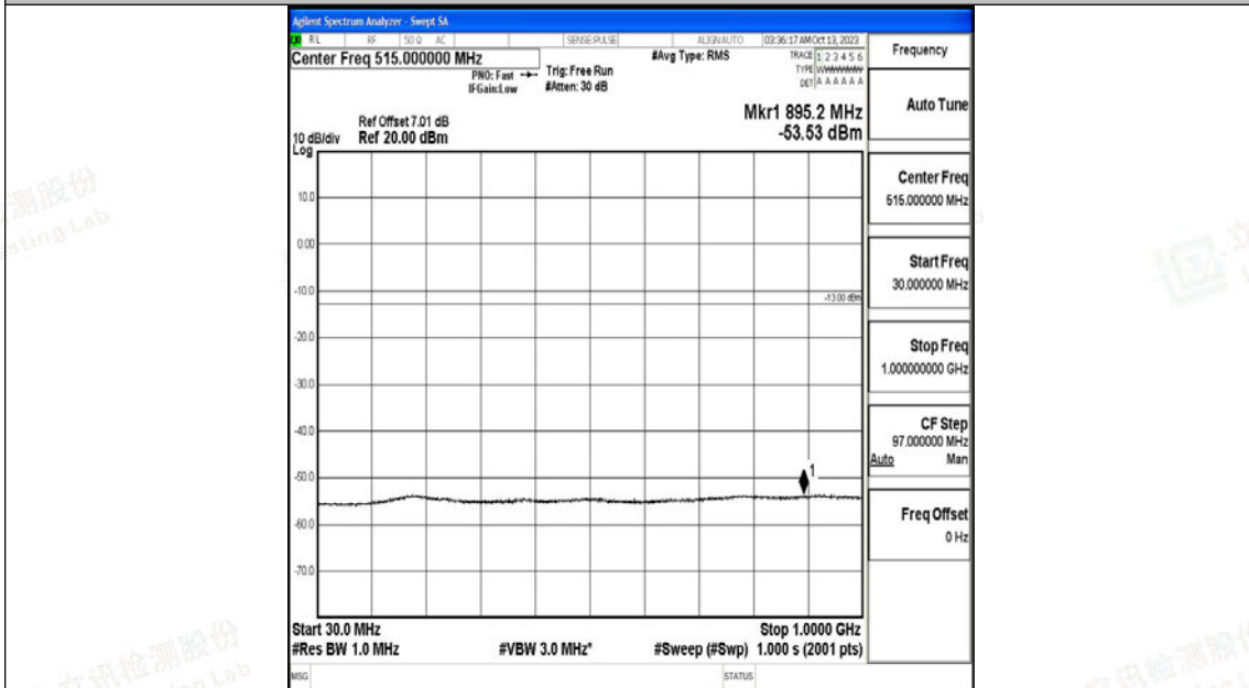
Band2_10MHz_16QAM_18900_1RB#0_30~1000_30~1000
