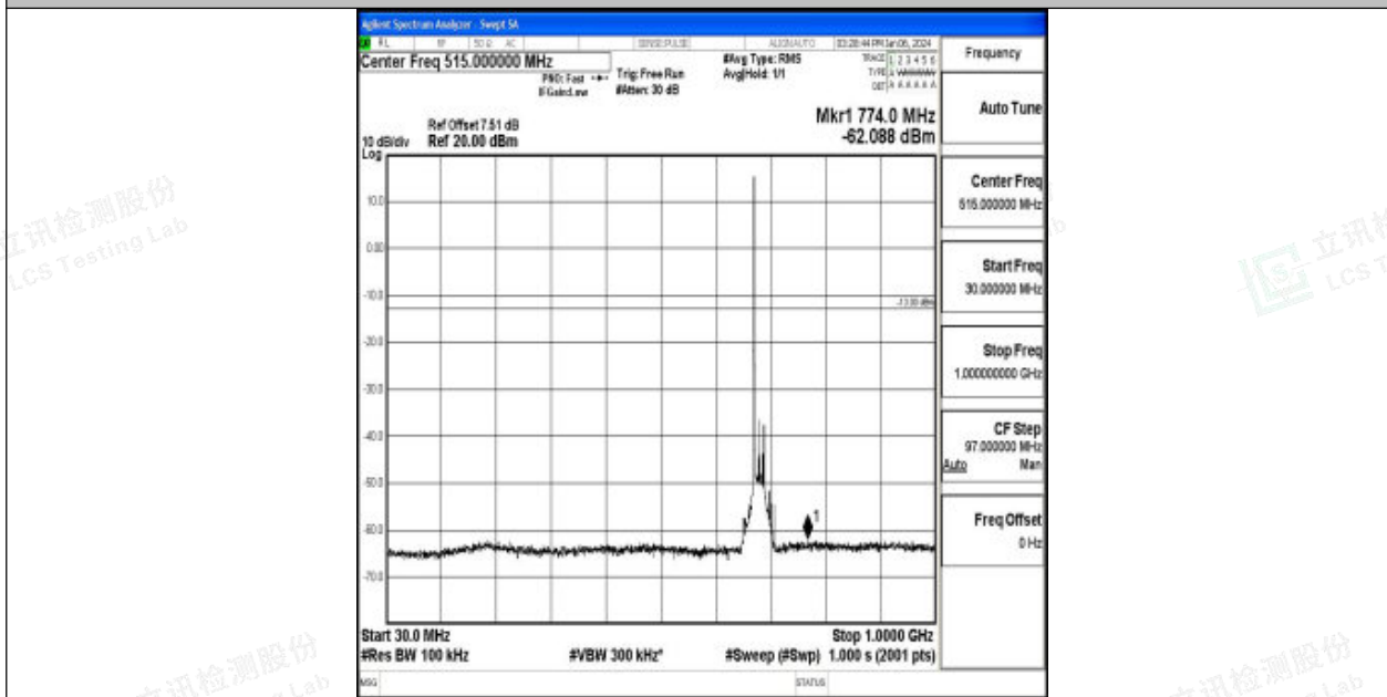
Band71_20MHz_QPSK_133372_1RB#0_30~1000_30~1000
