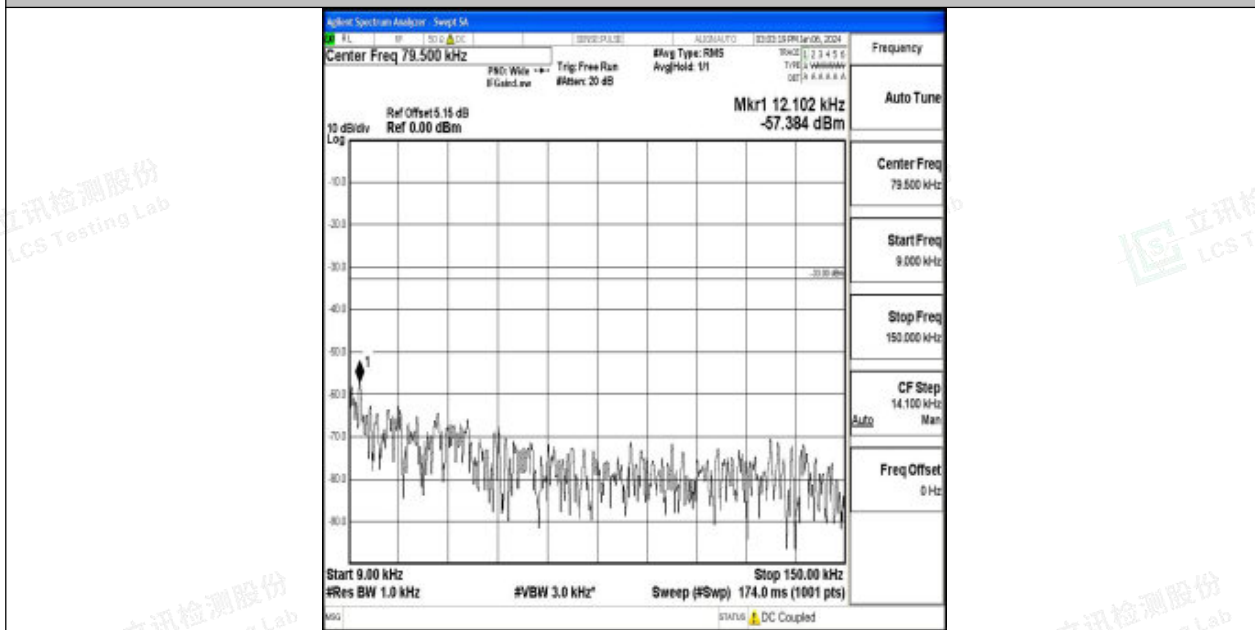
Band71_15MHz_16QAM_133297_1RB#0_0.009~0.15_0.009~0.15
