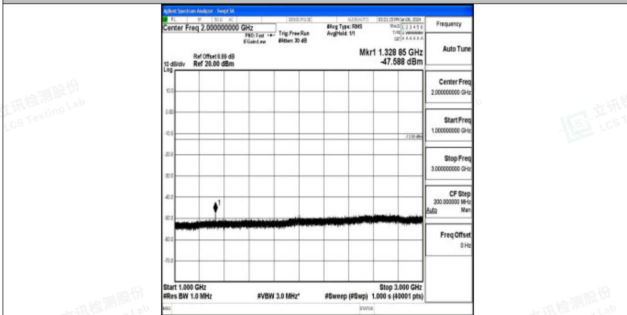
Band71_20MHz_QPSK_133222_1RB#0_1000~3000_1000~3000
