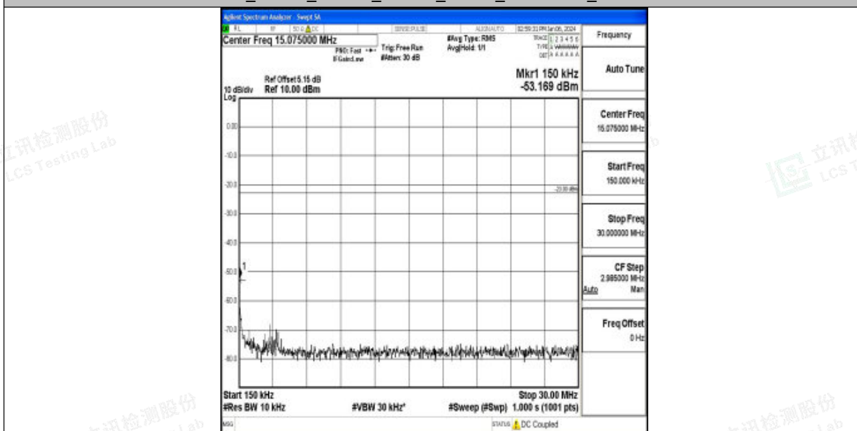
Band71_15MHz_16QAM_133197_1RB#0_0.15~30_0.15~30
