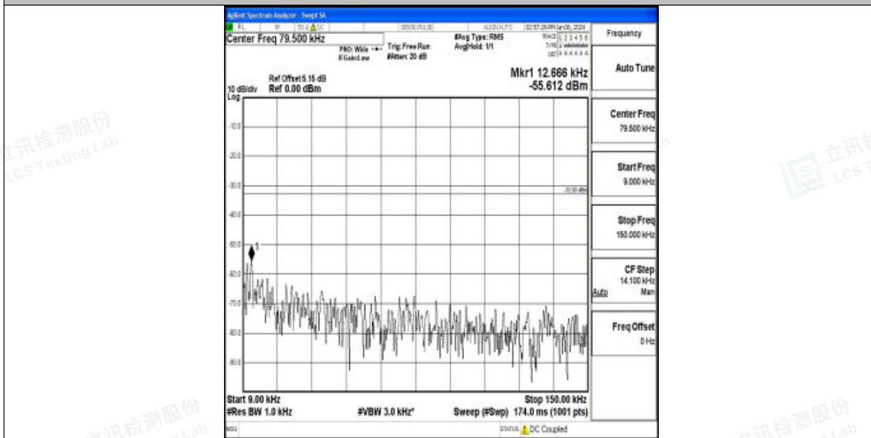
Band71_15MHz_QPSK_133197_1RB#0_0.009~0.15_0.009~0.15
