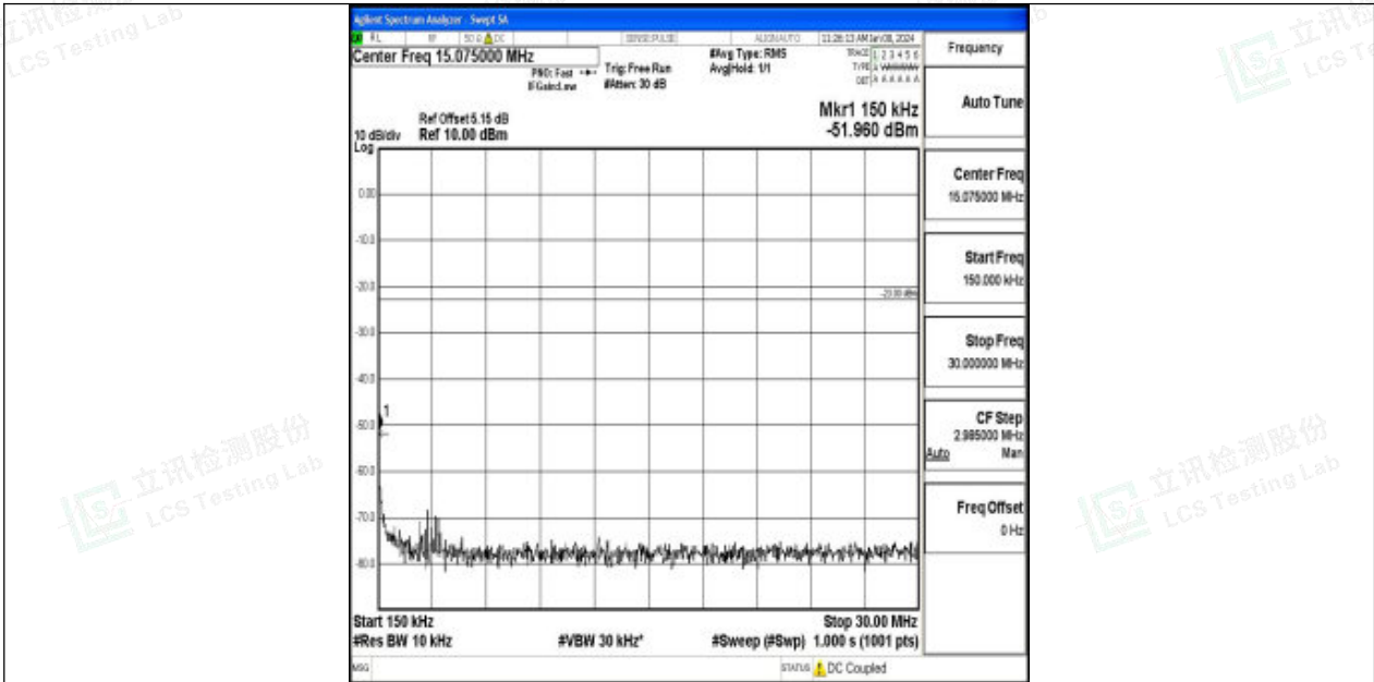
Band71_5MHz_16QAM_133297_1RB#0_0.15~30_0.15~30
