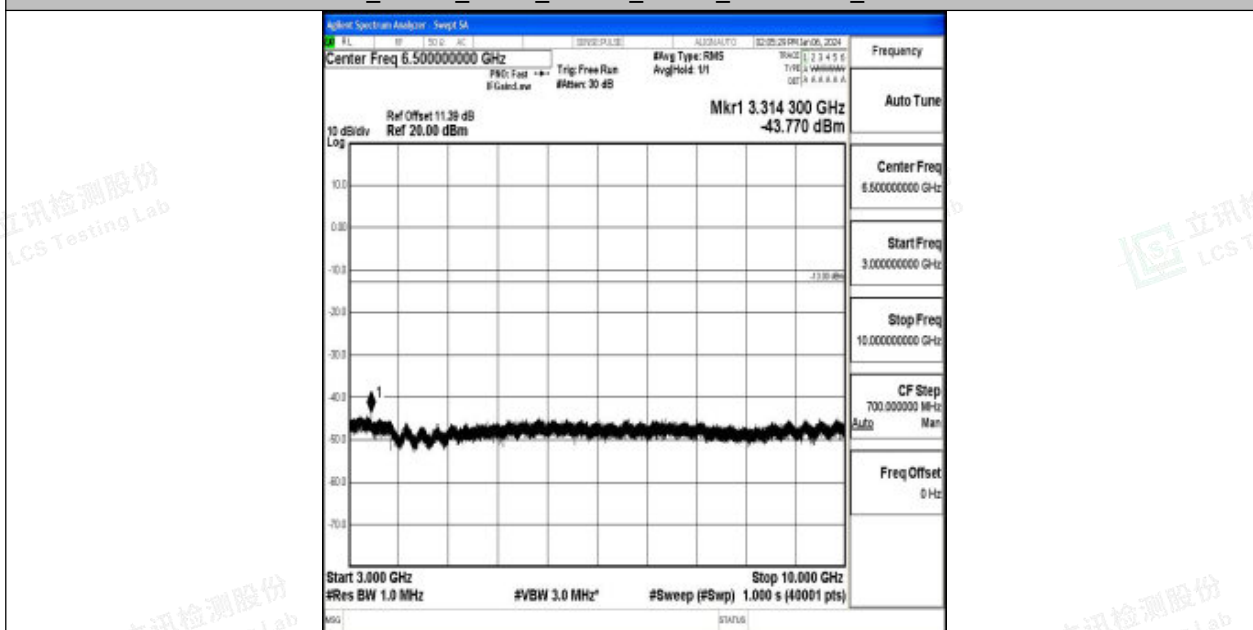
Band71_10MHz_QPSK_133422_1RB#0_3000~10000_3000~10000
