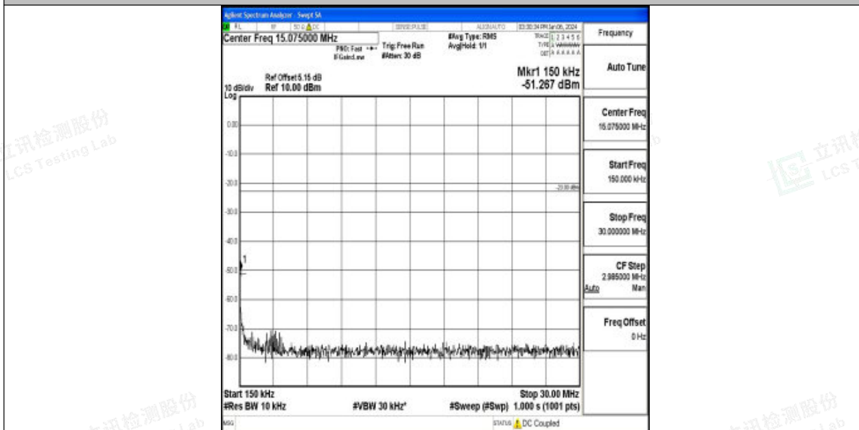
Band71_20MHz_16QAM_133372_1RB#0_0.15~30_0.15~30
