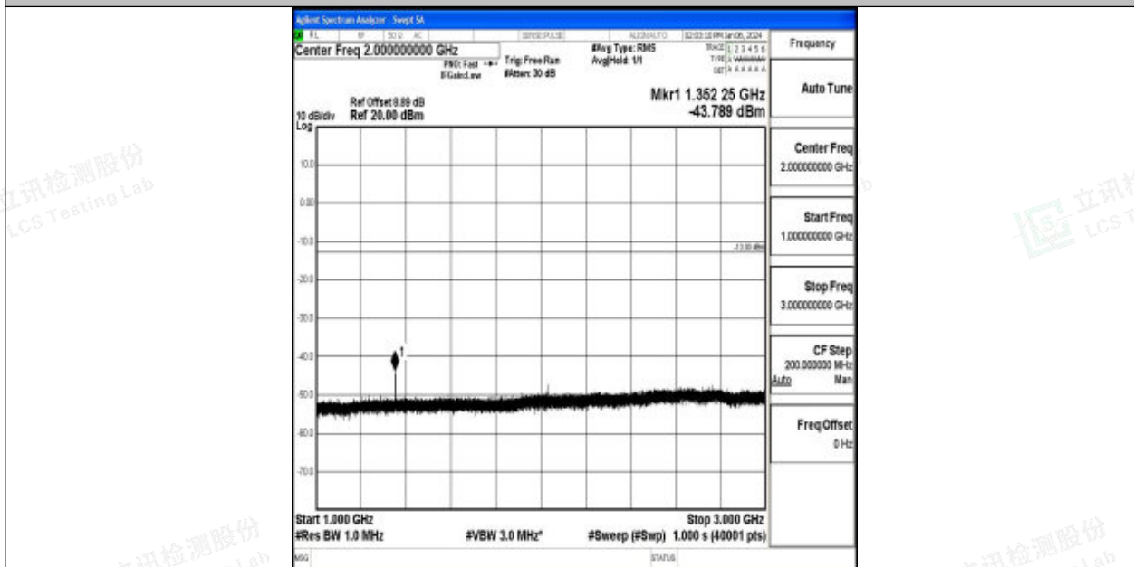
Band71_10MHz_16QAM_133297_1RB#0_1000~3000_1000~3000
