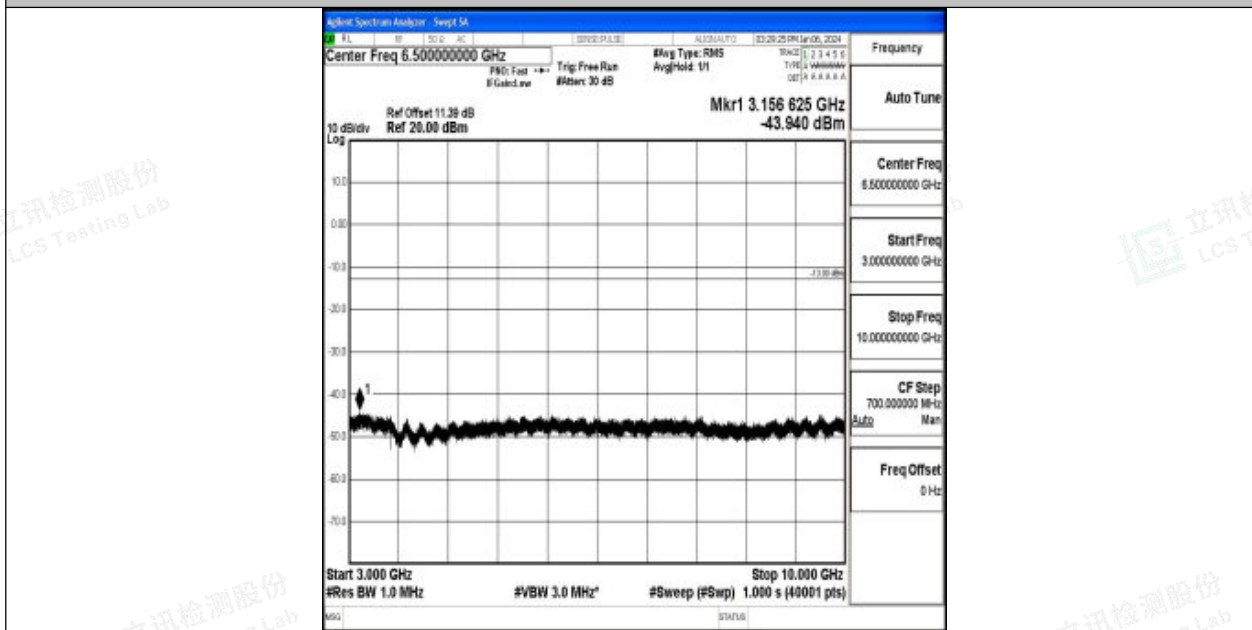
Band71_20MHz_QPSK_133372_1RB#0_3000~10000_3000~10000
