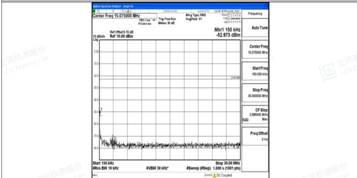
Band71_10MHz_16QAM_133422_1RB#0_0.15~30_0.15~30
