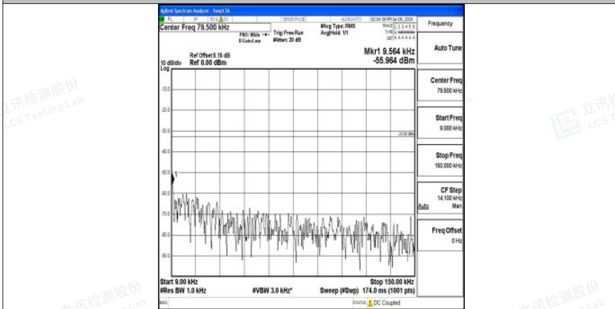
Band71_10MHz_QPSK_133422_1RB#0_0.009~0.15_0.009~0.15
