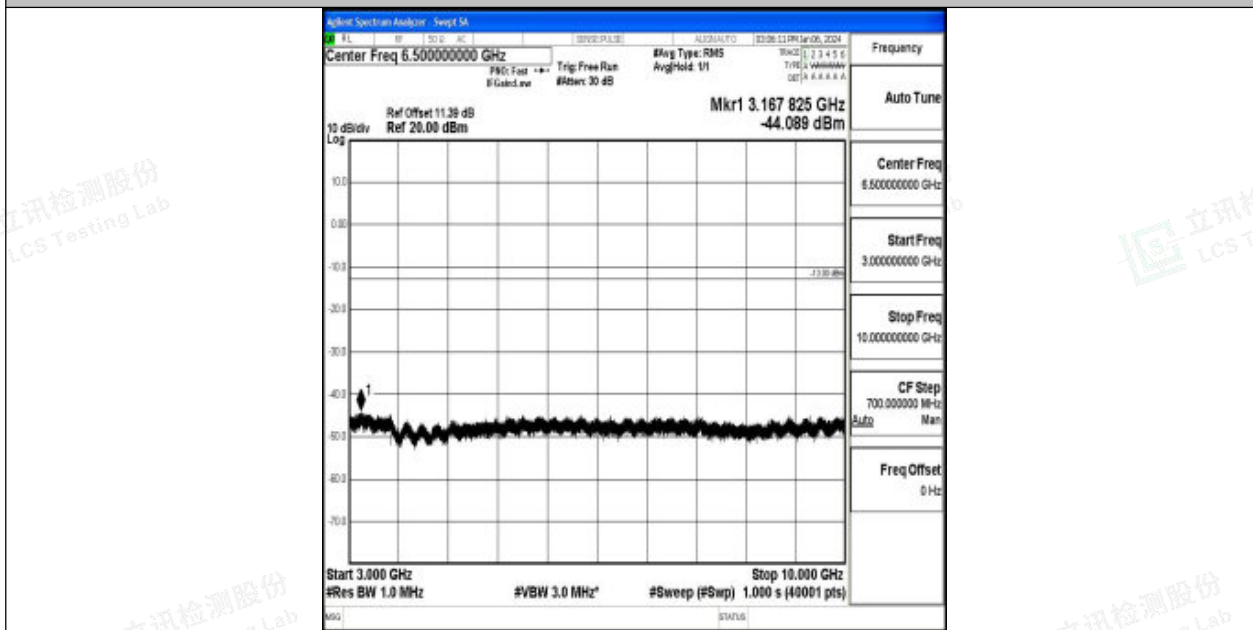
Band71_15MHz_QPSK_133397_1RB#0_3000~10000_3000~10000
