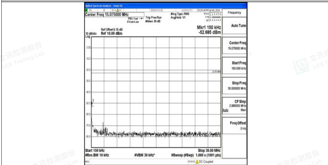
Band71_20MHz_QPSK_133222_1RB#0_0.15~30_0.15~30
