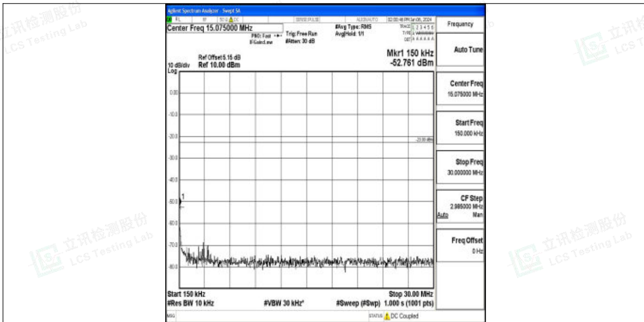
Band71_10MHz_QPSK_133297_1RB#0_0.15~30_0.15~30
