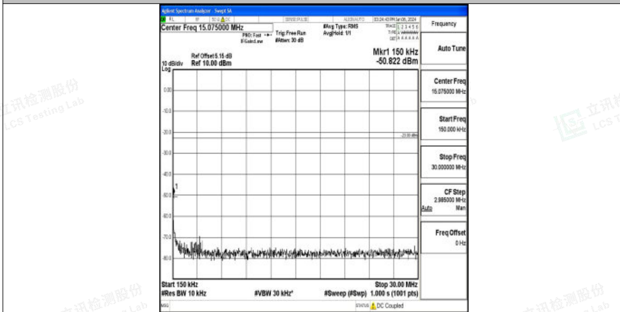
Band71_20MHz_QPSK_133322_1RB#0_0.15~30_0.15~30
