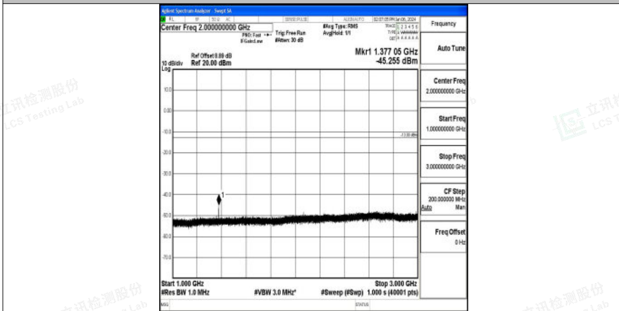
Band71_10MHz_16QAM_133422_1RB#0_1000~3000_1000~3000
