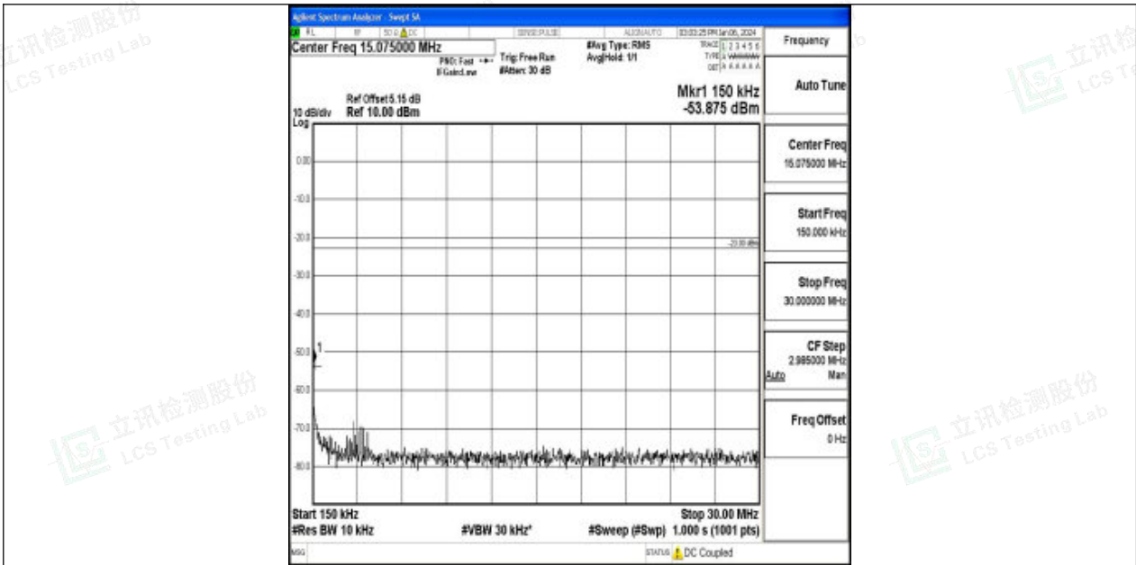
Band71_15MHz_16QAM_133297_1RB#0_0.15~30_0.15~30
