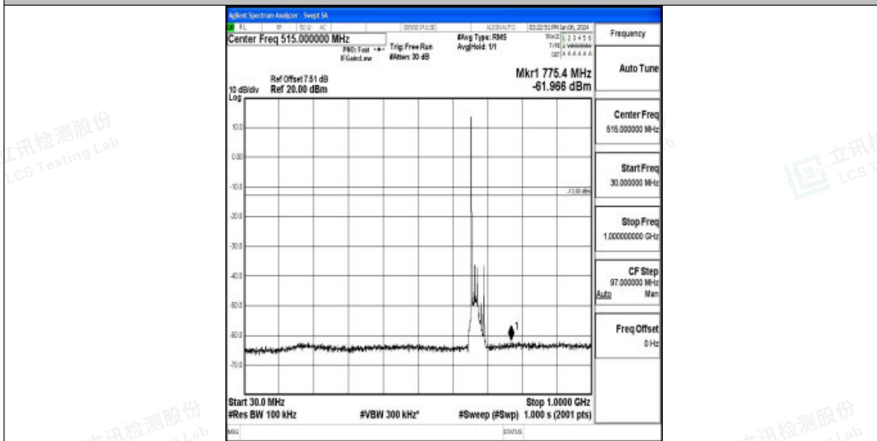
Band71_20MHz_16QAM_133222_1RB#0_30~1000_30~1000
