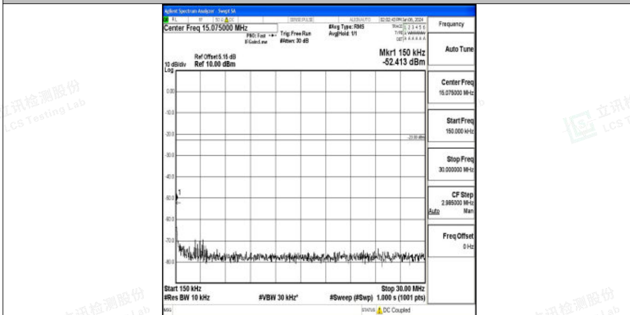
Band71_10MHz_16QAM_133297_1RB#0_0.15~30_0.15~30
