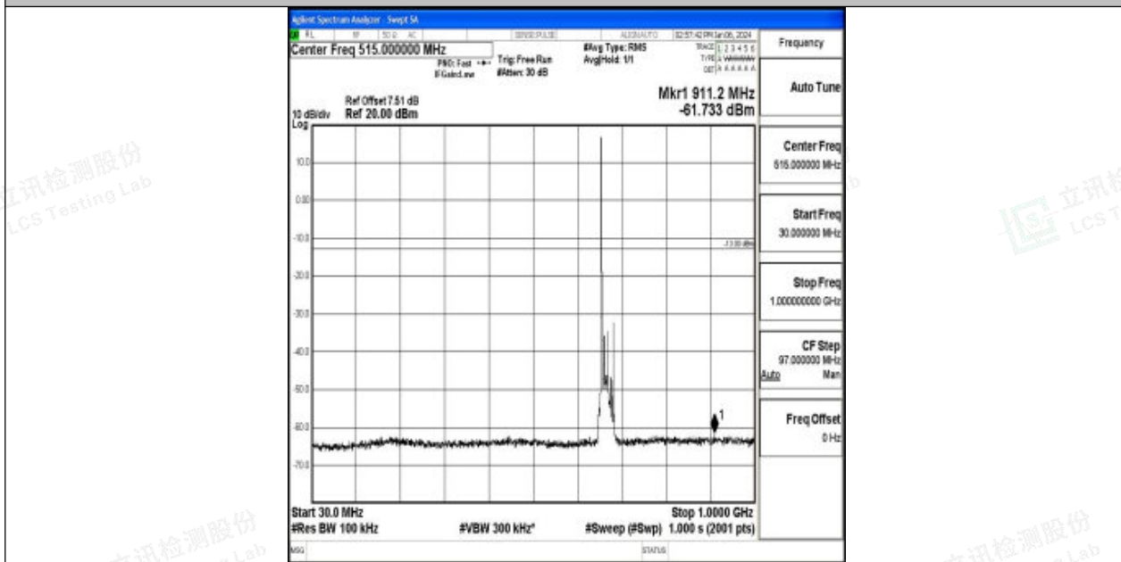
Band71_15MHz_QPSK_133197_1RB#0_30~1000_30~1000
