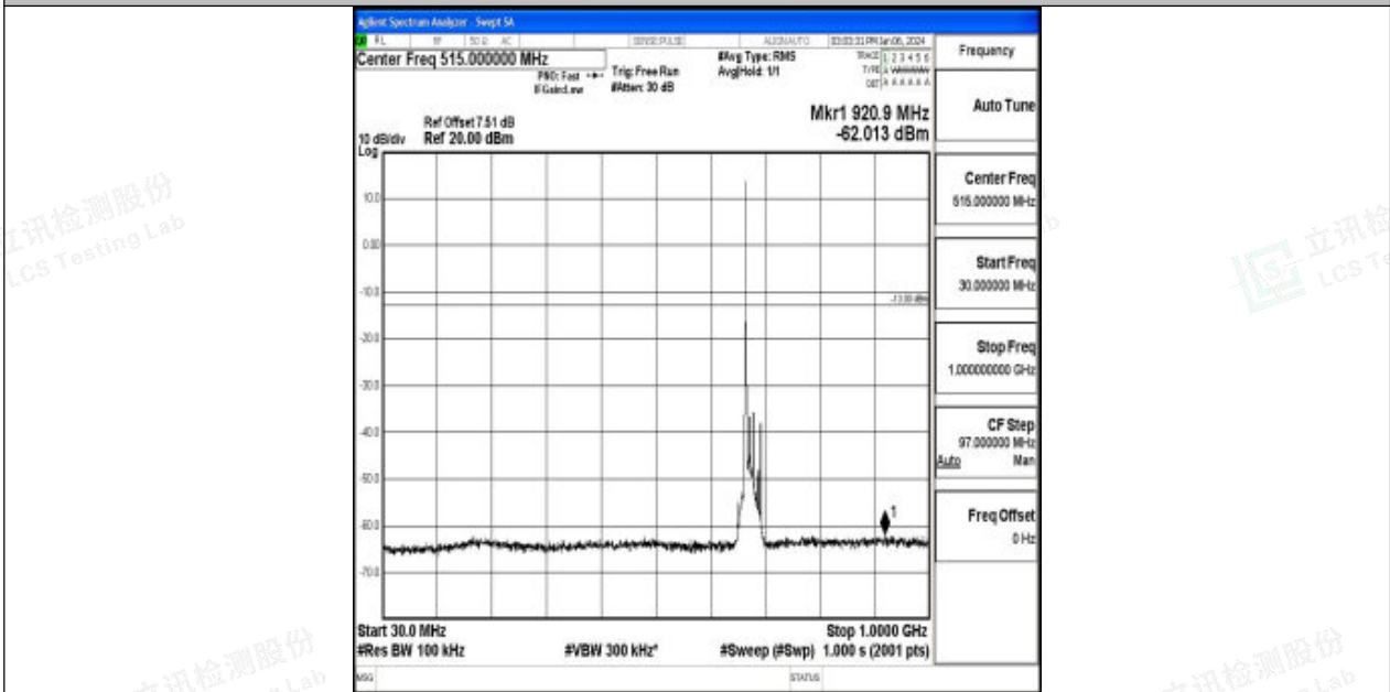
Band71_15MHz_16QAM_133297_1RB#0_30~1000_30~1000
