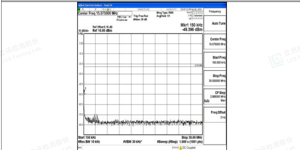
Band71_15MHz_16QAM_133397_1RB#0_0.15~30_0.15~30
