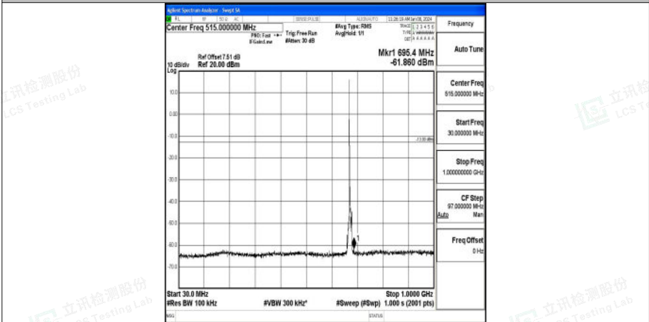
Band71_5MHz_16QAM_133297_1RB#0_30~1000_30~1000
