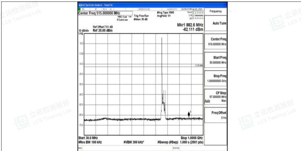
Band71_15MHz_16QAM_133197_1RB#0_30~1000_30~1000
