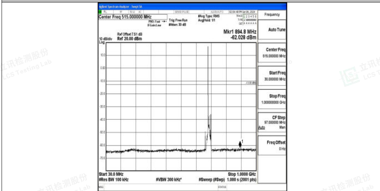
Band71_10MHz_QPSK_133422_1RB#0_30~1000_30~1000
