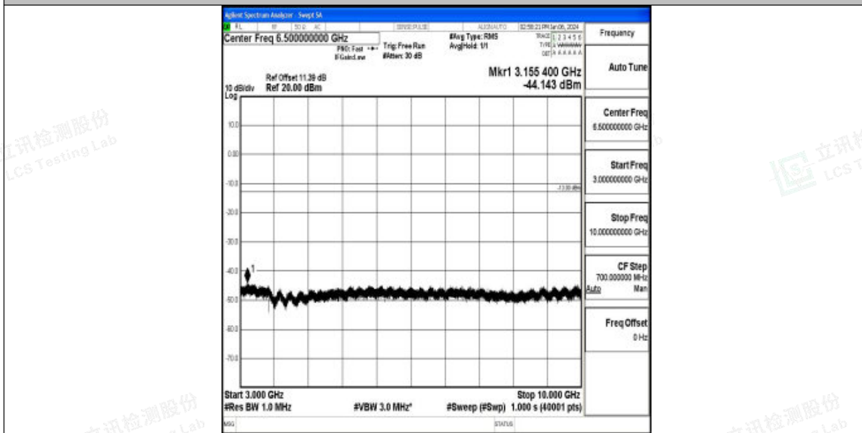
Band71_15MHz_QPSK_133197_1RB#0_3000~10000_3000~10000
