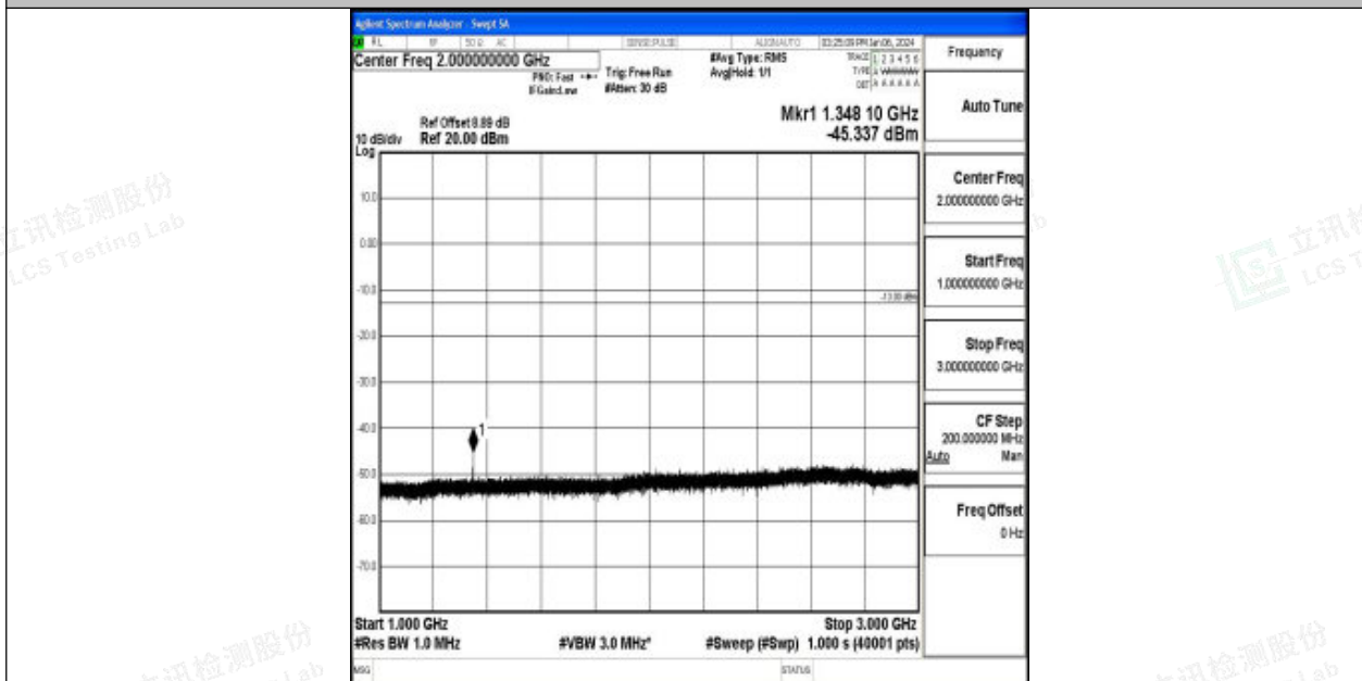
Band71_20MHz_QPSK_133322_1RB#0_1000~3000_1000~3000
