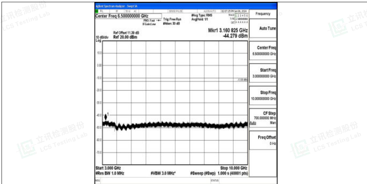
Band71_10MHz_16QAM_133422_1RB#0_3000~10000_3000~10000
