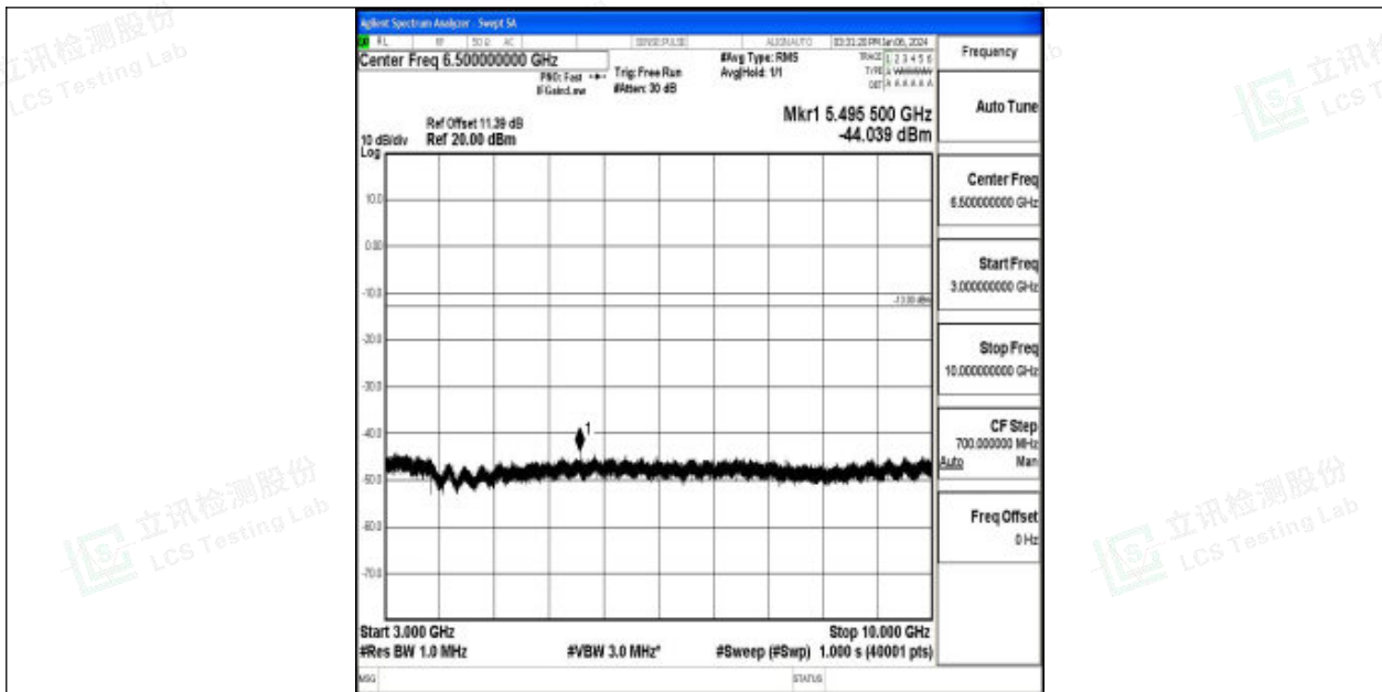
Band71_20MHz_16QAM_133372_1RB#0_3000~10000_3000~10000
