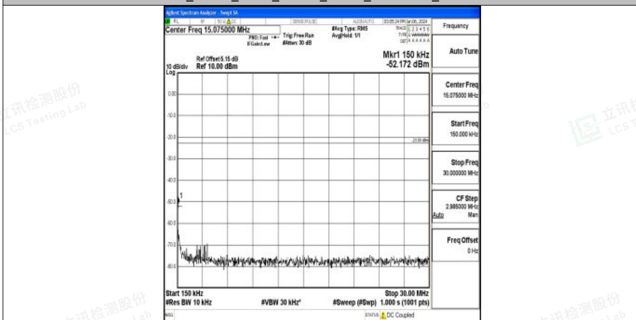
Band71_15MHz_QPSK_133397_1RB#0_0.15~30_0.15~30
