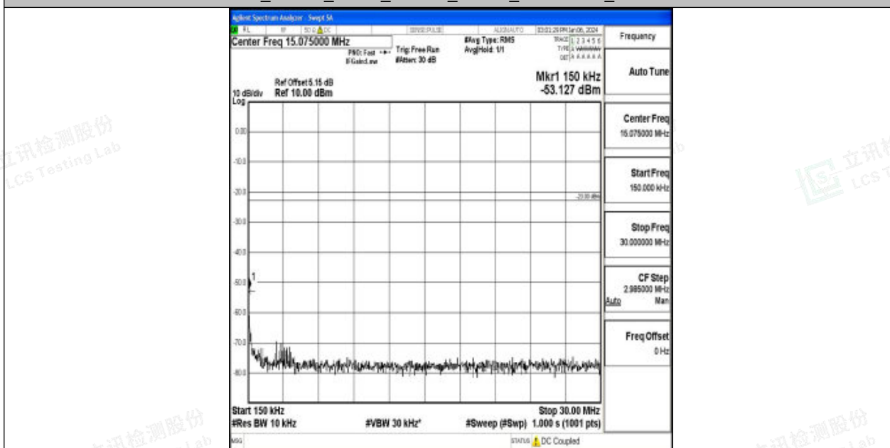
Band71_15MHz_QPSK_133297_1RB#0_0.15~30_0.15~30
