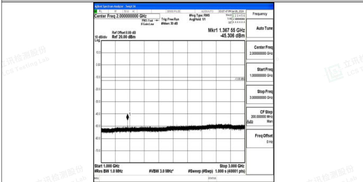
Band71_15MHz_16QAM_133397_1RB#0_1000~3000_1000~3000
